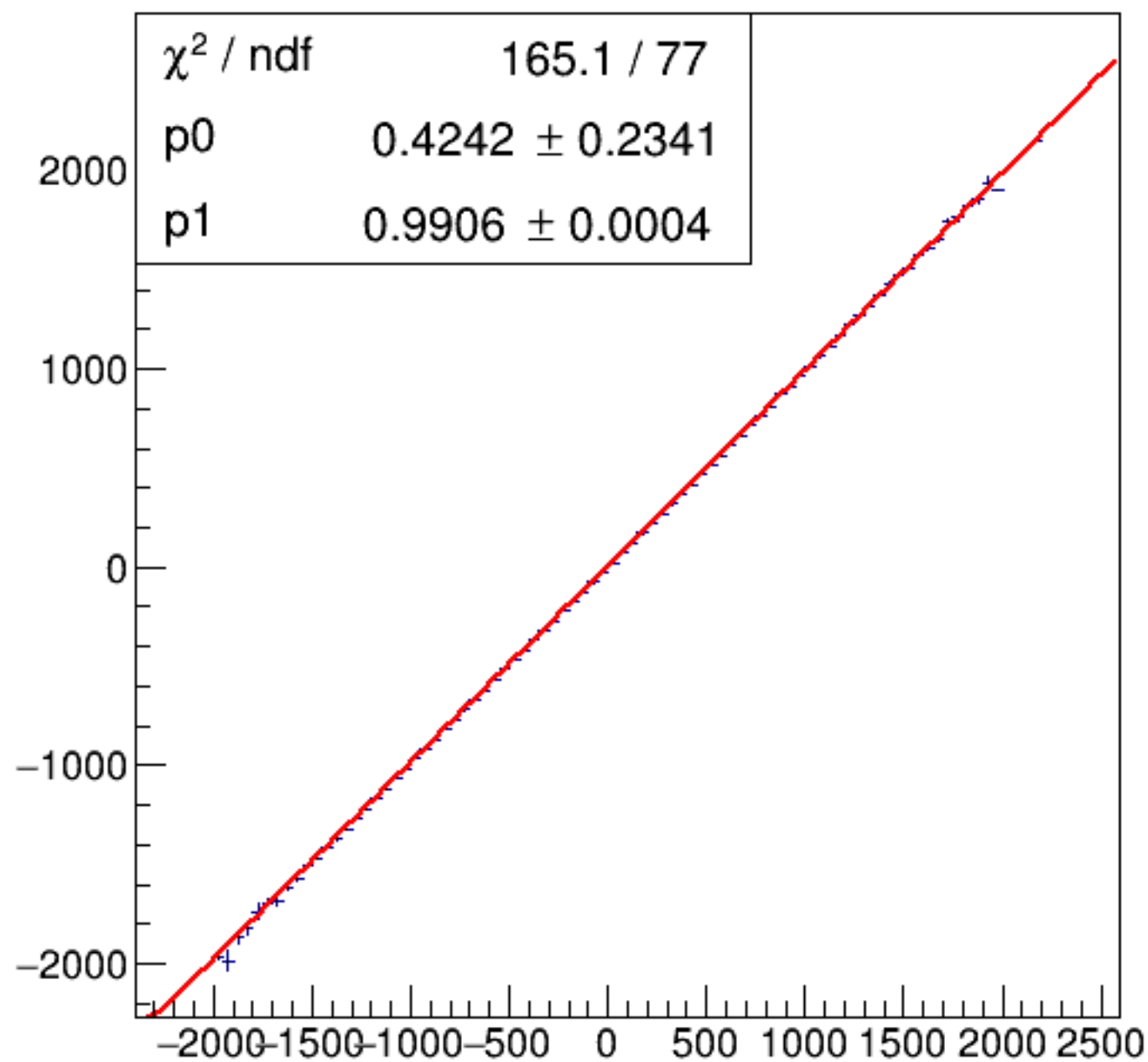
run6346_000_asym_bcm_dg_us_vs_asym_bcm_dg_ds_pr.png
