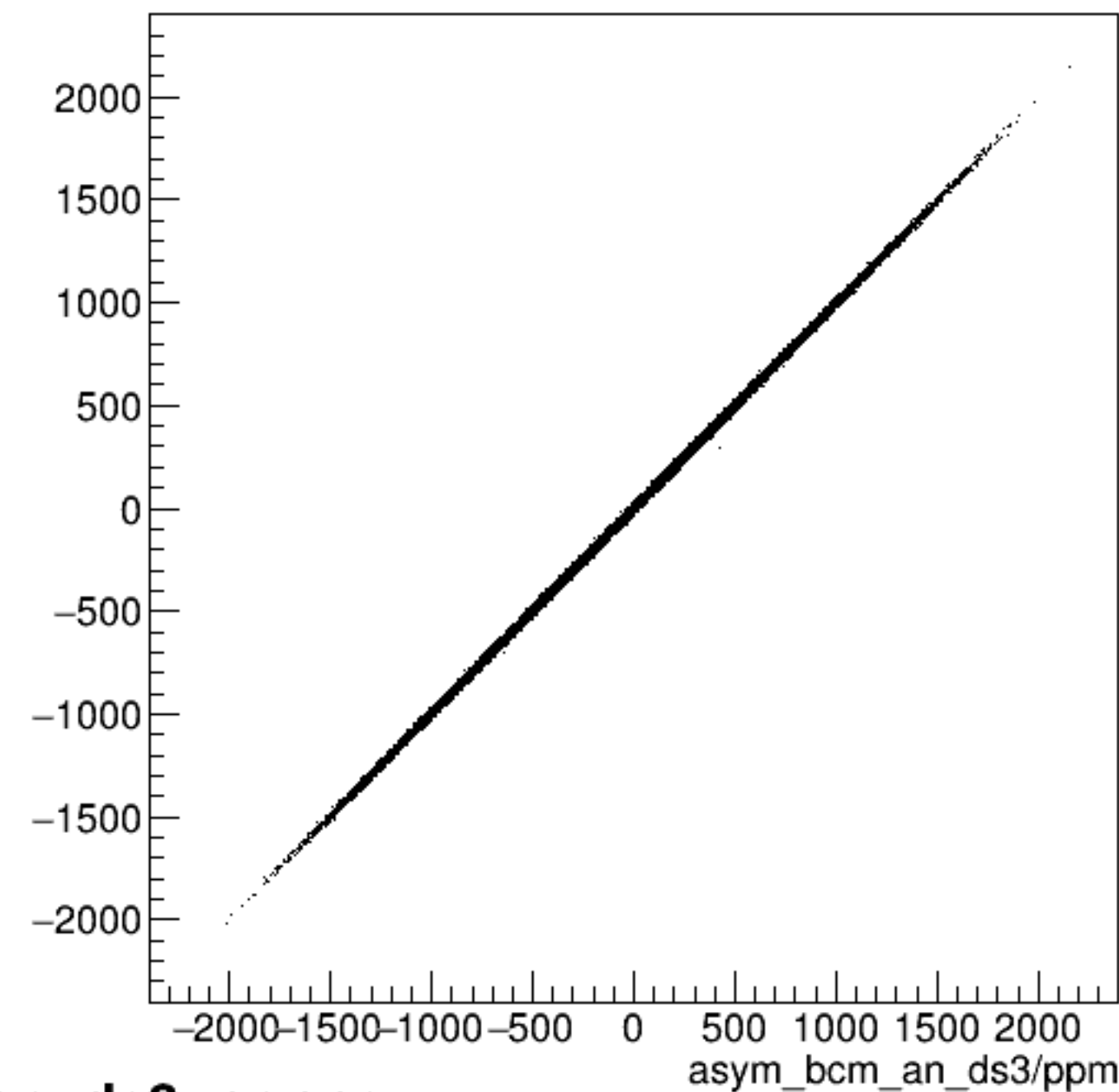
run6346_000_asym_bcm_an_ds_vs_asym_bcm_an_ds3_pr.png
