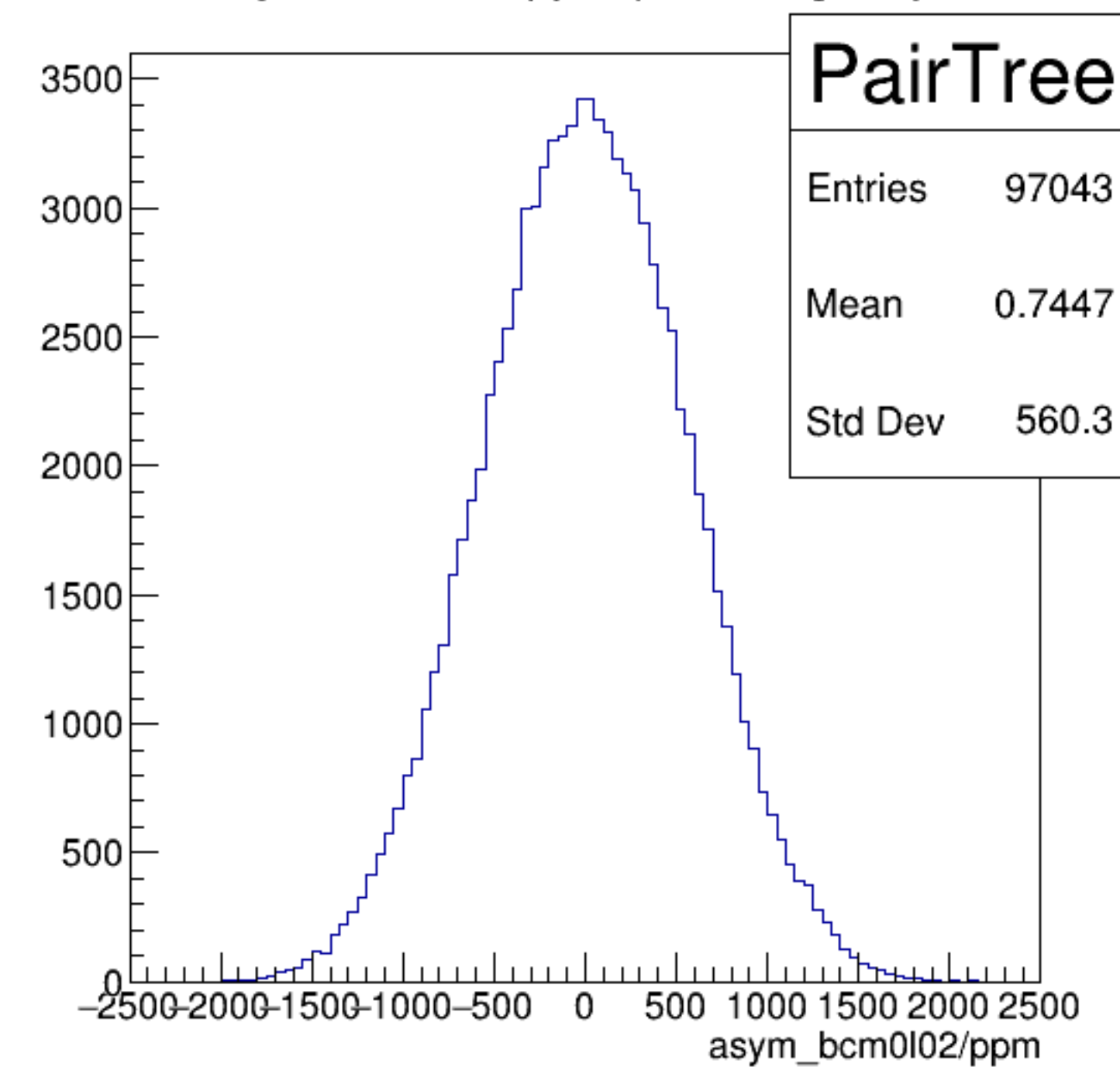
asym_bcm0l02/ppm {ErrorFlag==0}
