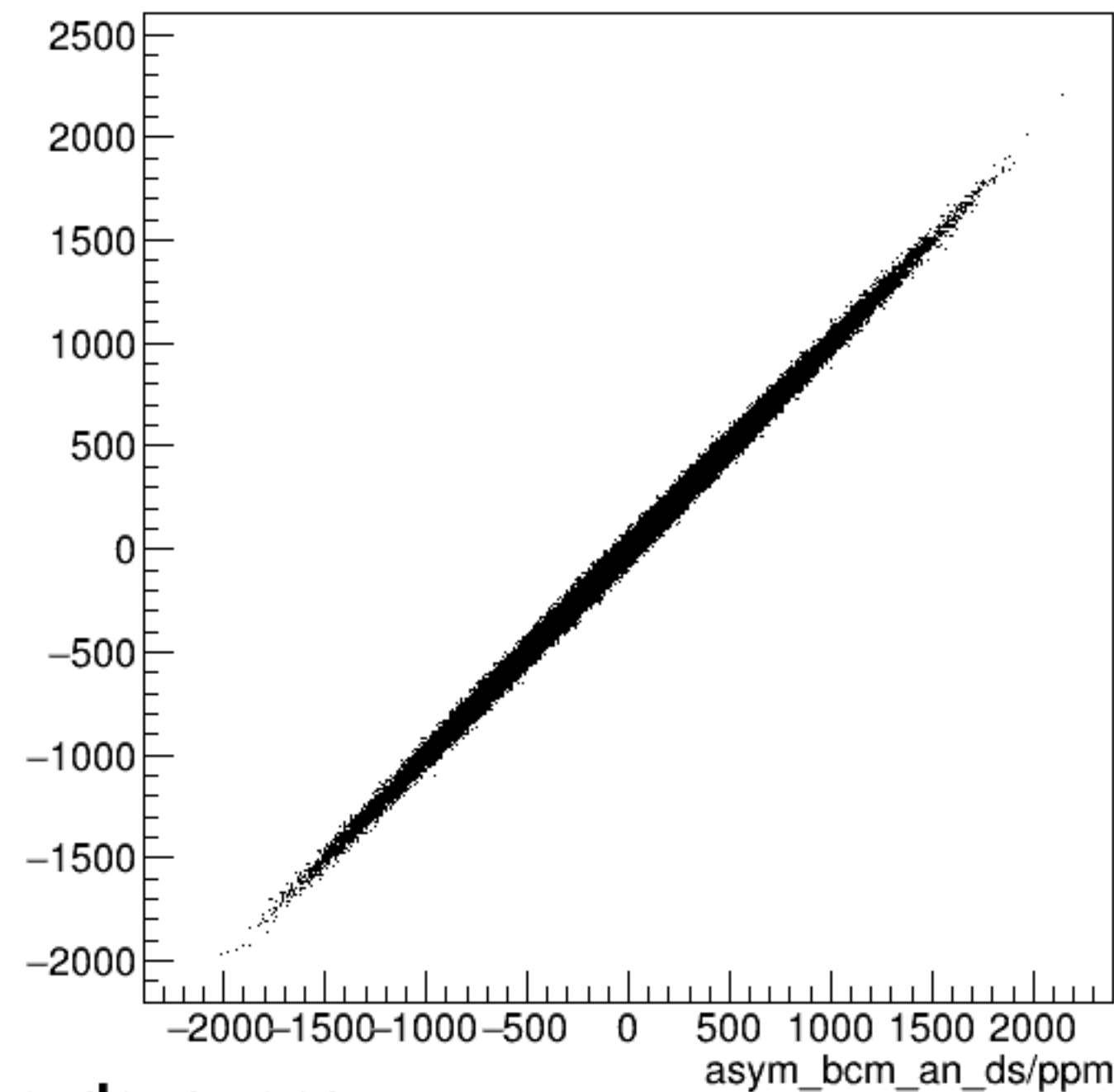
run6346_000_asym_bcm_an_us_vs_asym_bcm_an_ds_pr.png
