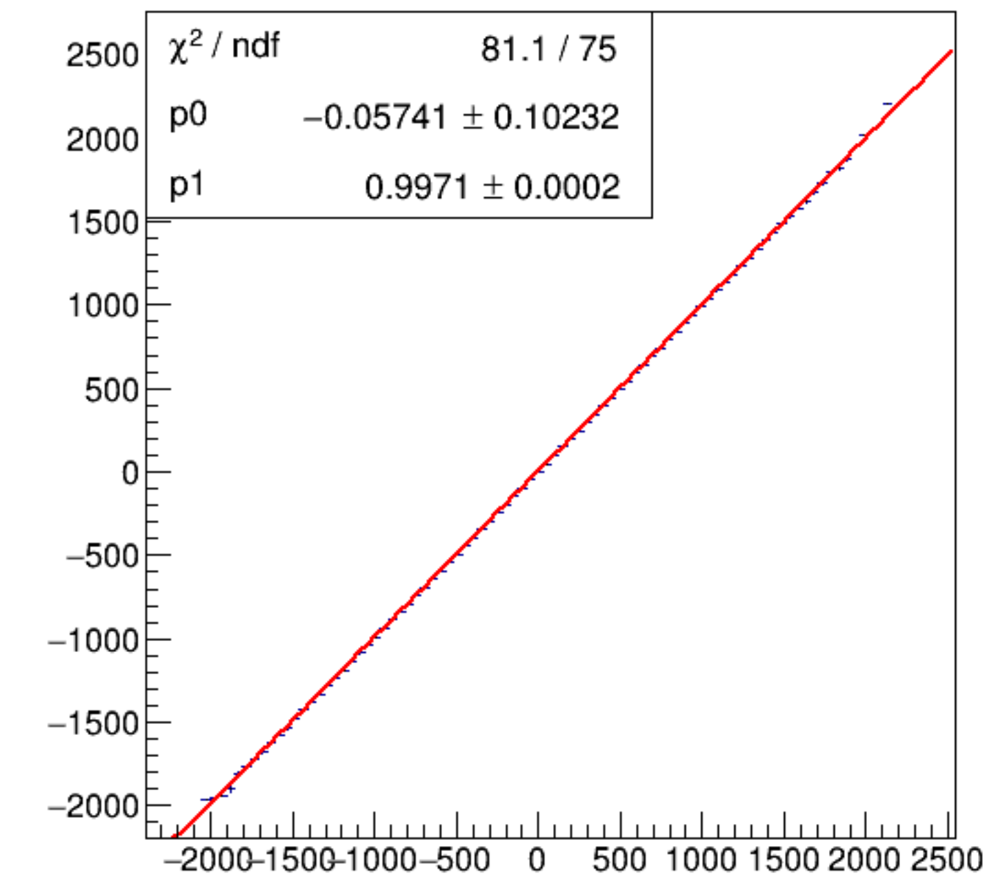
run6346_000_asym_bcm_an_us_vs_asym_bcm_an_ds3_pr.png
