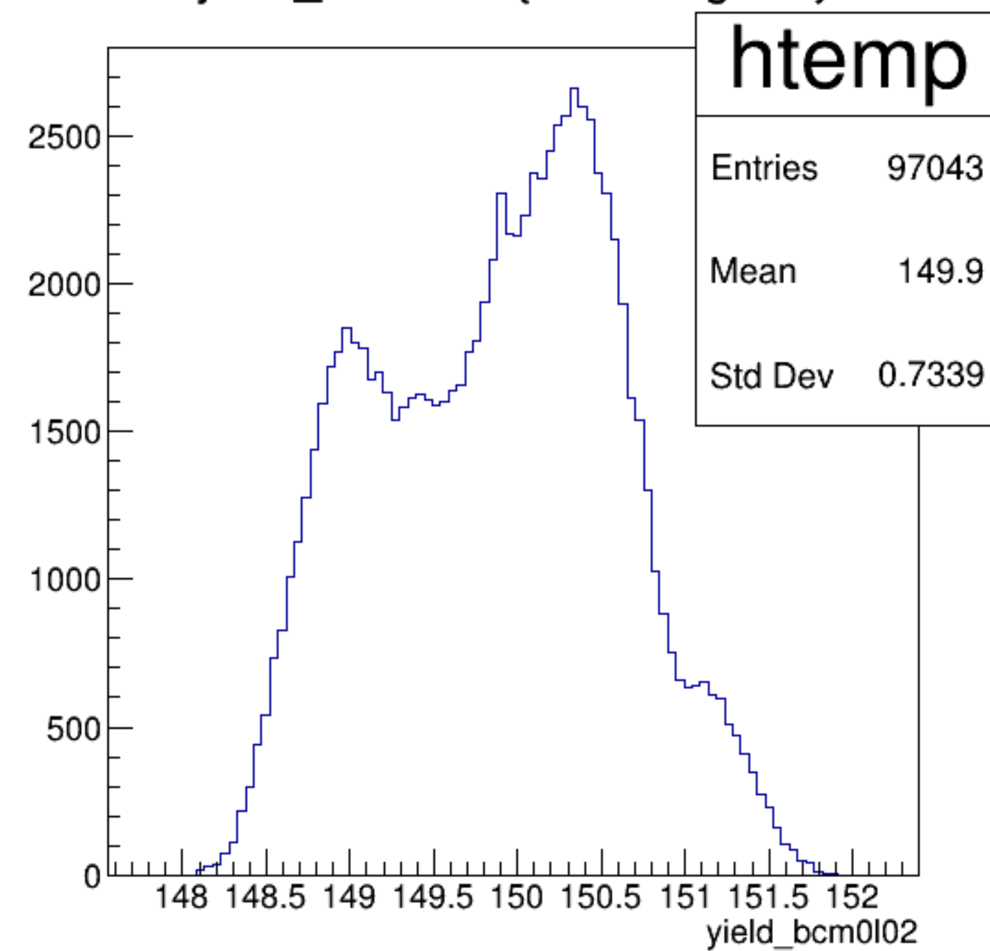
yield_bcm0l02 {ErrorFlag==0}
