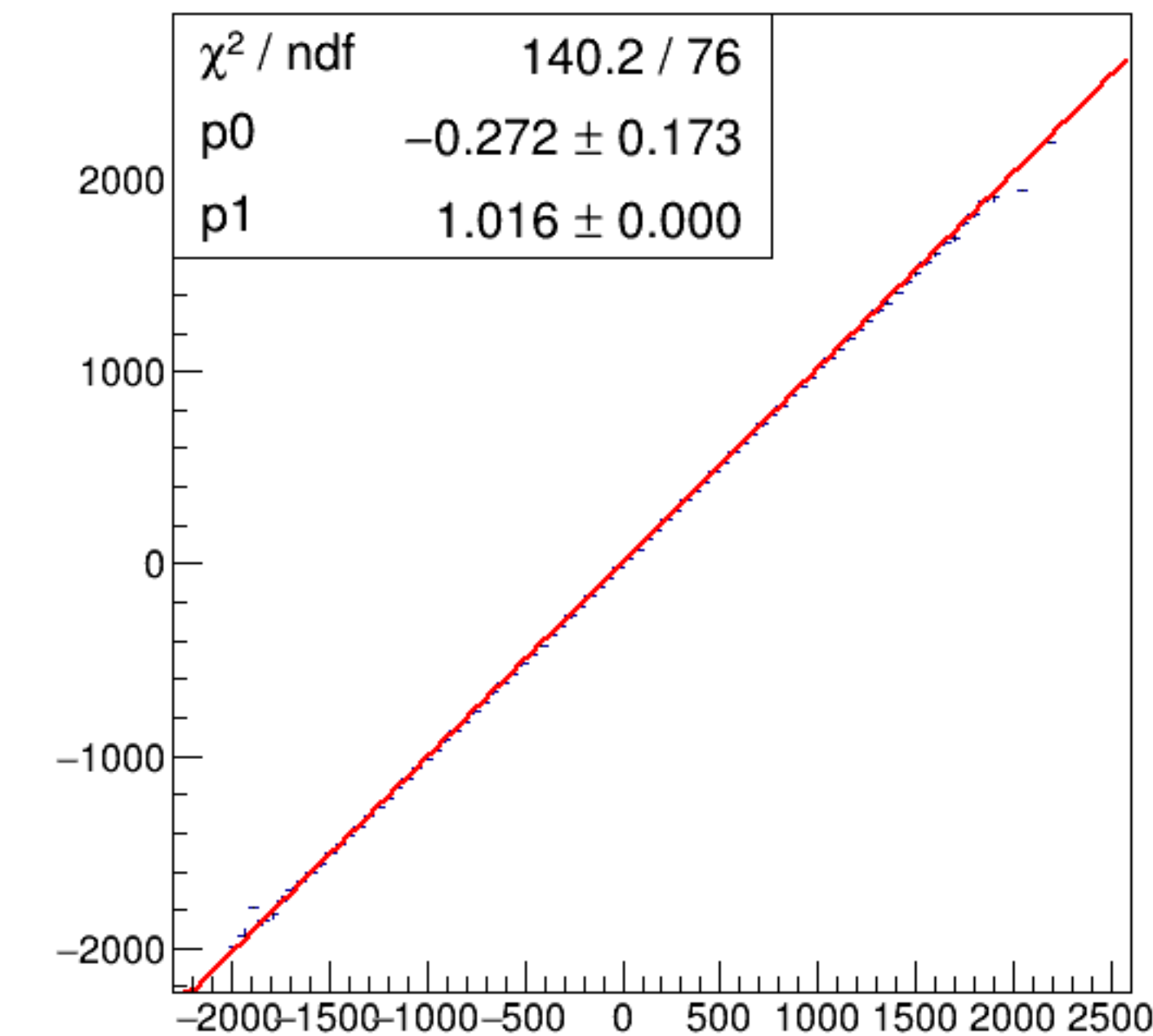
run6346_000_asym_bcm_dg_ds_vs_asym_bcm_an_us_pr.png
