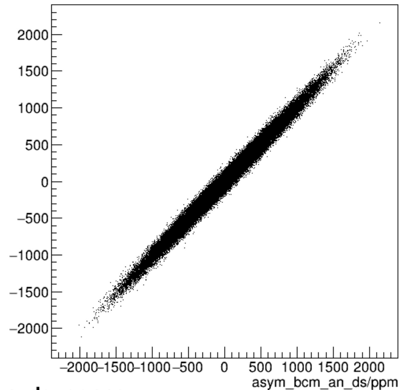
run6346_000_asym_bcm_dg_us_vs_asym_bcm_an_ds_pr.png
