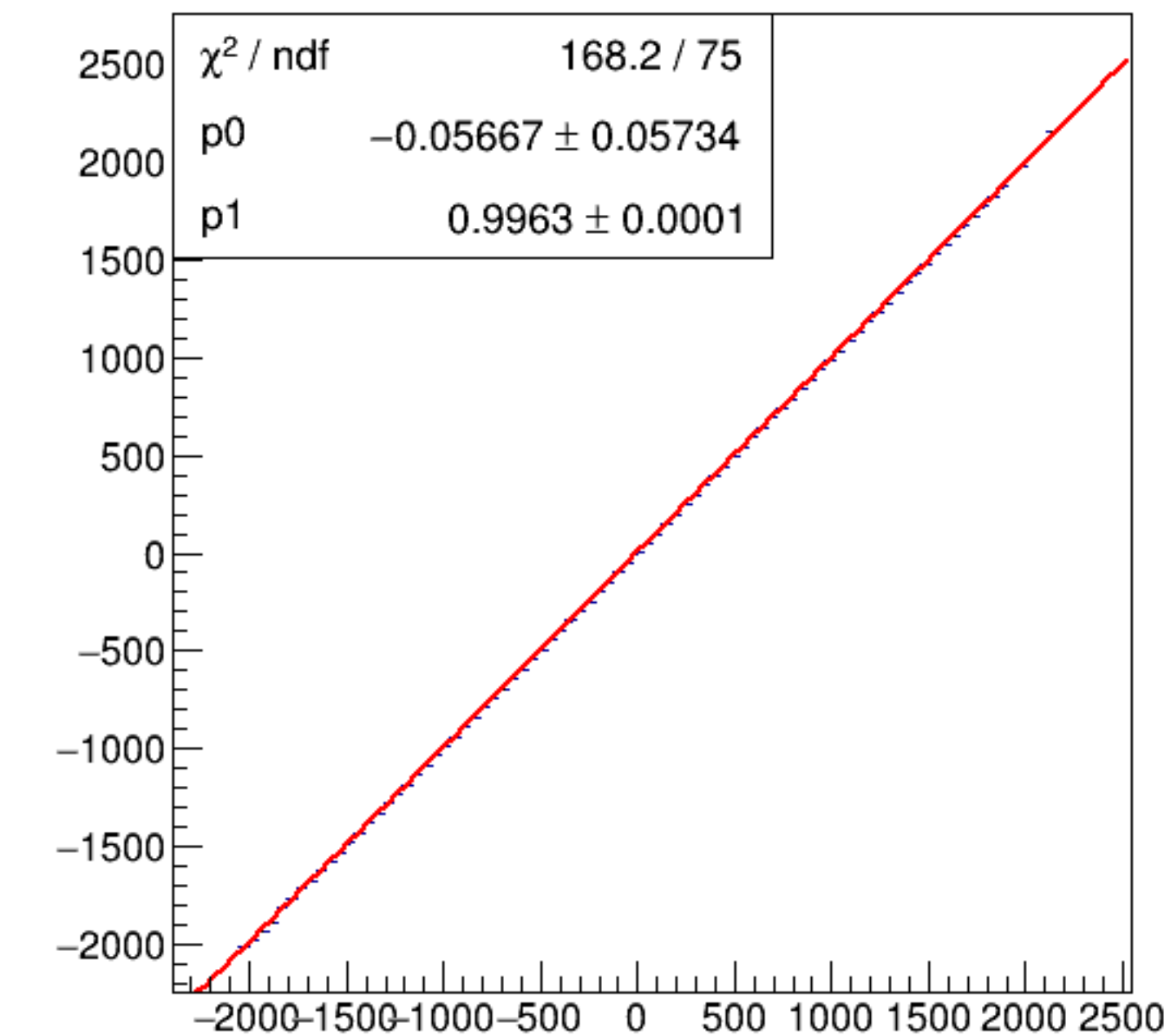
run6346_000_asym_bcm_an_ds_vs_asym_bcm_an_ds3_pr.png
