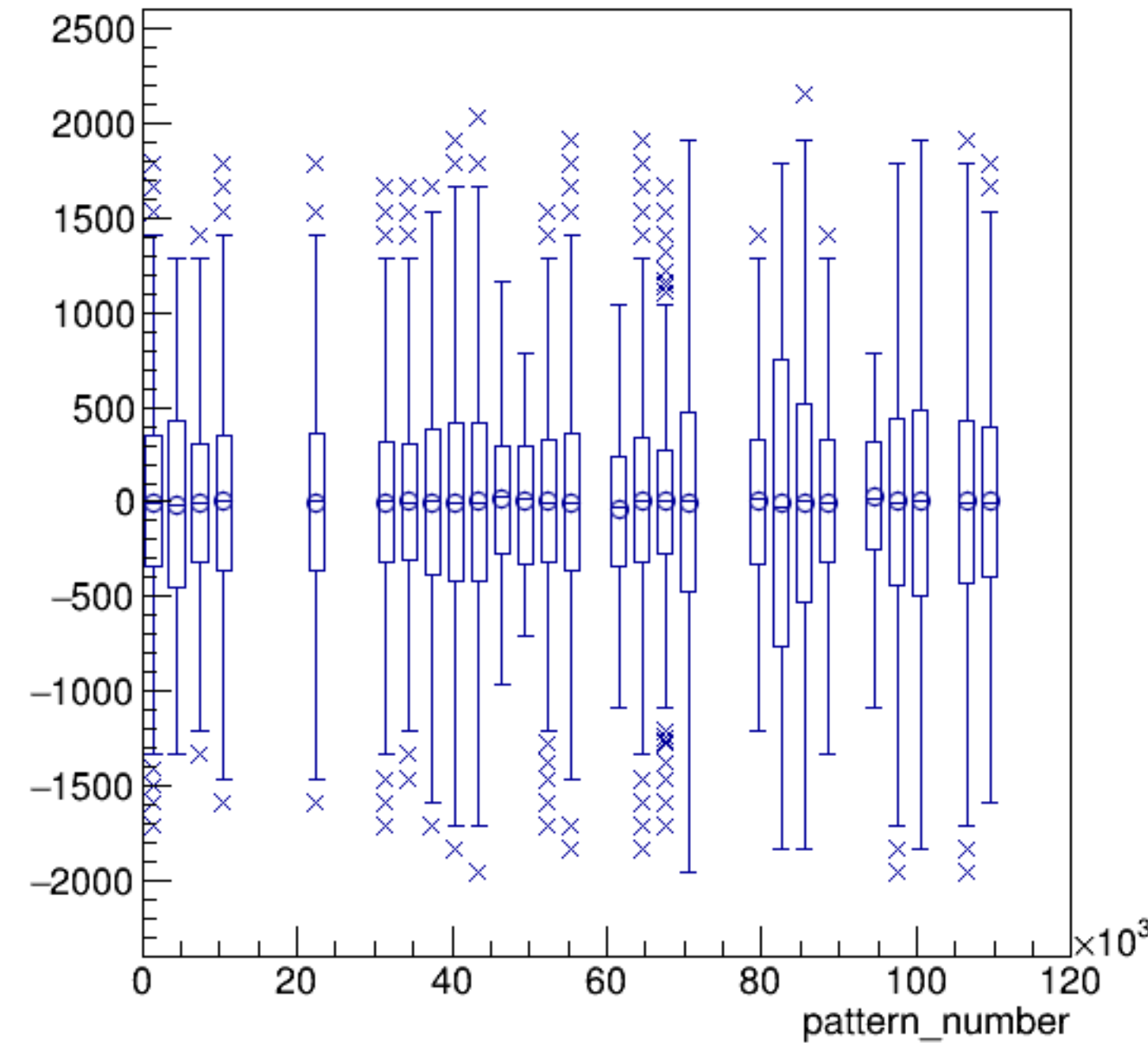
asym_bcm_dg_ds/ppm:pattern_number {ErrorFlag==0}
