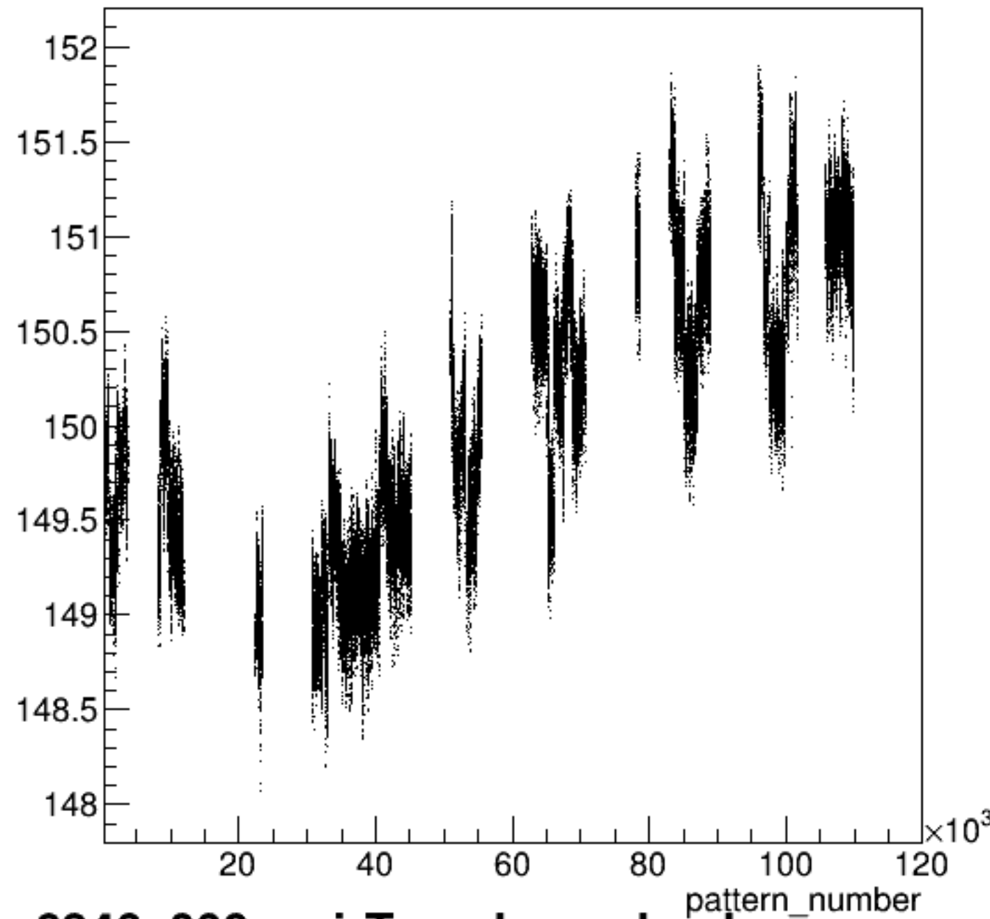
yield_bcm_dg_ds:pattern_number {ErrorFlag==0}
