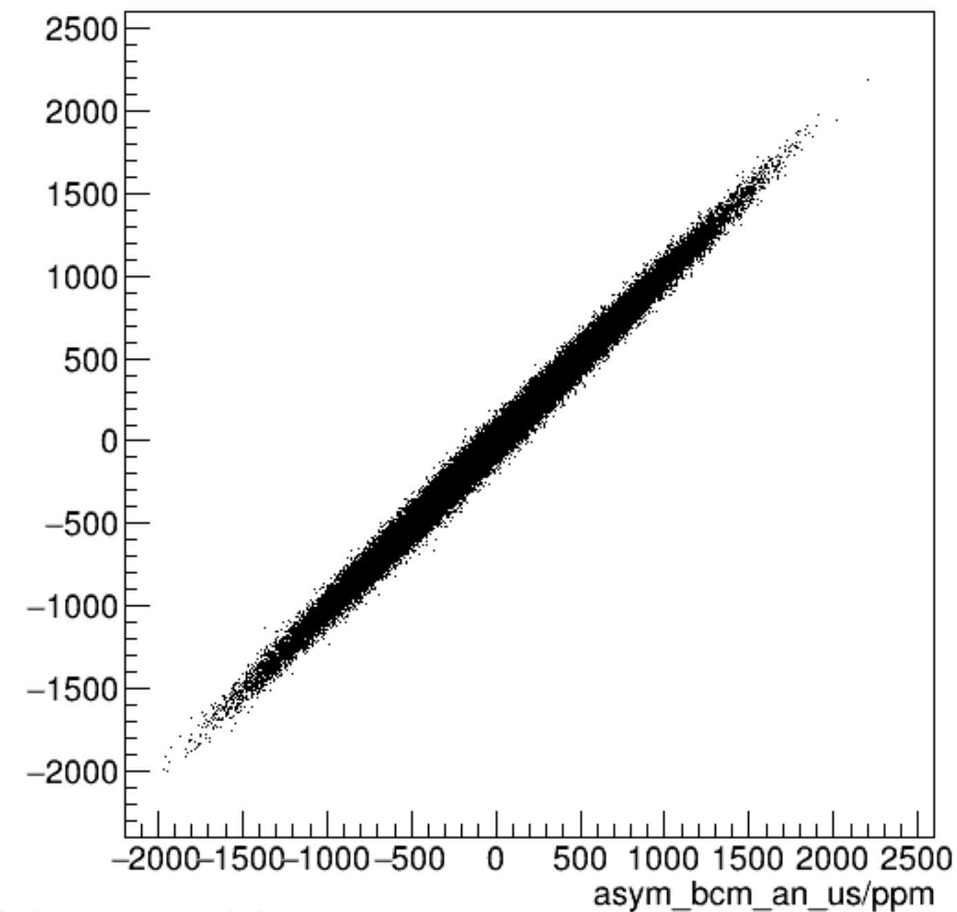
run6346_000_asym_bcm_dg_ds_vs_asym_bcm_an_us_pr.png
