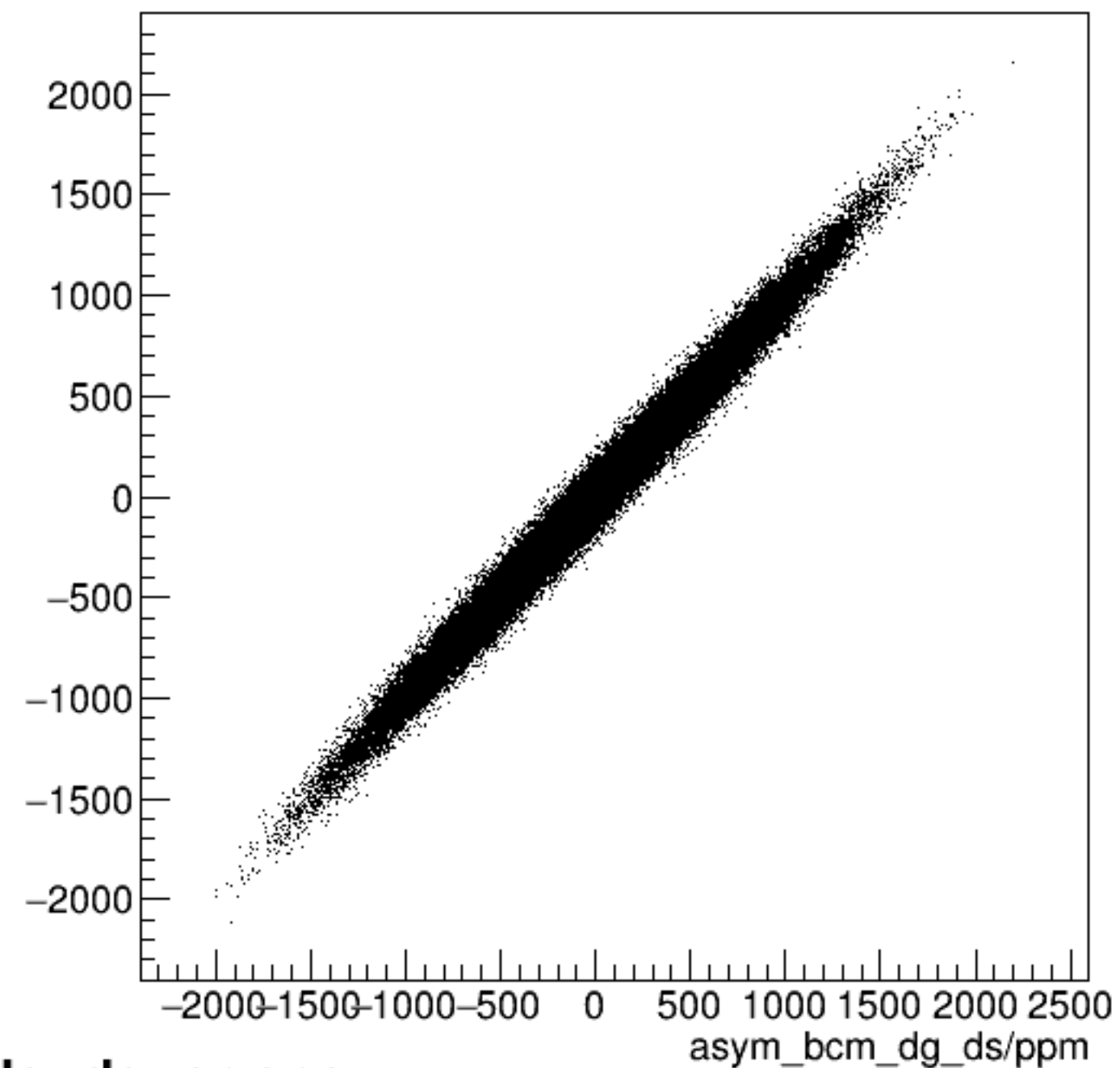
run6346_000_asym_bcm_dg_us_vs_asym_bcm_dg_ds_pr.png
