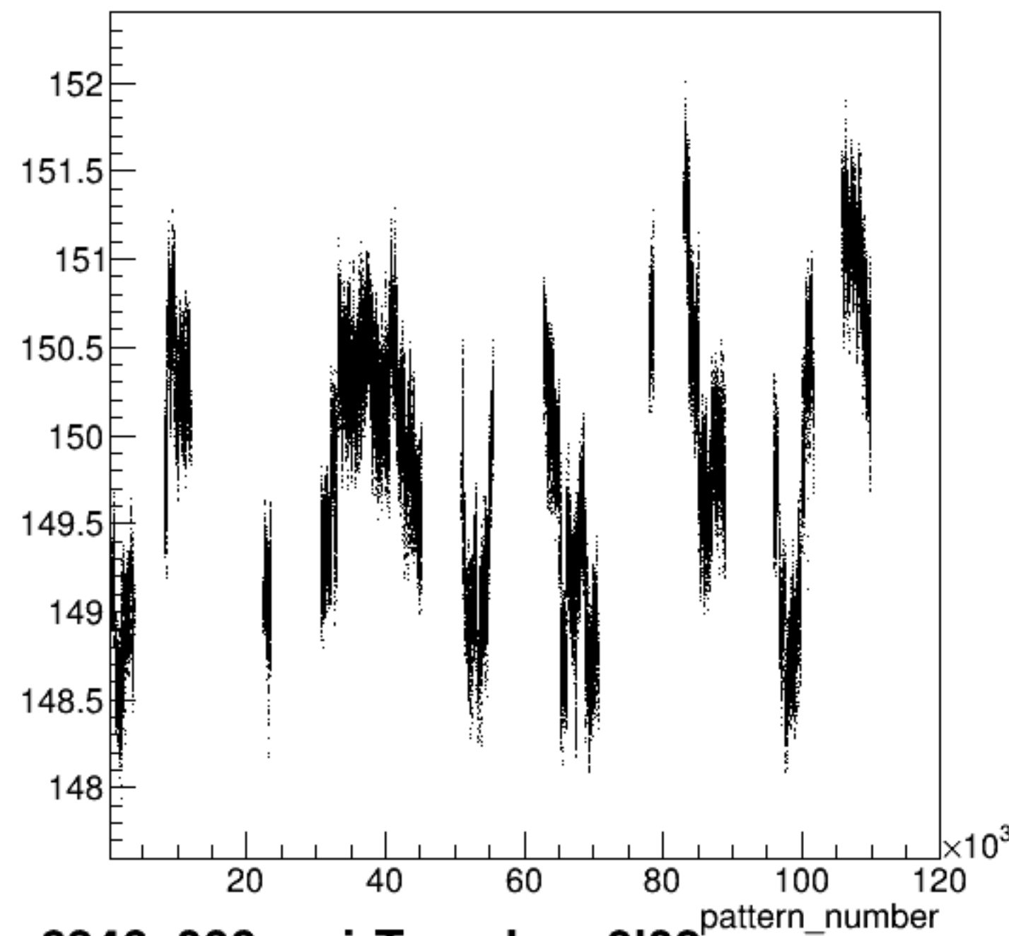
yield_bcm0l02:pattern_number {ErrorFlag==0}
