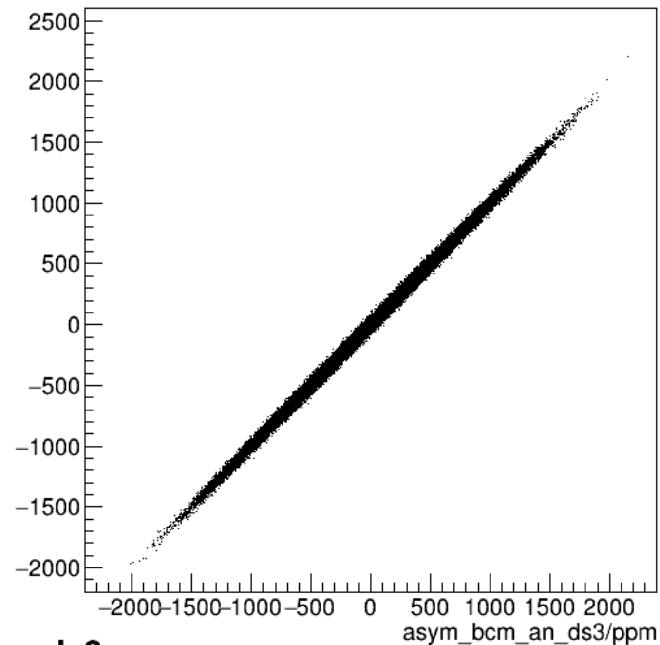
run6346_000_asym_bcm_an_us_vs_asym_bcm_an_ds3_pr.png
