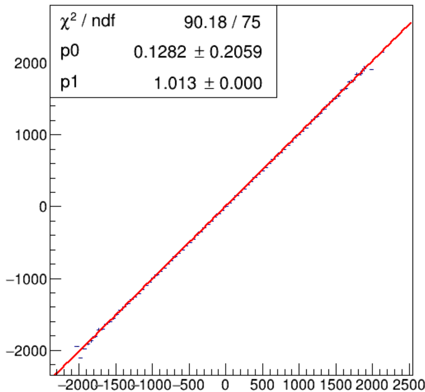
run6346_000_asym_bcm_dg_us_vs_asym_bcm_an_ds3_pr.png
