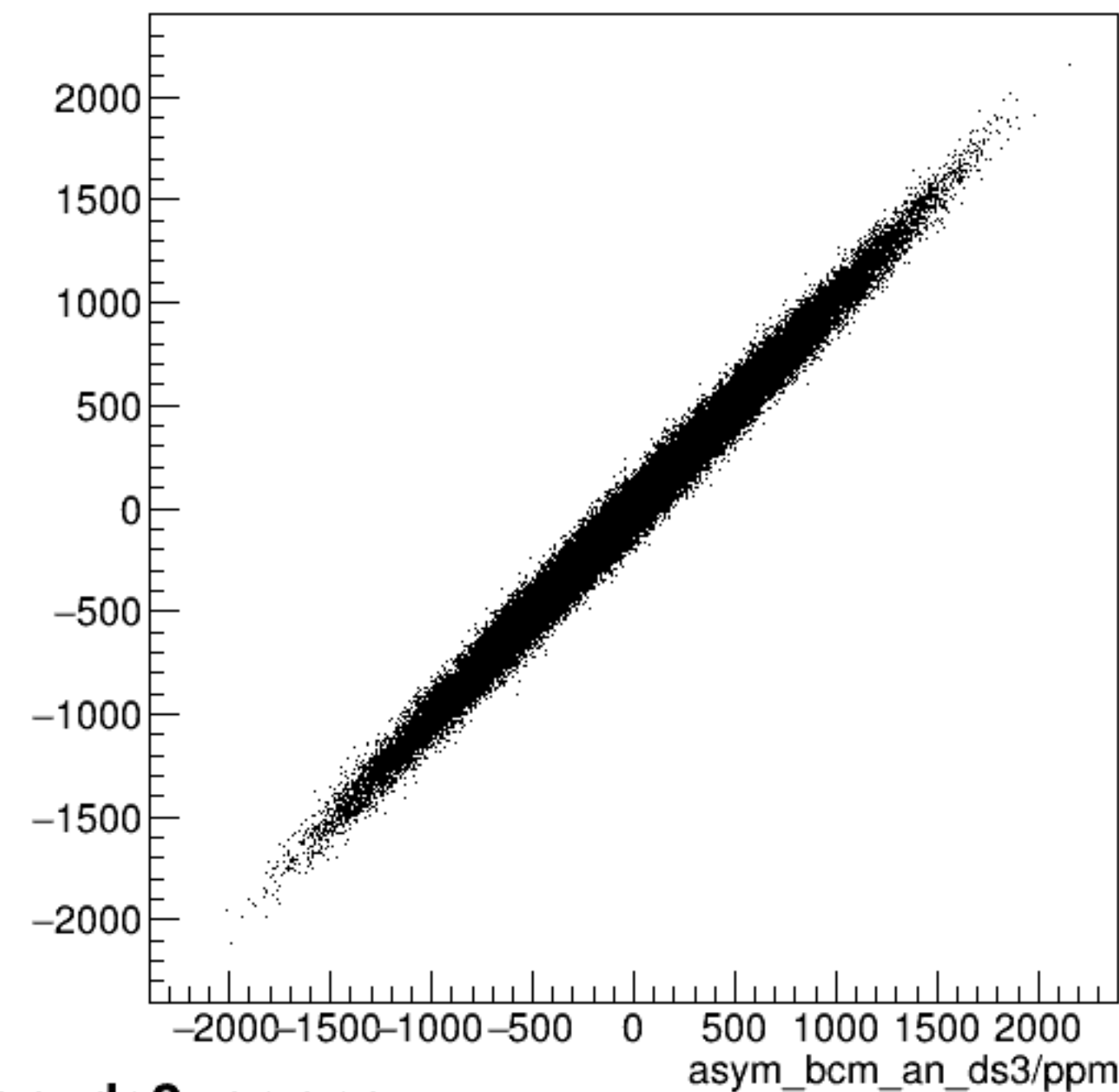
run6346_000_asym_bcm_dg_us_vs_asym_bcm_an_ds3_pr.png
