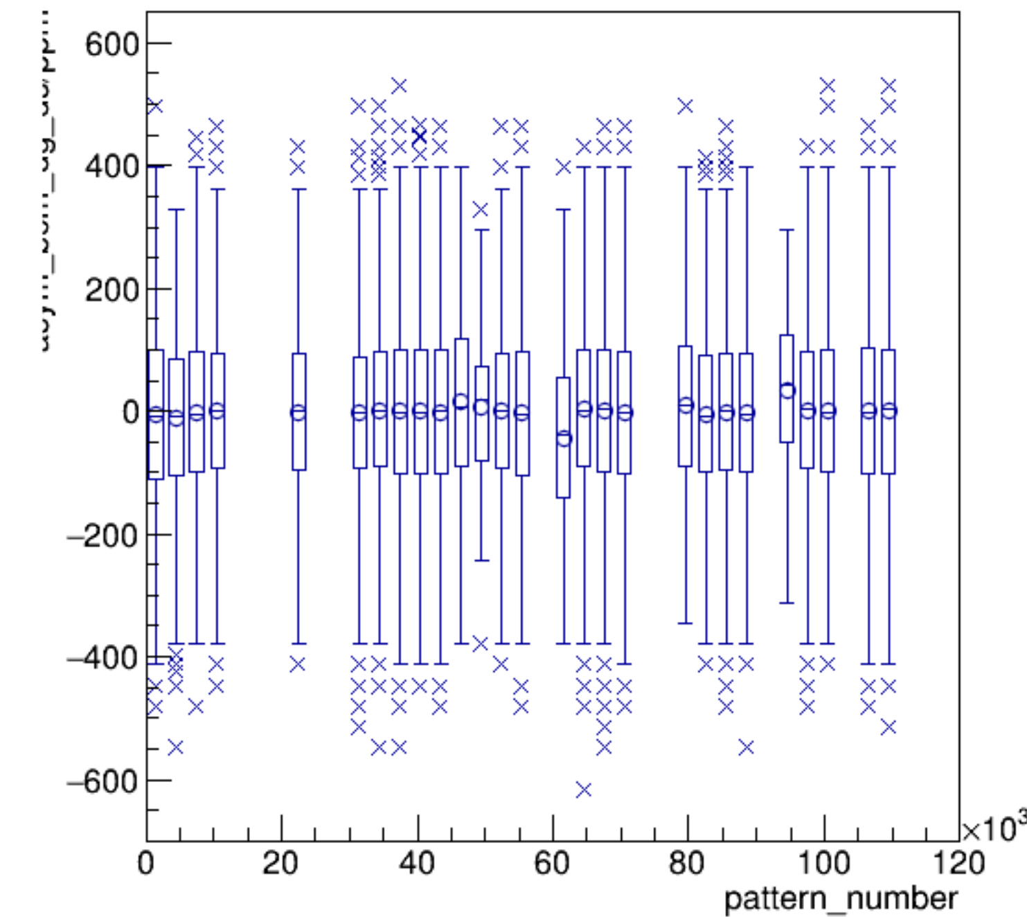
asym_bcm_dg_ds/ppm:pattern_number {ErrorFlag==0}
