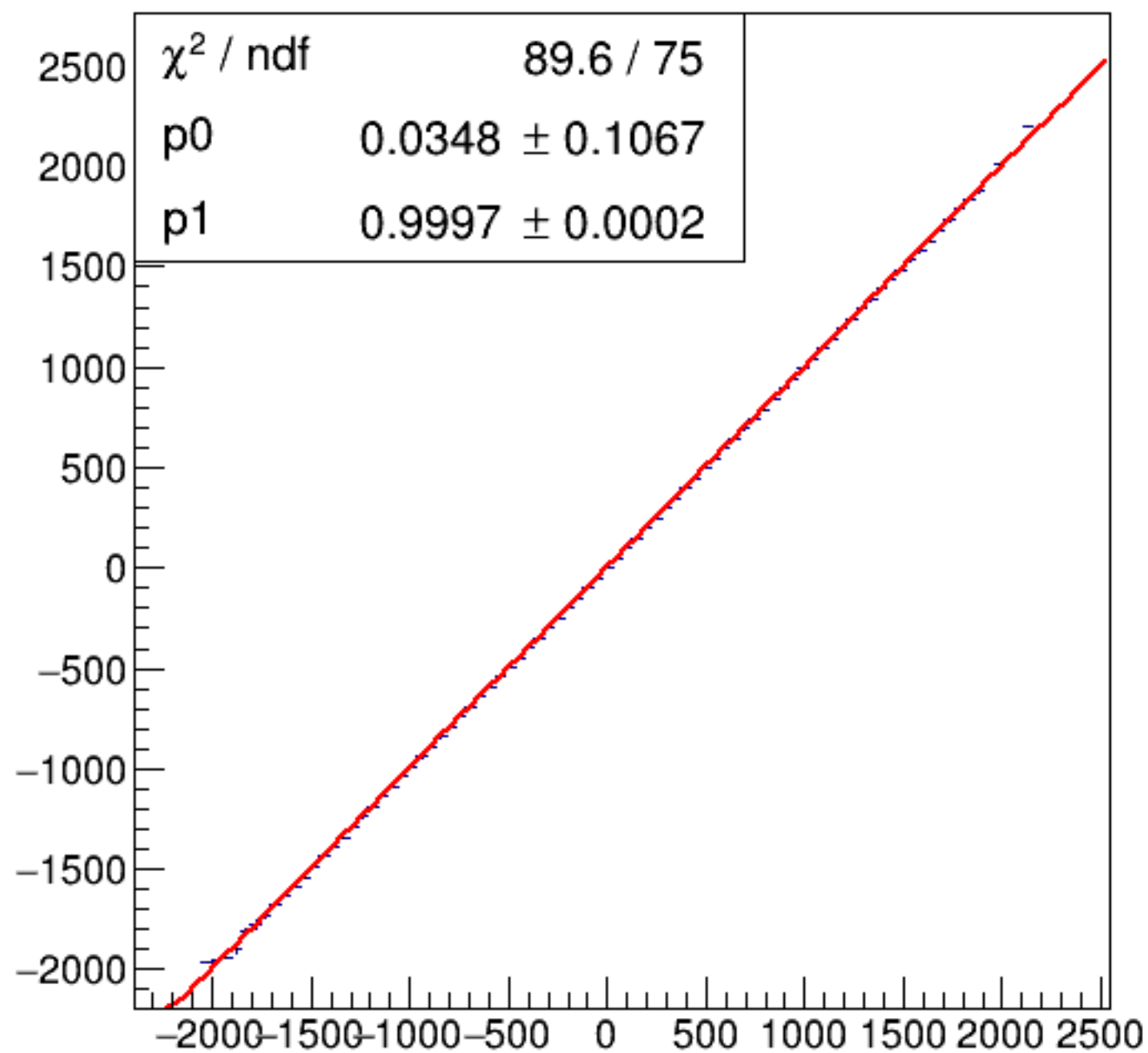
run6346_000_asym_bcm_an_us_vs_asym_bcm_an_ds_pr.png
