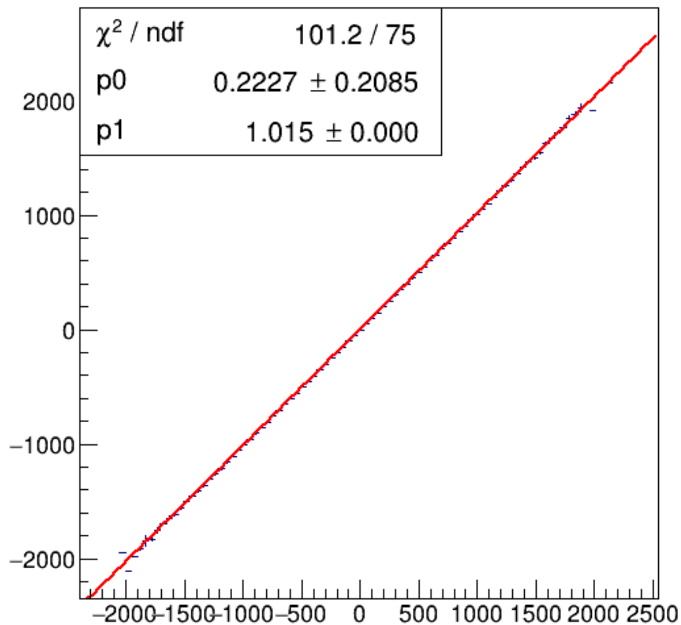
run6346_000_asym_bcm_dg_us_vs_asym_bcm_an_ds_pr.png
