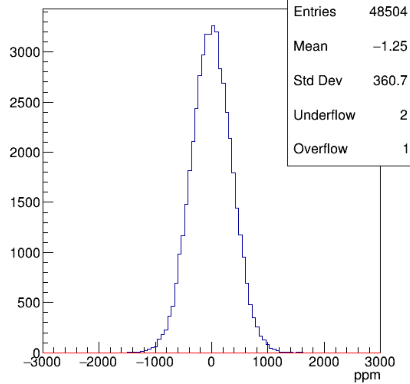
asym_sam7
