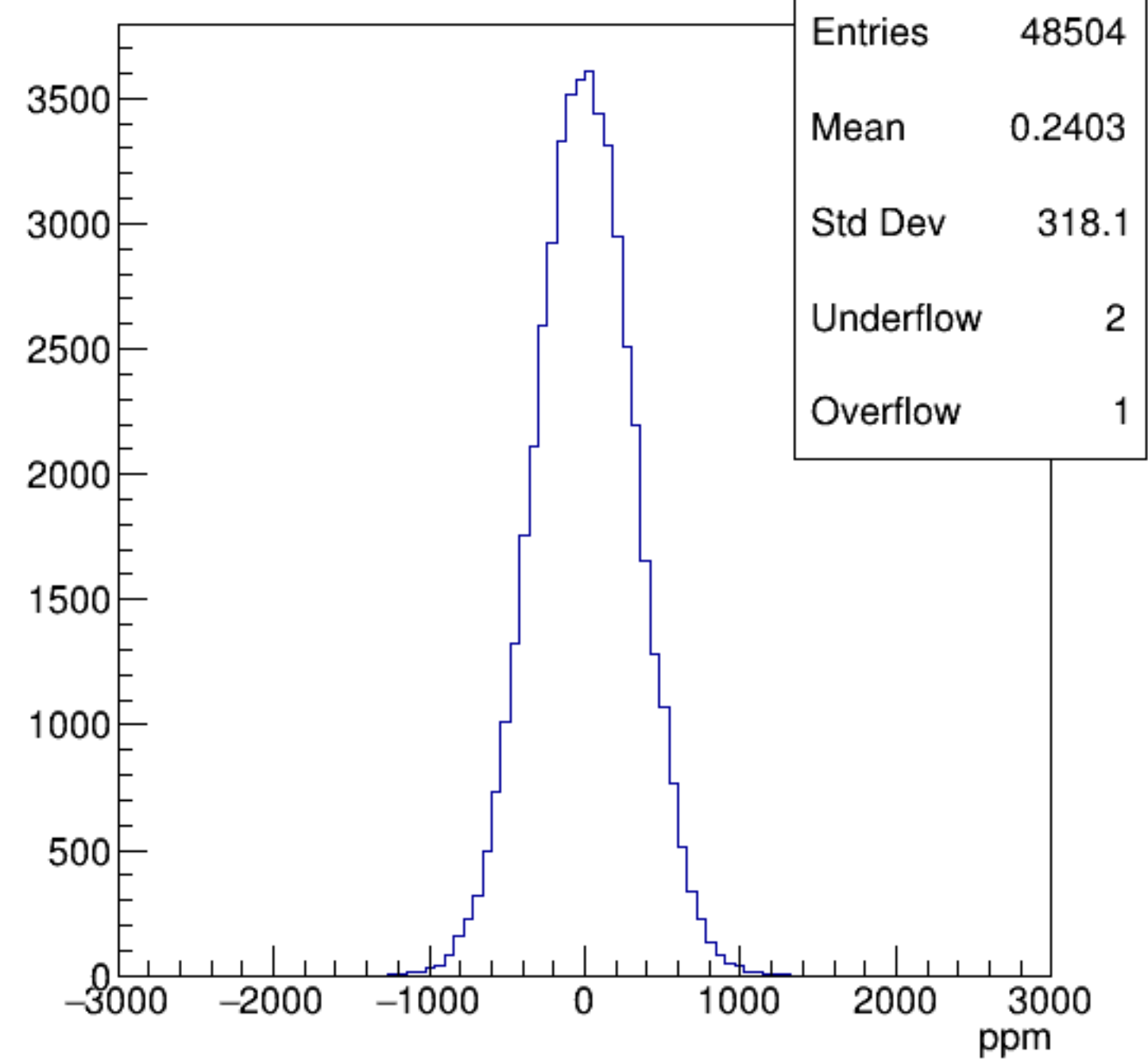
asym_sam8
