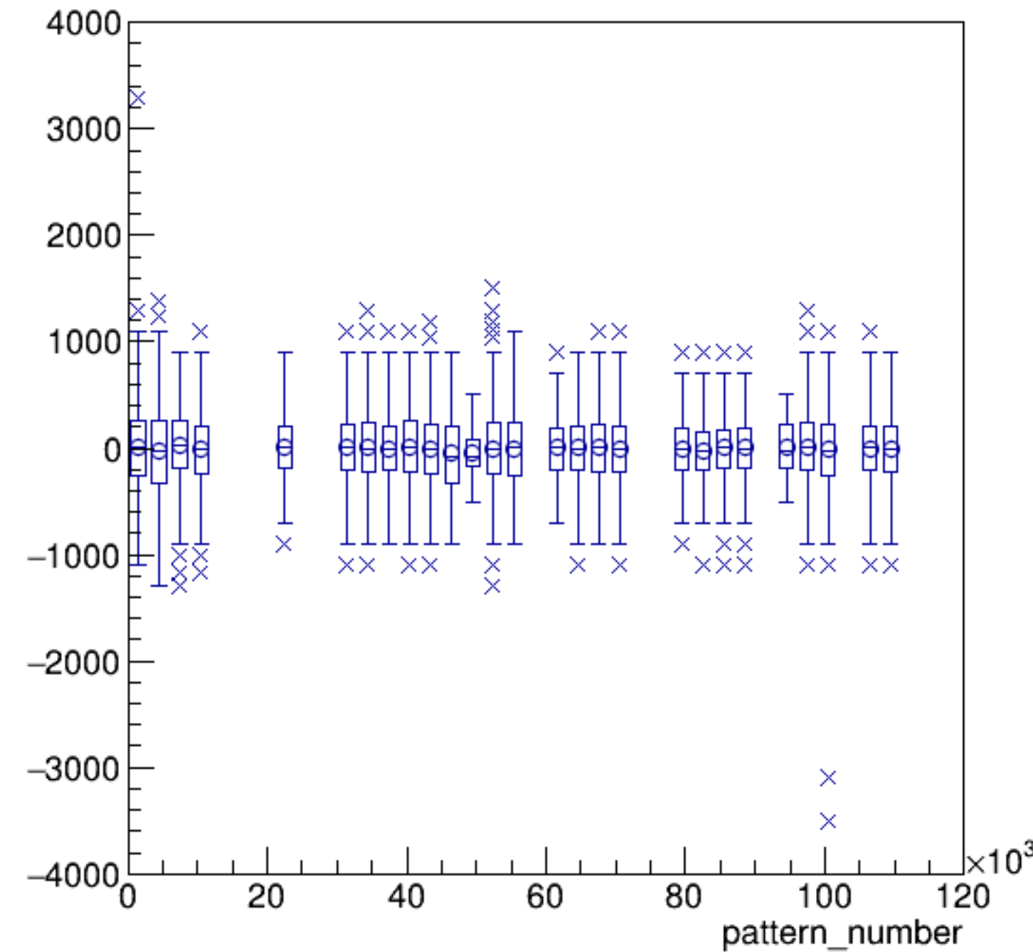
asym_sam8/ppm:pattern_number {ErrorFlag==0}
