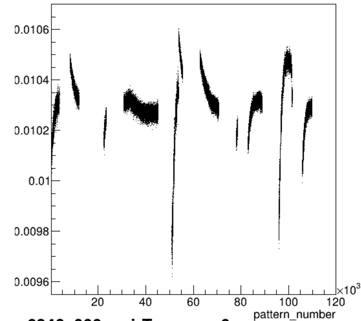
yield_sam6:pattern_number {ErrorFlag==0}
