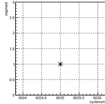
segment:cyclenum {run == 6348}
