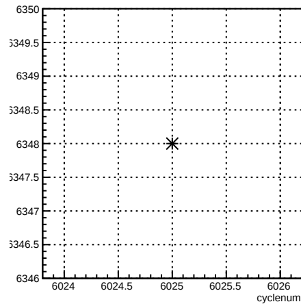
run:cyclenum {run == 6348}
