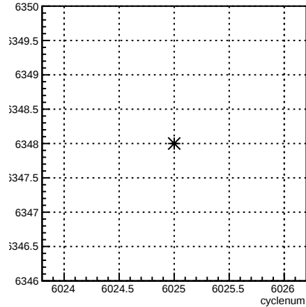
run:cyclenum {run == 6348}
