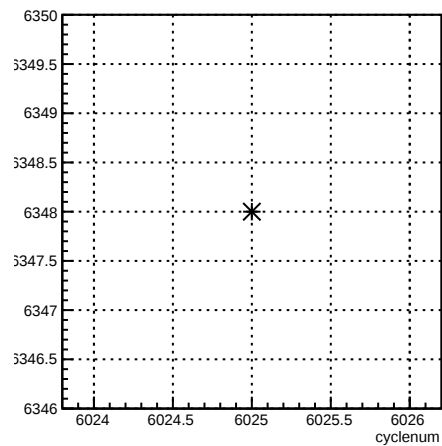
run:cyclenum {run == 6348}
