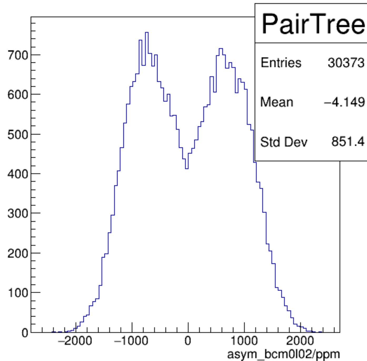
asym_bcm0l02/ppm {ErrorFlag==0}
