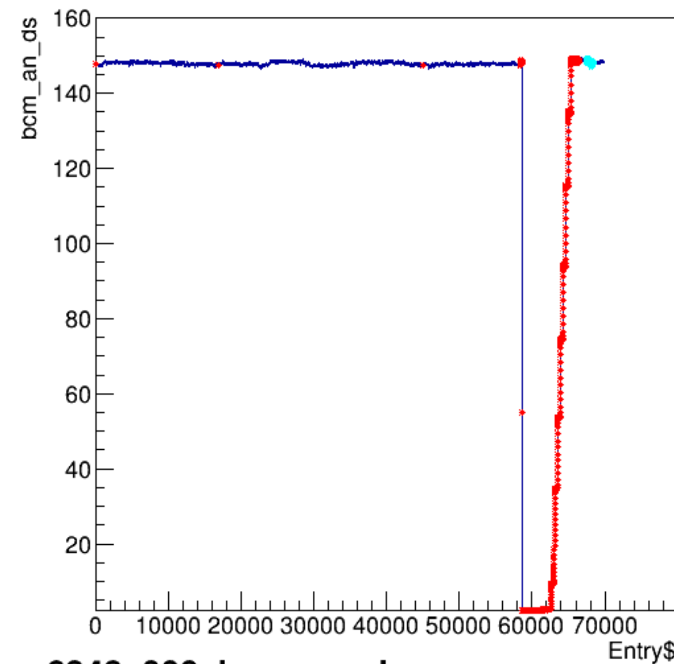
bcm_an_ds:Entry$
