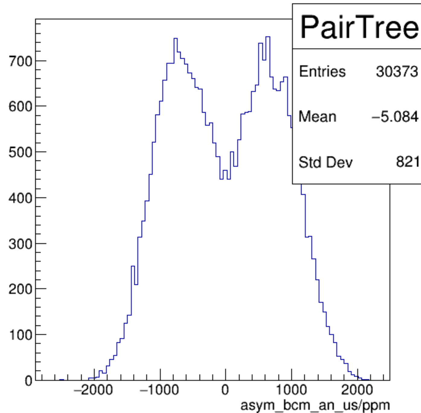
asym_bcm_an_us/ppm {ErrorFlag==0}
