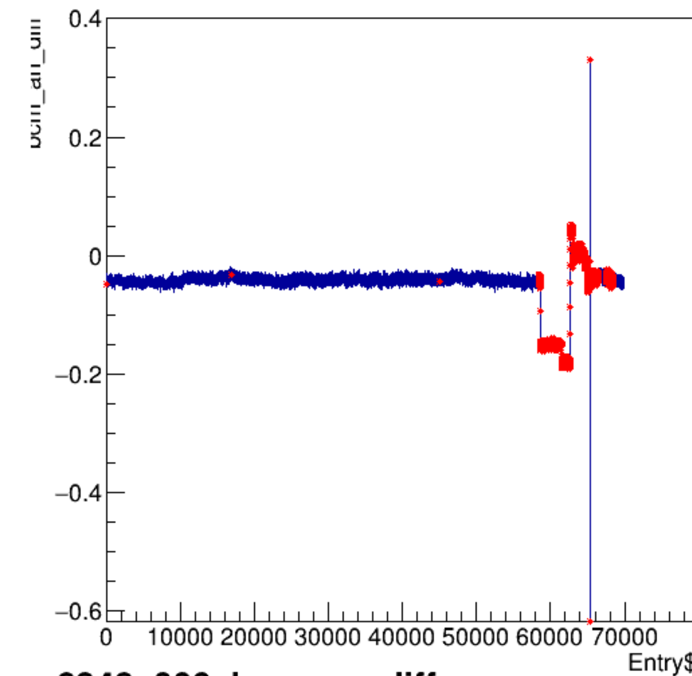
bcm_an_diff:Entry$
