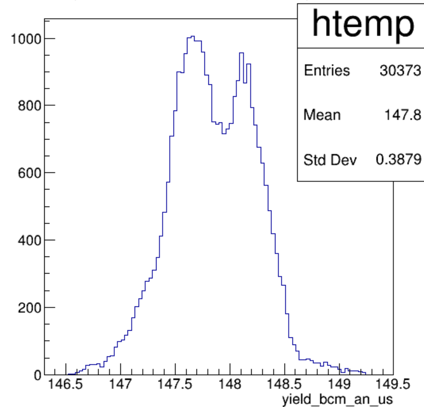
yield_bcm_an_us {ErrorFlag==0}
