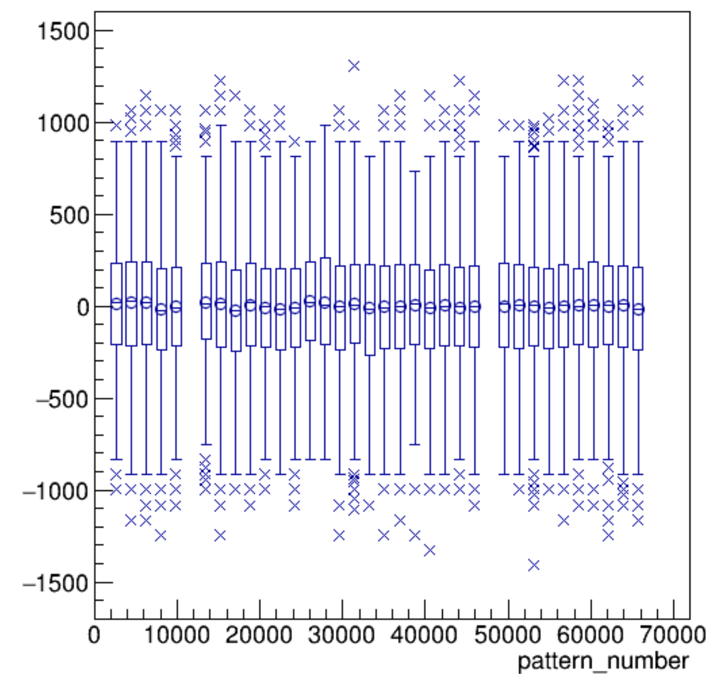
asym_dsl/ppm:pattern_number {ErrorFlag==0}
