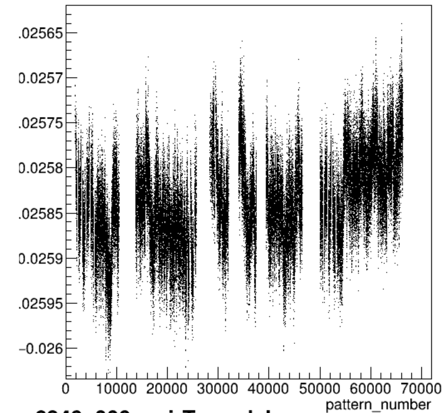
yield_dsl:pattern_number {ErrorFlag==0}
