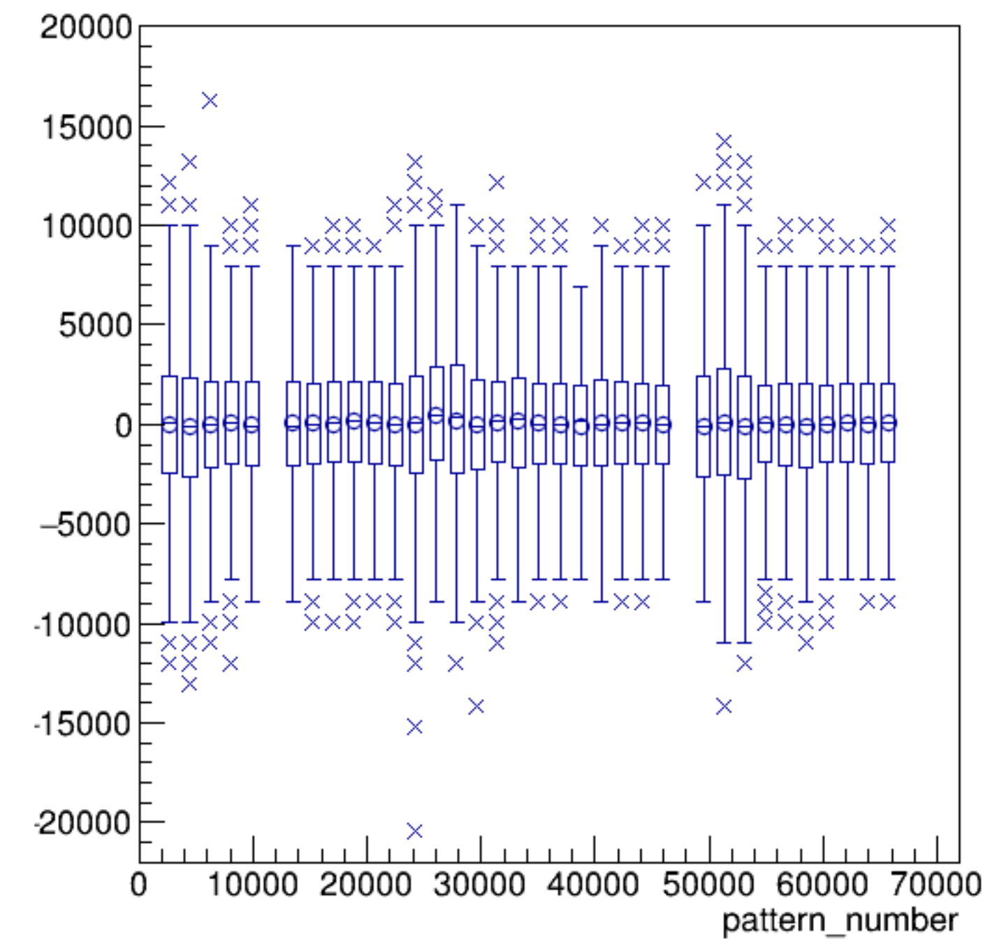
asym_usl/ppm:pattern_number {ErrorFlag==0}
