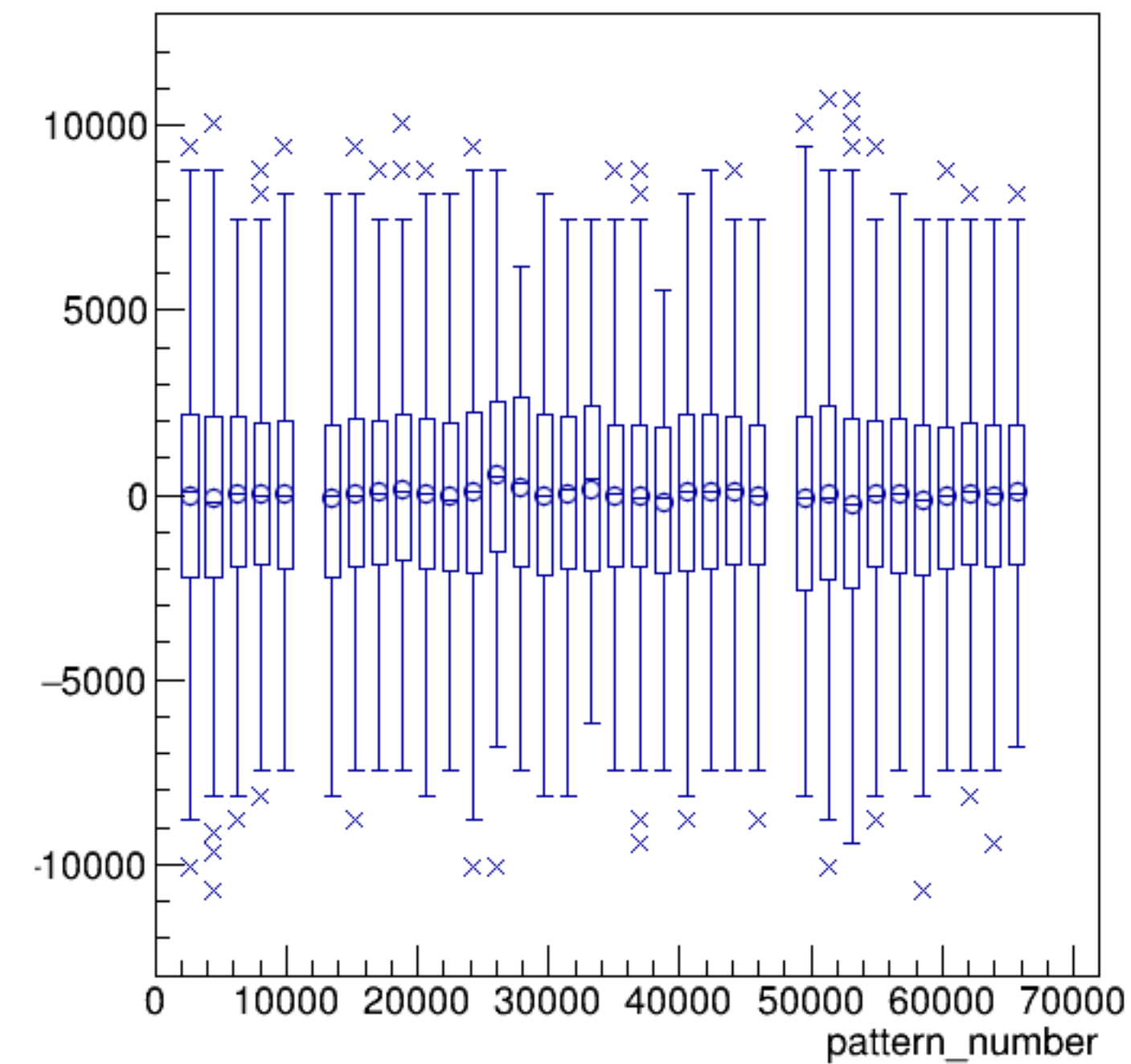
asym_usr/ppm:pattern_number {ErrorFlag==0}
