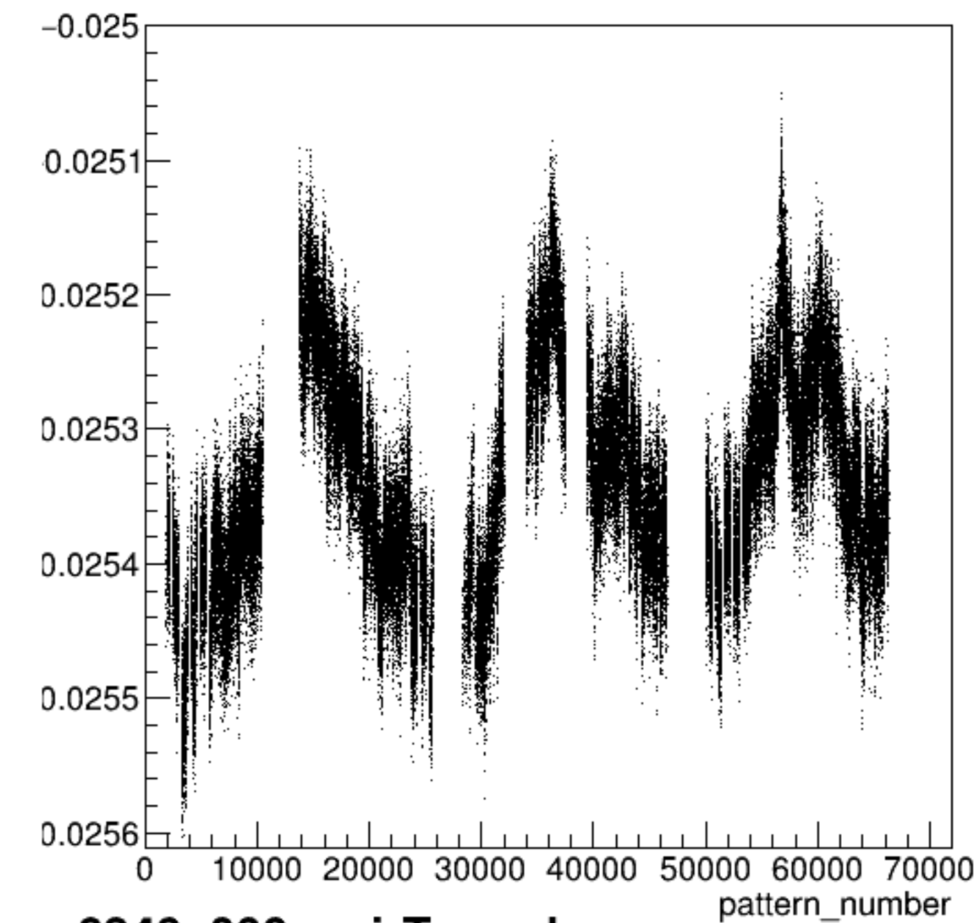
yield_dsr:pattern_number {ErrorFlag==0}
