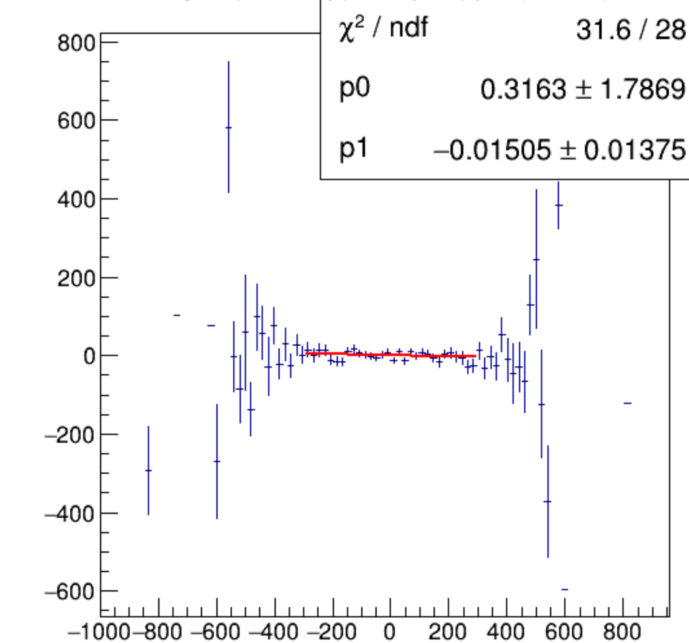
reg_asym_dsr/ppm:AqUS/ppm {ok_cut}
