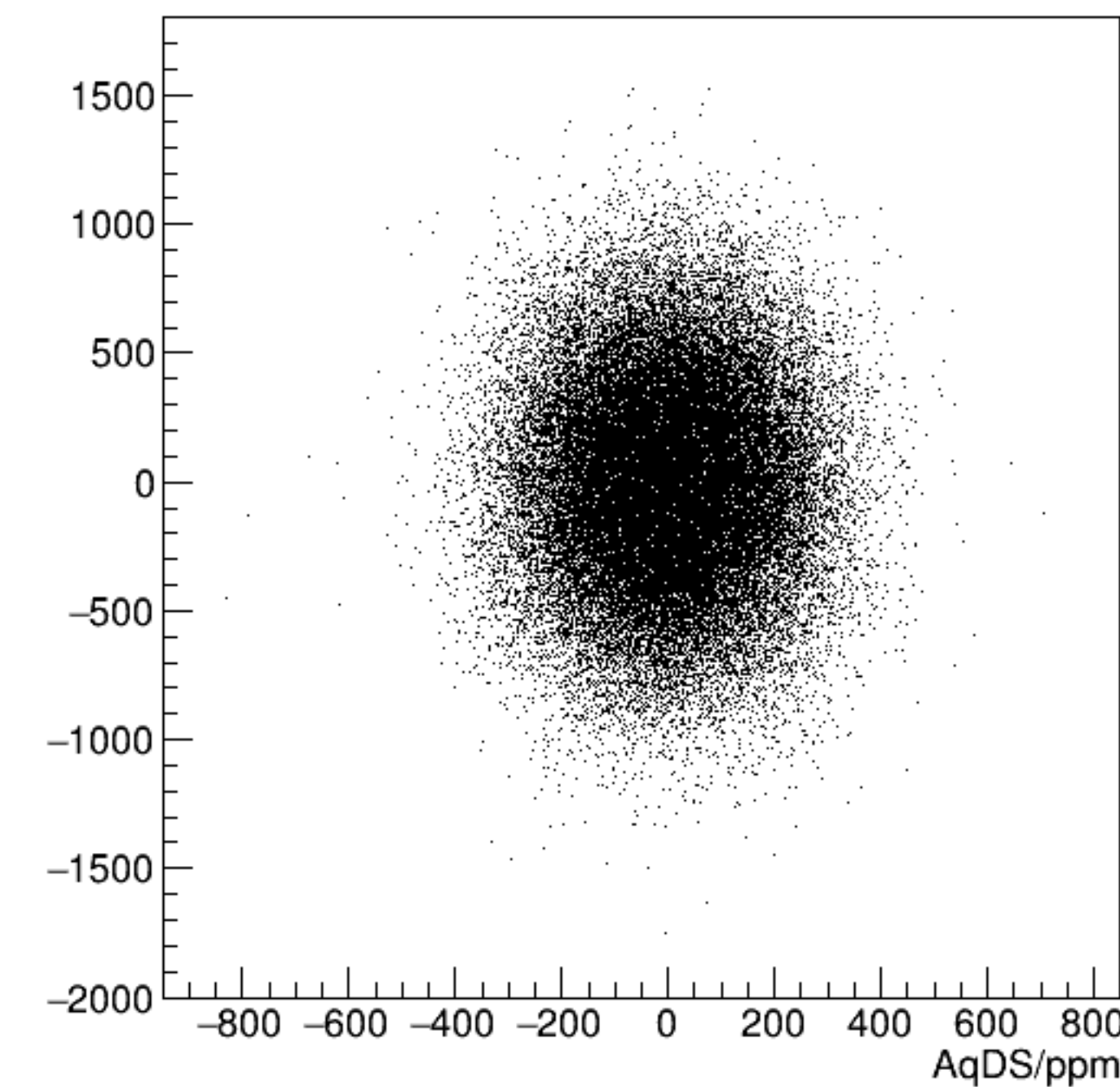
reg_asym_dsr/ppm:AqDS/ppm {ok_cut}
