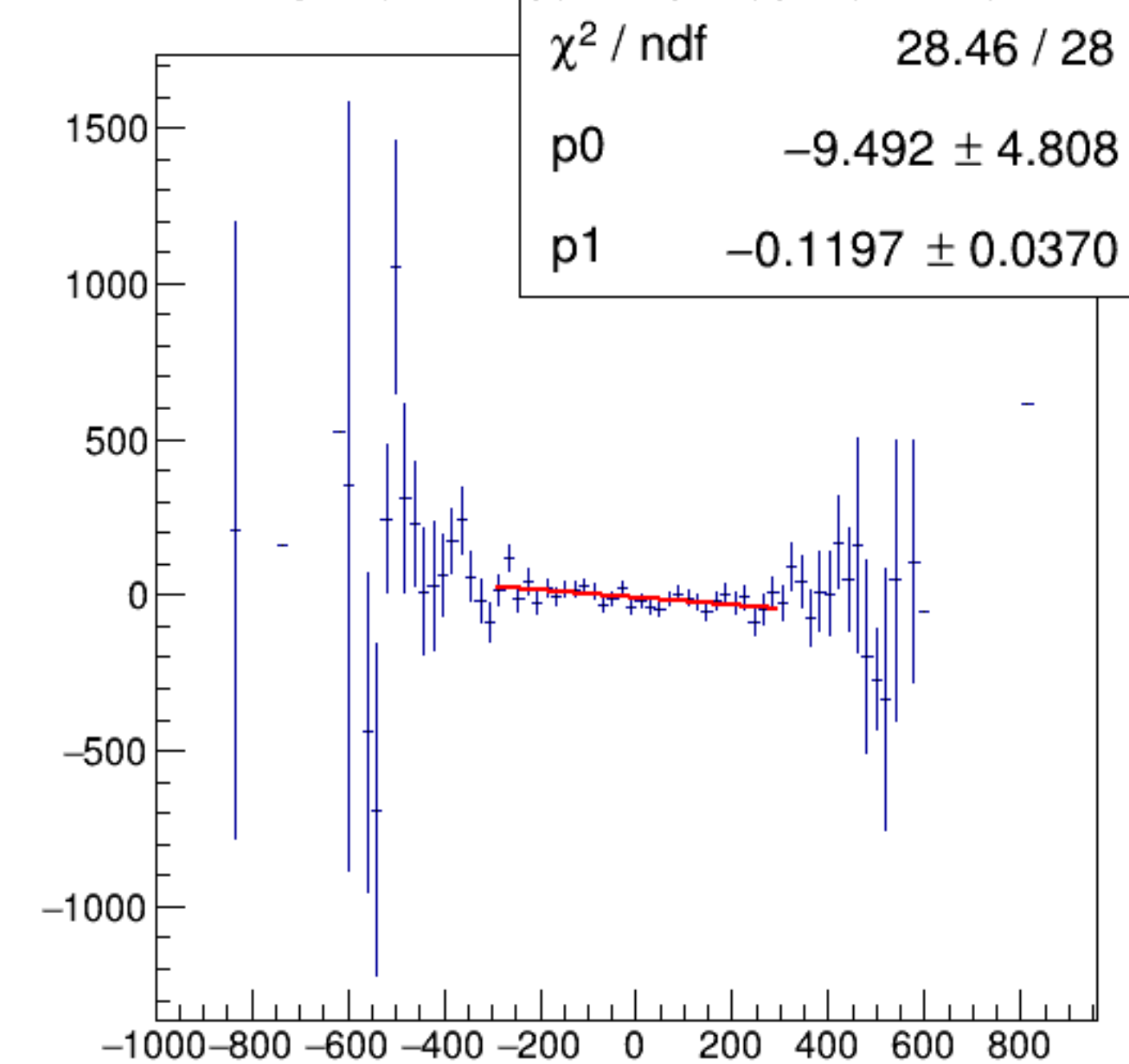
reg_asym_usr/ppm:AqUS/ppm {ok_cut}
