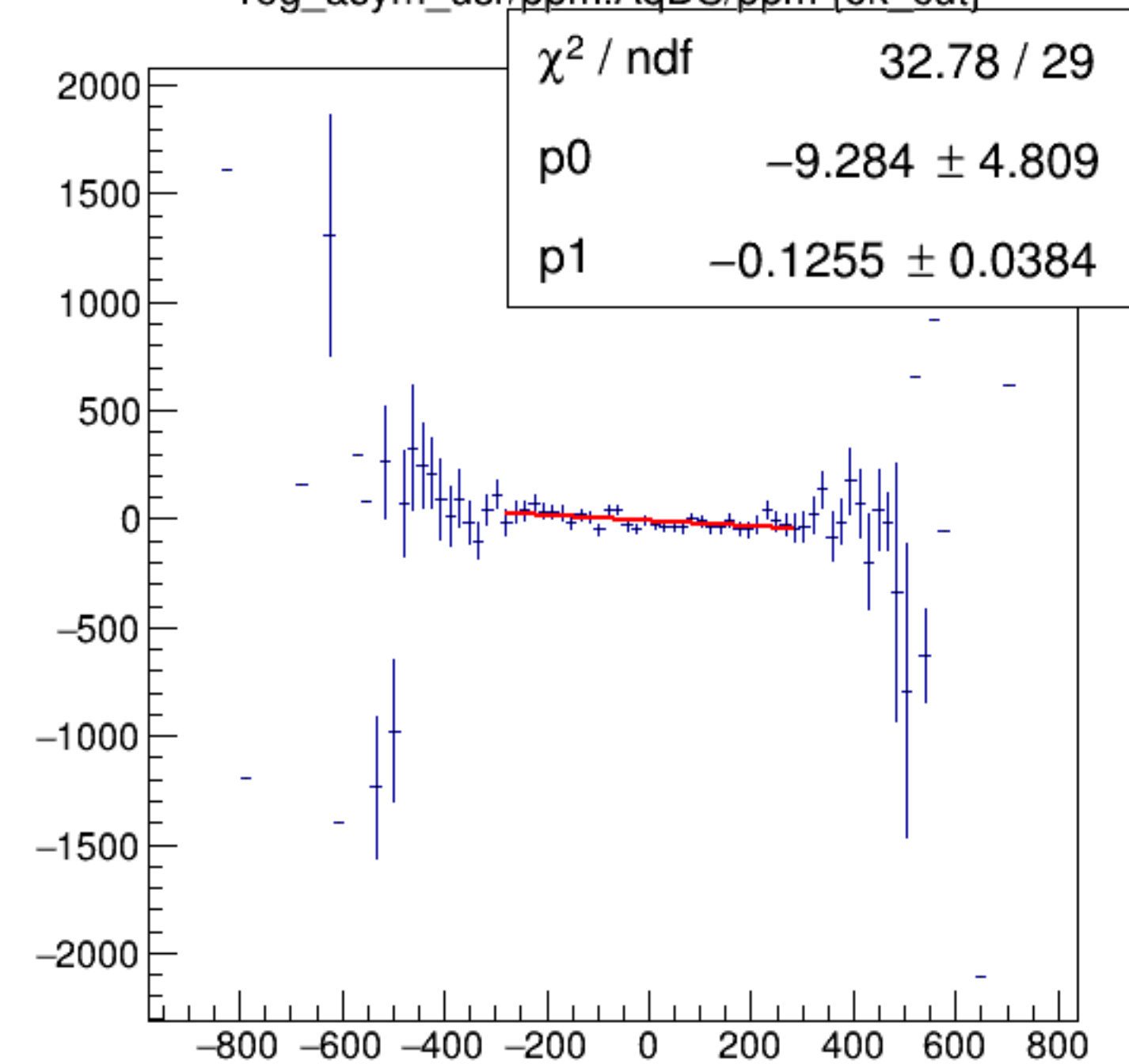
reg_asym_usr/ppm:AqDS/ppm {ok_cut}
