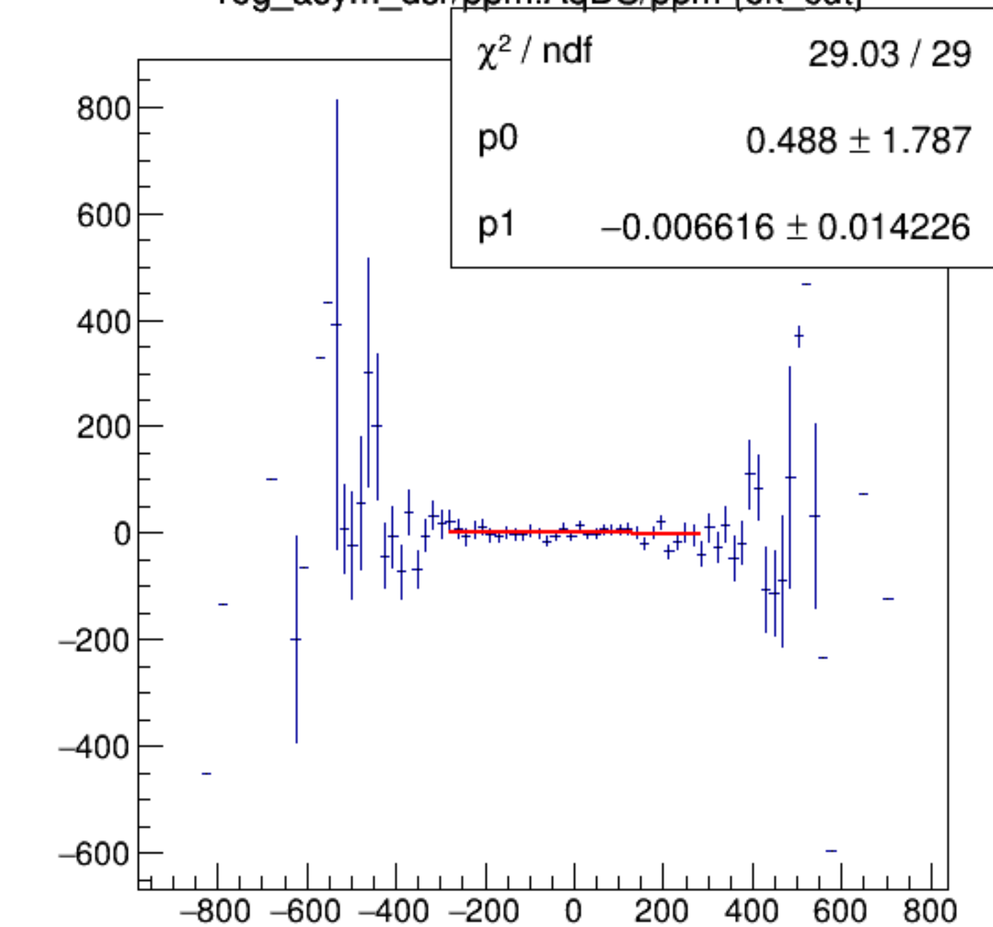
reg_asym_dsr/ppm:AqDS/ppm {ok_cut}
