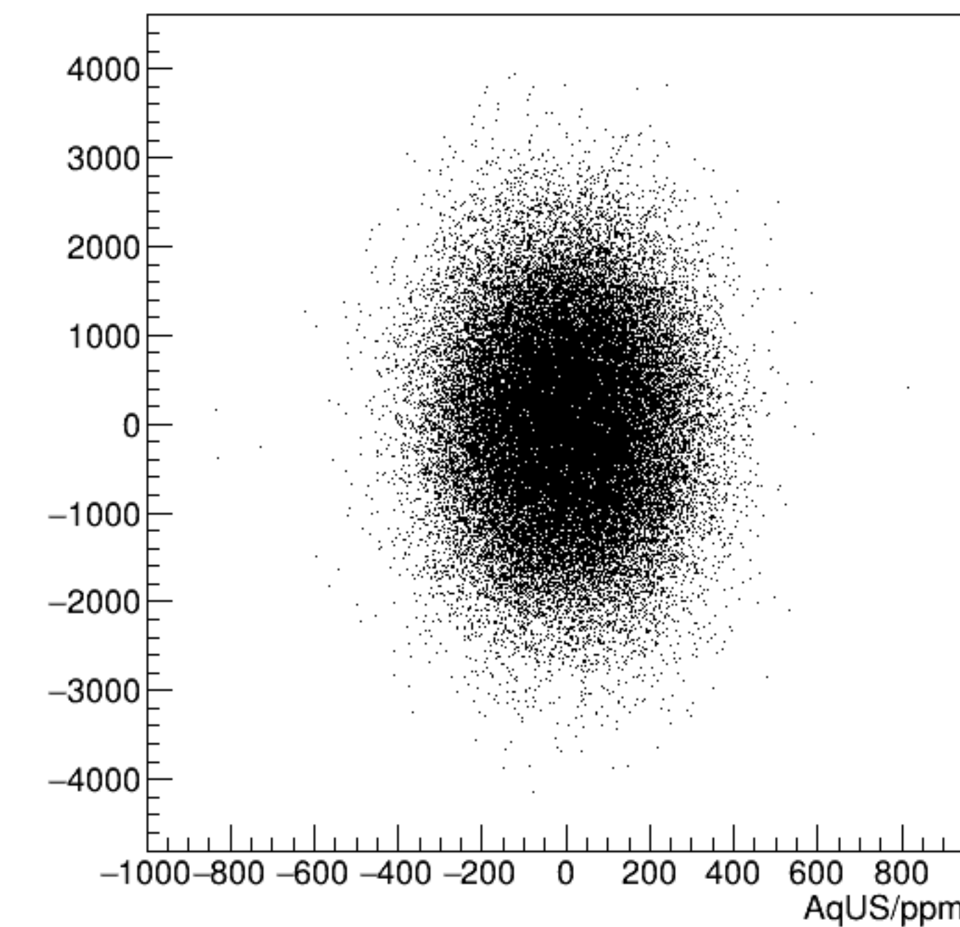
reg_asym_usl/ppm:AqUS/ppm {ok_cut}
