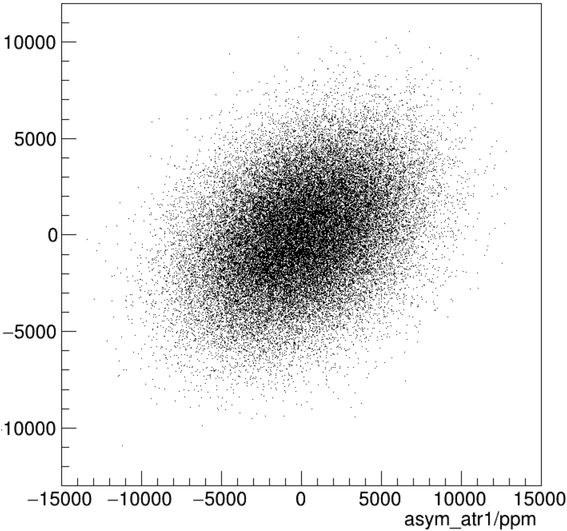
asym_atl1/ppm:asym_atr1/ppm {ok_cut}
