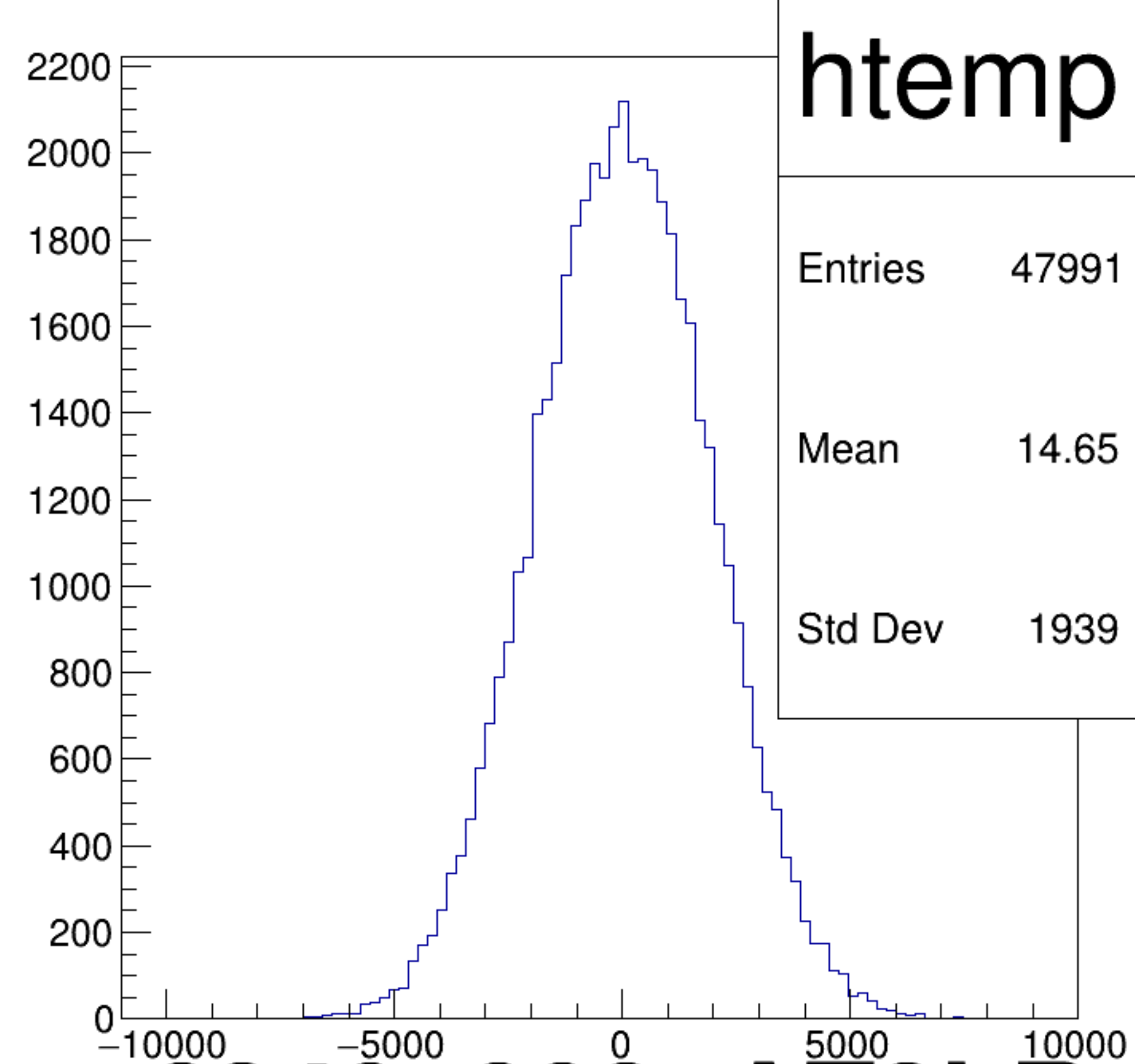
(asym_atl2/ppm-asym_atr2/ppm)/2 {ok_cut}
