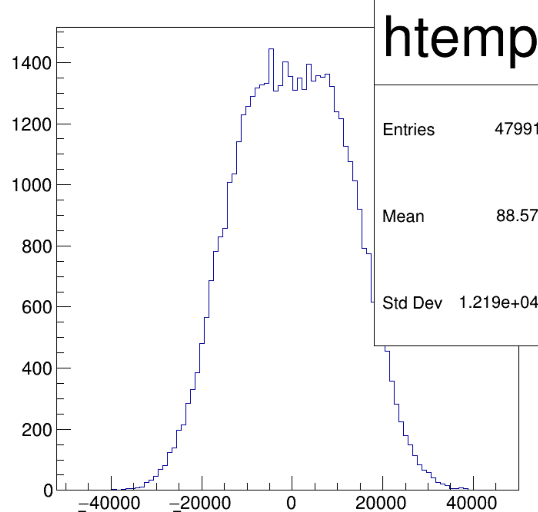
(asym_atl2/ppm+asym_atr2/ppm)/2 {ok_cut}
