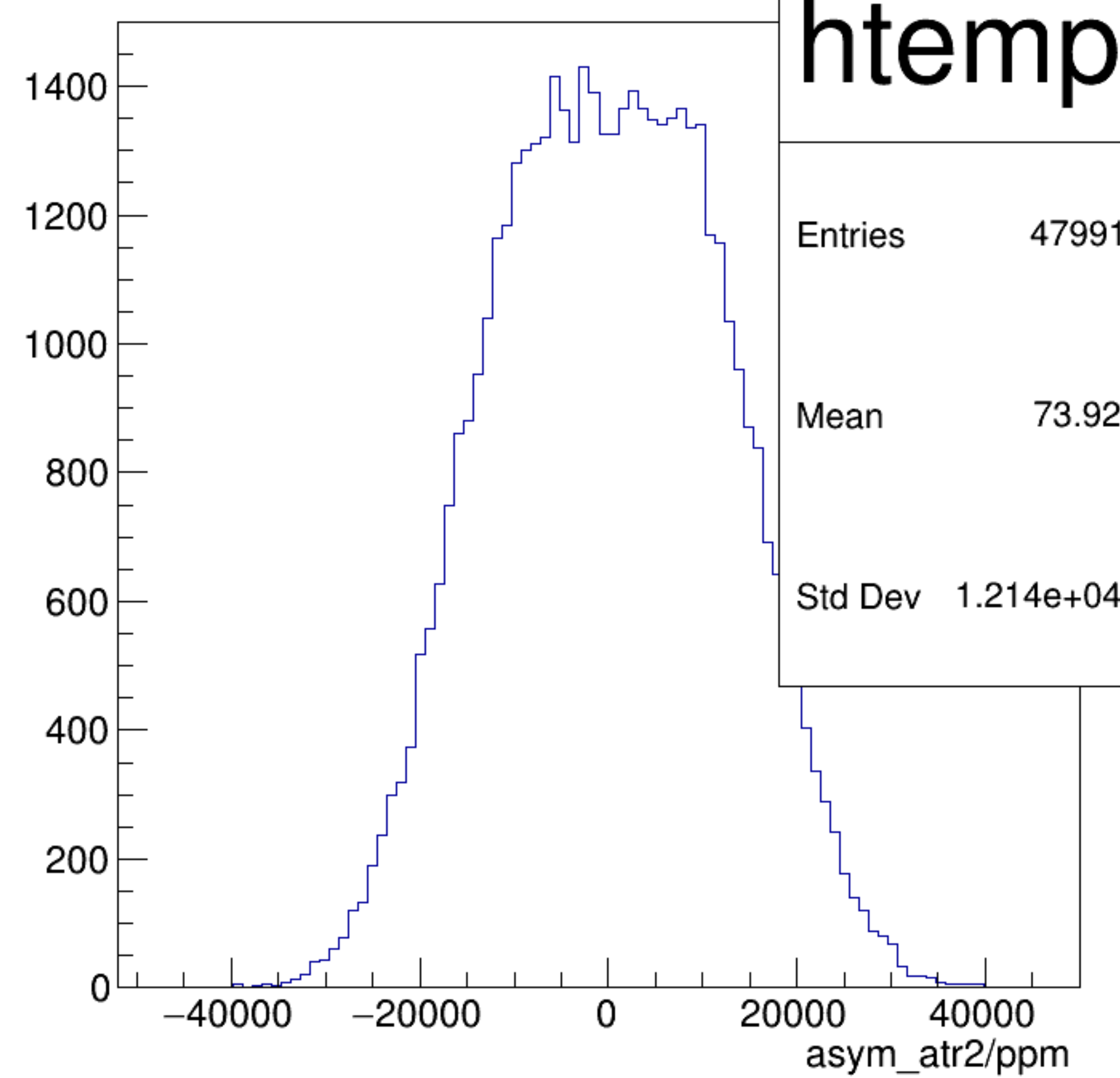
asym_atr2/ppm {ok_cut}
