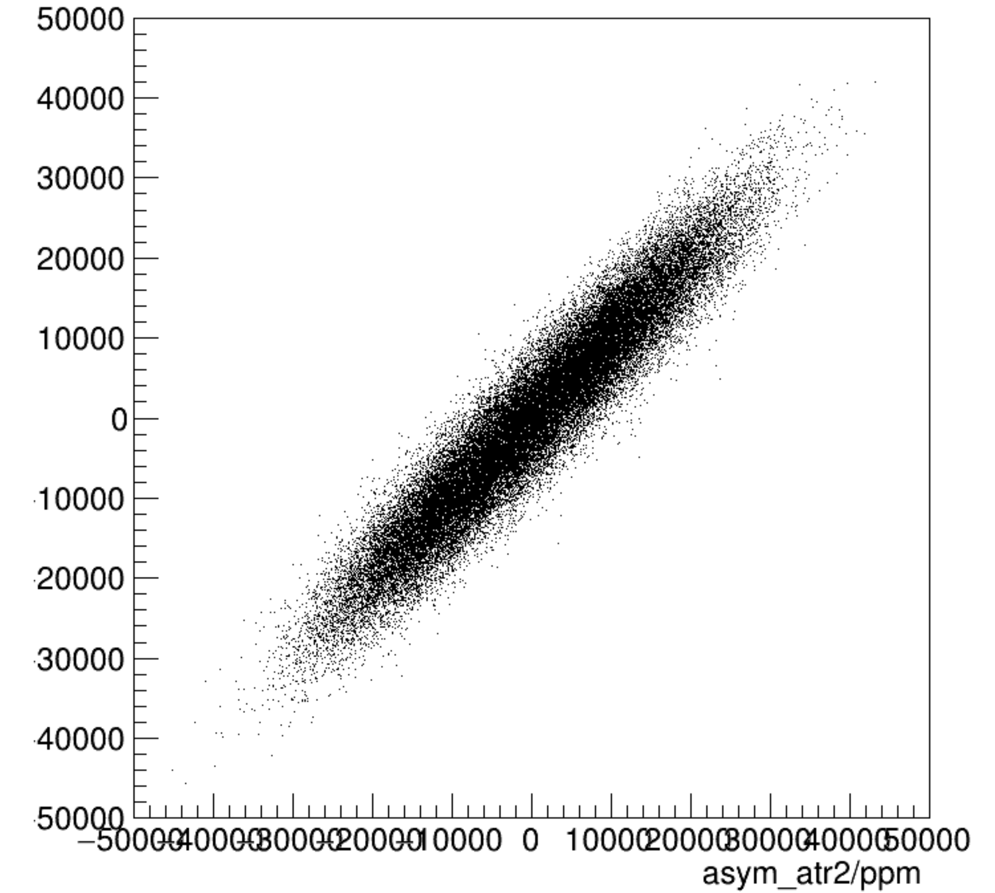
asym_atl2/ppm:asym_atr2/ppm {ok_cut}
