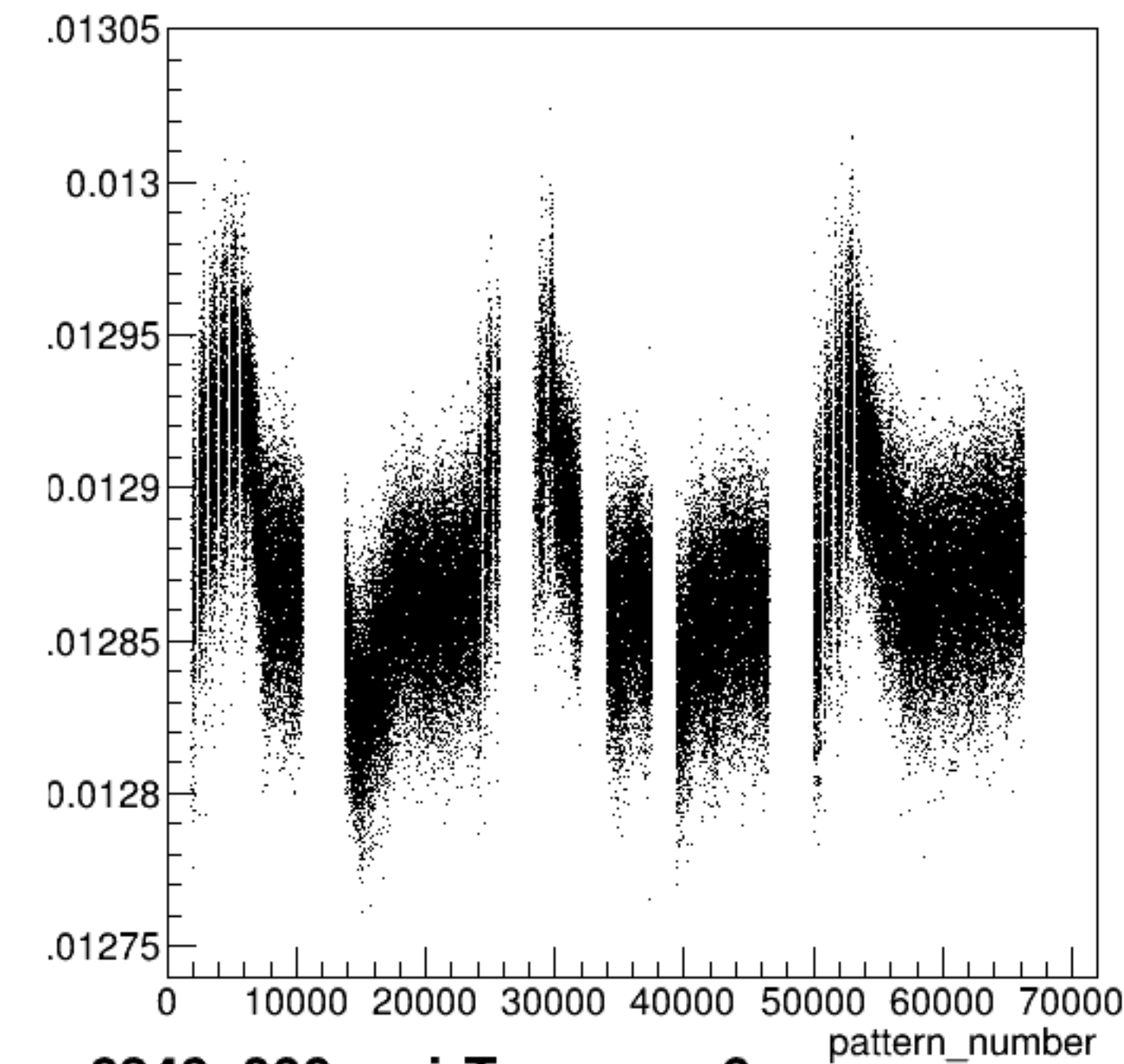
yield_sam6:pattern_number {ErrorFlag==0}
