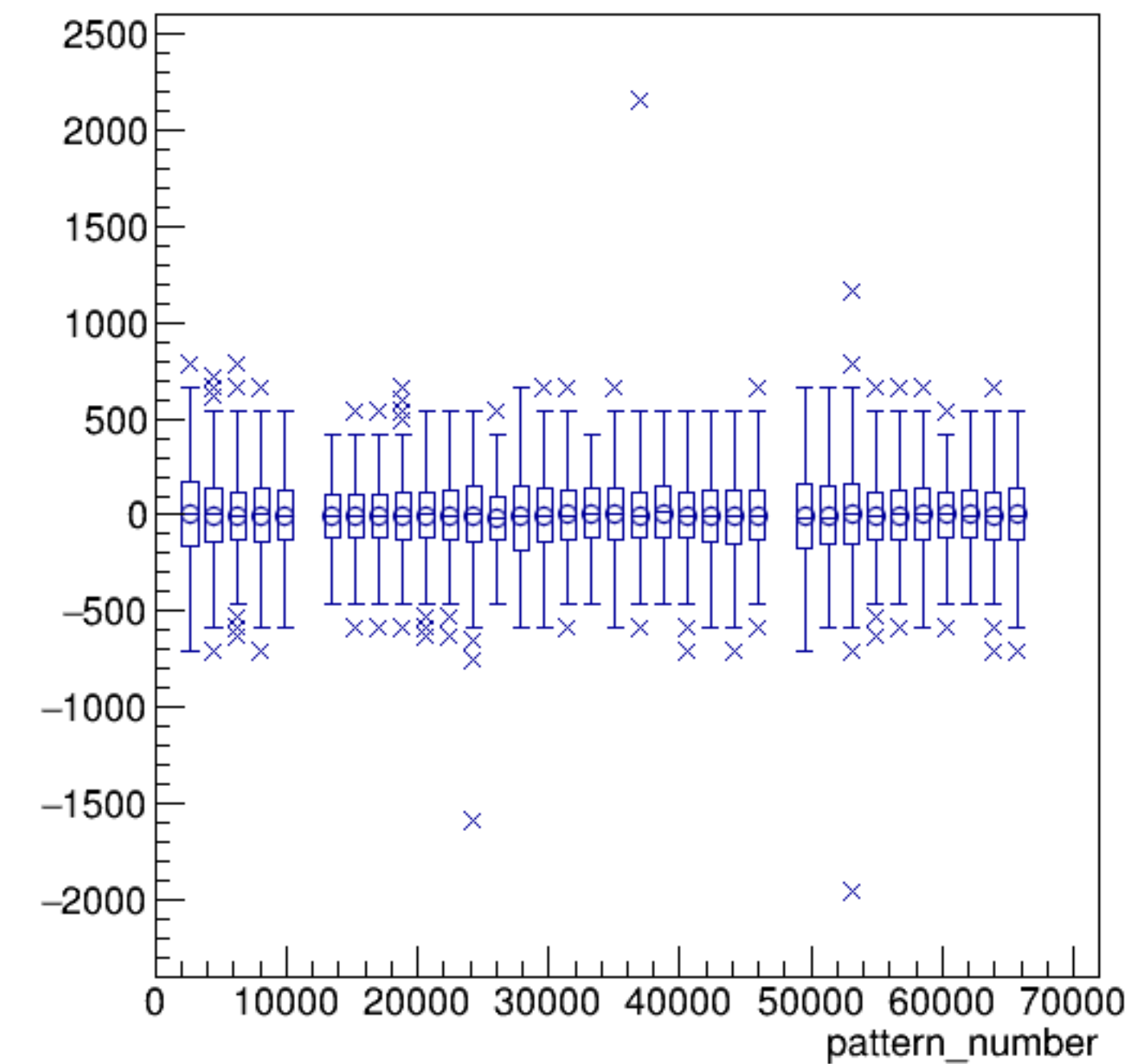
asym_sam7/ppm:pattern_number {ErrorFlag==0}
