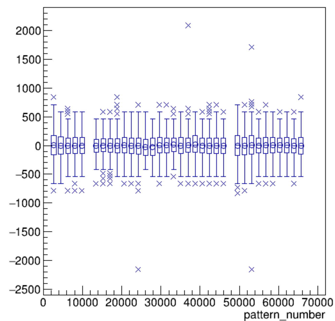
asym_sam8/ppm:pattern_number {ErrorFlag==0}
