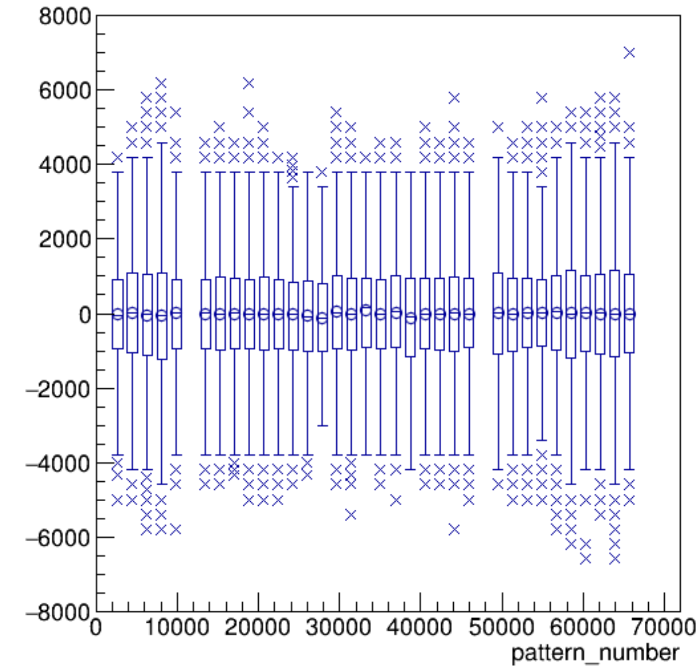
asym_sam5/ppm:pattern_number {ErrorFlag==0}
