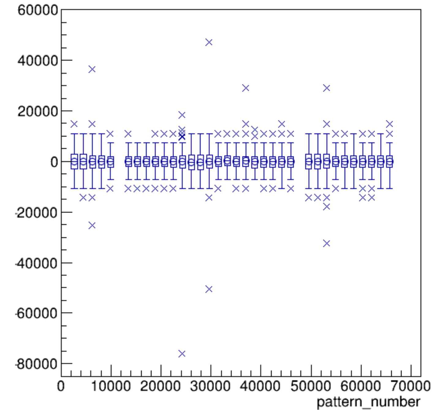
asym_sam4/ppm:pattern_number {ErrorFlag==0}
