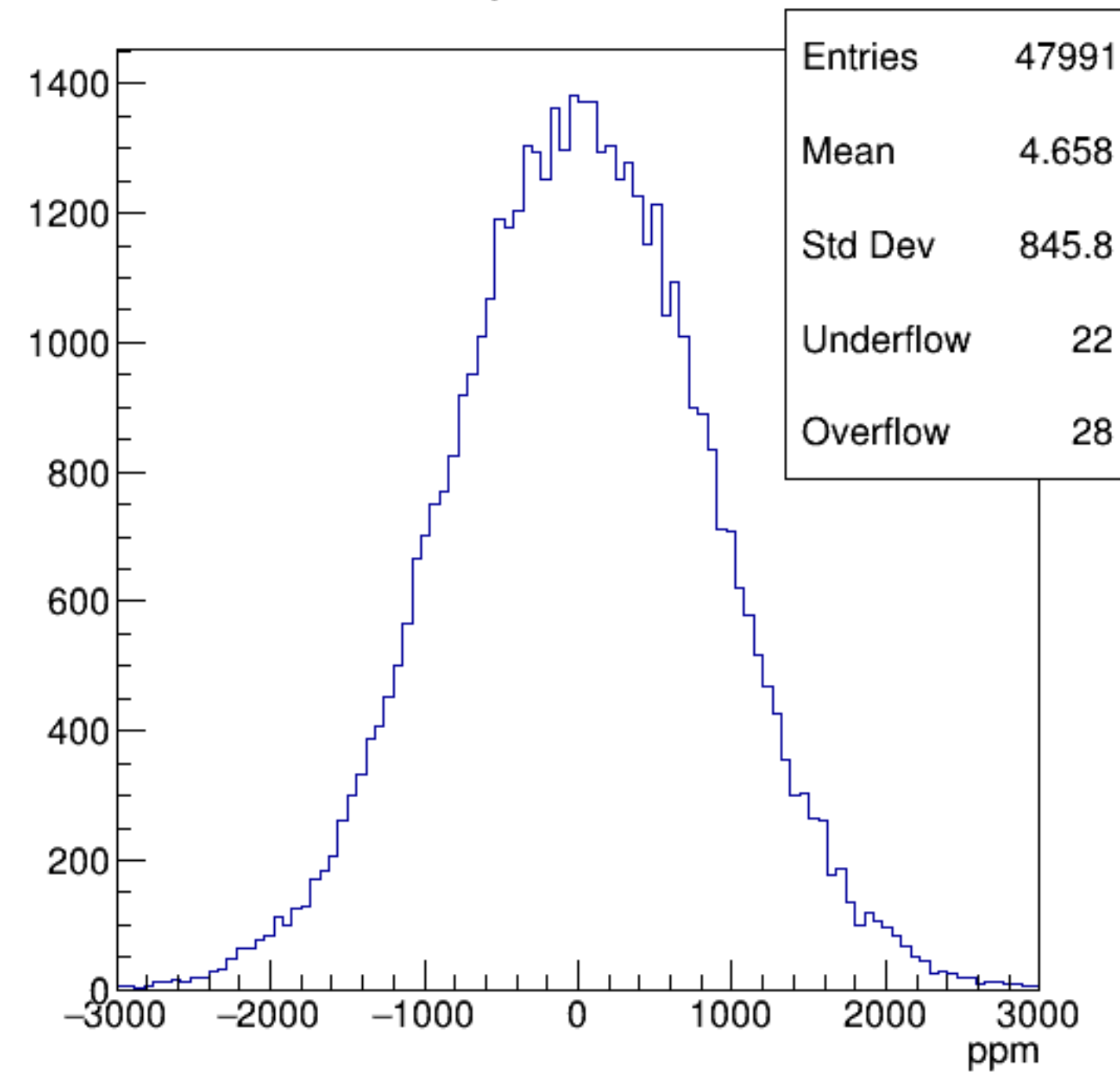
asym_sam3
