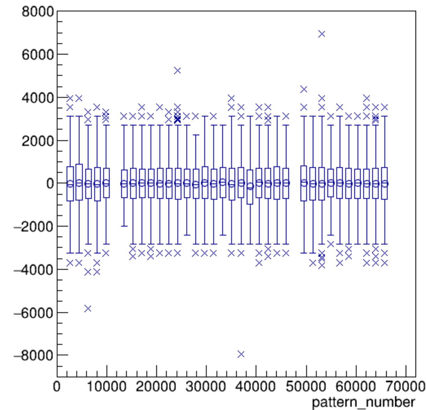
asym_sam6/ppm:pattern_number {ErrorFlag==0}
