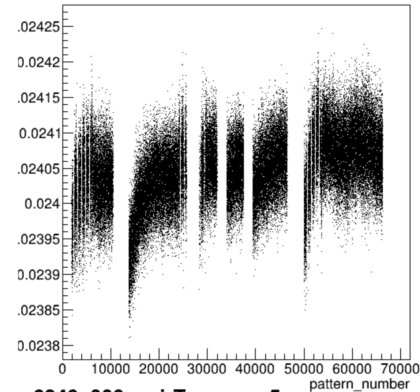
yield_sam5:pattern_number {ErrorFlag==0}
