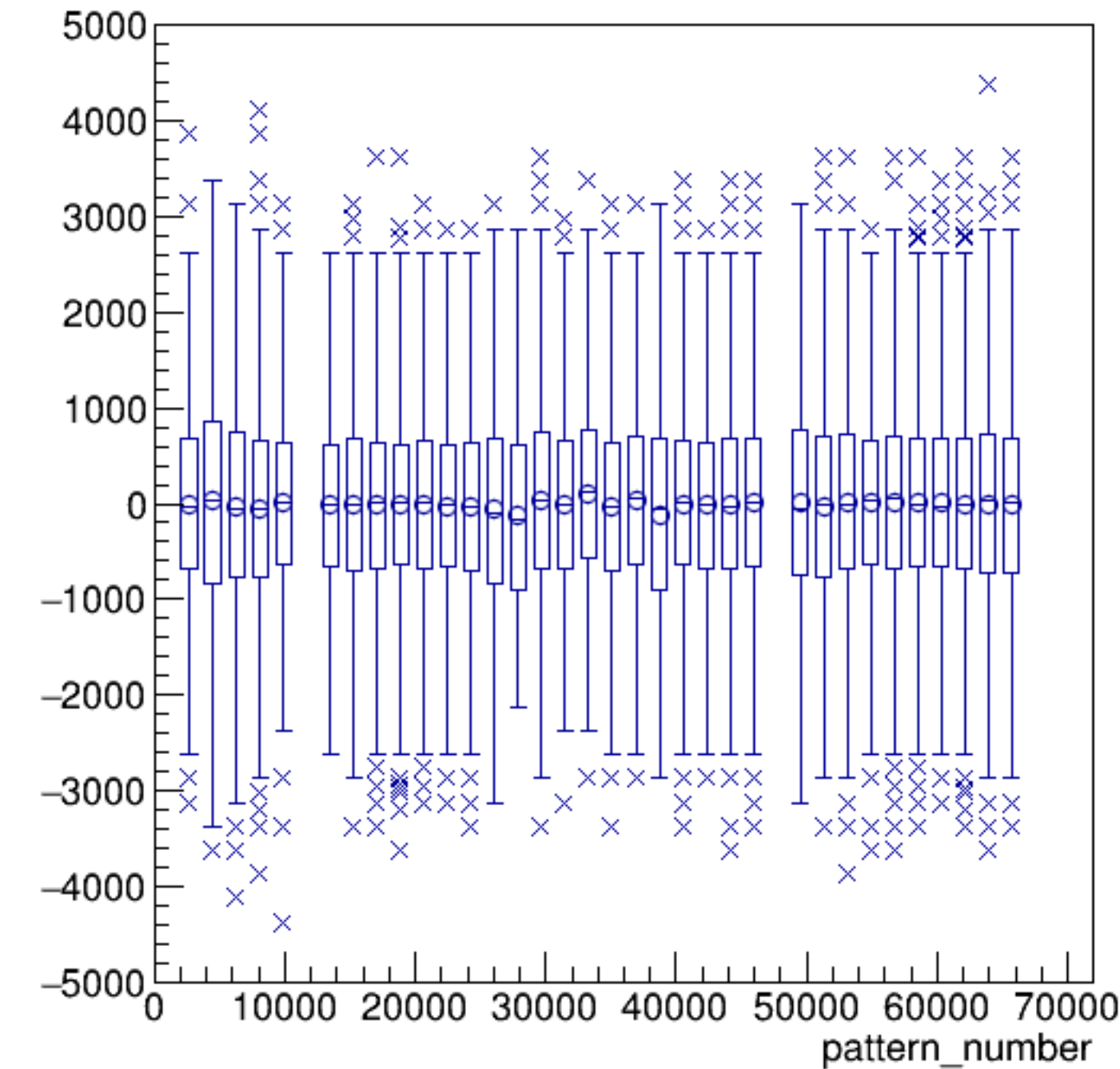
asym_sam5/ppm:pattern_number {ErrorFlag==0}
