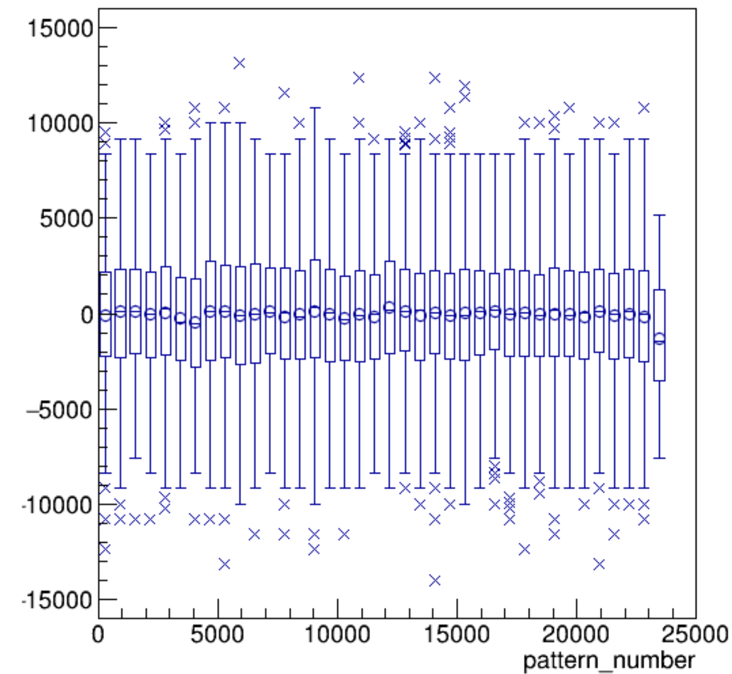
asym_atr1/ppm:pattern_number {ErrorFlag==0}
