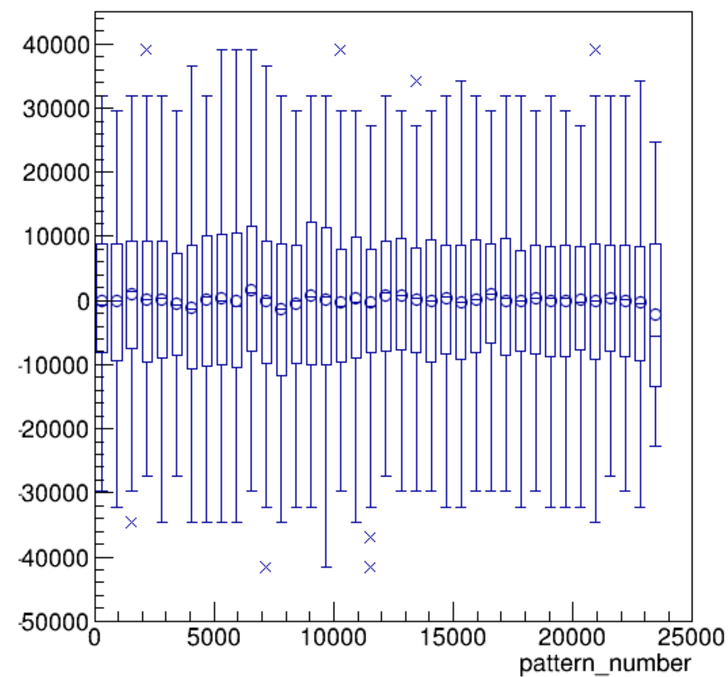
asym_atr2/ppm:pattern_number {ErrorFlag==0}
