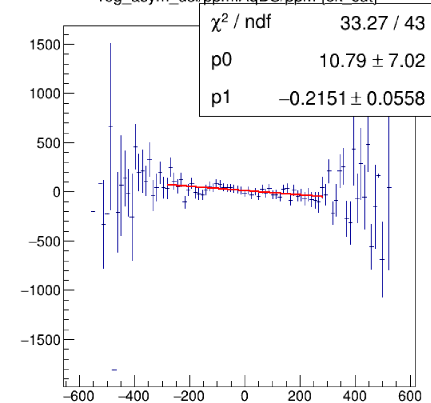
reg_asym_usl/ppm:AqDS/ppm {ok_cut}
