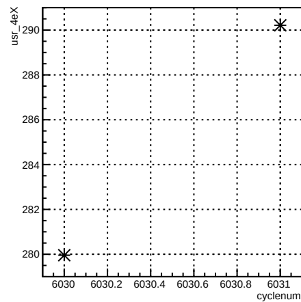
usr_4eX:cyclenum {run == 6351}
