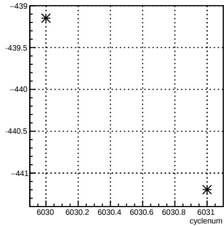
1X_coil1:cyclenum {run == 6351}
