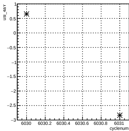
usl_4aY:cyclenum {run == 6351}
