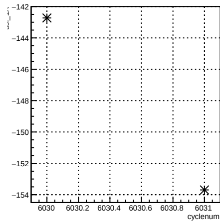
usl_1X:cyclenum {run == 6351}
