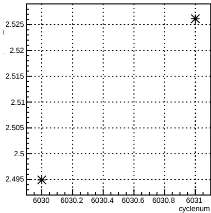
alpha46_4eY4aY:cyclenum {run == 6351}
