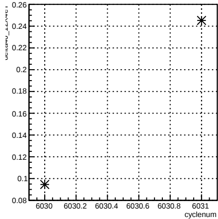
delta46_12X4eY:cyclenum {run == 6351}
