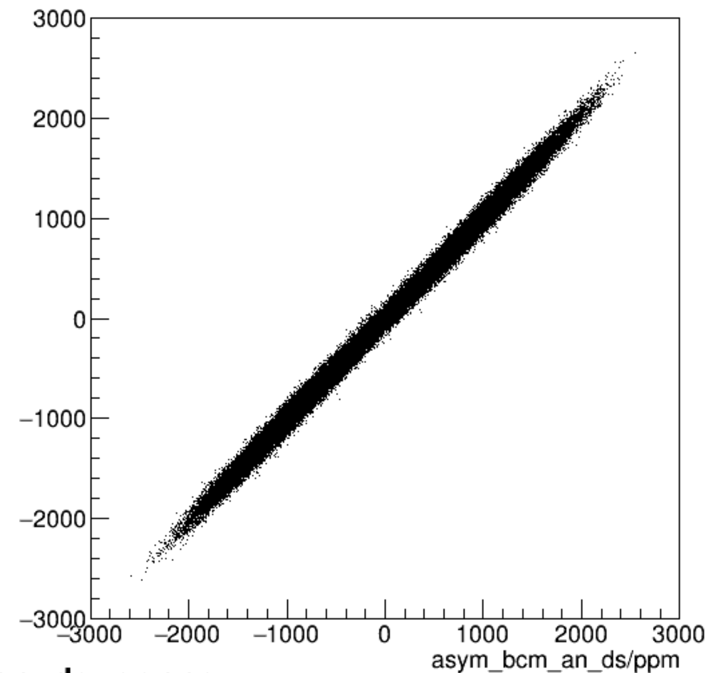
run6352_000_asym_bcm_dg_us_vs_asym_bcm_an_ds_pr.png
