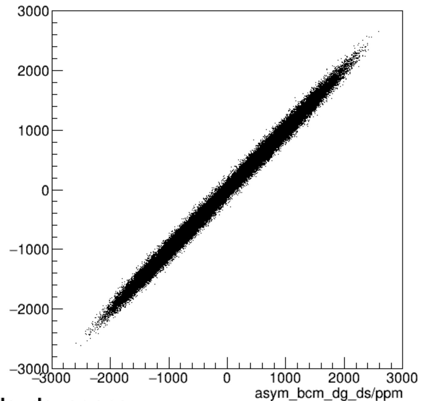
run6352_000_asym_bcm_dg_us_vs_asym_bcm_dg_ds_pr.png
