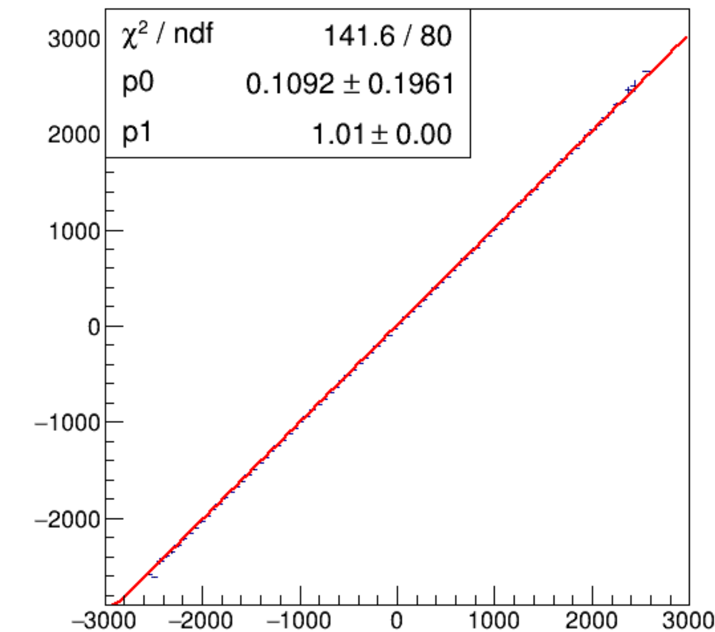
run6352_000_asym_bcm_dg_us_vs_asym_bcm_an_ds3_pr.png
