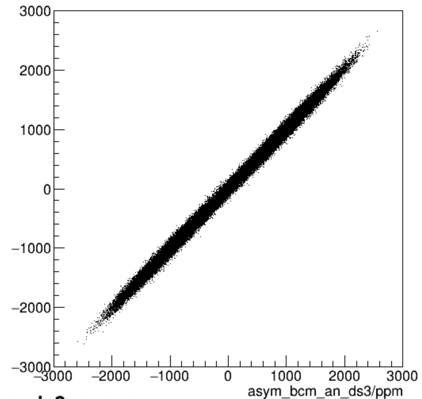
run6352_000_asym_bcm_dg_us_vs_asym_bcm_an_ds3_pr.png
