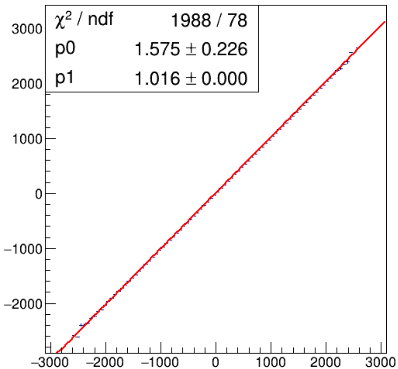
run6352_000_asym_bcm_dg_us_vs_asym_bcm_dg_ds_pr.png
