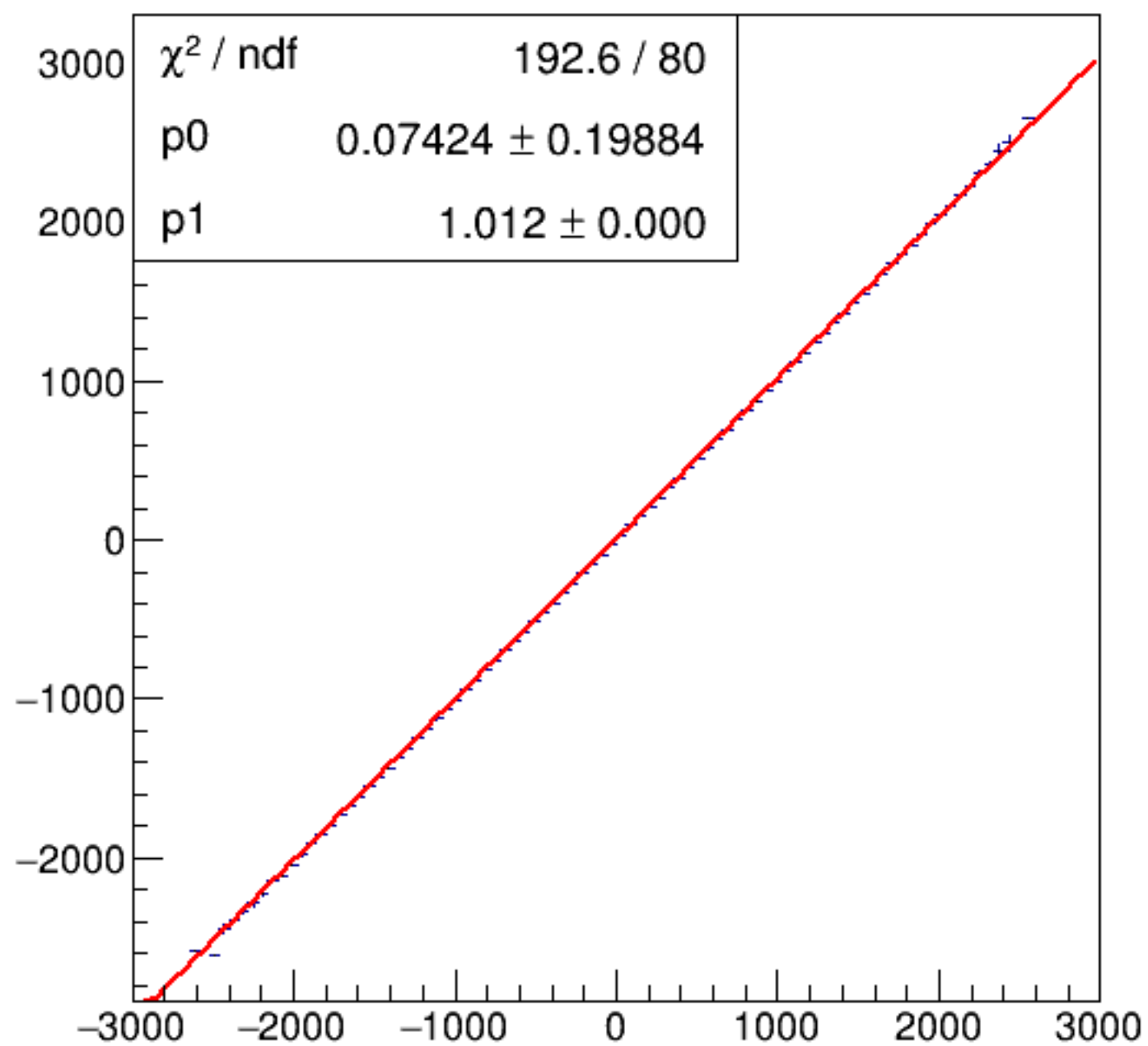
run6352_000_asym_bcm_dg_us_vs_asym_bcm_an_ds_pr.png
