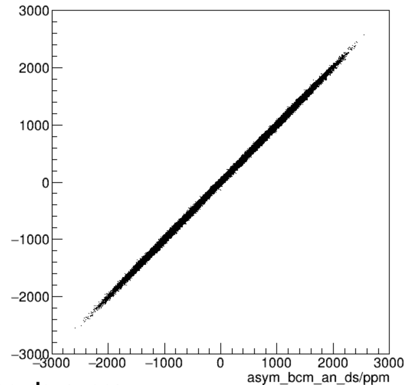
run6352_000_asym_bcm_an_us_vs_asym_bcm_an_ds_pr.png
