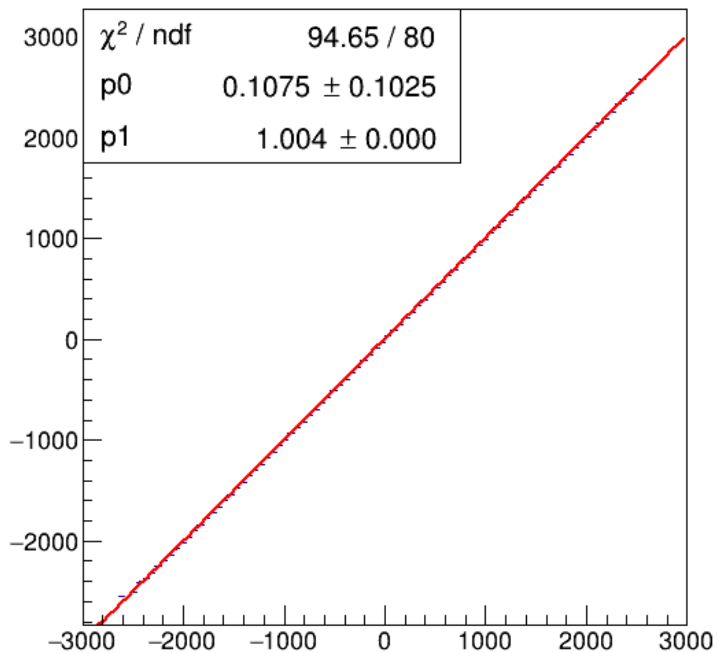
run6352_000_asym_bcm_an_us_vs_asym_bcm_an_ds_pr.png
