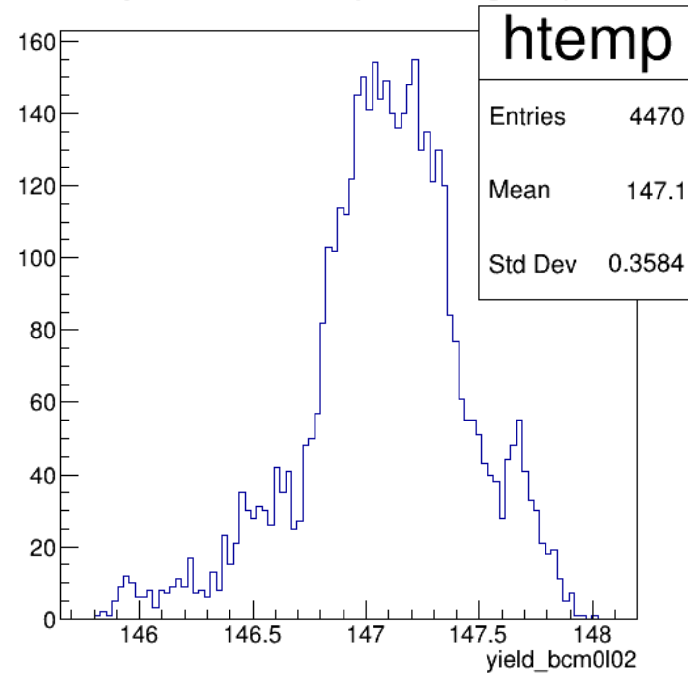
yield_bcm0l02 {ErrorFlag==0}
