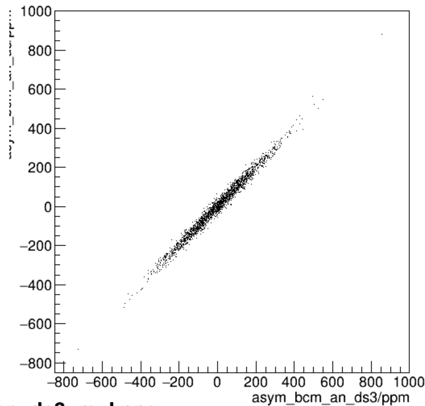
run6353_000_asym_bcm_an_us_vs_asym_bcm_an_ds3_mul.png
