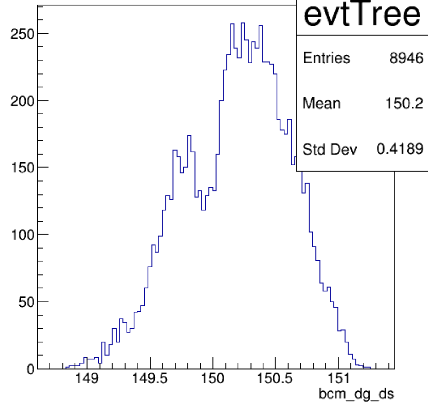
bcm_dg_ds {ErrorFlag==0}
