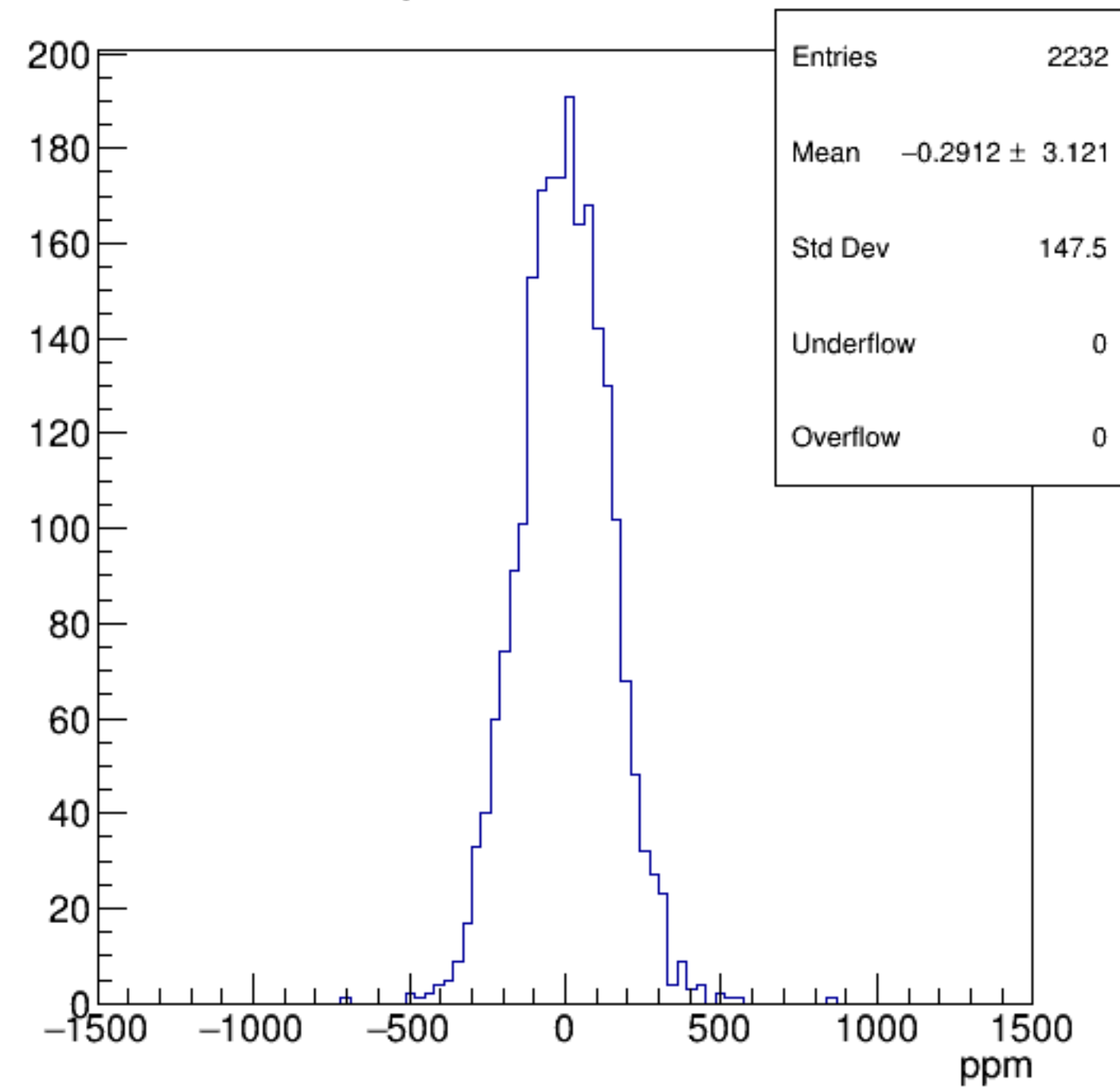
asym_bcm_an_ds
