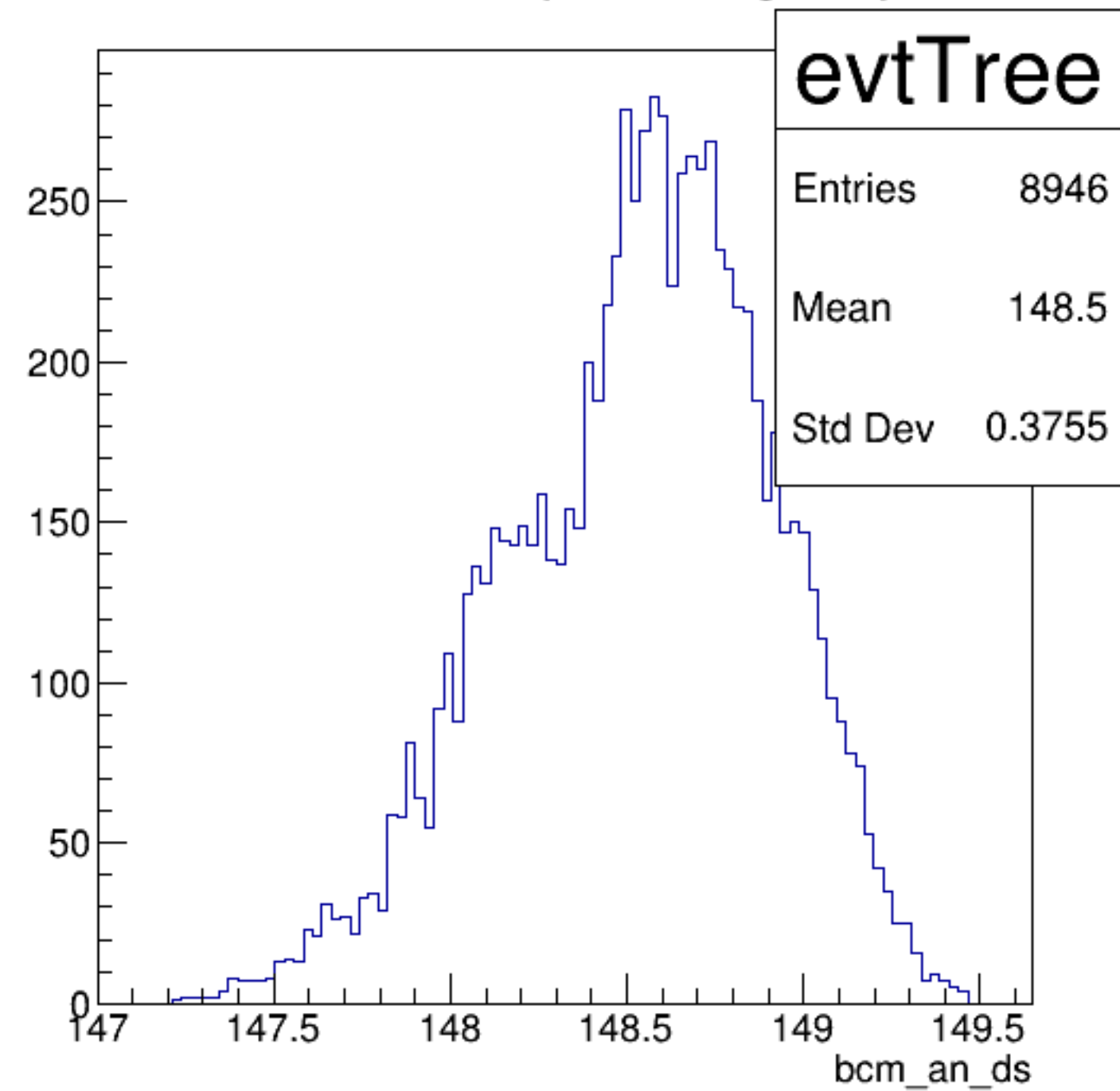
bcm_an_ds {ErrorFlag==0}
