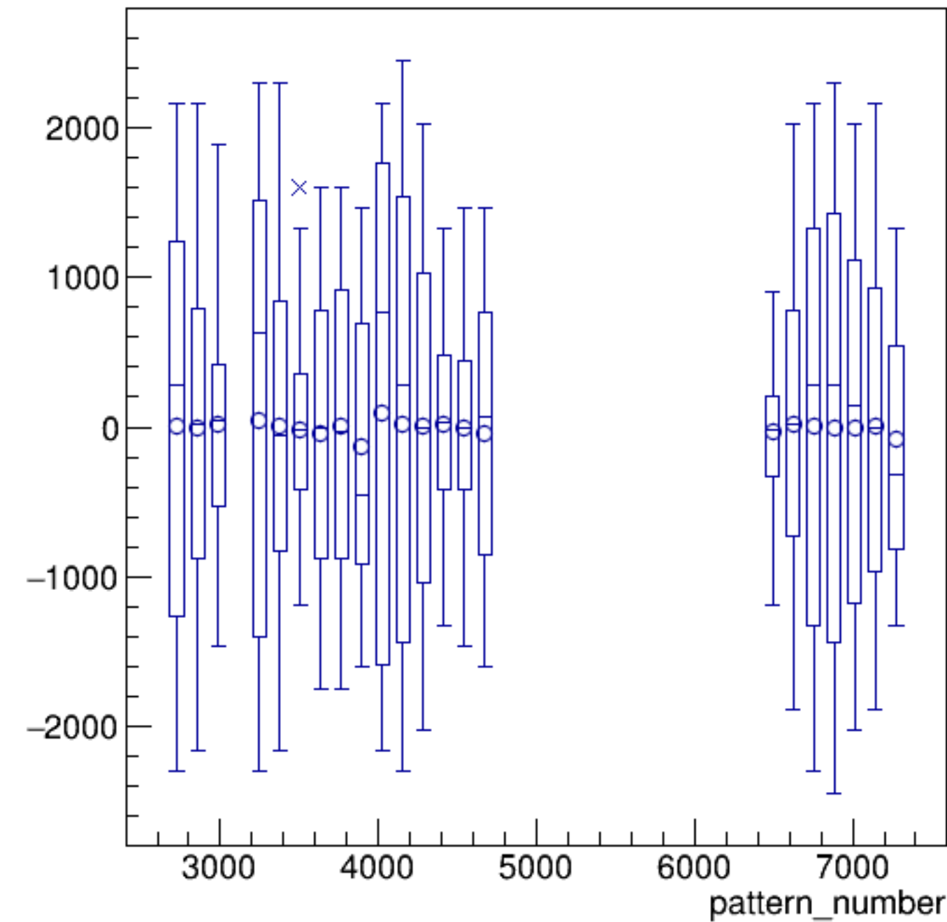
asym_bcm_dg_ds/ppm:pattern_number {ErrorFlag==0}
