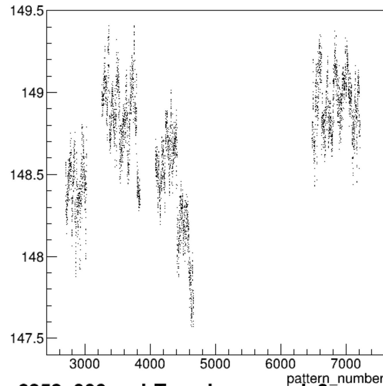
yield_bcm_an_ds3:pattern_number {ErrorFlag==0}
