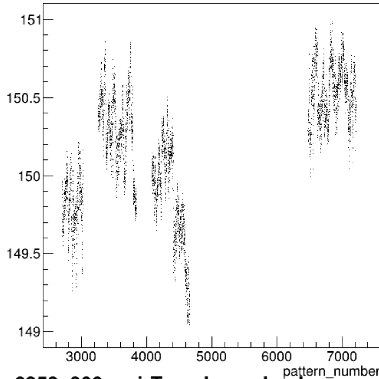
yield_bcm_dg_ds:pattern_number {ErrorFlag==0}
