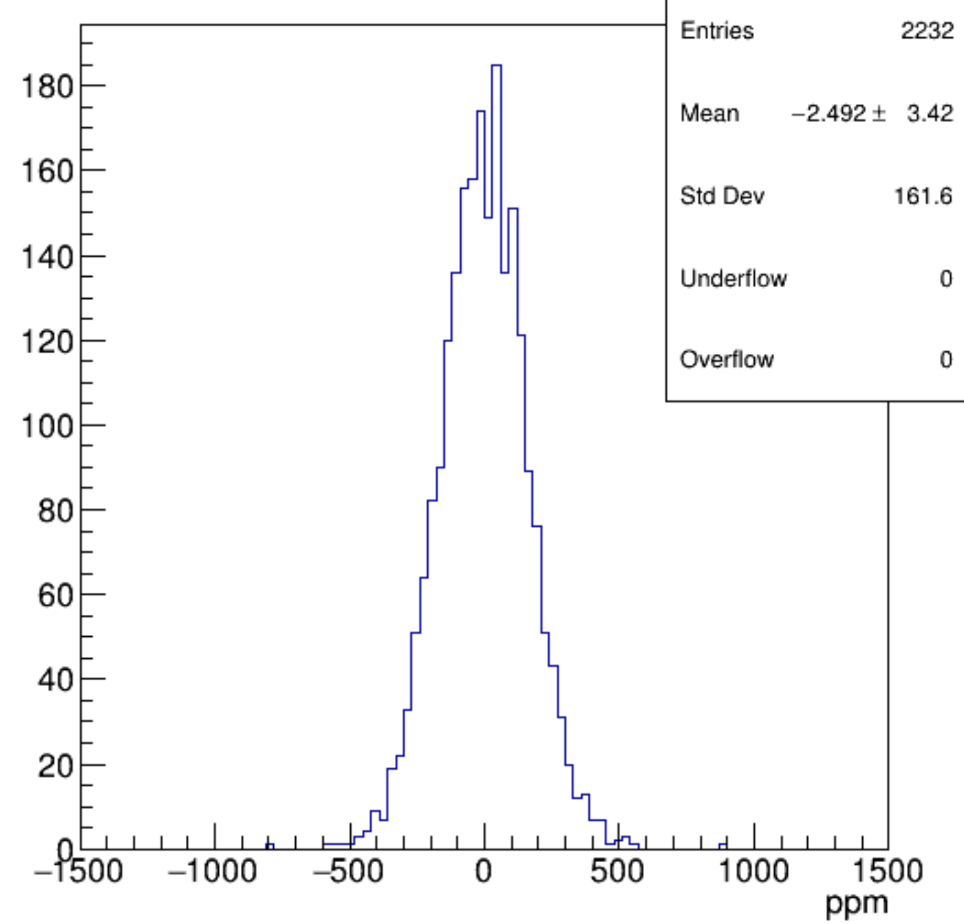
asym_bcm0l02
