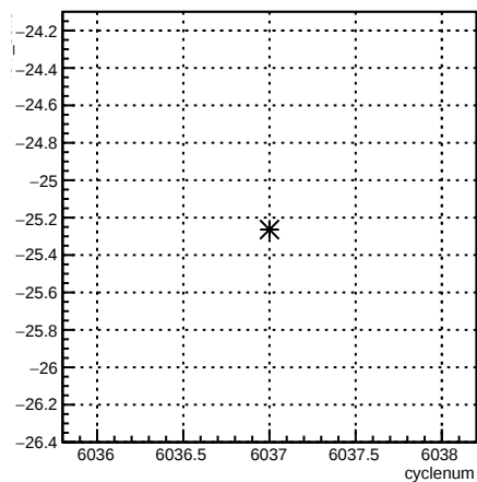
4eY_coil6:cyclenum {run == 6354}
