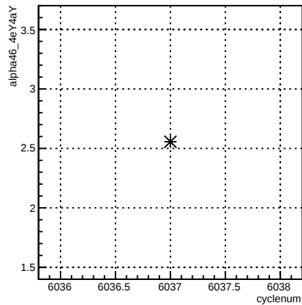
alpha46_4eY4aY:cyclenum {run == 6354}
