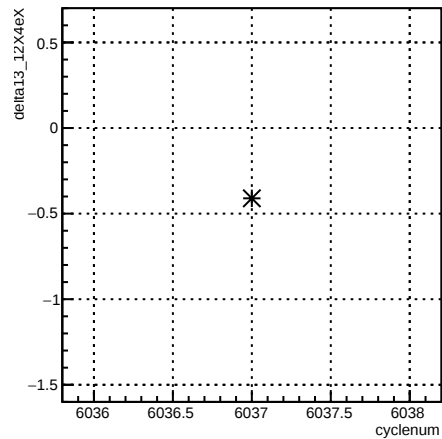
delta13_12X4eX:cyclenum {run == 6354}
