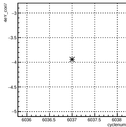
4eY_coil7:cyclenum {run == 6354}
