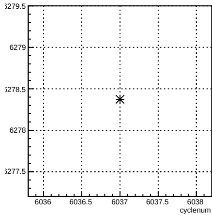
usl_coil3:cyclenum {run == 6354}
