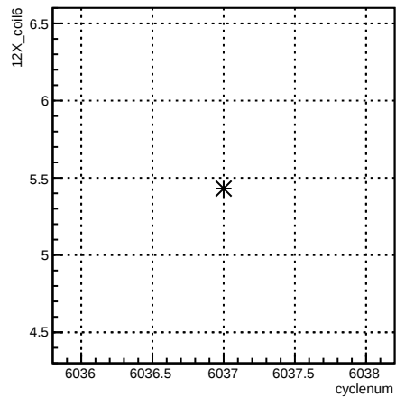
12X_coil6:cyclenum {run == 6354}
