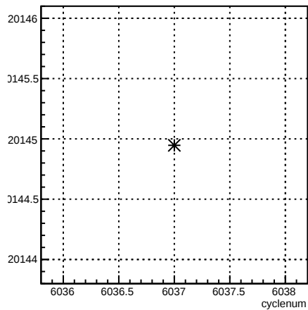
usr_coil7:cyclenum {run == 6354}
