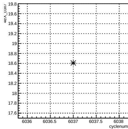
4eX_coil7:cyclenum {run == 6354}
