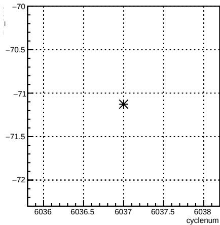
1X_coil3:cyclenum {run == 6354}
