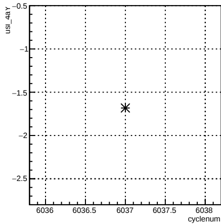
usl_4aY:cyclenum {run == 6354}
