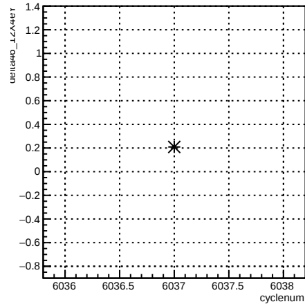
delta46_12X4eY:cyclenum {run == 6354}
