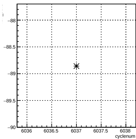
4eX_coil3:cyclenum {run == 6354}
