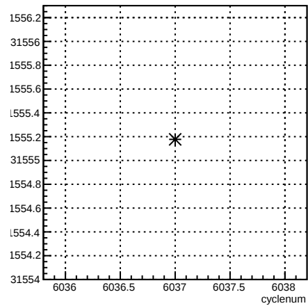
usl_coil6:cyclenum {run == 6354}
