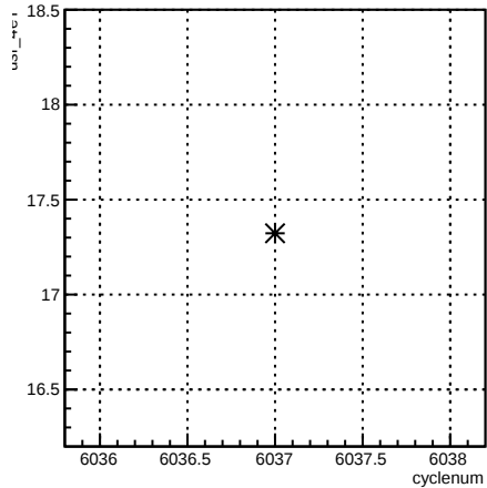
usr_4eY:cyclenum {run == 6354}
