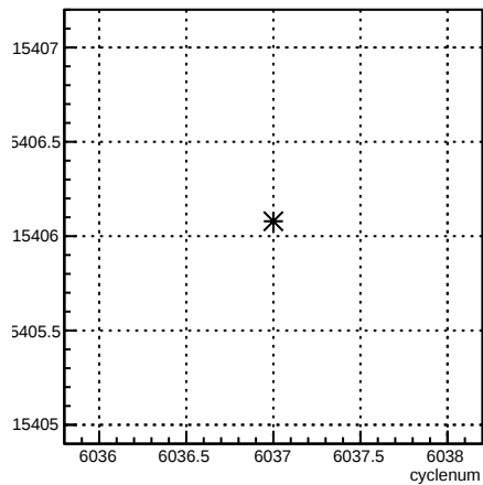
usl_coil7:cyclenum {run == 6354}
