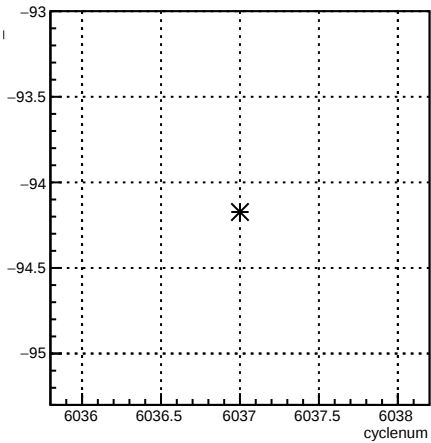
usl_1X:cyclenum {run == 6354}
