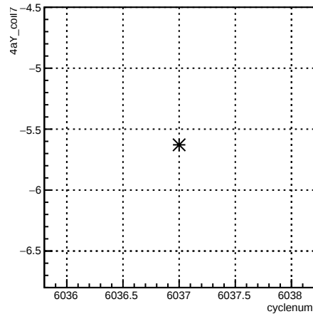
4aY_coil7:cyclenum {run == 6354}
