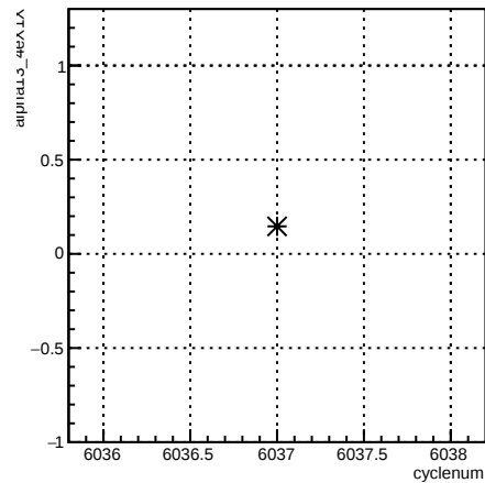
alpha13_4eX1X:cyclenum {run == 6354}
