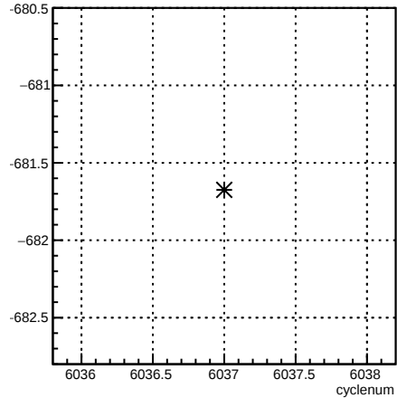
usr_coil6:cyclenum {run == 6354}
