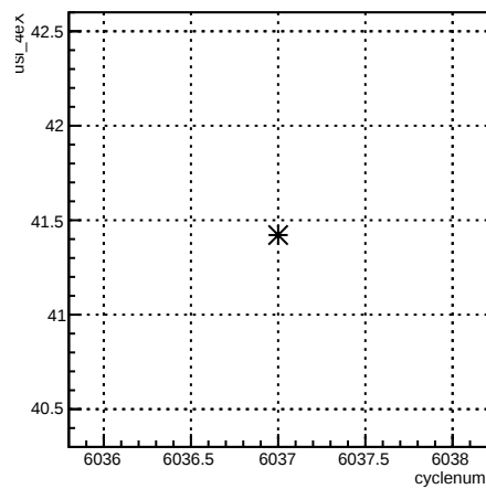
usl_4eX:cyclenum {run == 6354}
