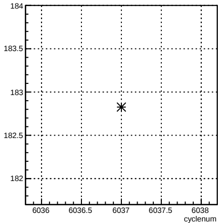
4eY_coil4:cyclenum {run == 6354}
