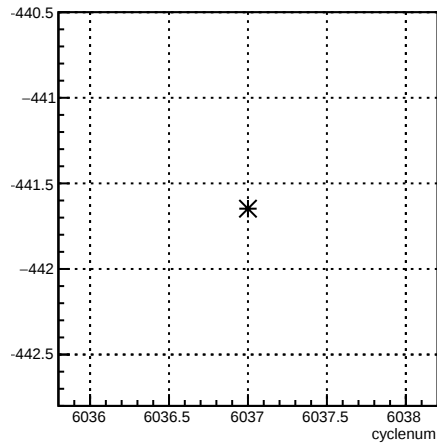
1X_coil1:cyclenum {run == 6354}
