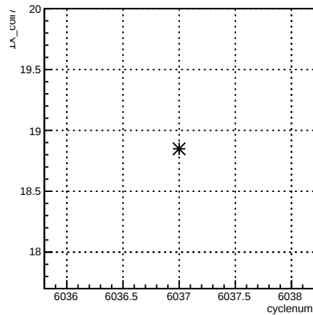
1X_coil7:cyclenum {run == 6354}
