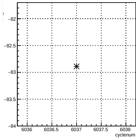
12X_coil7:cyclenum {run == 6354}
