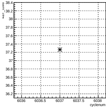
4aY_coil6:cyclenum {run == 6354}
