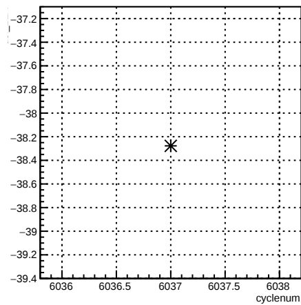
usl_12X:cyclenum {run == 6354}
