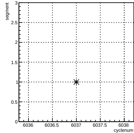
segment:cyclenum {run == 6354}
