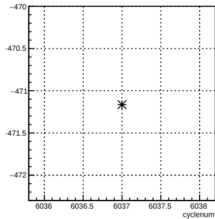
4eX_coil1:cyclenum {run == 6354}
