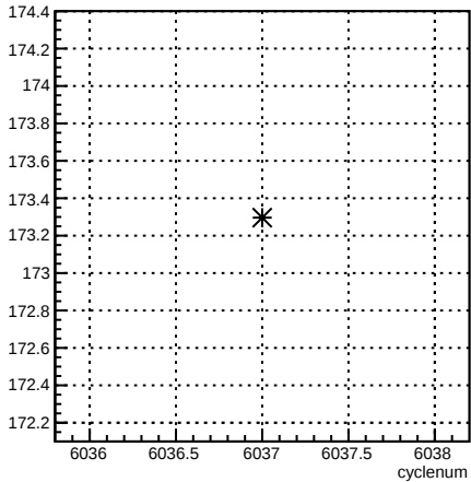
4aY_coil4:cyclenum {run == 6354}
