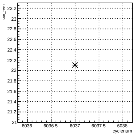
usl_4eY:cyclenum {run == 6354}
