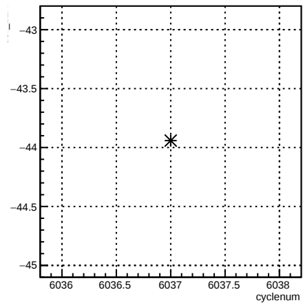
usr_12X:cyclenum {run == 6354}
