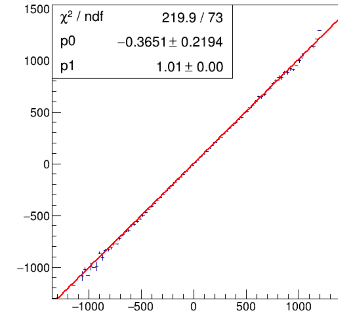
run6355_000_asym_bcm_dg_us_vs_asym_bcm_an_ds3_mul.png
