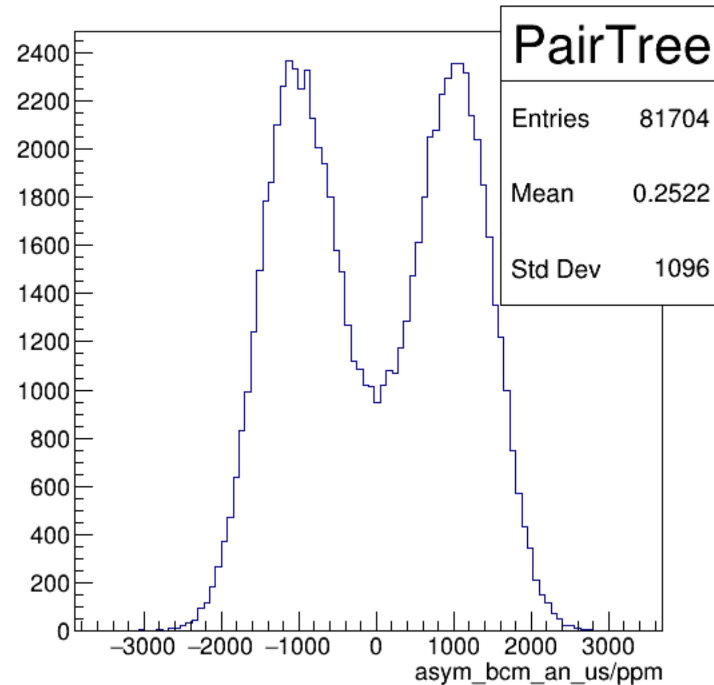
asym_bcm_an_us/ppm {ErrorFlag==0}
