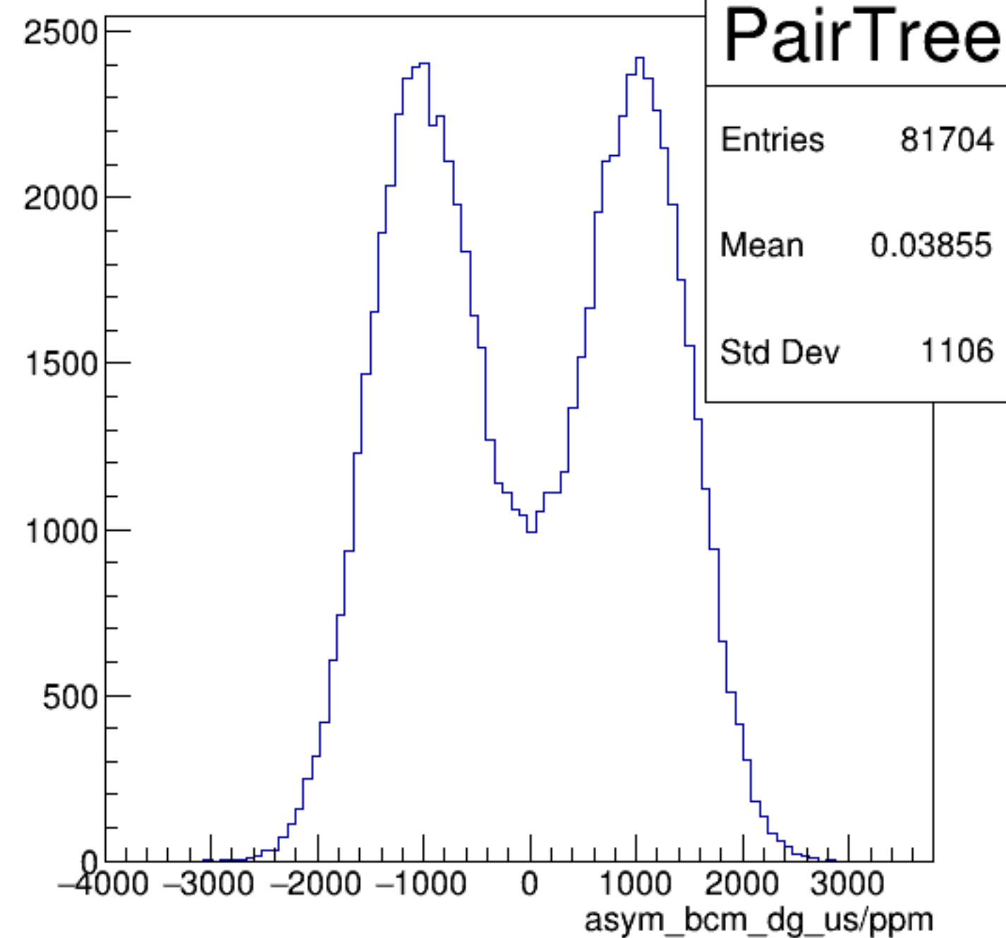
asym_bcm_dg_us/ppm {ErrorFlag==0}
