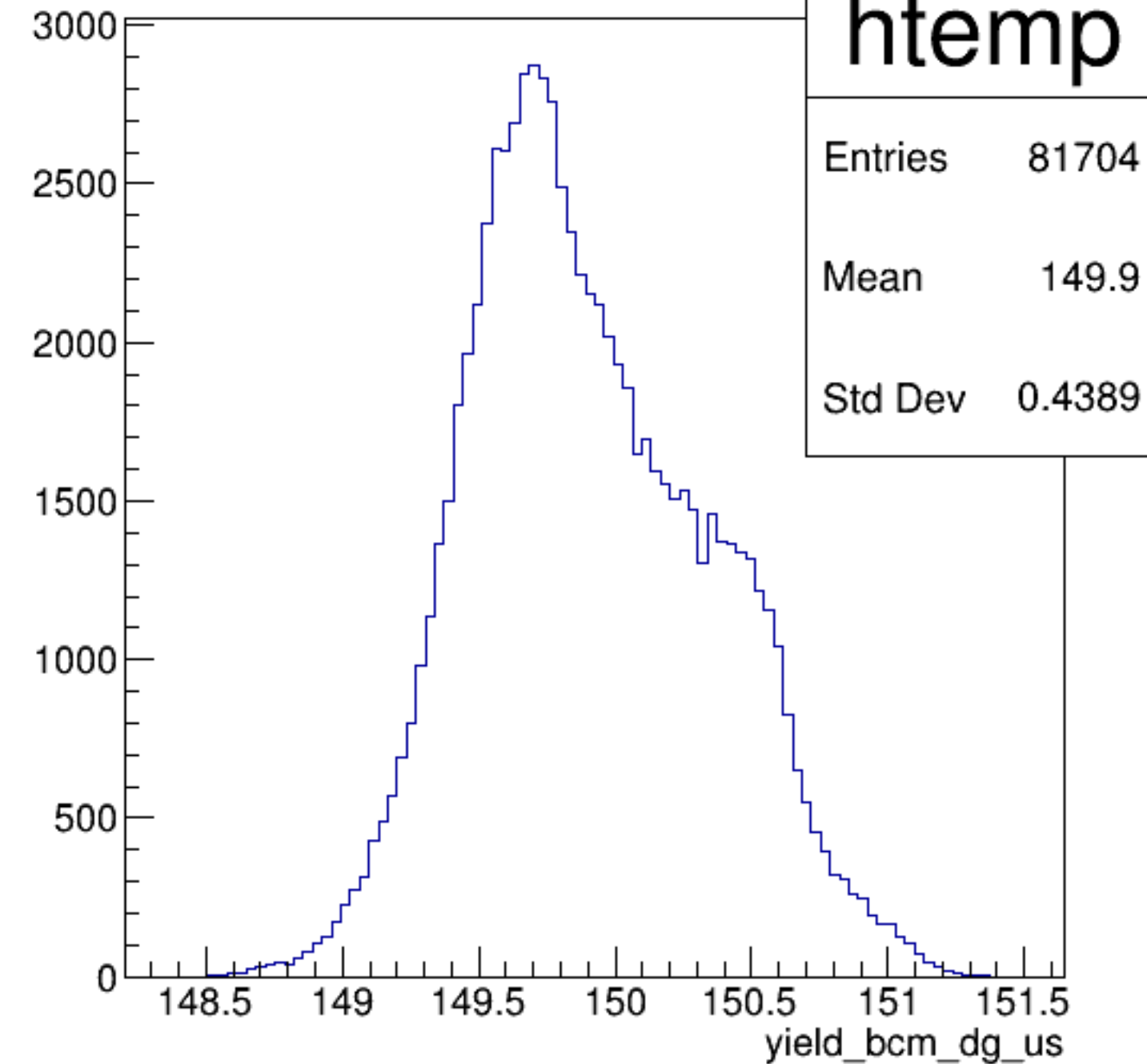
yield_bcm_dg_us {ErrorFlag==0}
