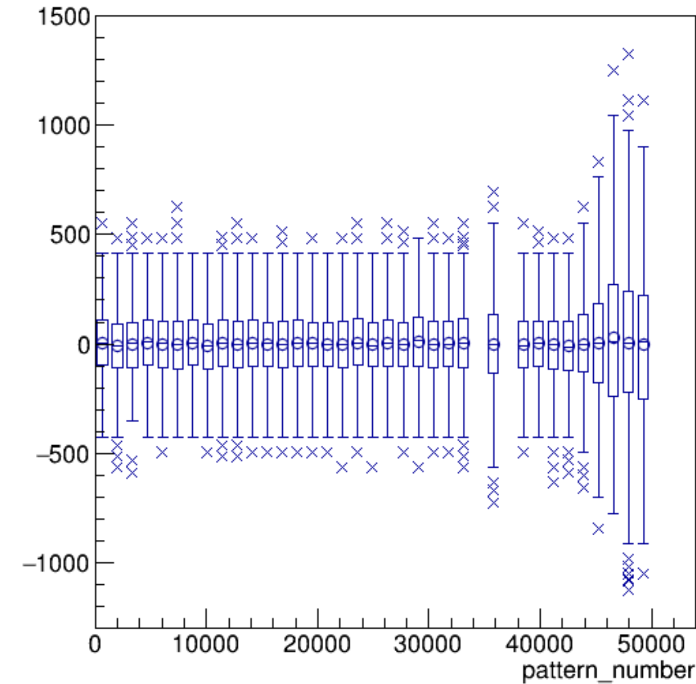
asym_bcm0l02/ppm:pattern_number {ErrorFlag==0}
