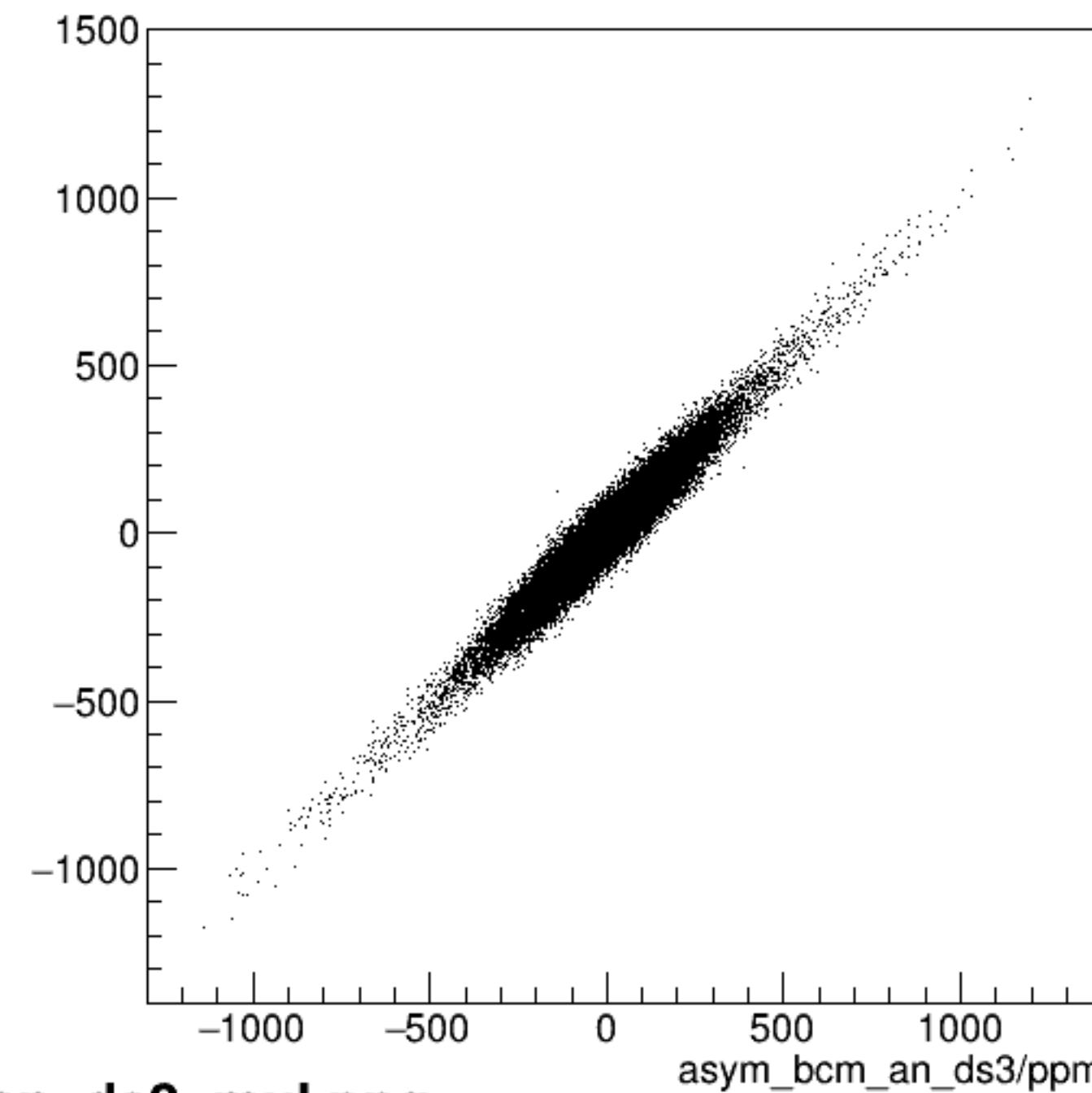
run6355_000_asym_bcm_dg_us_vs_asym_bcm_an_ds3_mul.png
