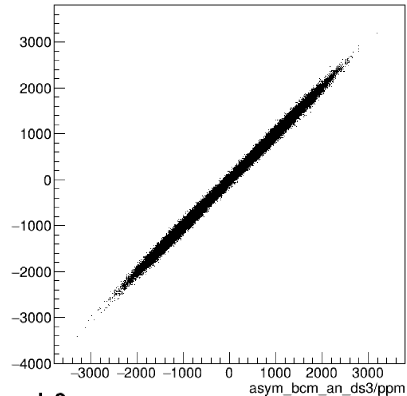
run6355_000_asym_bcm_dg_us_vs_asym_bcm_an_ds3_pr.png
