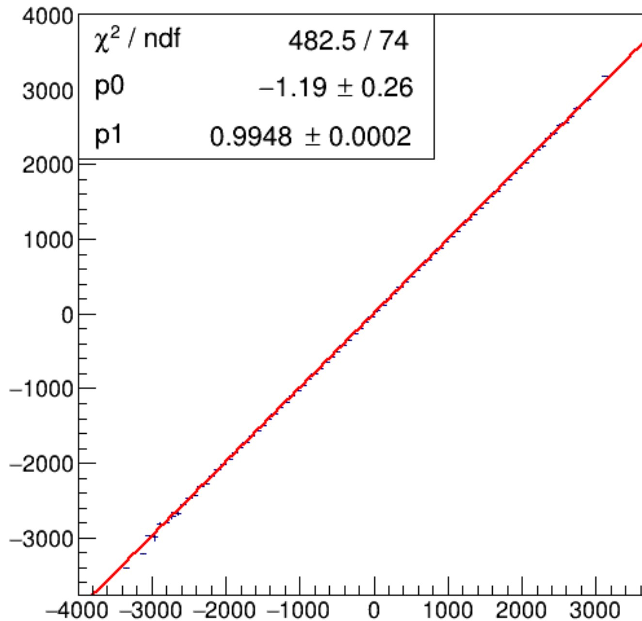
run6355_000_asym_bcm_dg_us_vs_asym_bcm_dg_ds_pr.png
