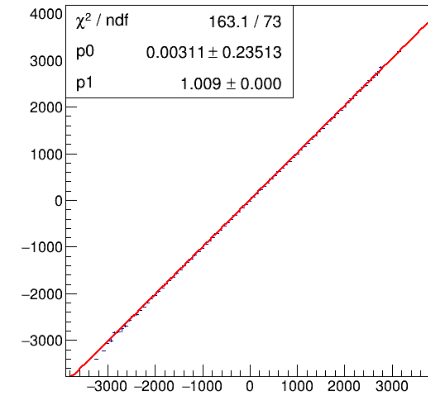
run6355_000_asym_bcm_dg_us_vs_asym_bcm_an_ds_pr.png
