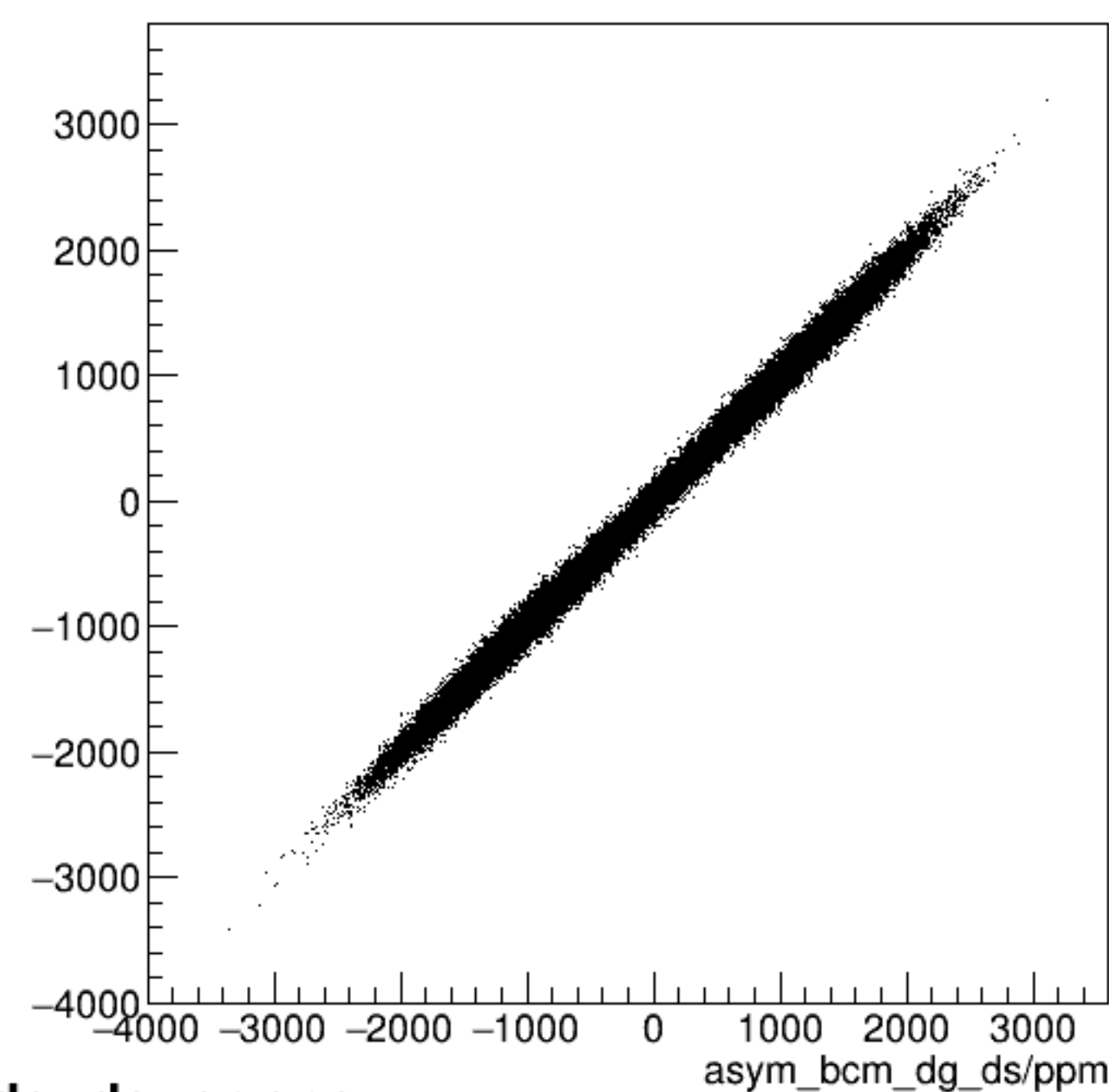
run6355_000_asym_bcm_dg_us_vs_asym_bcm_dg_ds_pr.png
