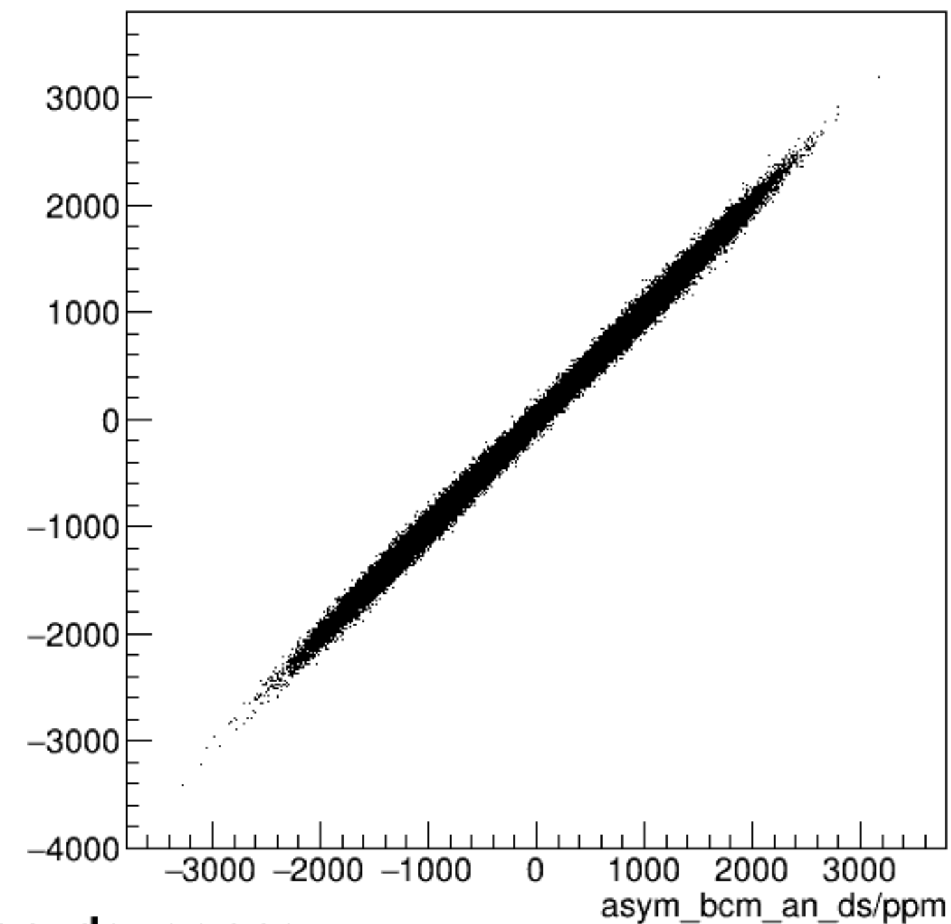
run6355_000_asym_bcm_dg_us_vs_asym_bcm_an_ds_pr.png
