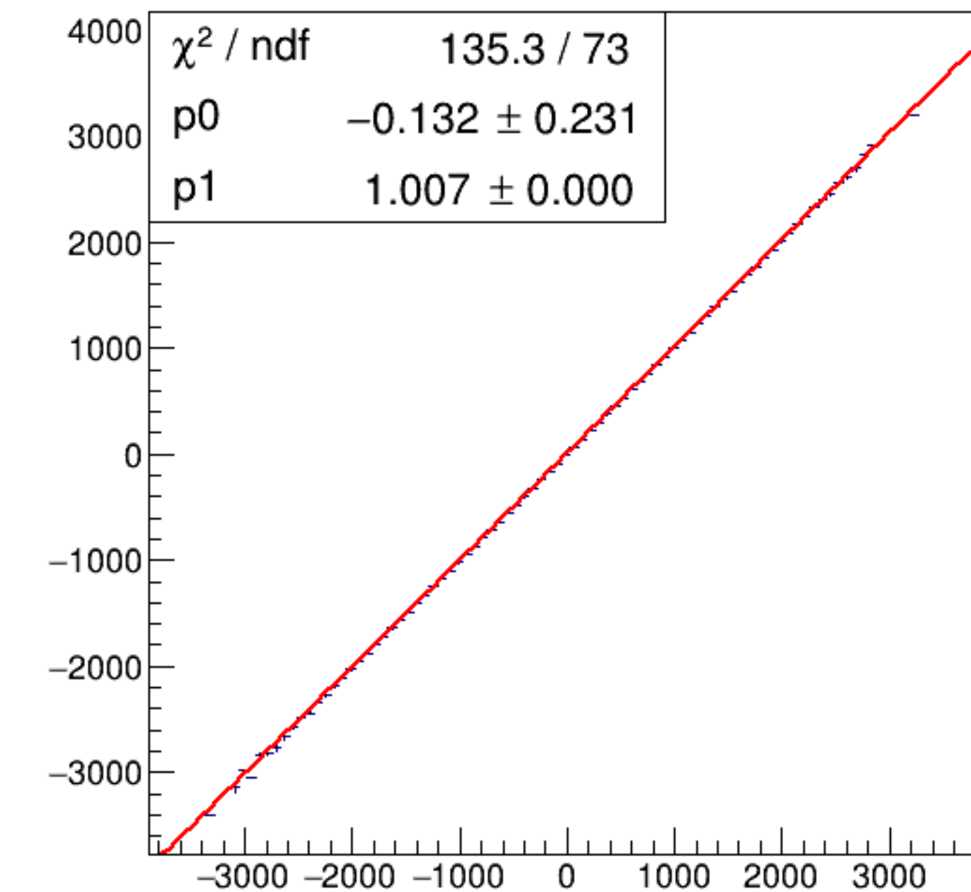
run6355_000_asym_bcm_dg_us_vs_asym_bcm_an_ds3_pr.png
