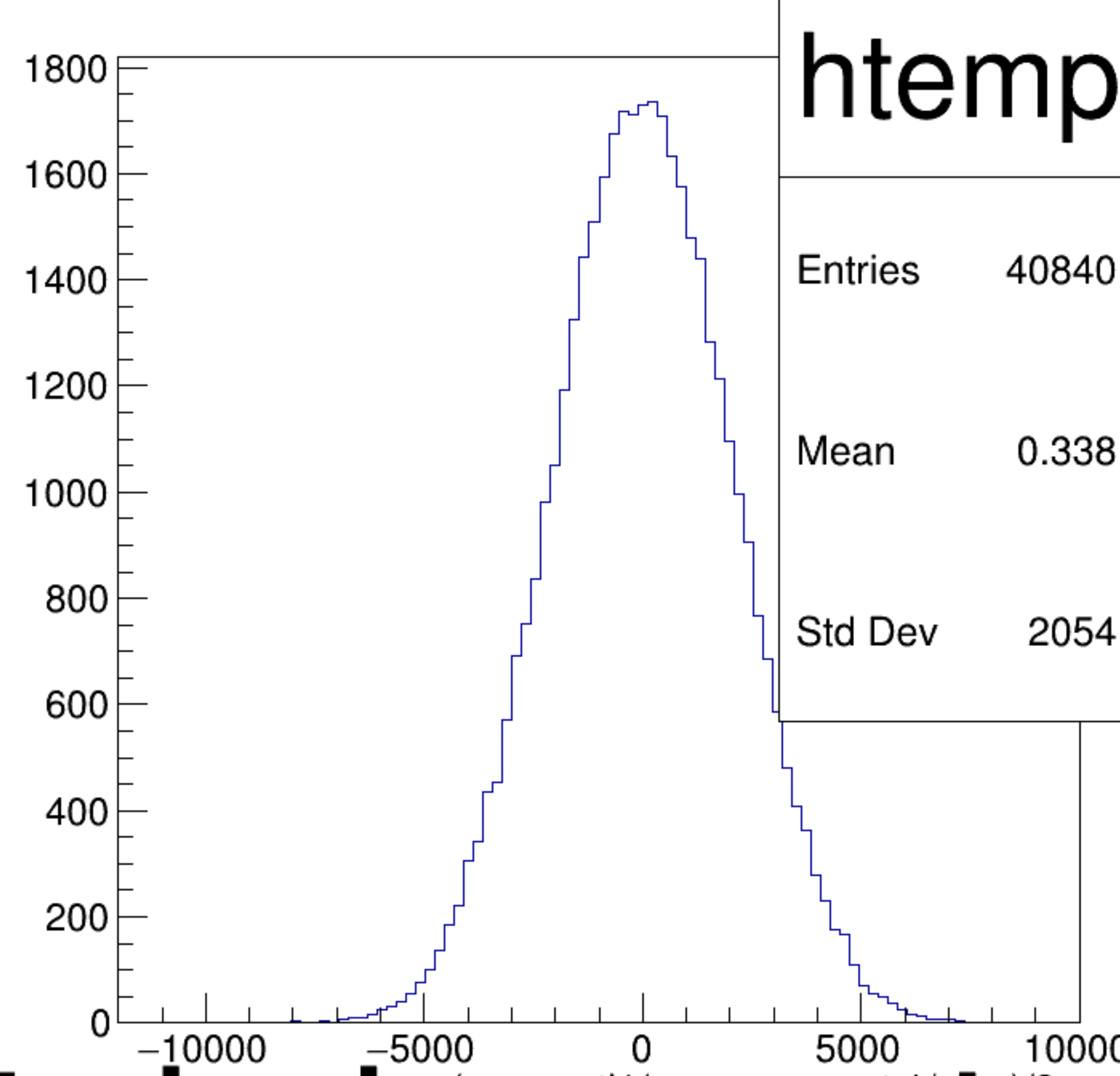
(asym_atl1/ppm+asym_atr1/ppm)/2 {ok_cut}
