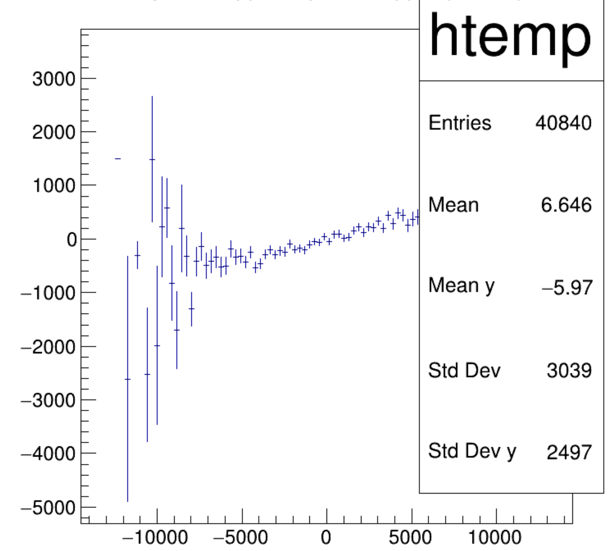
asym_atl1/ppm:asym_atr1/ppm {ok_cut}
