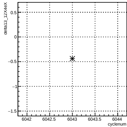
delta13_12X4eX:cyclenum {run == 6356}
