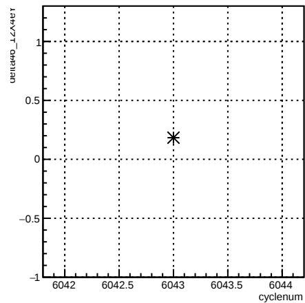
delta46_12X4eY:cyclenum {run == 6356}
