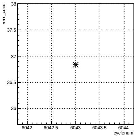
4aY_coil6:cyclenum {run == 6356}
