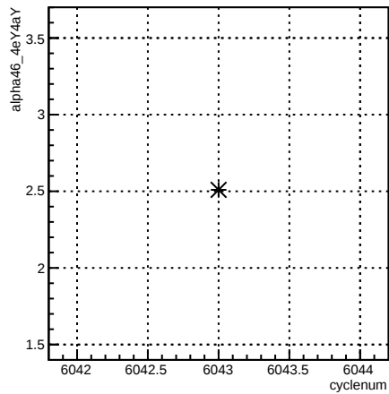
alpha46_4eY4aY:cyclenum {run == 6356}
