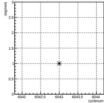
segment:cyclenum {run == 6356}
