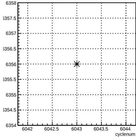
run:cyclenum {run == 6356}
