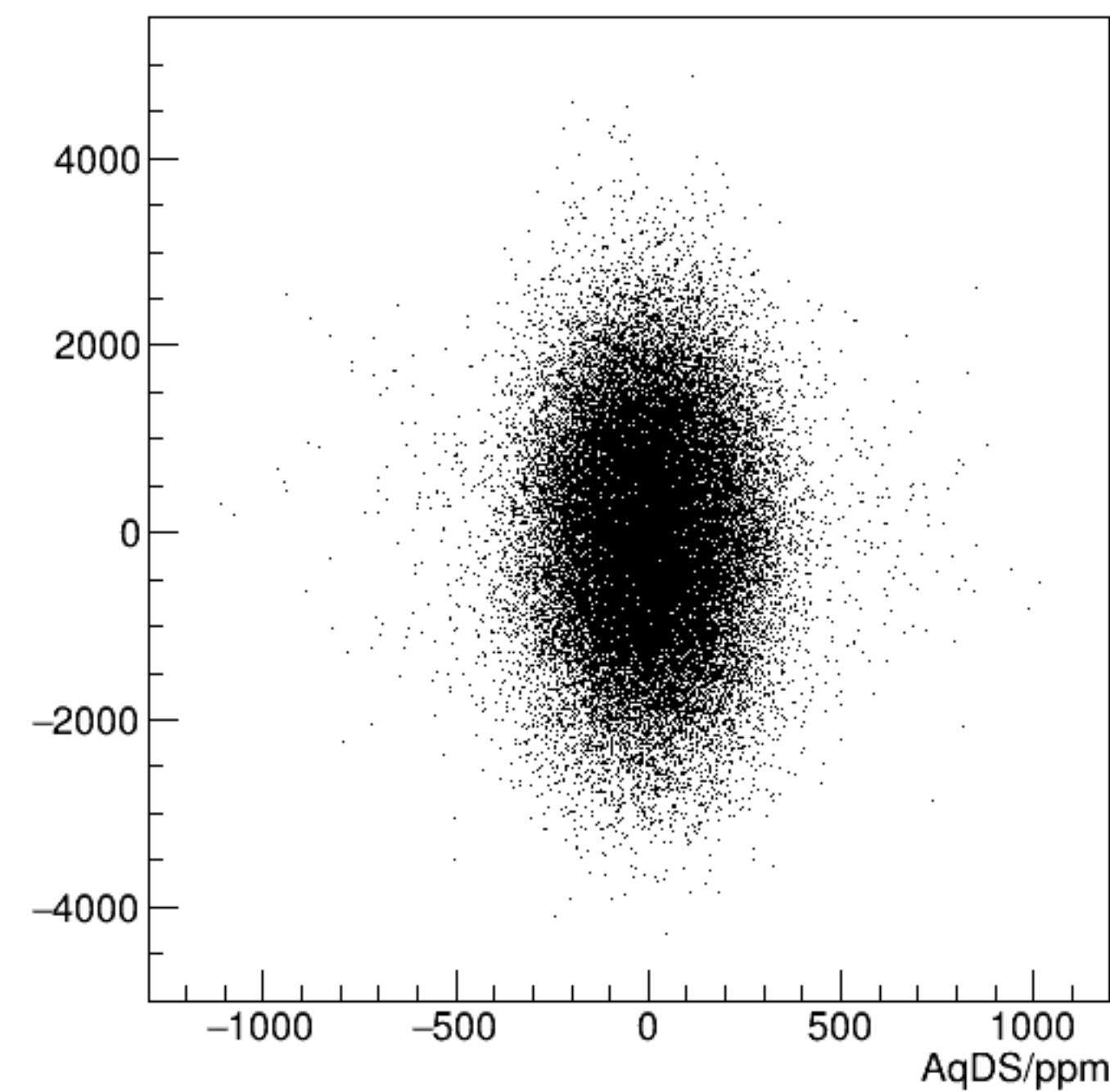
reg_asym_usr/ppm:AqDS/ppm {ok_cut}
