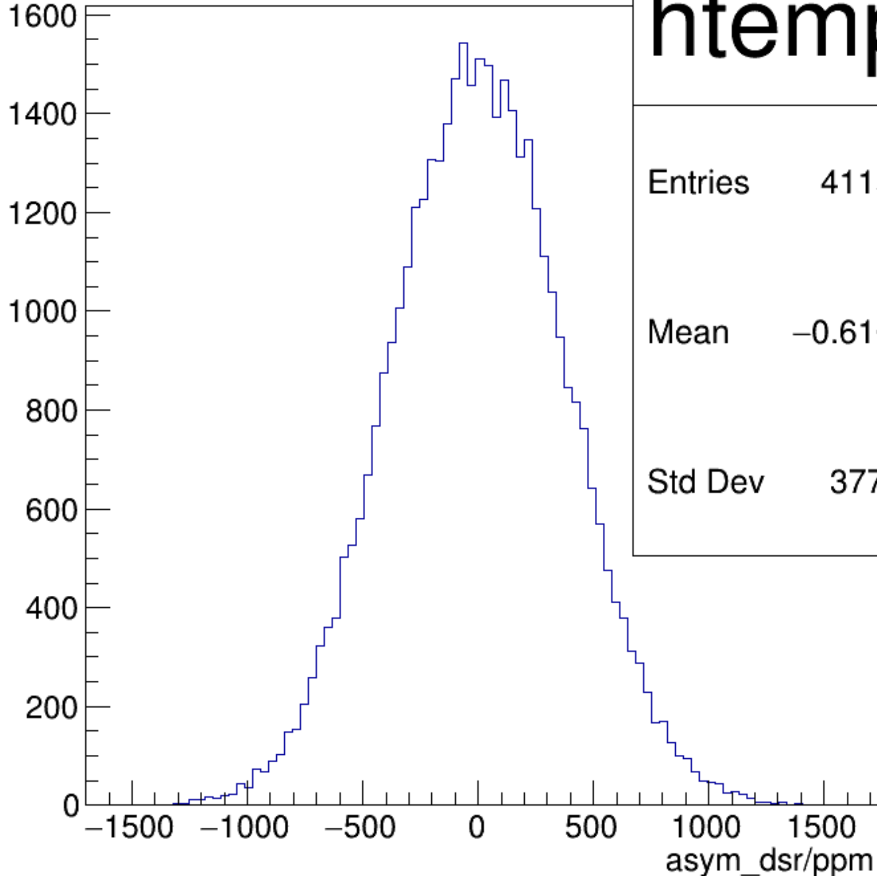
asym_dsr/ppm {ok_cut}
