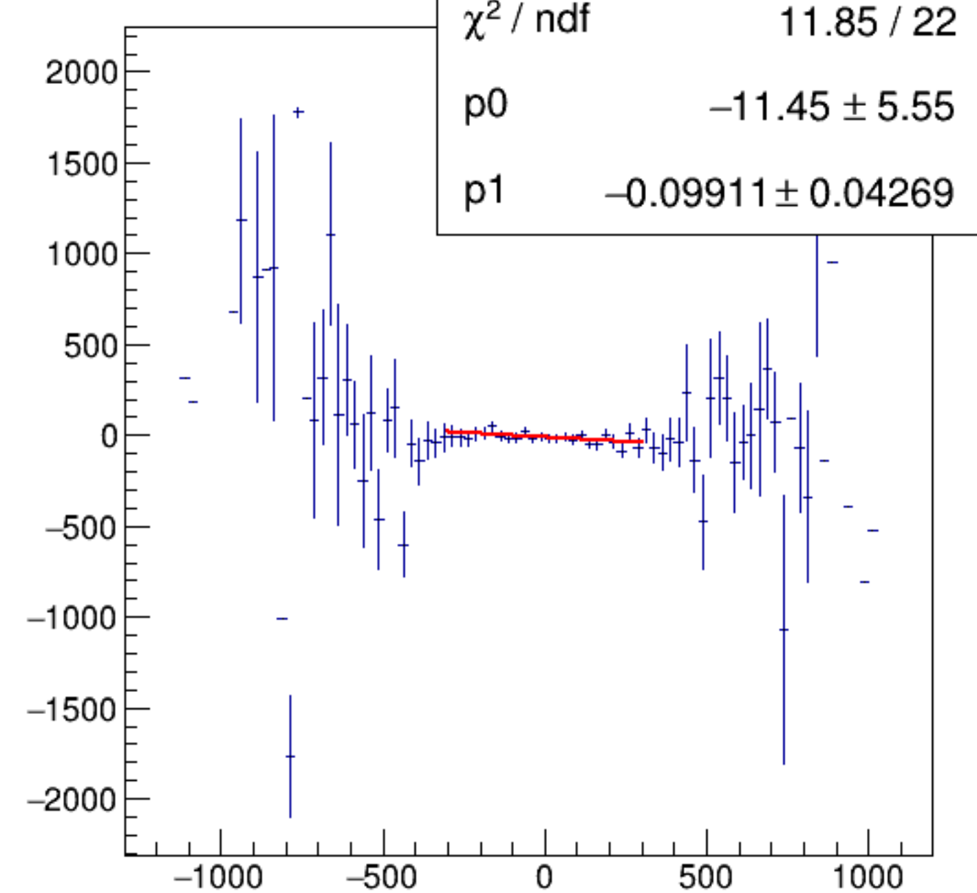
reg_asym_usr/ppm:AqDS/ppm {ok_cut}
