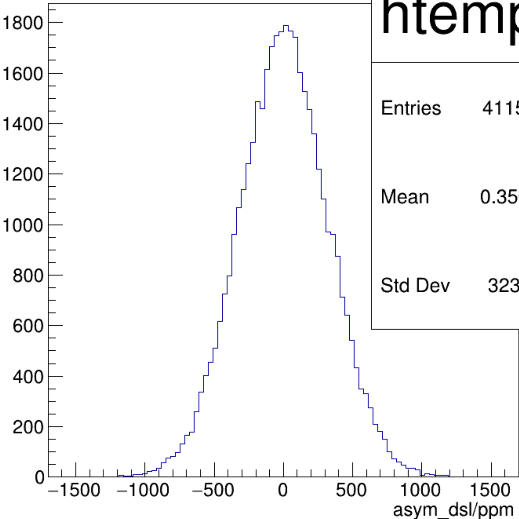
asym_dsl/ppm {ok_cut}
