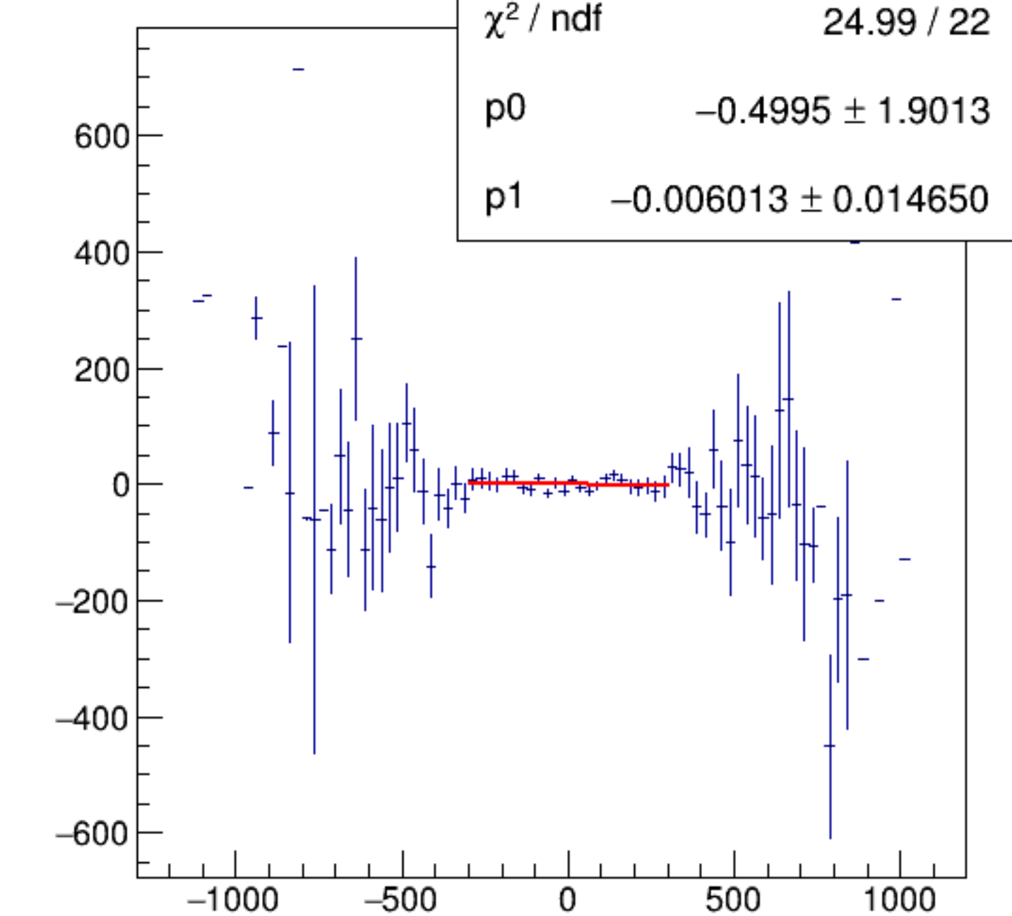
reg_asym_dsr/ppm:AqDS/ppm {ok_cut}
