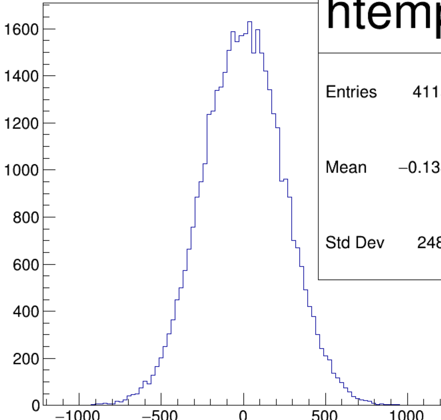
(asym_dsl/ppm+asym_dsr/ppm)/2 {ok_cut}
