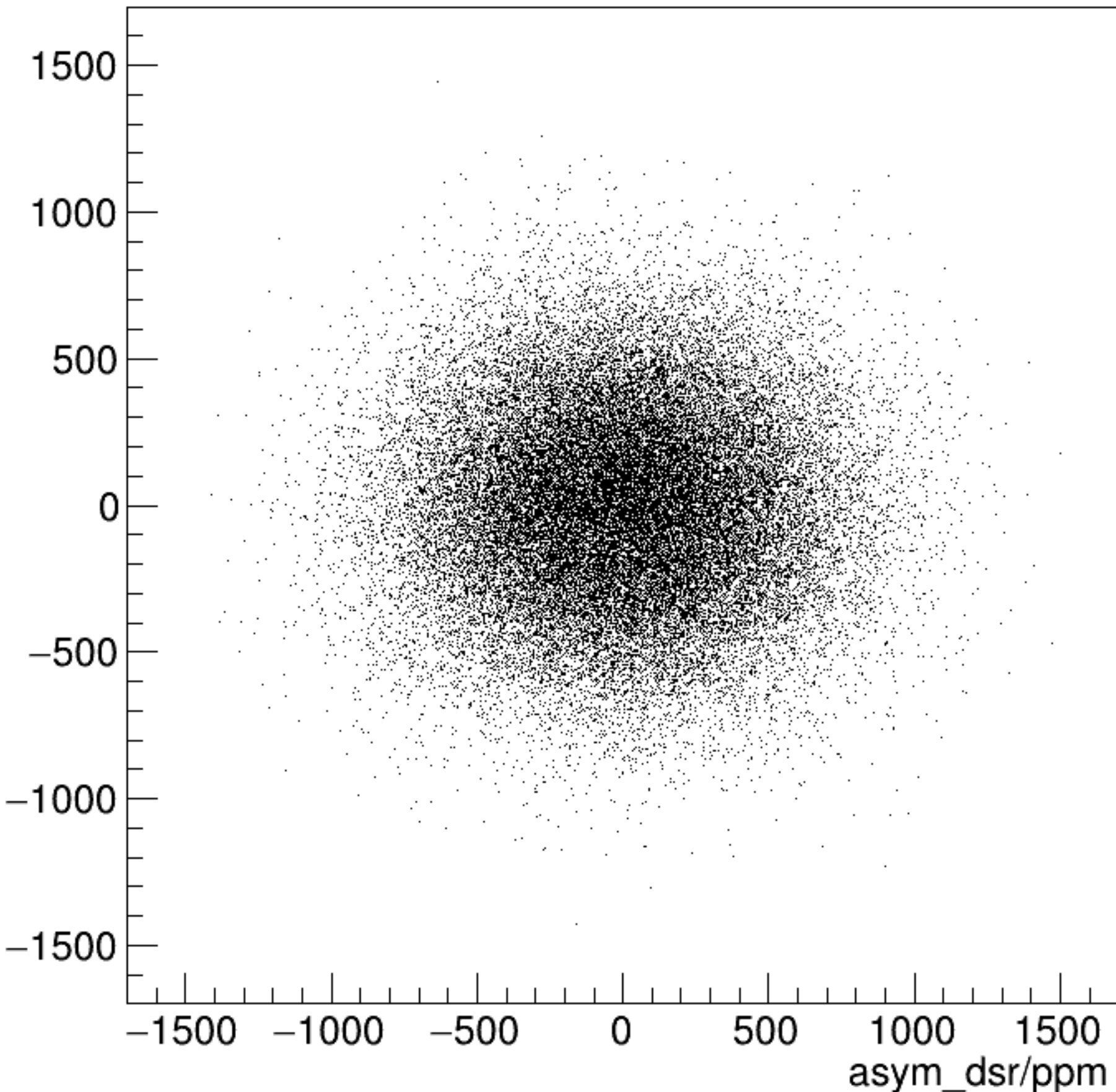
asym_dsl/ppm:asym_dsr/ppm {ok_cut}
