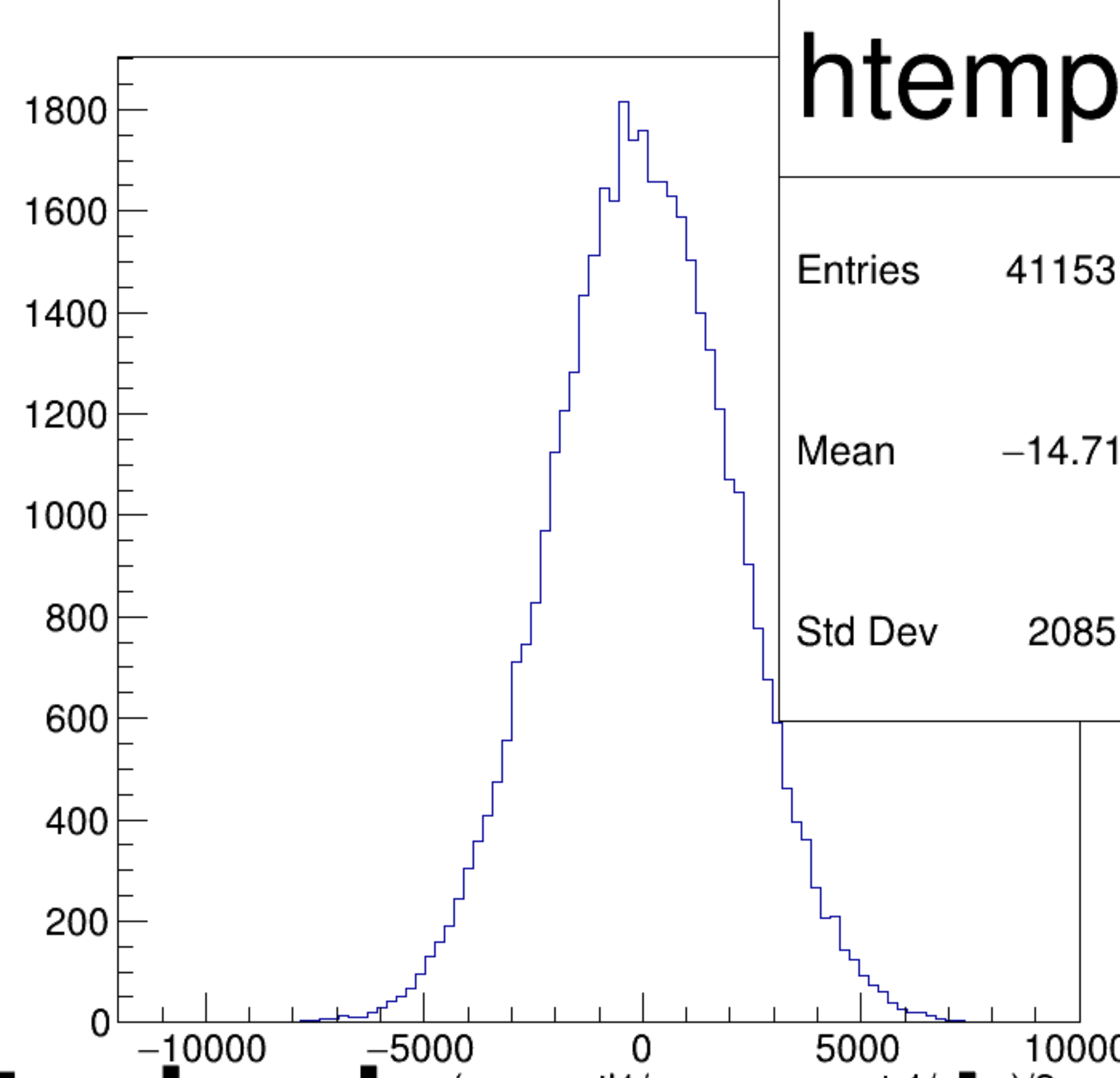
(asym_atl1/ppm+asym_atr1/ppm)/2 {ok_cut}
