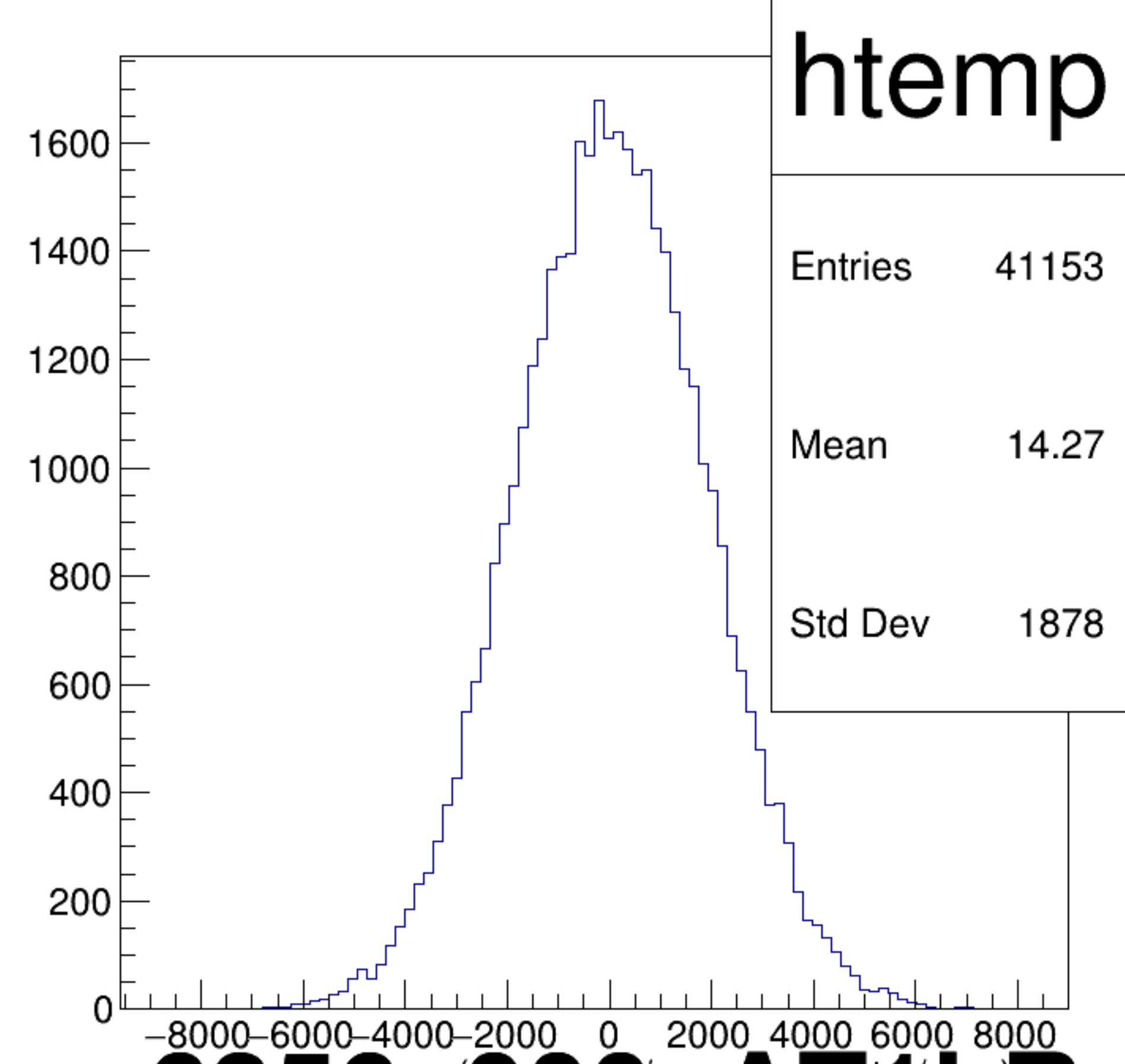
(asym_atl1/ppm-asym_atr1/ppm)/2 {ok_cut}
