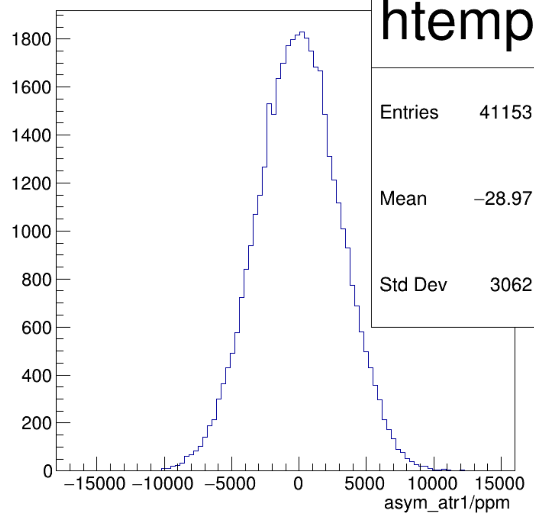
asym_atr1/ppm {ok_cut}
