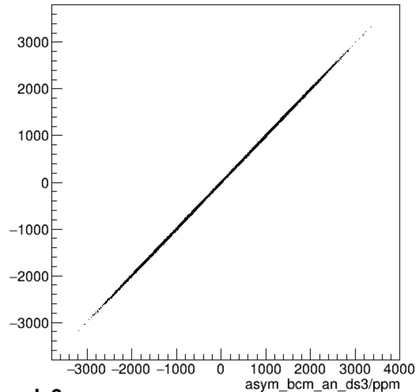
run6357_000_asym_bcm_an_ds_vs_asym_bcm_an_ds3_pr.png
