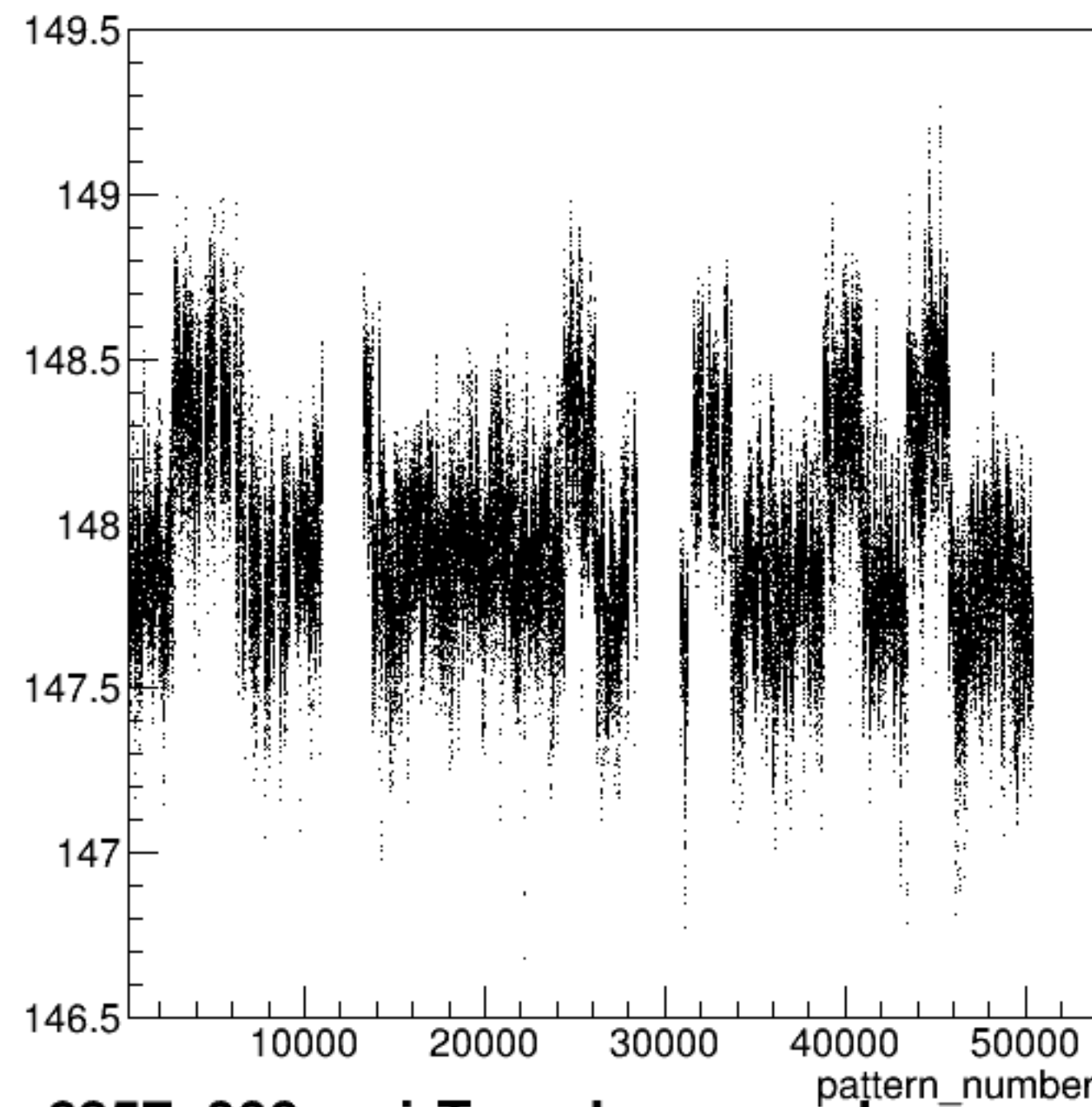
yield_bcm_an_ds:pattern_number {ErrorFlag==0}
