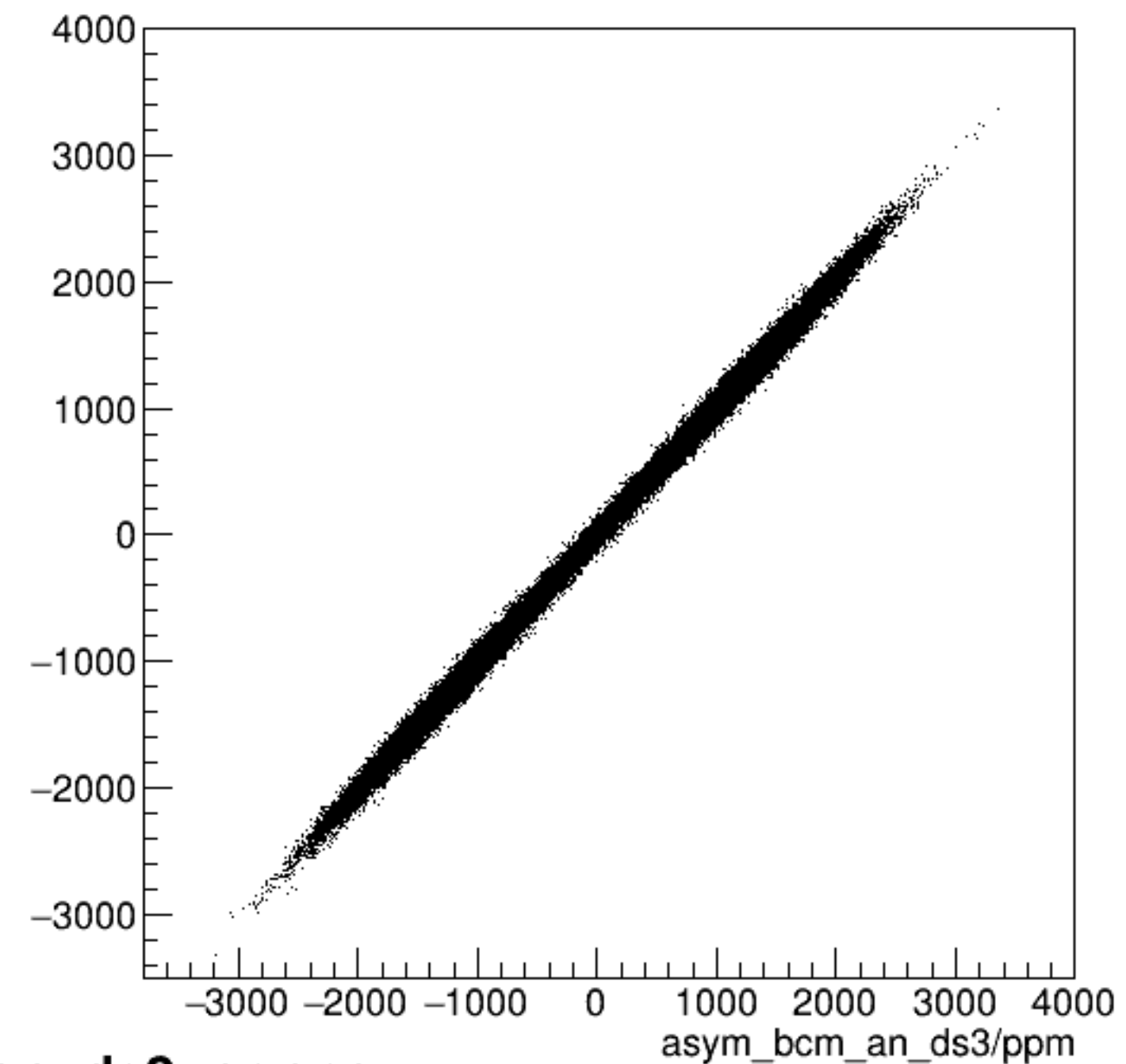
run6357_000_asym_bcm_dg_us_vs_asym_bcm_an_ds3_pr.png
