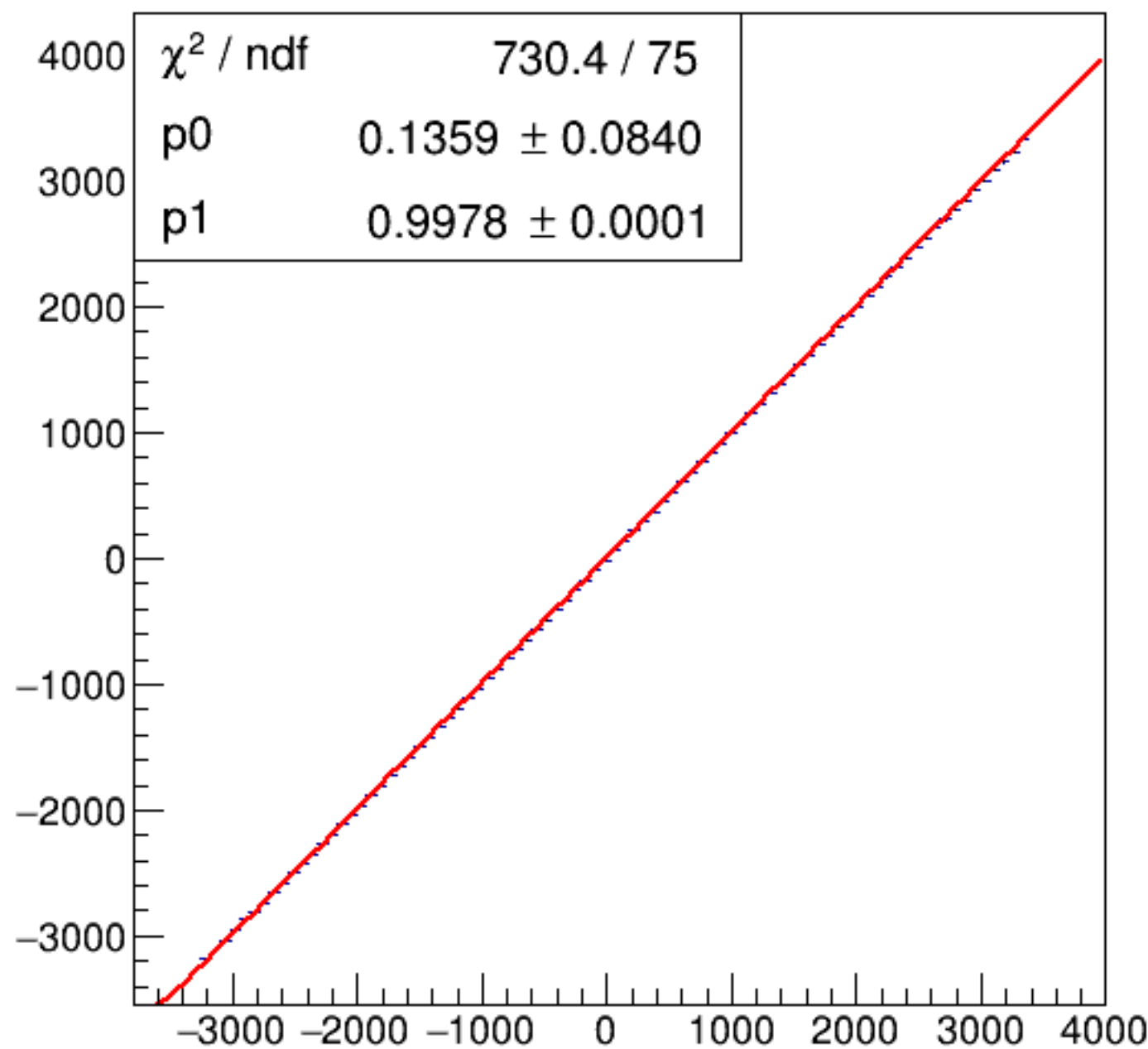
run6357_000_asym_bcm_an_ds_vs_asym_bcm_an_ds3_pr.png
