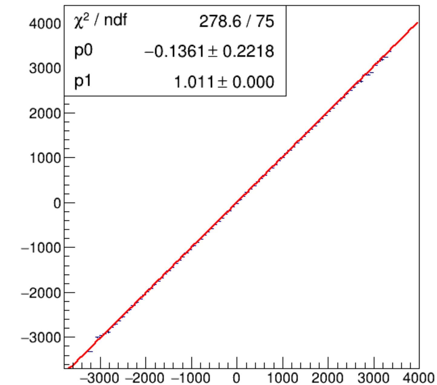
run6357_000_asym_bcm_dg_us_vs_asym_bcm_an_ds3_pr.png
