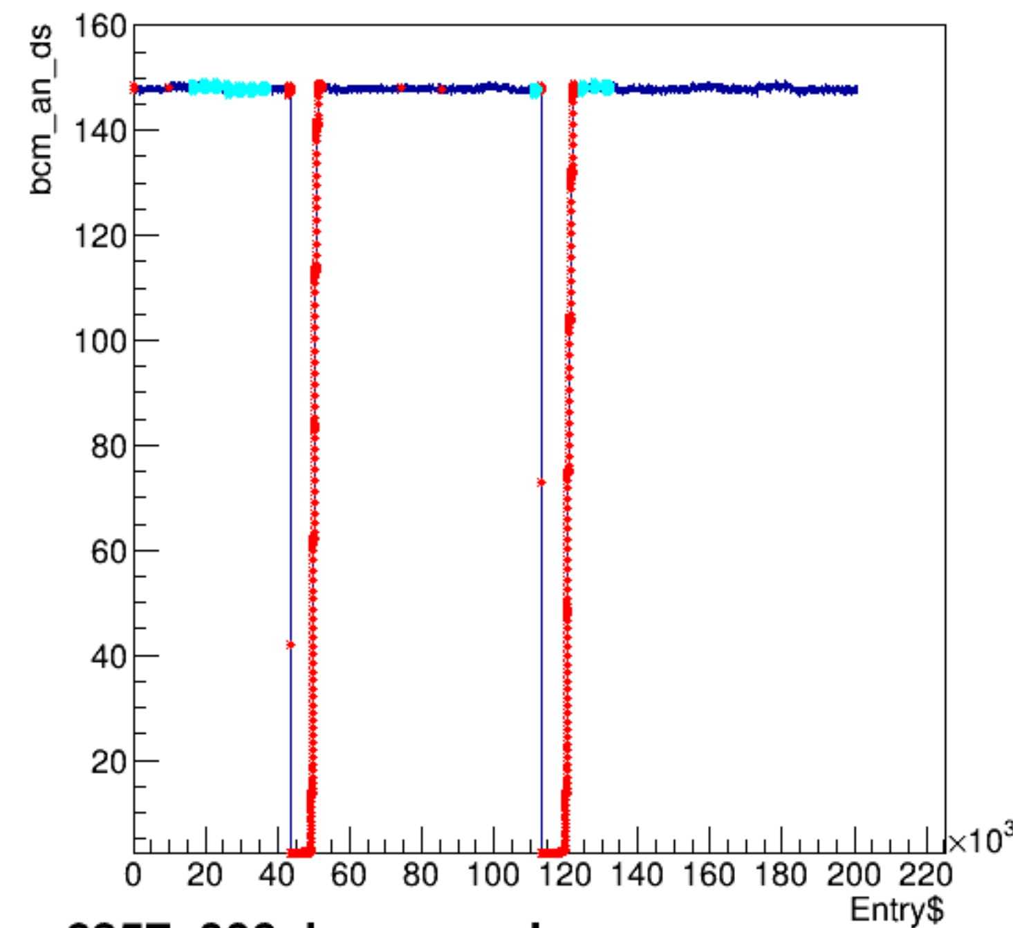
bcm_an_ds:Entry$
