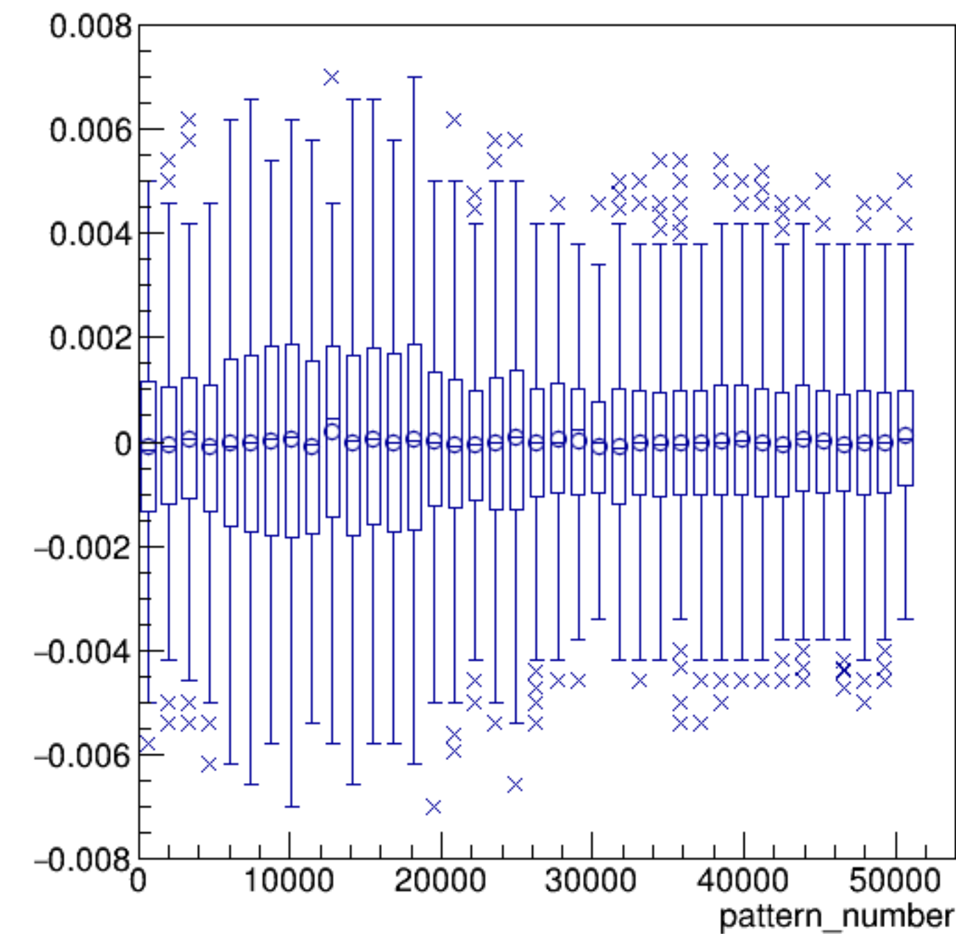
asym_bcm_an_diff*yield_bcm_an_diff:pattern_number {ErrorFlag==0}
