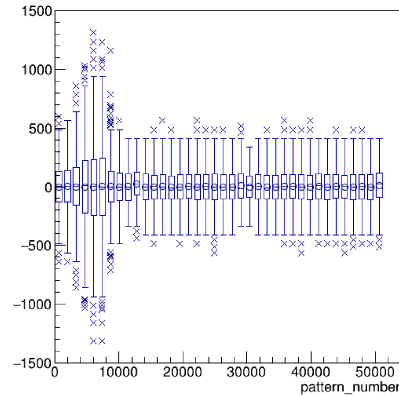
asym_bcm_dg_ds/ppm:pattern_number {ErrorFlag==0}
