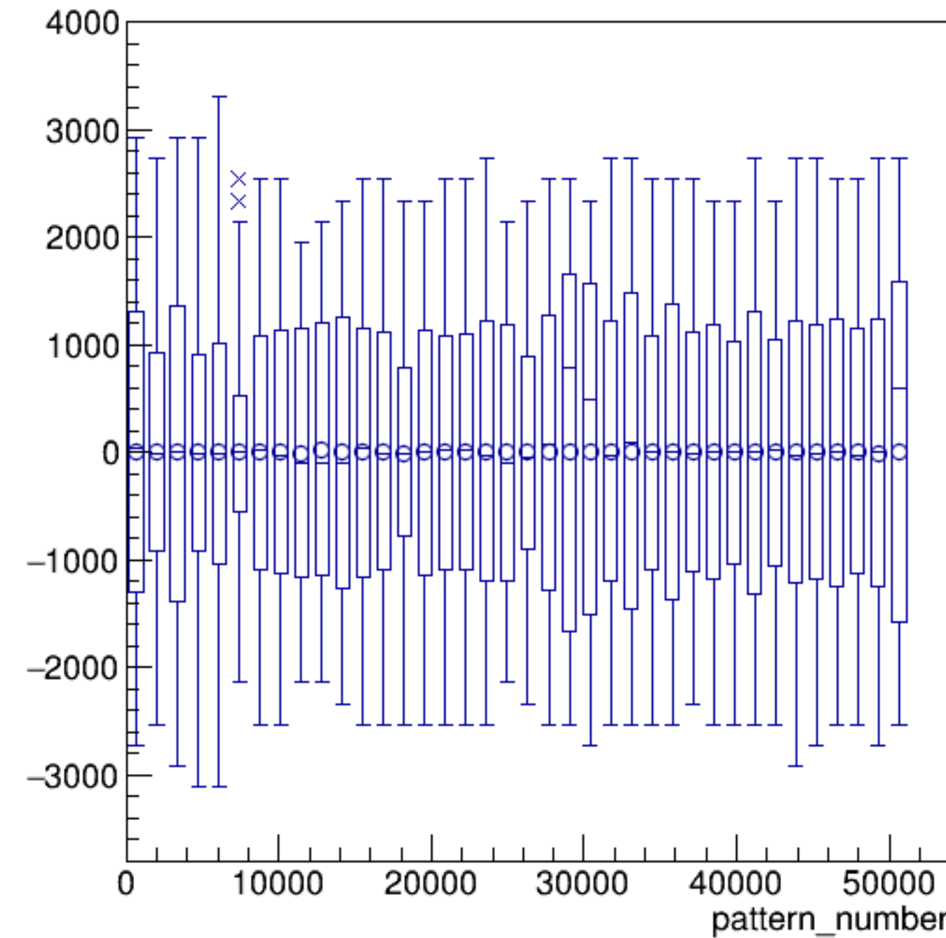
asym_bcm_an_ds3/ppm:pattern_number {ErrorFlag==0}
