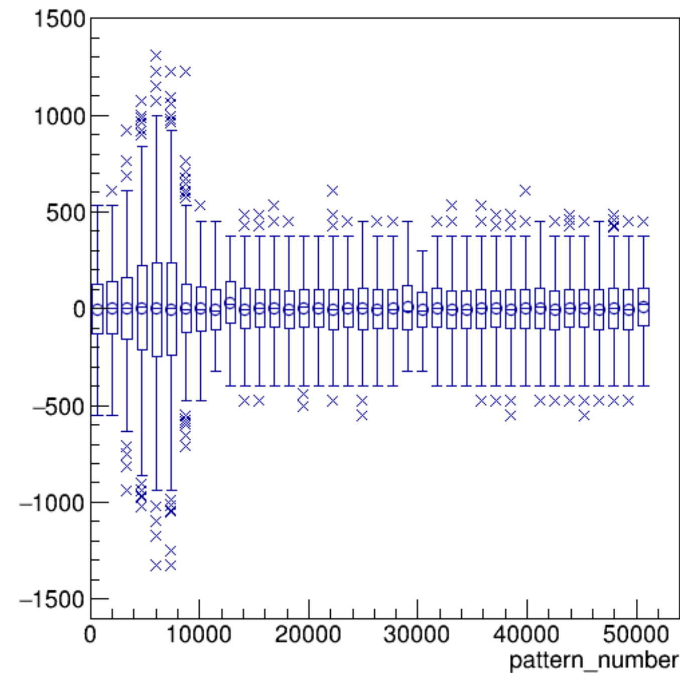
asym_bcm_an_us/ppm:pattern_number {ErrorFlag==0}
