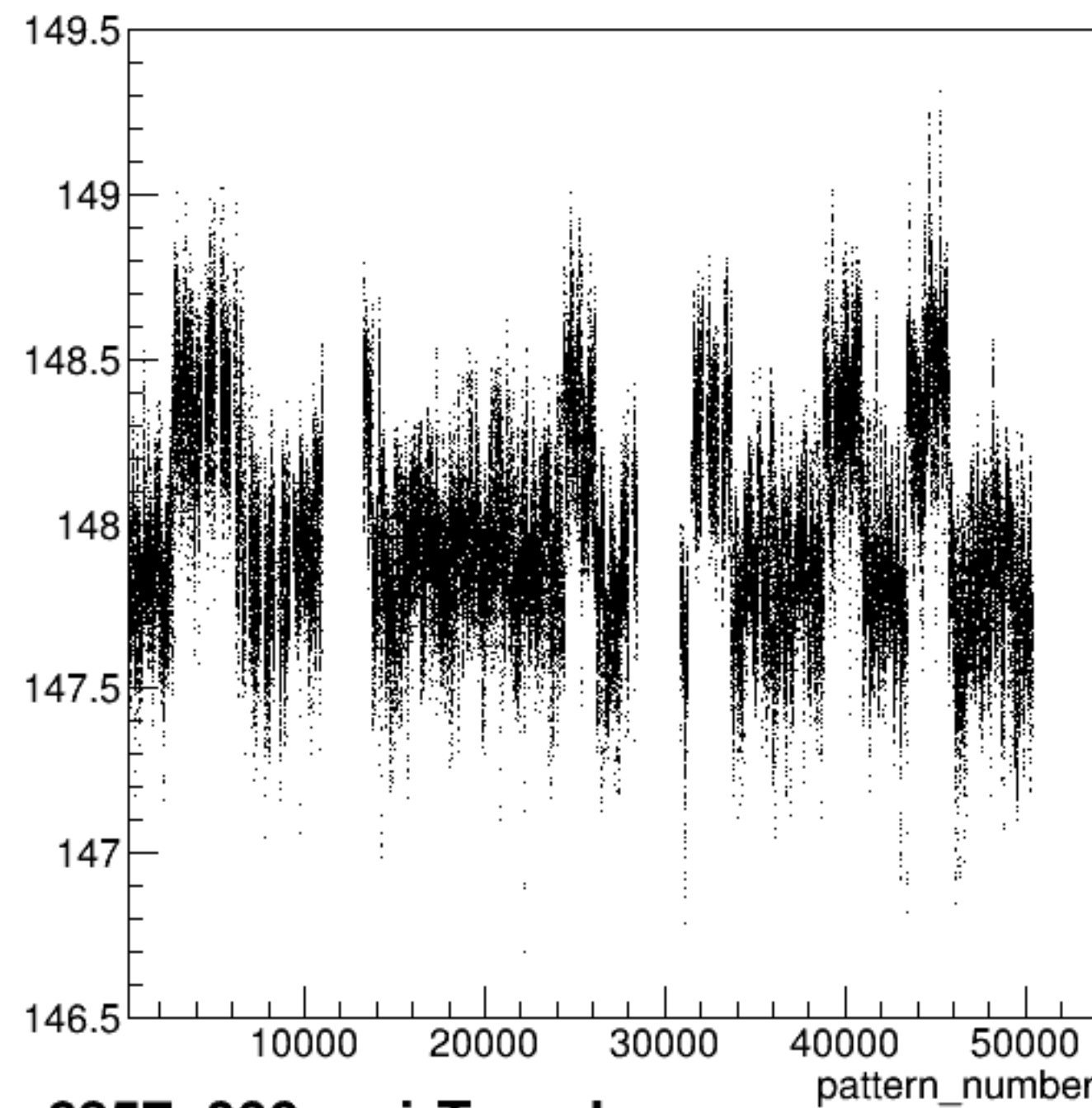
yield_bcm_an_us:pattern_number {ErrorFlag==0}
