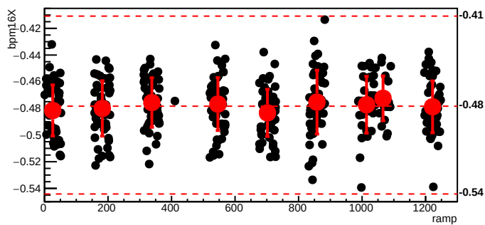
bmod_trim4,cyc=6050
