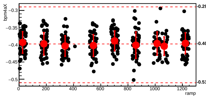
bmod_trim4,cyc=6050
