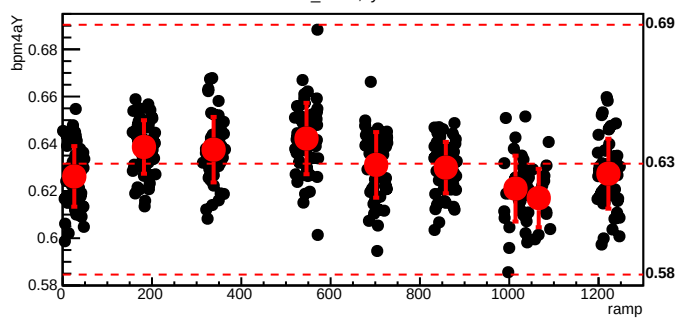
bmod_trim3,cyc=6050
