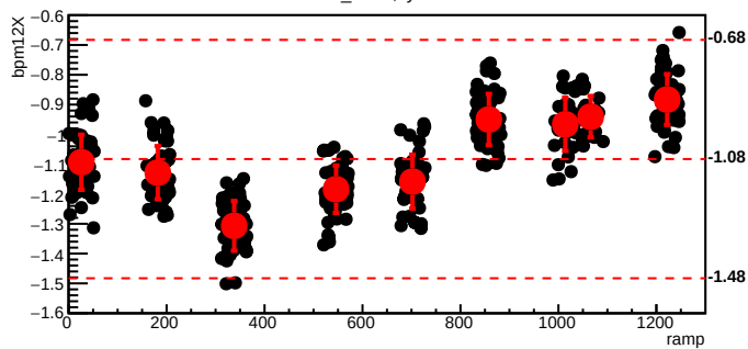
bmod_trim3,cyc=6050
