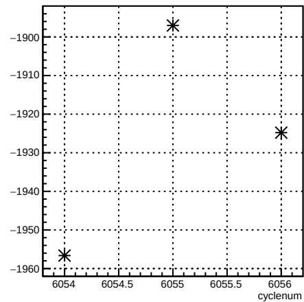
usr_coil6:cyclenum {run == 6361}
