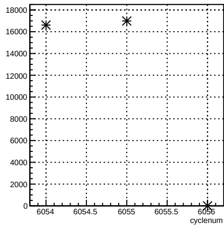
usr_coil7:cyclenum {run == 6361}
