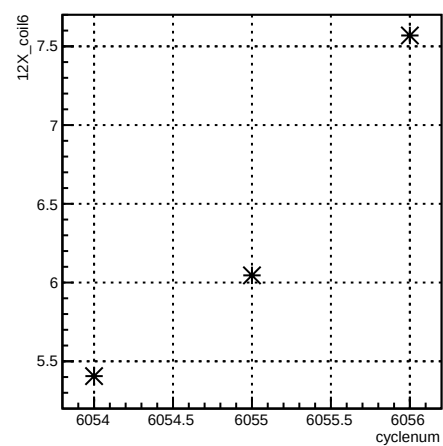
12X_coil6:cyclenum {run == 6361}
