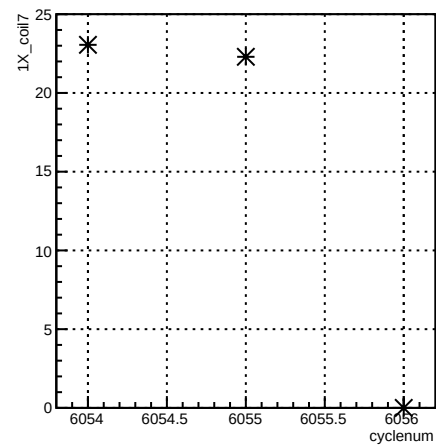
1X_coil7:cyclenum {run == 6361}
