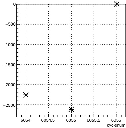
usr_coil3:cyclenum {run == 6361}
