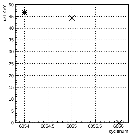
usl_4eY:cyclenum {run == 6361}
