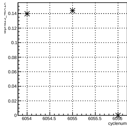
alpha13_4eX1X:cyclenum {run == 6361}
