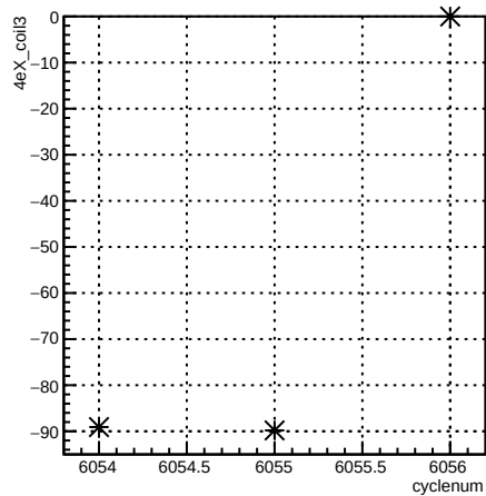
4eX_coil3:cyclenum {run == 6361}
