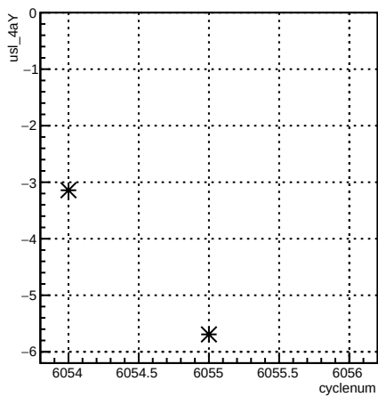
usl_4aY:cyclenum {run == 6361}
