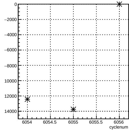
usr_coil1:cyclenum {run == 6361}
