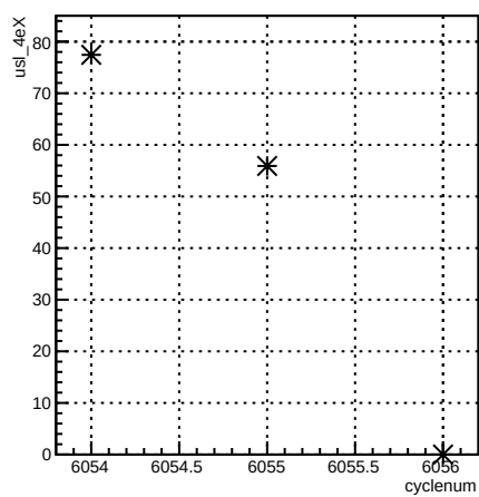
usl_4eX:cyclenum {run == 6361}
