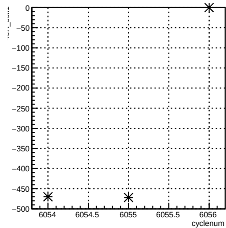
4eX_coil1:cyclenum {run == 6361}
