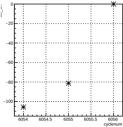
usl_1X:cyclenum {run == 6361}
