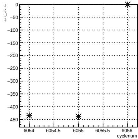
1X_coil1:cyclenum {run == 6361}
