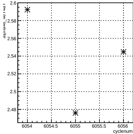
alpha46_4eY4aY:cyclenum {run == 6361}
