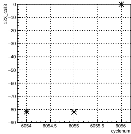
12X_coil3:cyclenum {run == 6361}
