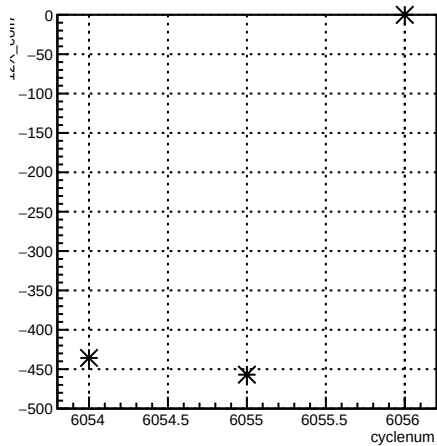
12X_coil7:cyclenum {run == 6361}
