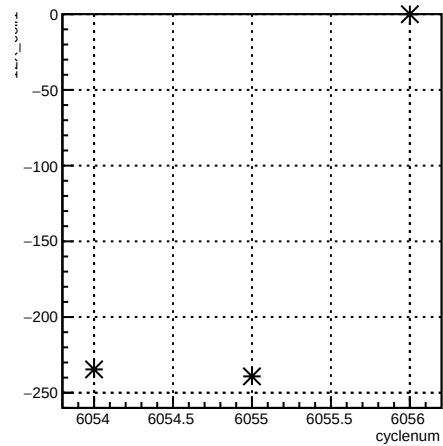
12X_coil1:cyclenum {run == 6361}
