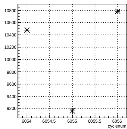
usr_coil4:cyclenum {run == 6361}
