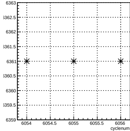
run:cyclenum {run == 6361}
