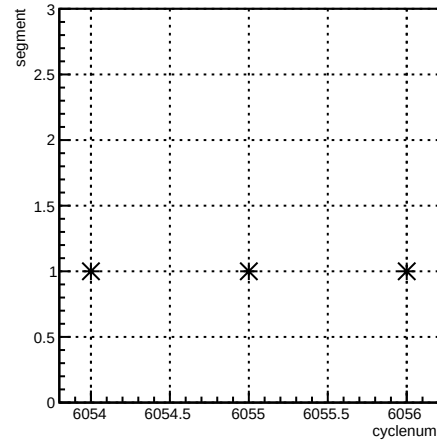
segment:cyclenum {run == 6361}
