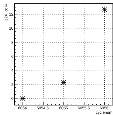
12X_coil4:cyclenum {run == 6361}
