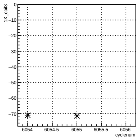
1X_coil3:cyclenum {run == 6361}
