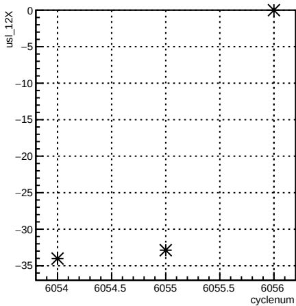
usl_12X:cyclenum {run == 6361}
