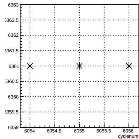
run:cyclenum {run == 6361}
