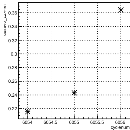
delta46_12X4eY:cyclenum {run == 6361}
