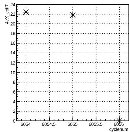
4eX_coil7:cyclenum {run == 6361}
