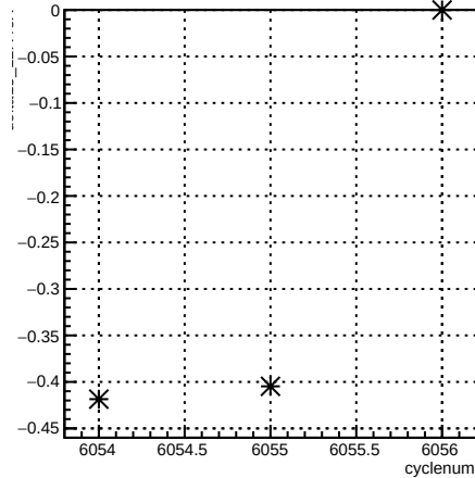
delta13_12X4eX:cyclenum {run == 6361}
