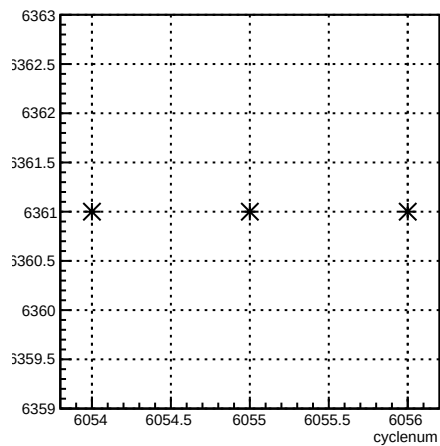
run:cyclenum {run == 6361}
