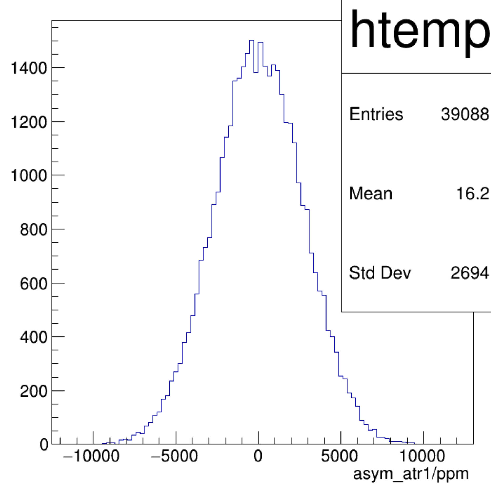
asym_atr1/ppm {ok_cut}
