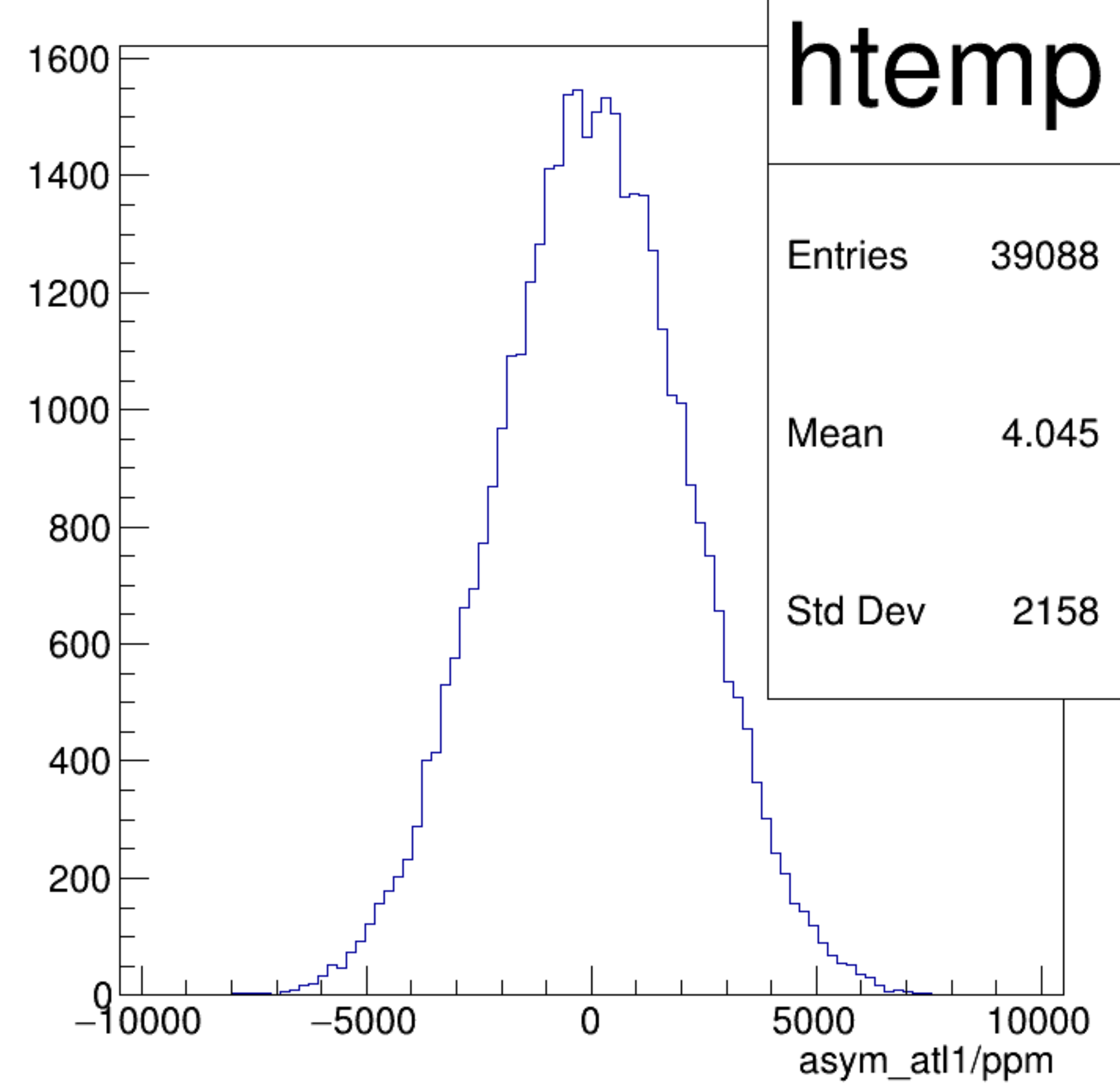
asym_atl1/ppm {ok_cut}
