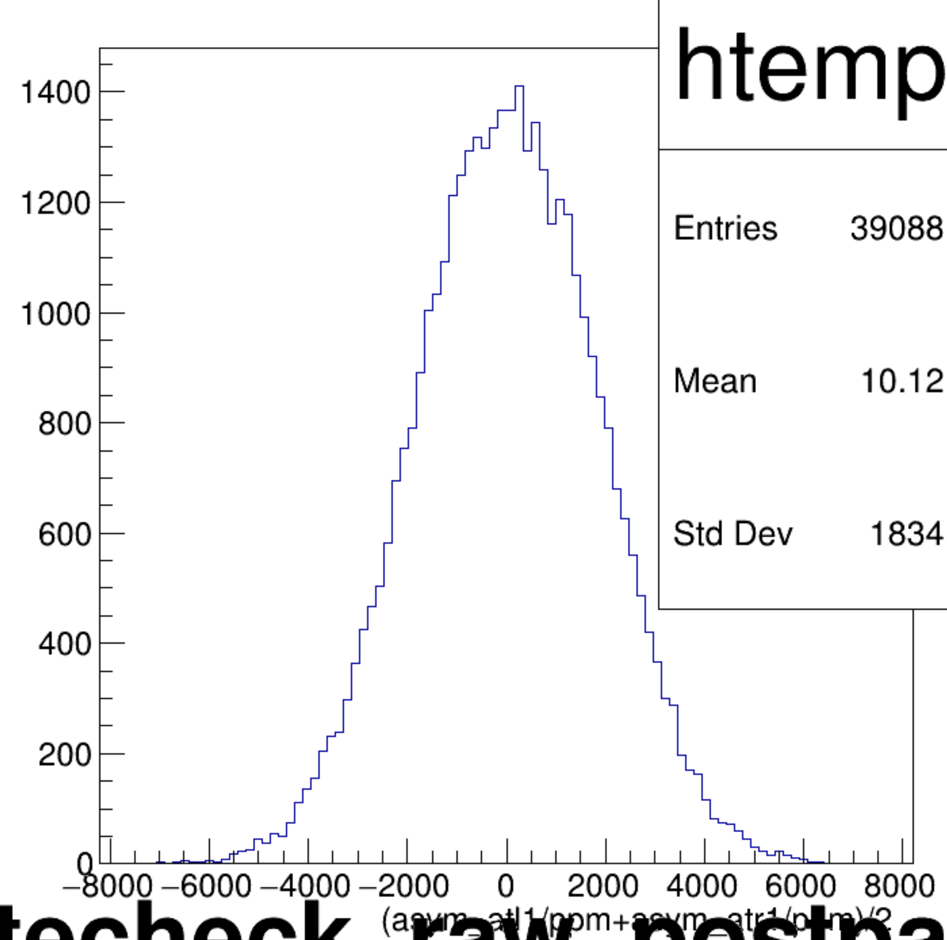
(asym_atl1/ppm+asym_atr1/ppm)/2 {ok_cut}
