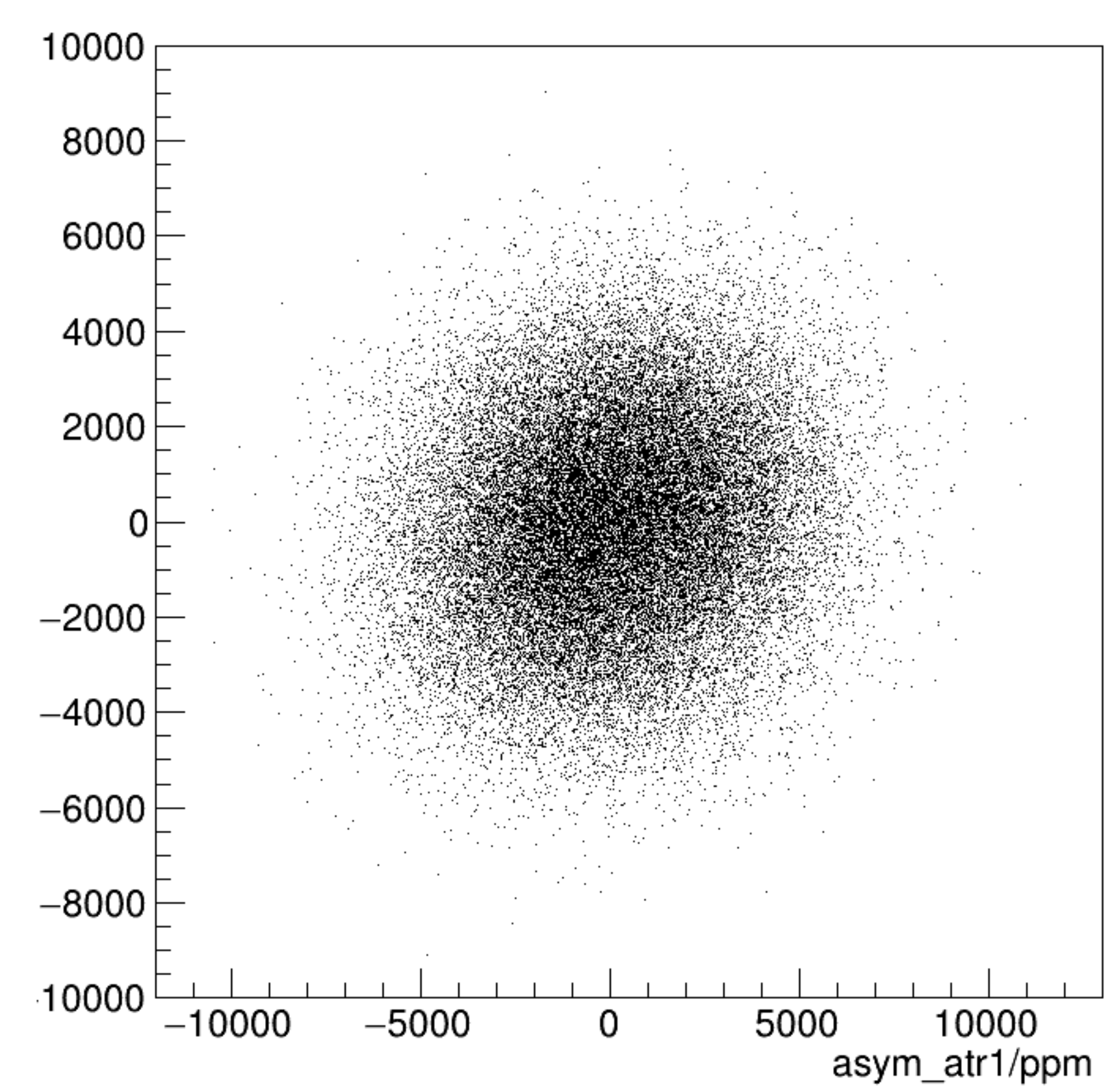
asym_atl1/ppm:asym_atr1/ppm {ok_cut}
