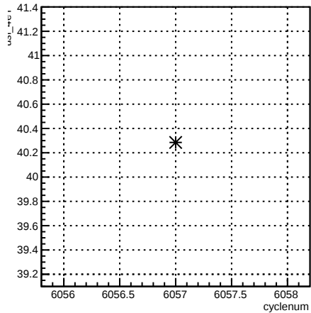
usl_4eY:cyclenum {run == 6362}
