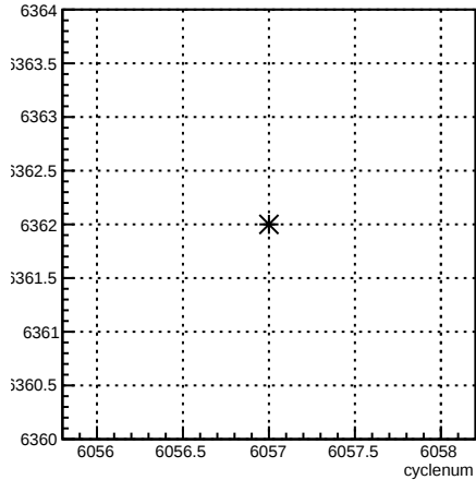
run:cyclenum {run == 6362}
