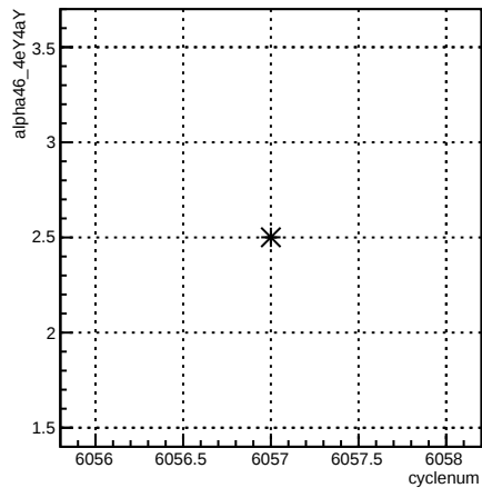
alpha46_4eY4aY:cyclenum {run == 6362}
