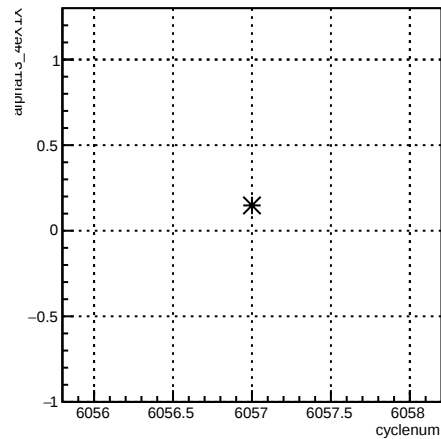
alpha13_4eX1X:cyclenum {run == 6362}
