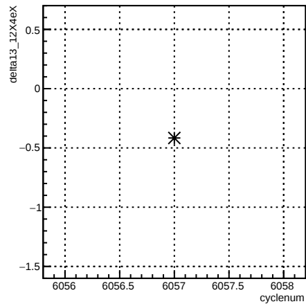
delta13_12X4eX:cyclenum {run == 6362}
