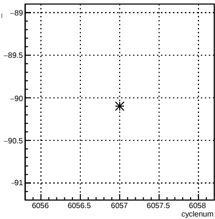
usl_4eY:cyclenum {run == 6362}
