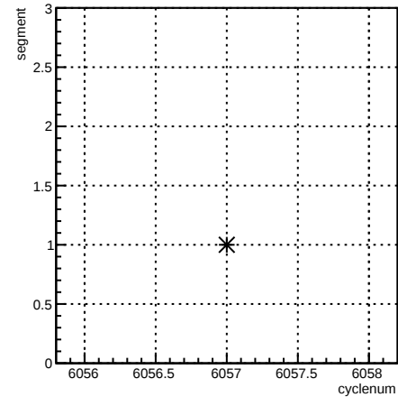
segment:cyclenum {run == 6362}
