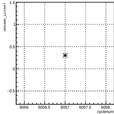
delta46_12X4eY:cyclenum {run == 6362}
