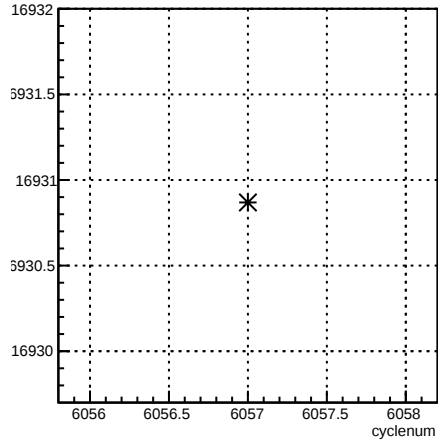
usr_coil7:cyclenum {run == 6362}
