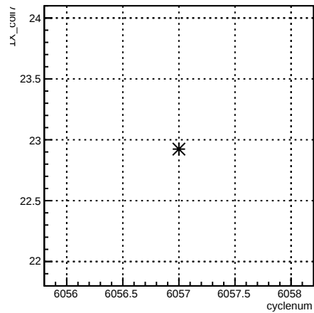
4eX_coil7:cyclenum {run == 6362}
