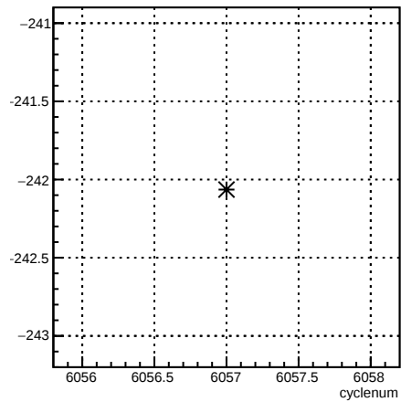
12X_coil6:cyclenum {run == 6362}
