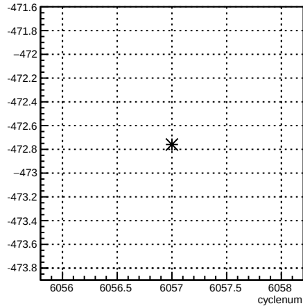
4eX_coil1:cyclenum {run == 6362}
