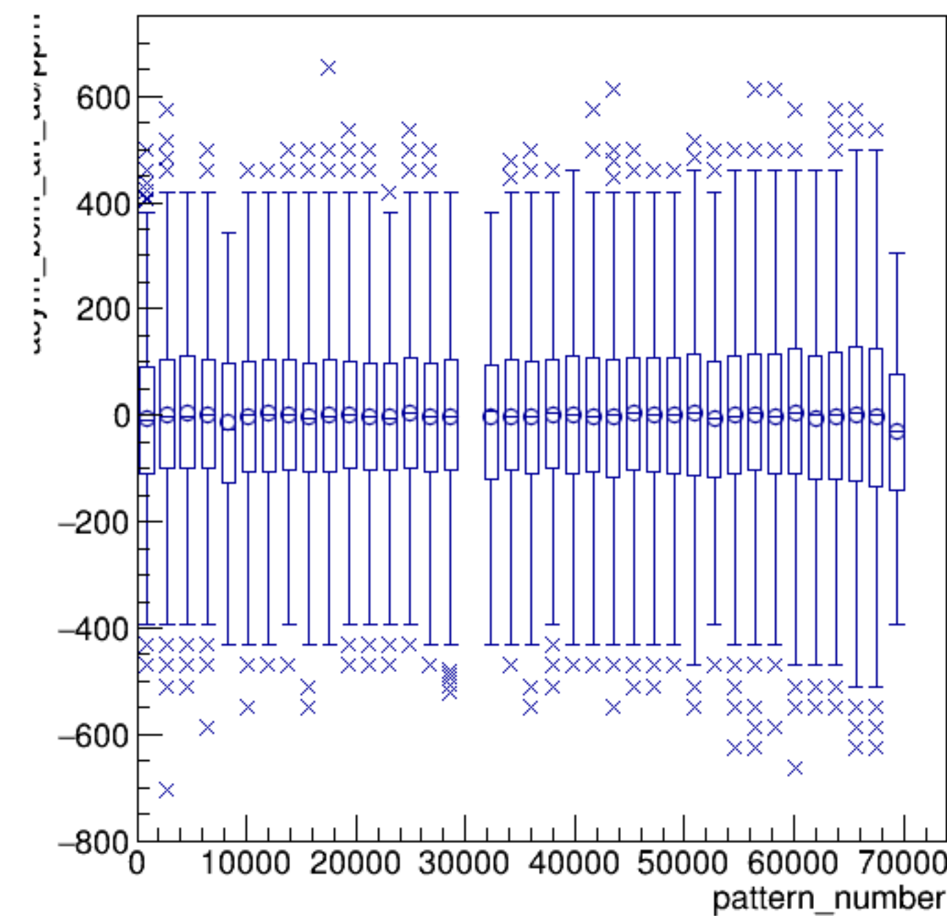
asym_bcm_an_us/ppm:pattern_number {ErrorFlag==0}
