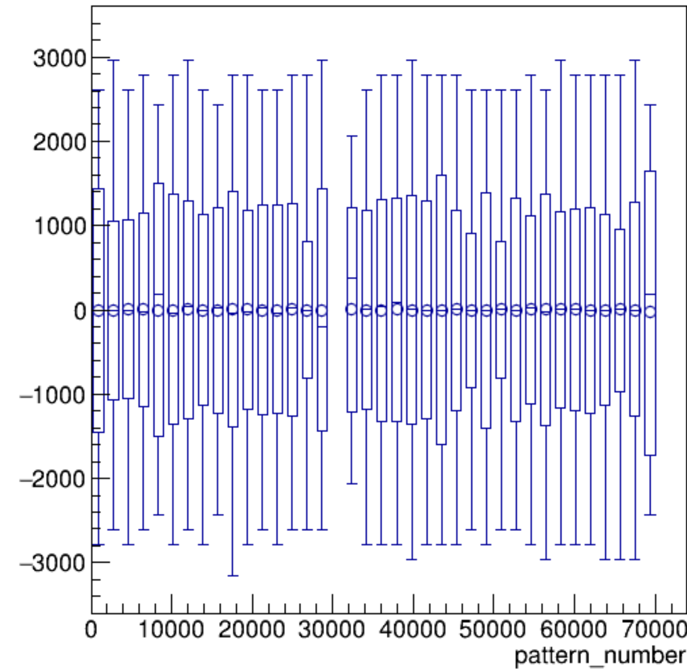
asym_bcm_an_us/ppm:pattern_number {ErrorFlag==0}
