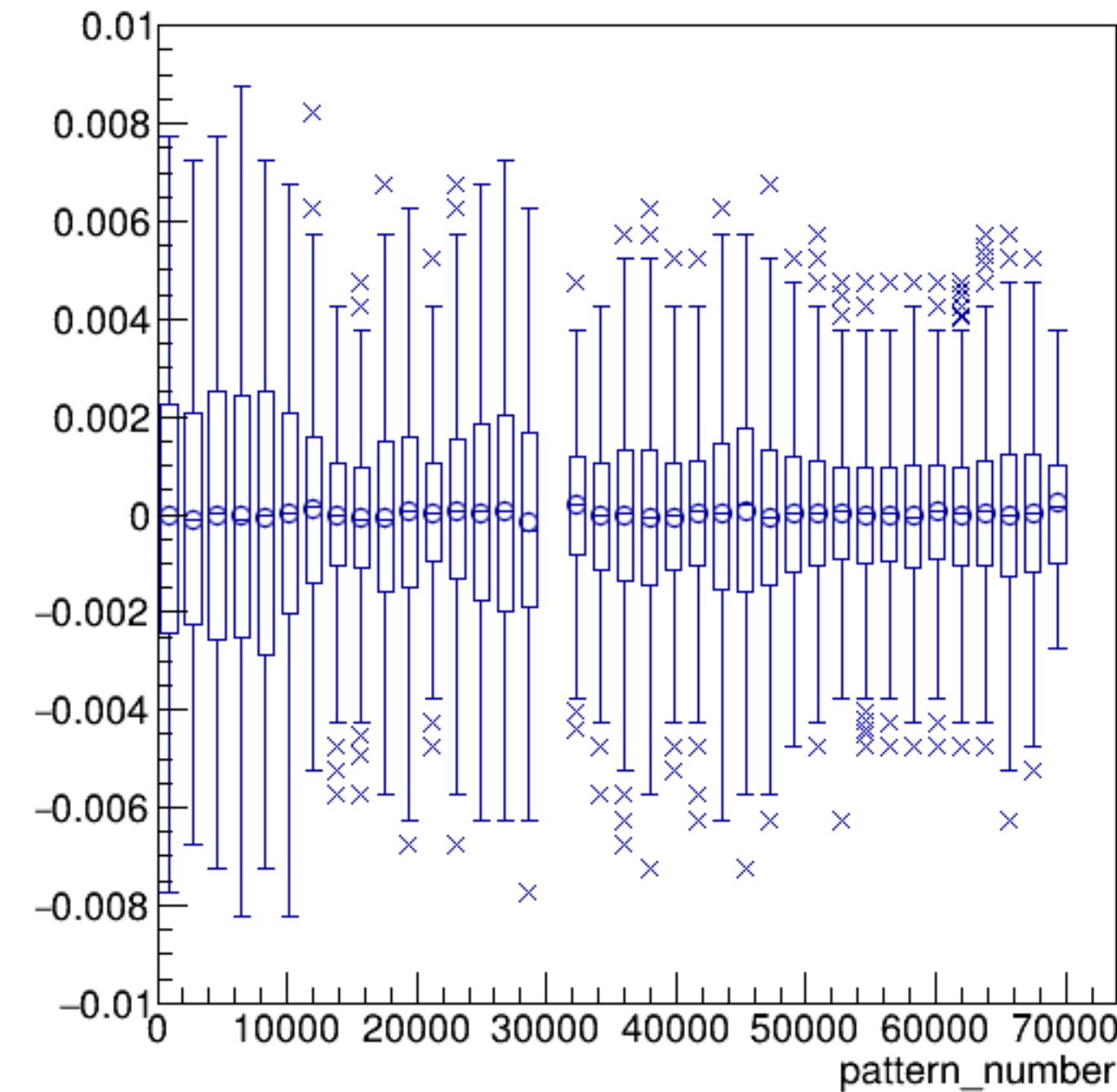
asym_bcm_an_diff*yield_bcm_an_diff:pattern_number {ErrorFlag==0}
