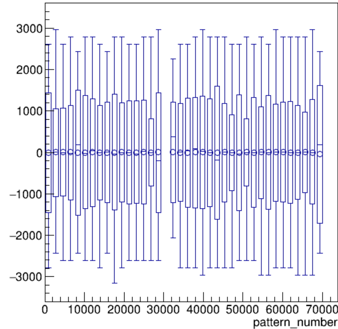
asym_bcm_an_ds/ppm:pattern_number {ErrorFlag==0}
