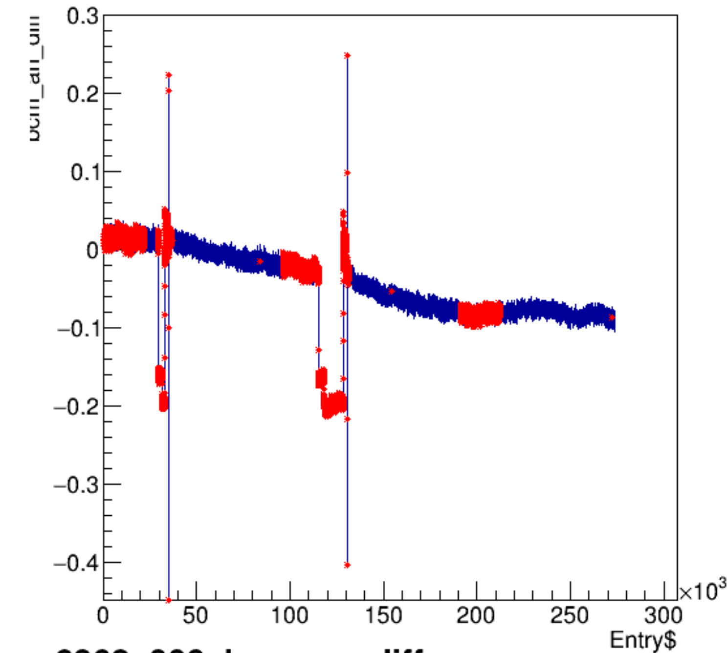
bcm_an_diff:Entry$
