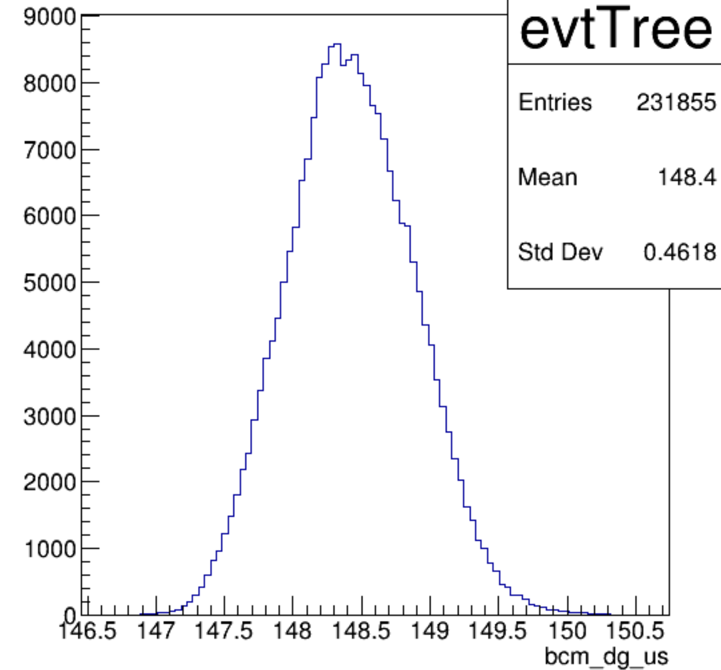
bcm_dg_us {ErrorFlag==0}
