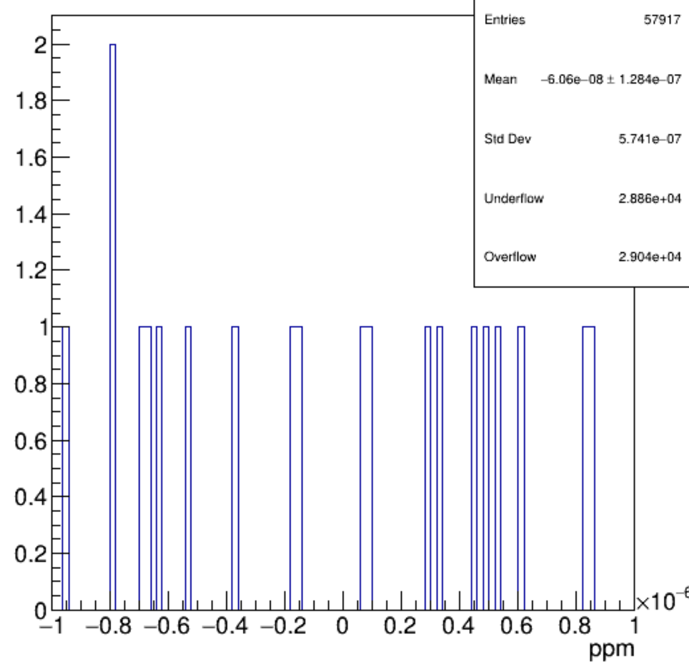
asym_bcm_an_diff
