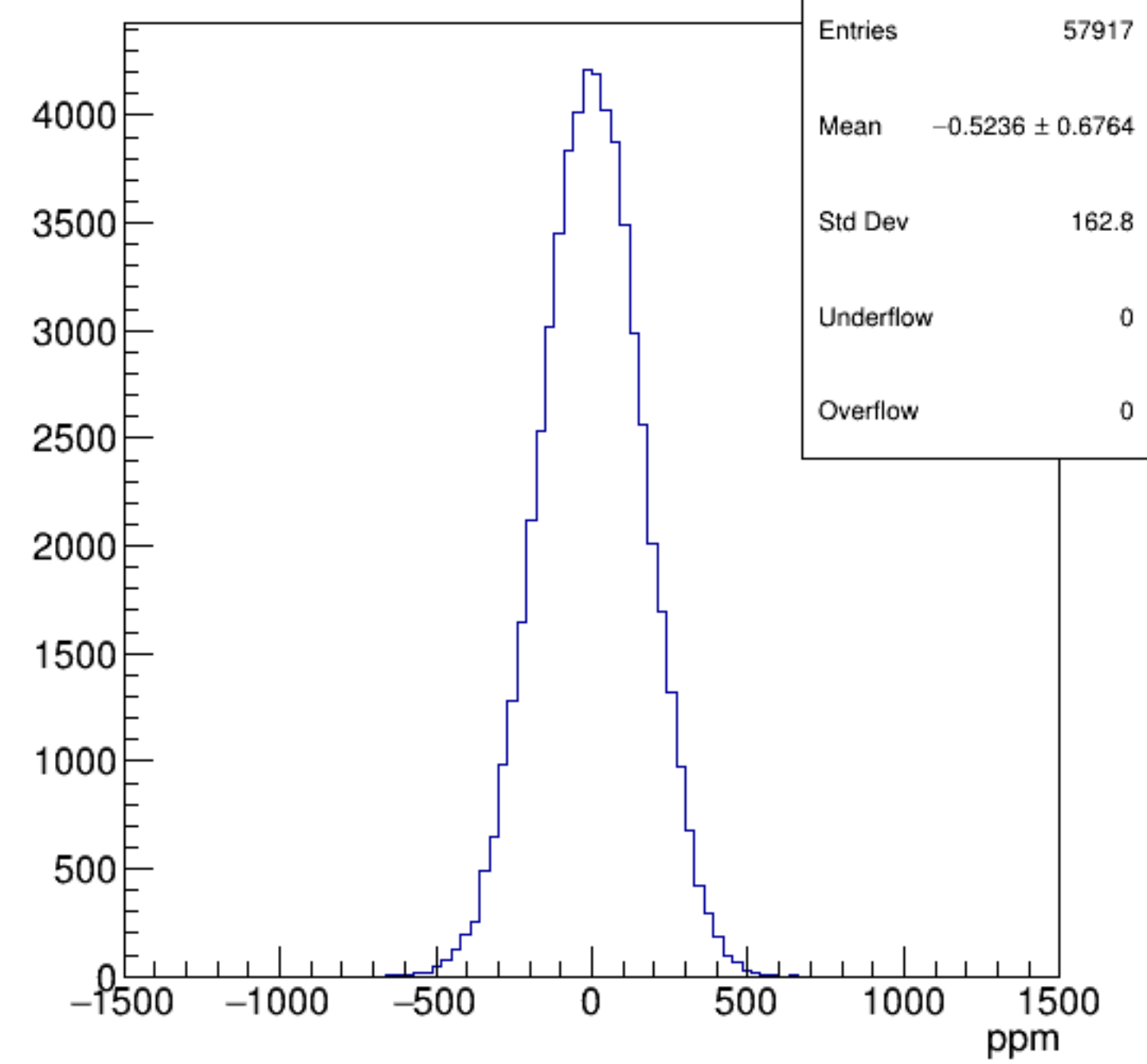
asym_bcm_dg_us
