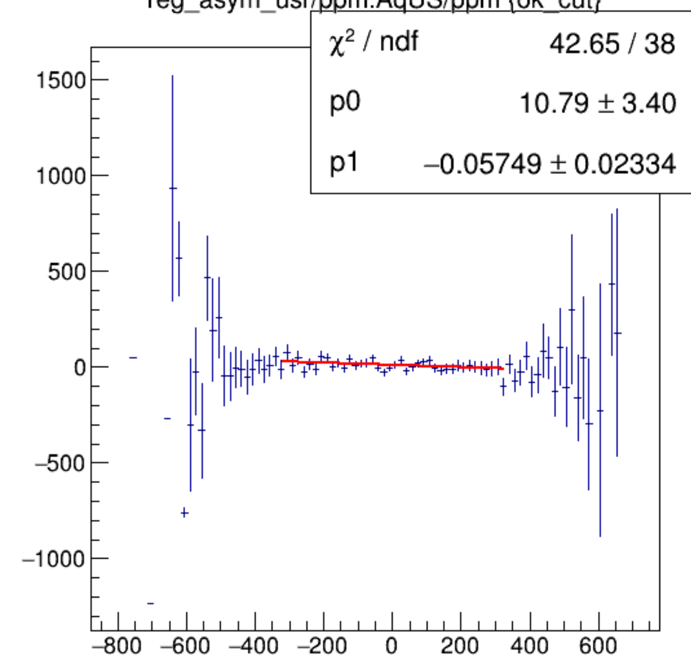
reg_asym_usr/ppm:AqUS/ppm {ok_cut}
