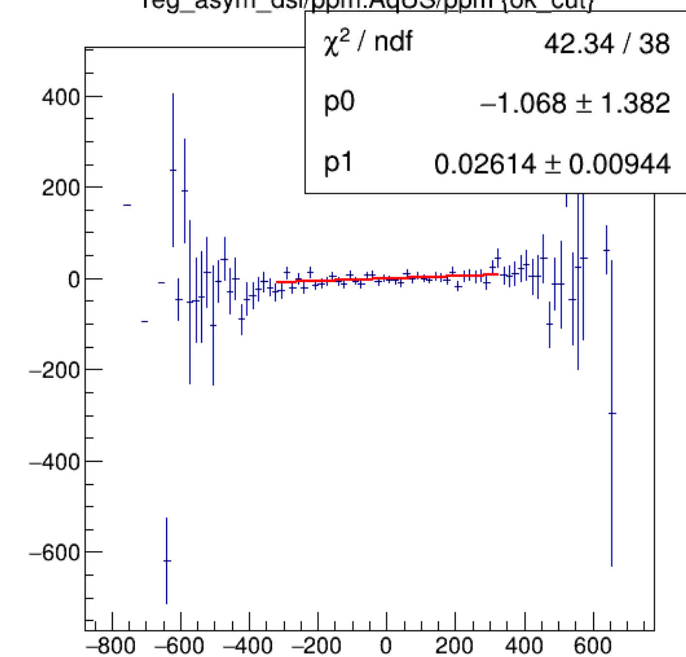
reg_asym_dsl/ppm:AqUS/ppm {ok_cut}
