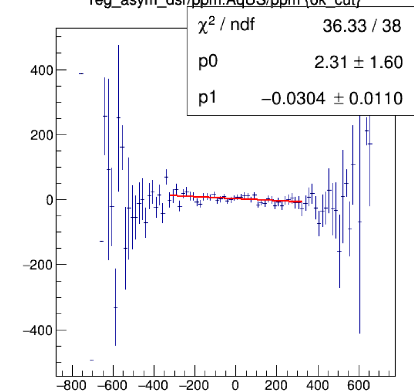
reg_asym_dsr/ppm:AqUS/ppm {ok_cut}
