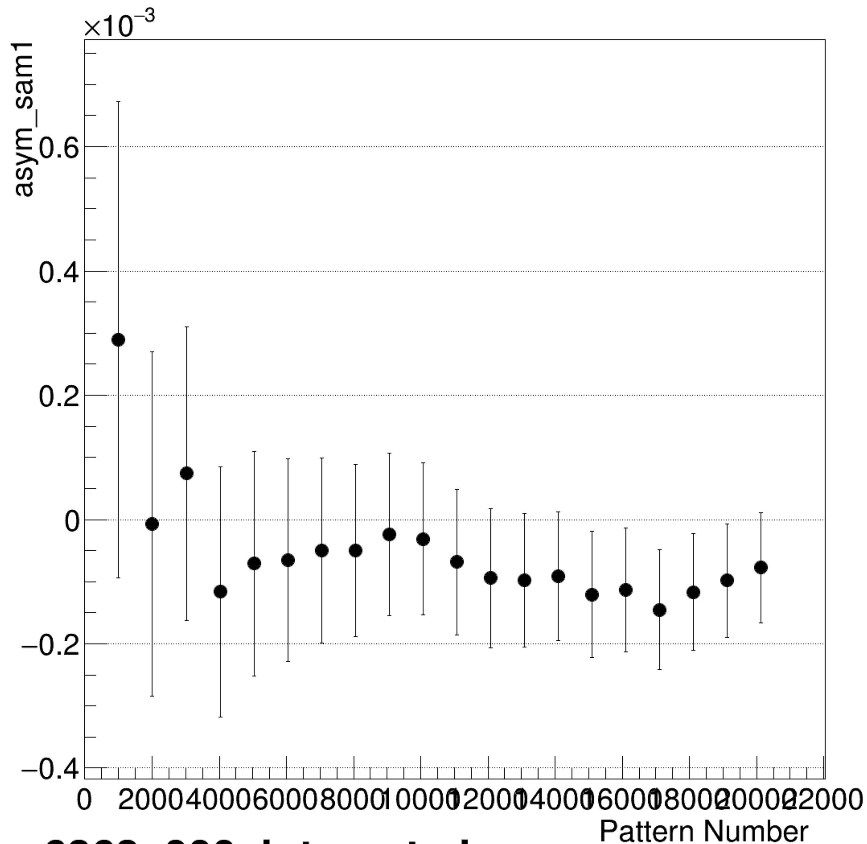
asym_sam1 Integrated Convergence
