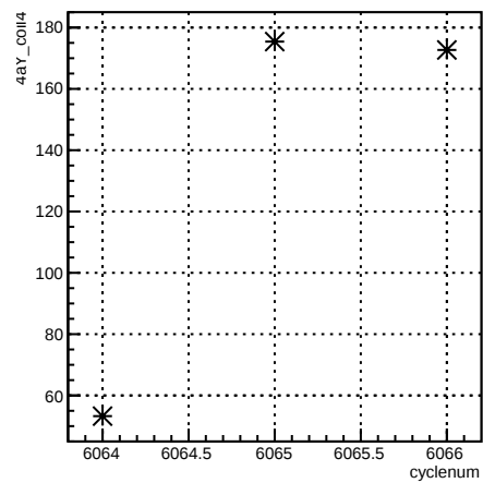
4aY_coil4:cyclenum {run == 6369}
