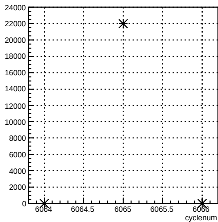
usr_coil7:cyclenum {run == 6369}
