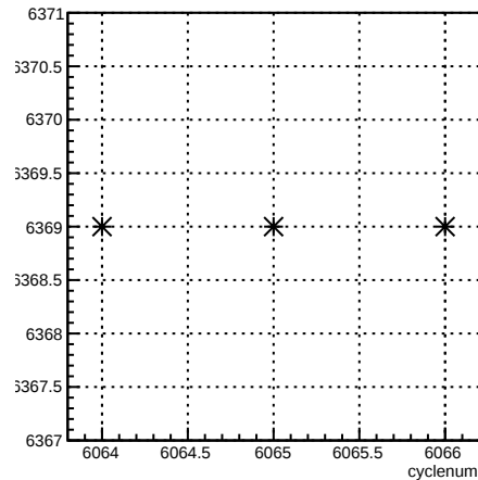
run:cyclenum {run == 6369}
