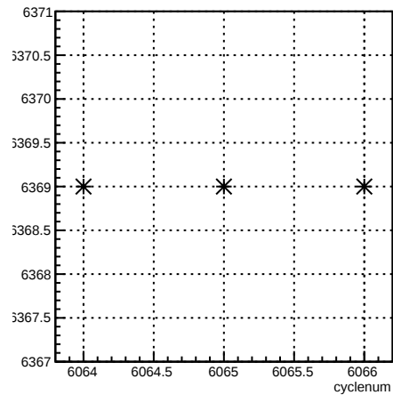
run:cyclenum {run == 6369}
