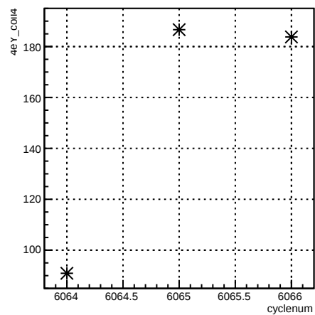
4eY_coil4:cyclenum {run == 6369}
