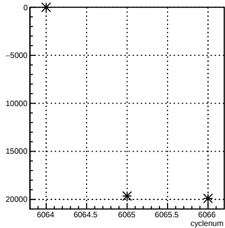
usr_coil1:cyclenum {run == 6369}
