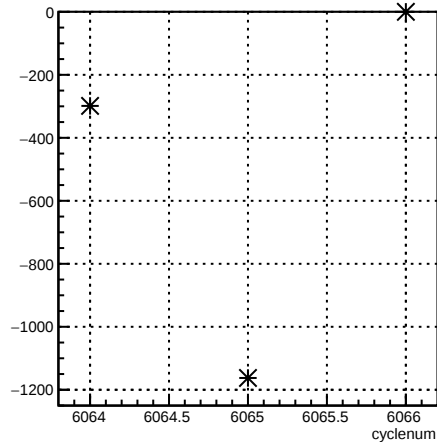
usl_coil6:cyclenum {run == 6369}
