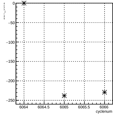
12X_coil1:cyclenum {run == 6369}
