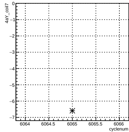
4aY_coil7:cyclenum {run == 6369}
