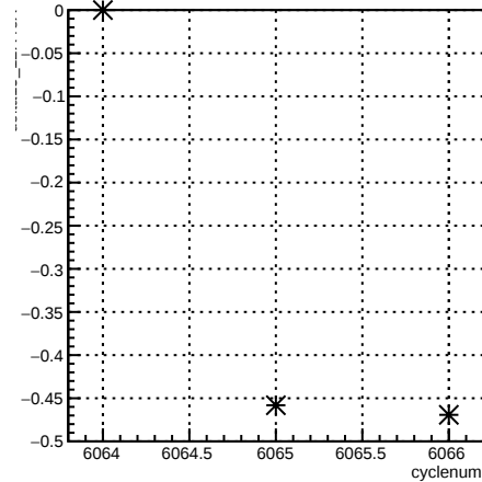
delta13_12X4eX:cyclenum {run == 6369}
