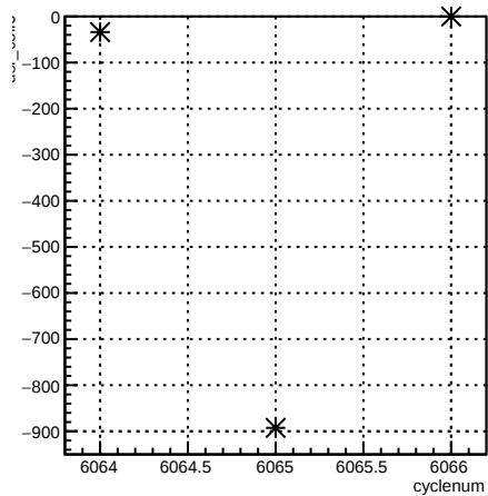
usr_coil6:cyclenum {run == 6369}
