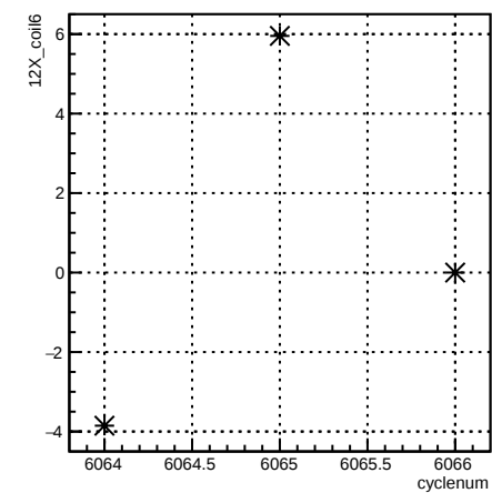
12X_coil6:cyclenum {run == 6369}
