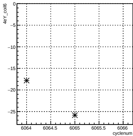
4eY_coil6:cyclenum {run == 6369}
