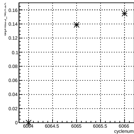
alpha13_4eX1X:cyclenum {run == 6369}
