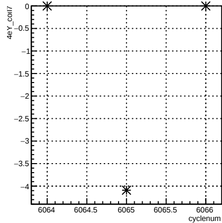
4eY_coil7:cyclenum {run == 6369}
