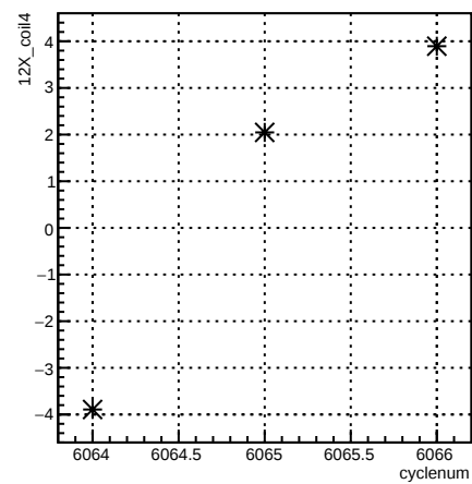
12X_coil4:cyclenum {run == 6369}
