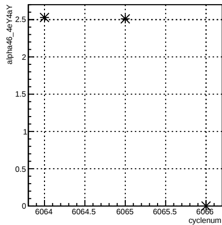
alpha46_4eY4aY:cyclenum {run == 6369}
