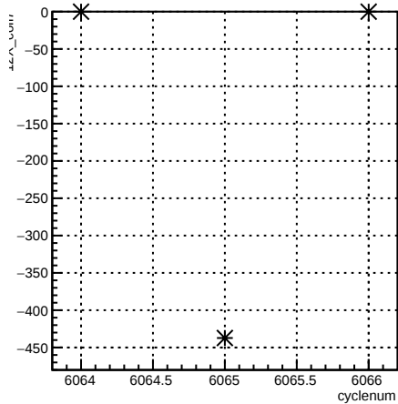
12X_coil7:cyclenum {run == 6369}
