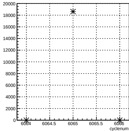
usl_coil7:cyclenum {run == 6369}
