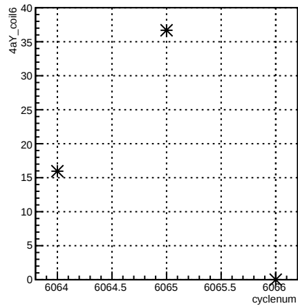
4aY_coil6:cyclenum {run == 6369}
