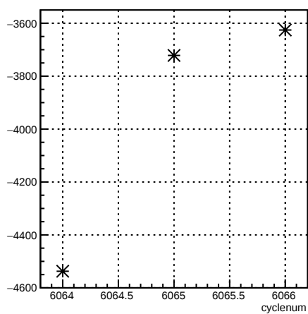
usr_coil3:cyclenum {run == 6369}
