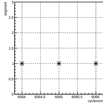
segment:cyclenum {run == 6369}
