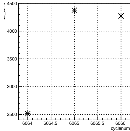
usl_coil4:cyclenum {run == 6369}
