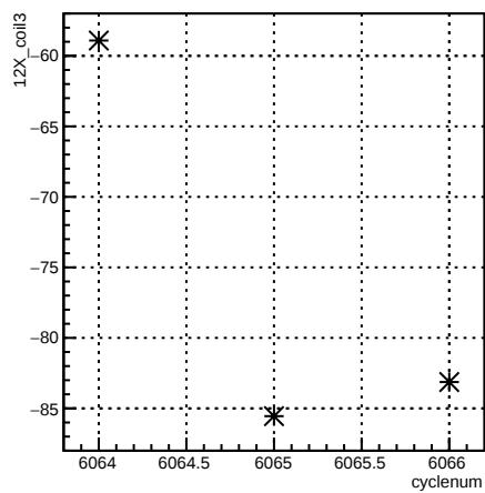
12X_coil3:cyclenum {run == 6369}
