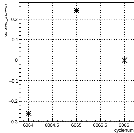
delta46_12X4eY:cyclenum {run == 6369}
