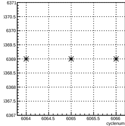
run:cyclenum {run == 6369}
