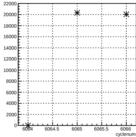
usl_coil1:cyclenum {run == 6369}
