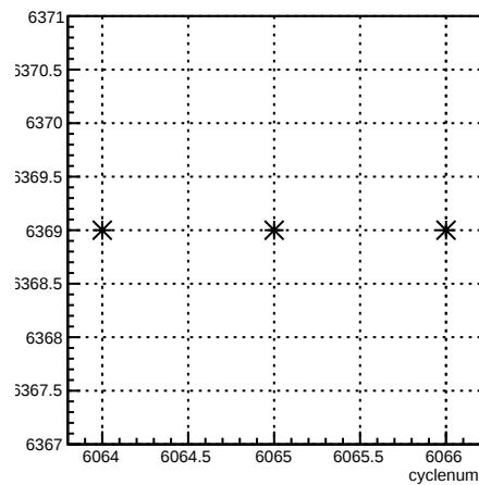
run:cyclenum {run == 6369}
