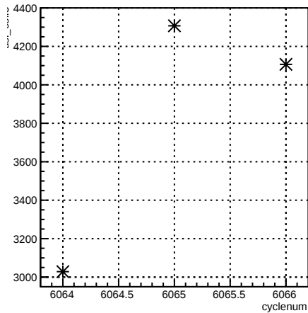
usl_coil3:cyclenum {run == 6369}
