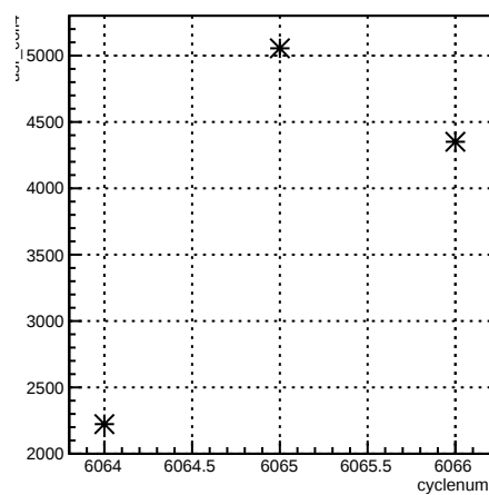
usr_coil4:cyclenum {run == 6369}
