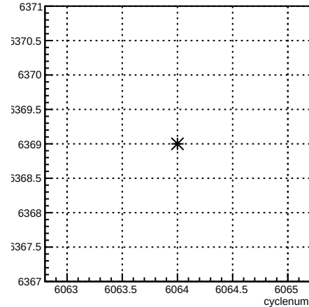
run:cyclenum {run == 6369}
