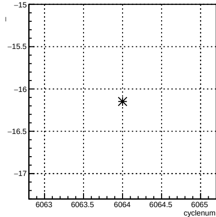
usr_4eY:cyclenum {run == 6369}
