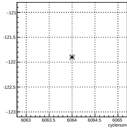
usl_4eY:cyclenum {run == 6369}
