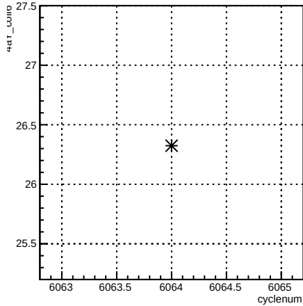
4eY_coil6:cyclenum {run == 6369}
