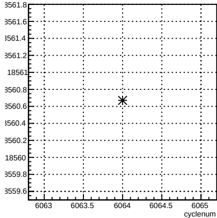
usl_coil7:cyclenum {run == 6369}
