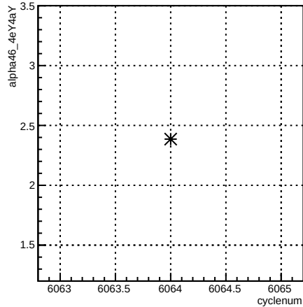
alpha46_4eY4aY:cyclenum {run == 6369}
