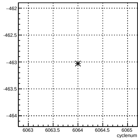
usr_coil6:cyclenum {run == 6369}
