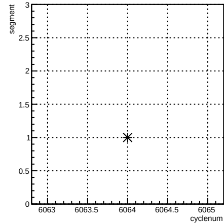
segment:cyclenum {run == 6369}
