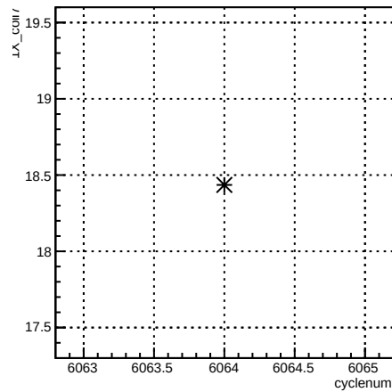
4eX_coil7:cyclenum {run == 6369}
