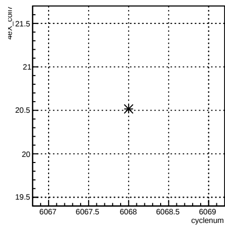
4eX_coil7:cyclenum {run == 6371}
