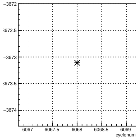
usr_coil3:cyclenum {run == 6371}
