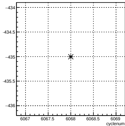
12X_coil7:cyclenum {run == 6371}
