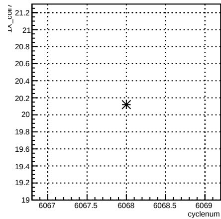
4eX_coil7:cyclenum {run == 6371}
