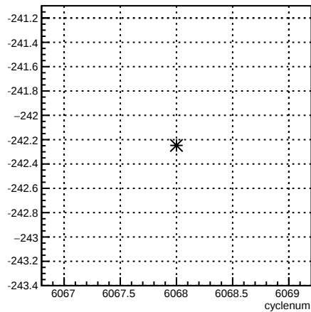
12X_coil1:cyclenum {run == 6371}
