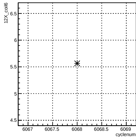
12X_coil6:cyclenum {run == 6371}
