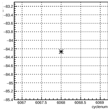
12X_coil3:cyclenum {run == 6371}
