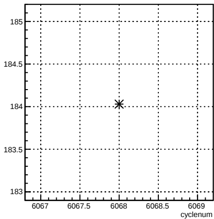
4eY_coil4:cyclenum {run == 6371}
