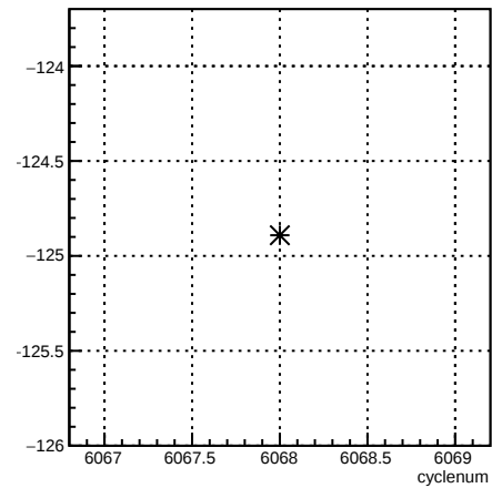
usl_4eY:cyclenum {run == 6371}
