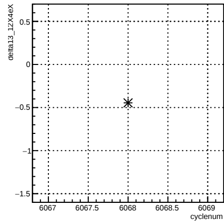
delta13_12X4eX:cyclenum {run == 6371}
