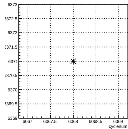
run:cyclenum {run == 6371}
