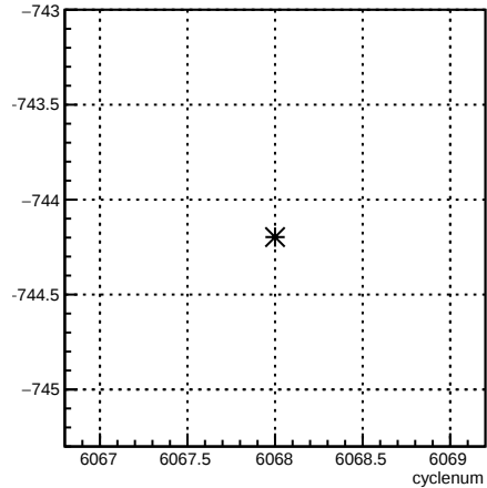
usr_coil6:cyclenum {run == 6371}
