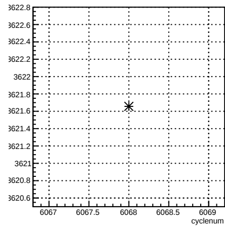
usl_coil4:cyclenum {run == 6371}
