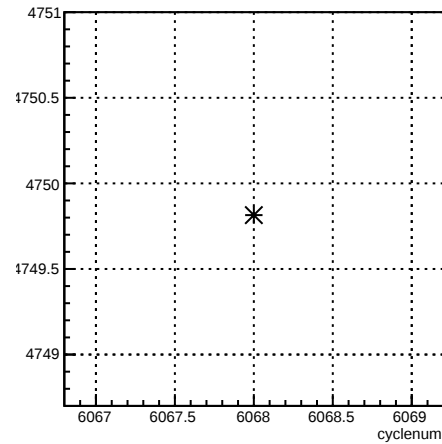
usr_coil4:cyclenum {run == 6371}
