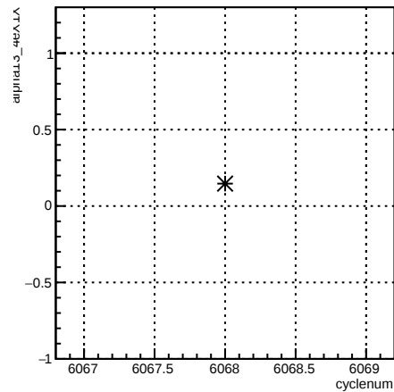
alpha13_4eX1X:cyclenum {run == 6371}
