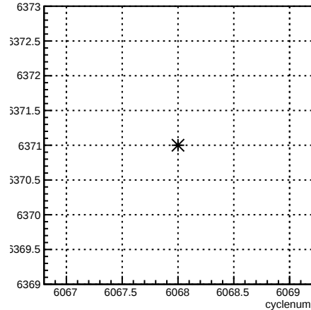
run:cyclenum {run == 6371}
