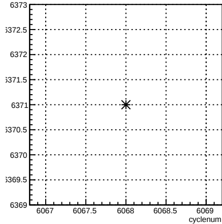
run:cyclenum {run == 6371}
