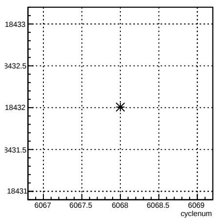
usl_coil7:cyclenum {run == 6371}
