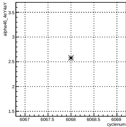
alpha46_4eY4aY:cyclenum {run == 6371}
