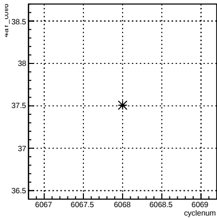
4eY_coil6:cyclenum {run == 6371}
