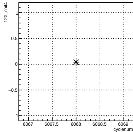
12X_coil4:cyclenum {run == 6371}
