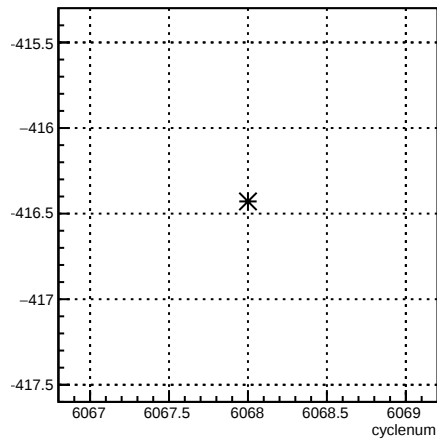
4eX_coil1:cyclenum {run == 6371}
