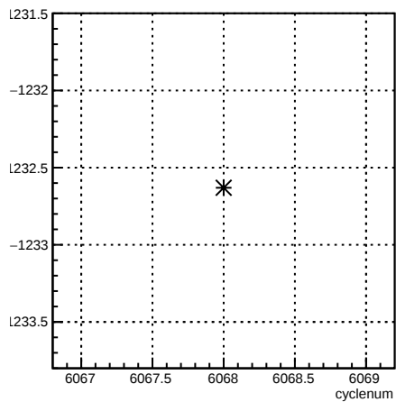
usl_coil6:cyclenum {run == 6371}
