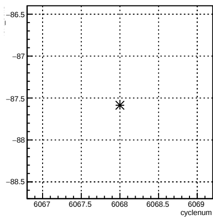
4eX_coil3:cyclenum {run == 6371}
