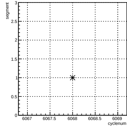
segment:cyclenum {run == 6371}
