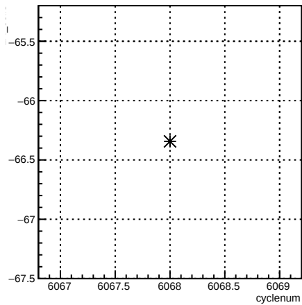
4eX_coil3:cyclenum {run == 6371}
