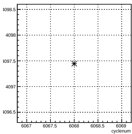
usl_coil3:cyclenum {run == 6371}
