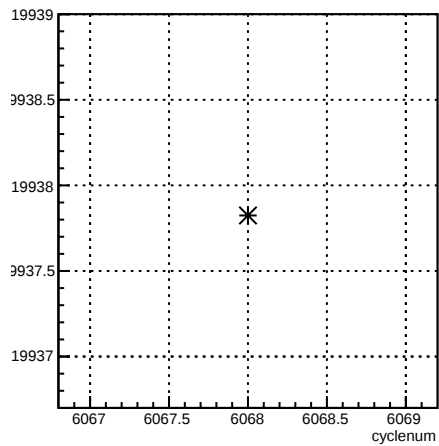
usl_coil1:cyclenum {run == 6371}
