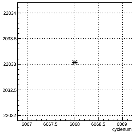
usr_coil7:cyclenum {run == 6371}
