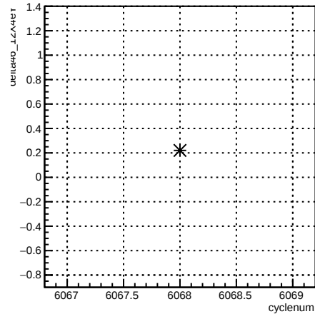
delta46_12X4eY:cyclenum {run == 6371}
