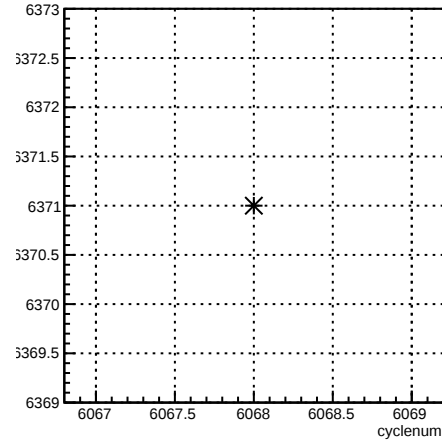
run:cyclenum {run == 6371}
