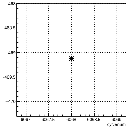
4eX_coil1:cyclenum {run == 6371}
