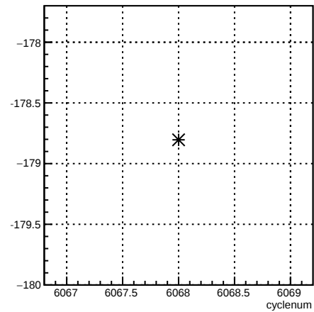
usr_4eY:cyclenum {run == 6371}
