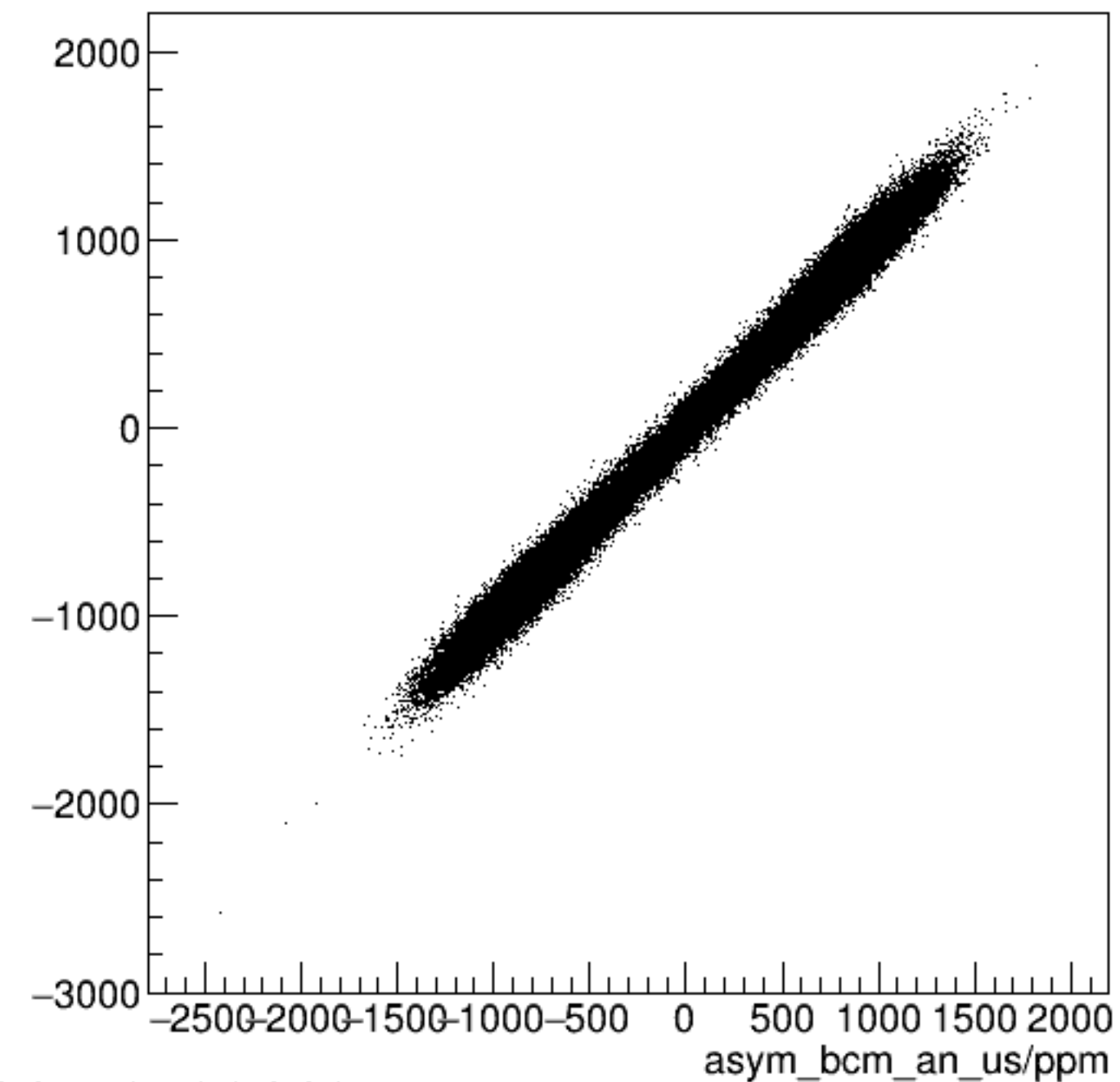
run6371_000_asym_bcm_dg_ds_vs_asym_bcm_an_us_pr.png
