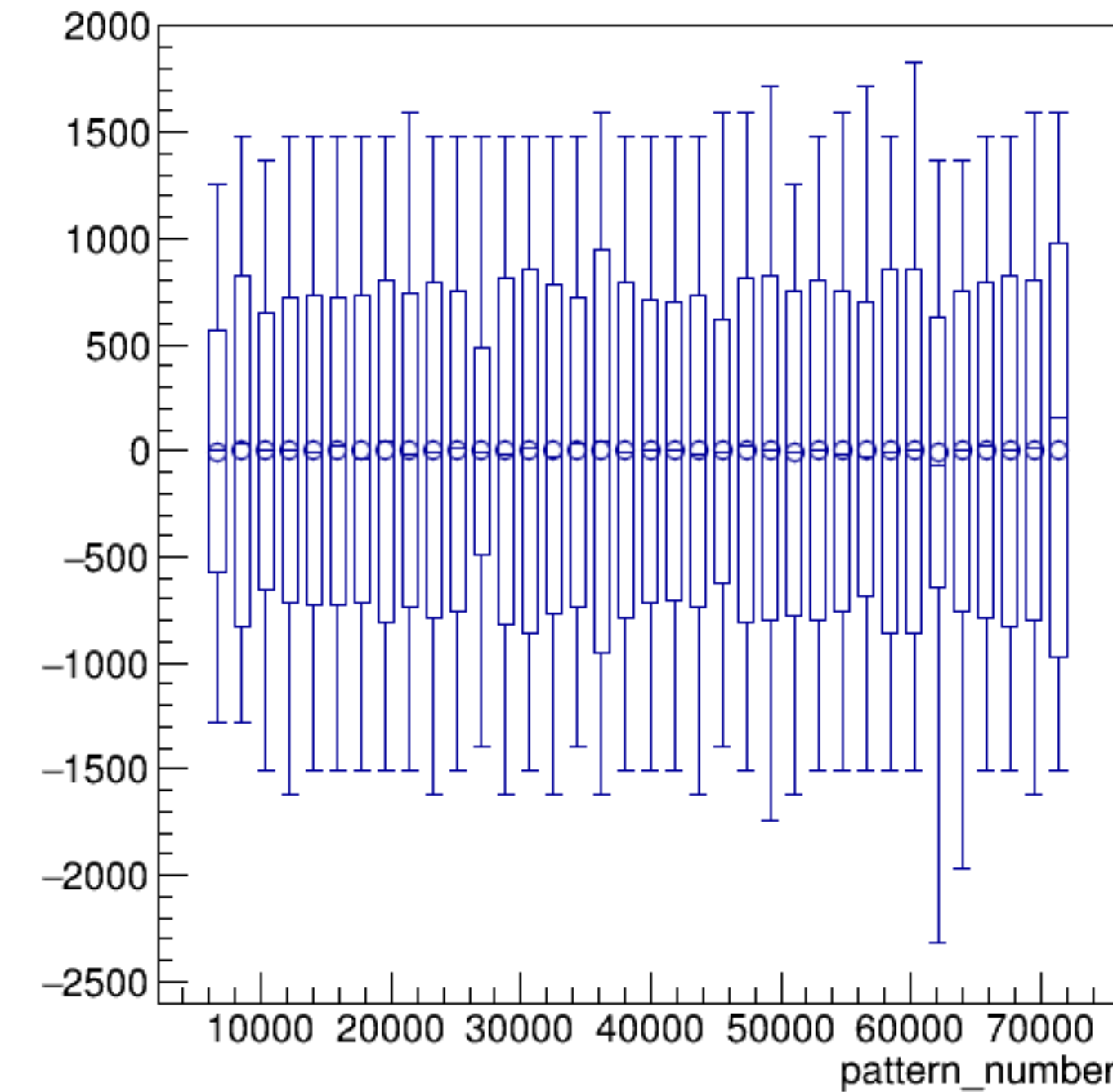
asym_bcm_an_ds3/ppm:pattern_number {ErrorFlag==0}
