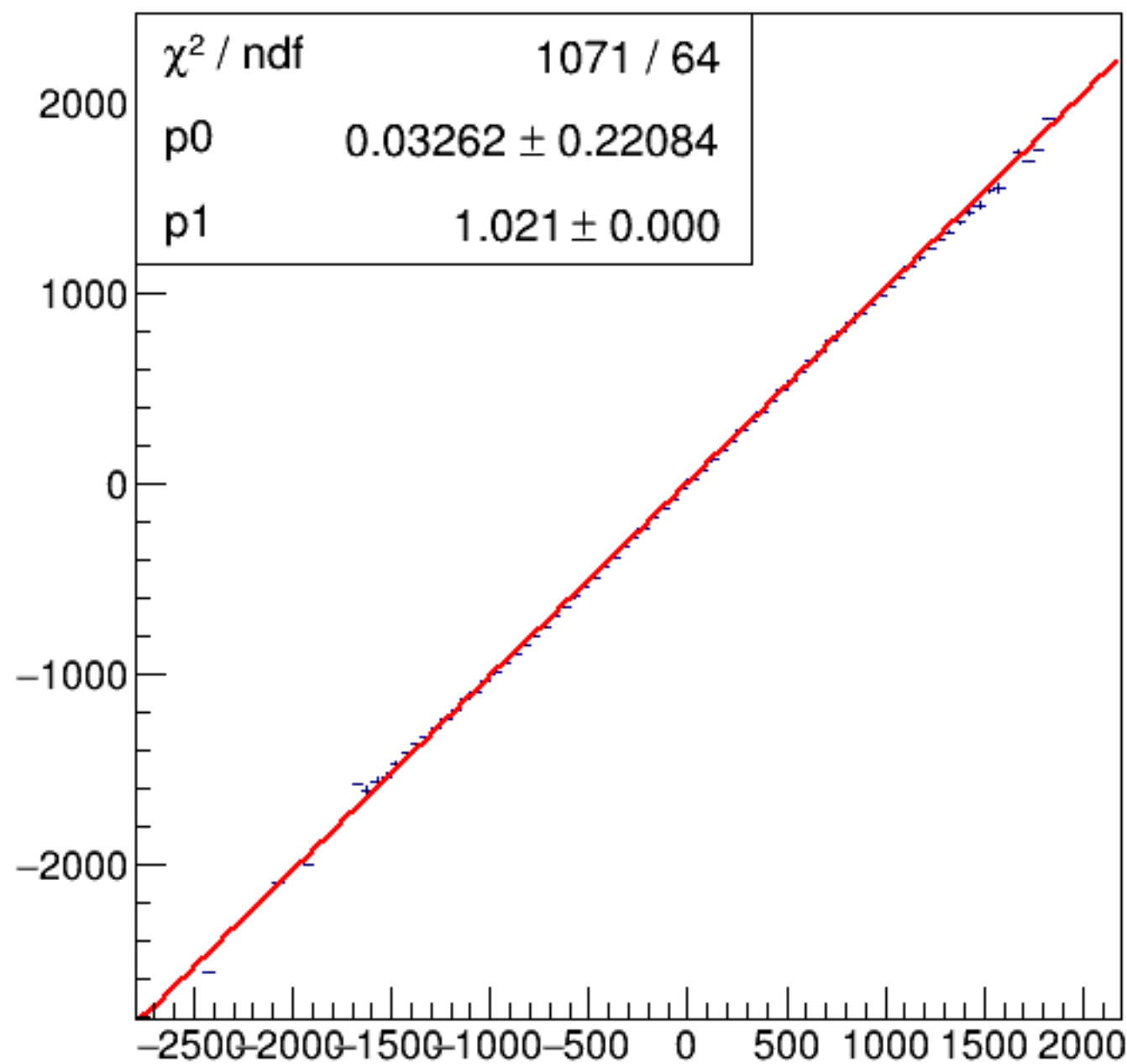
run6371_000_asym_bcm_dg_ds_vs_asym_bcm_an_us_pr.png
