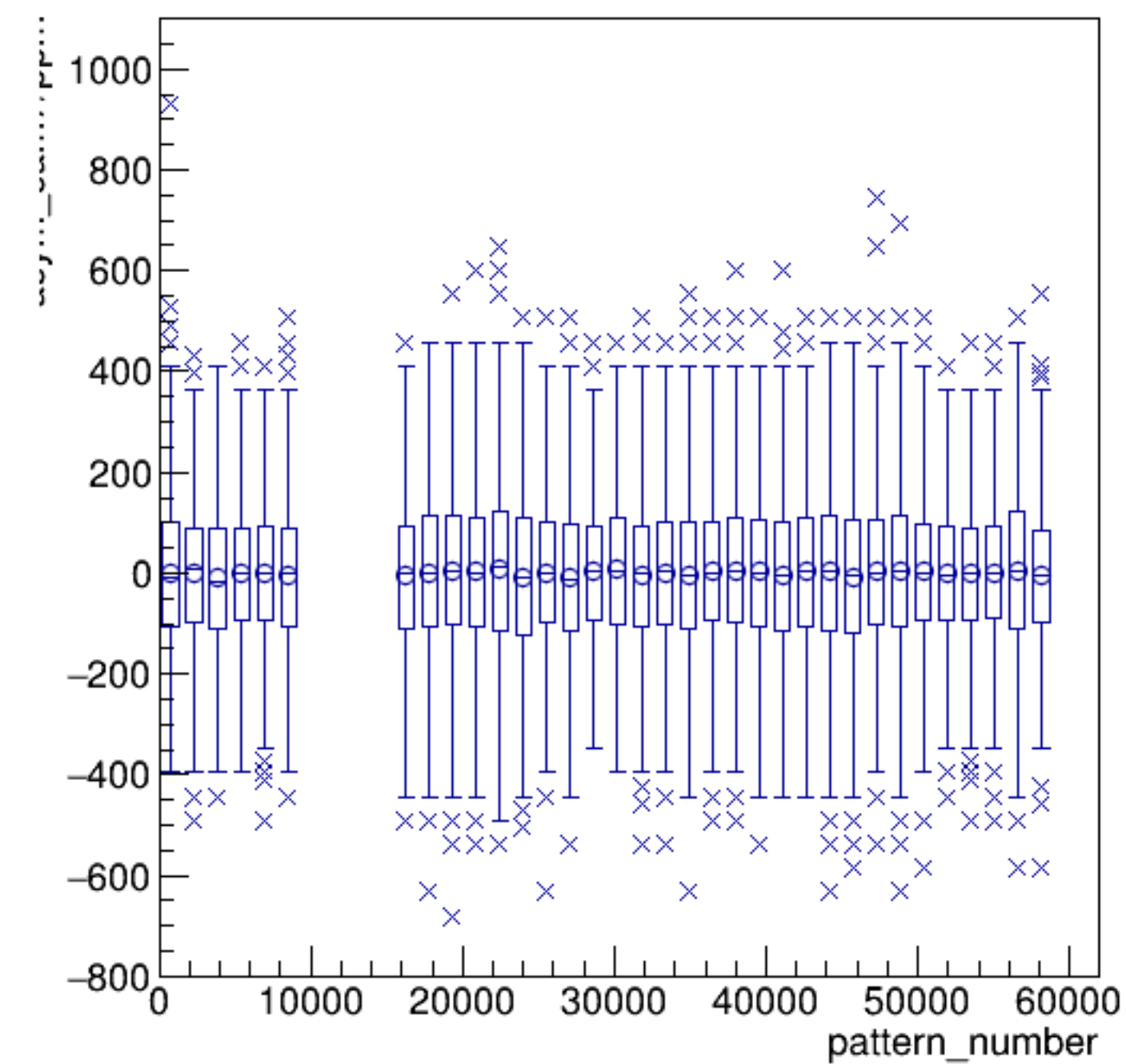
asym_sam7/ppm:pattern_number {ErrorFlag==0}
