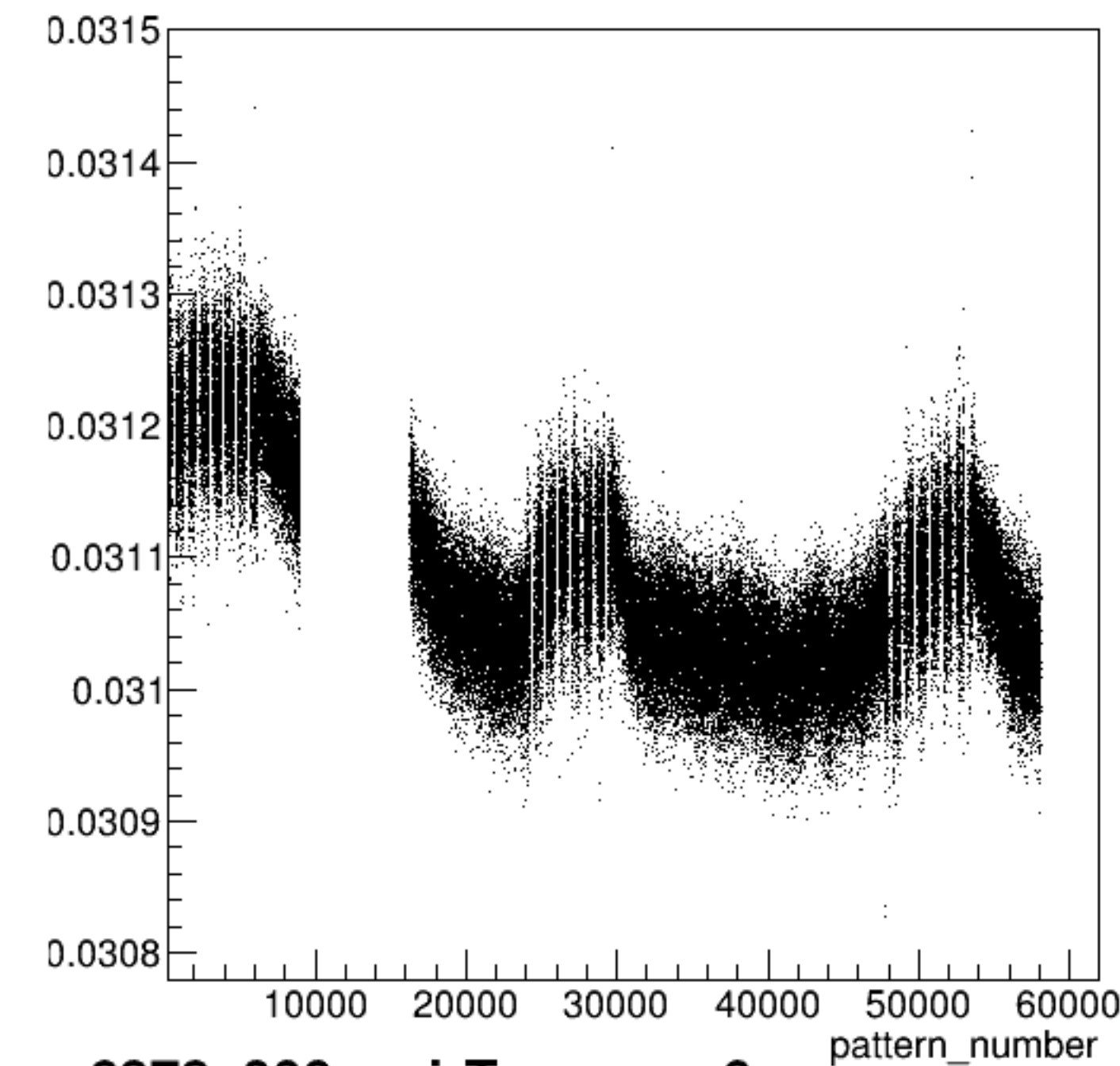
yield_sam6:pattern_number {ErrorFlag==0}
