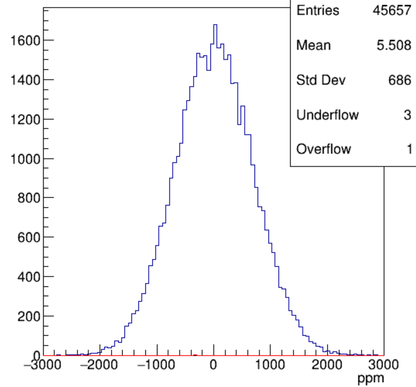
asym_sam6
