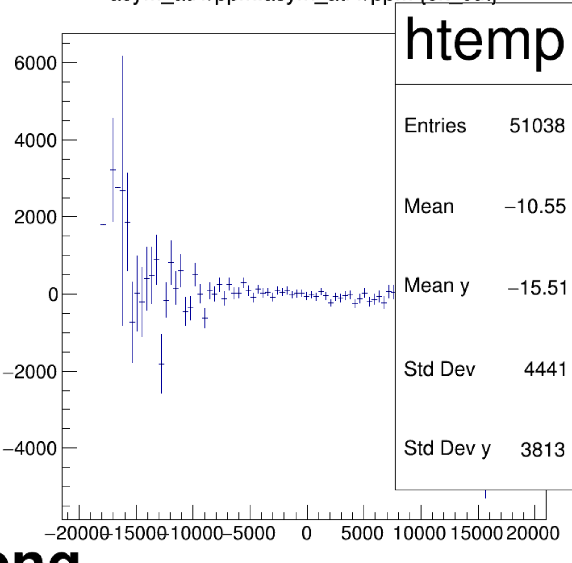
asym_atl1/ppm:asym_atr1/ppm {ok_cut}
