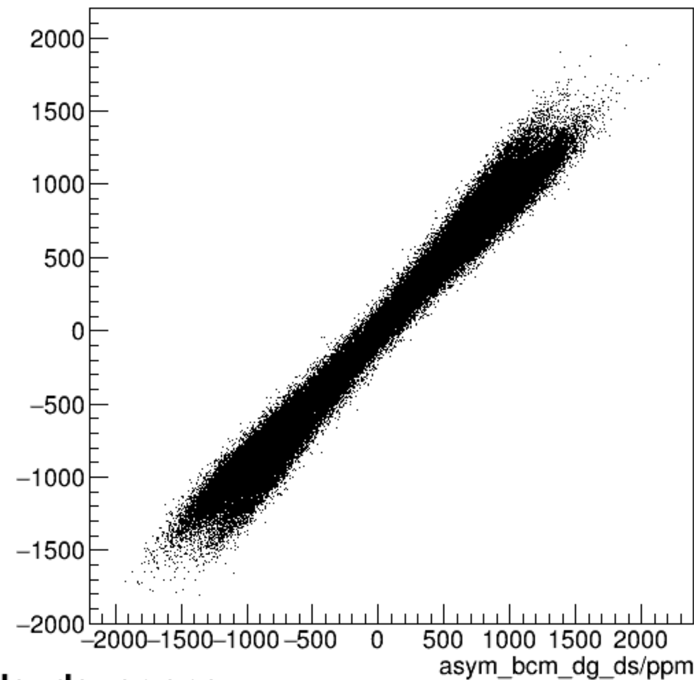
run6374_000_asym_bcm_dg_us_vs_asym_bcm_dg_ds_pr.png
