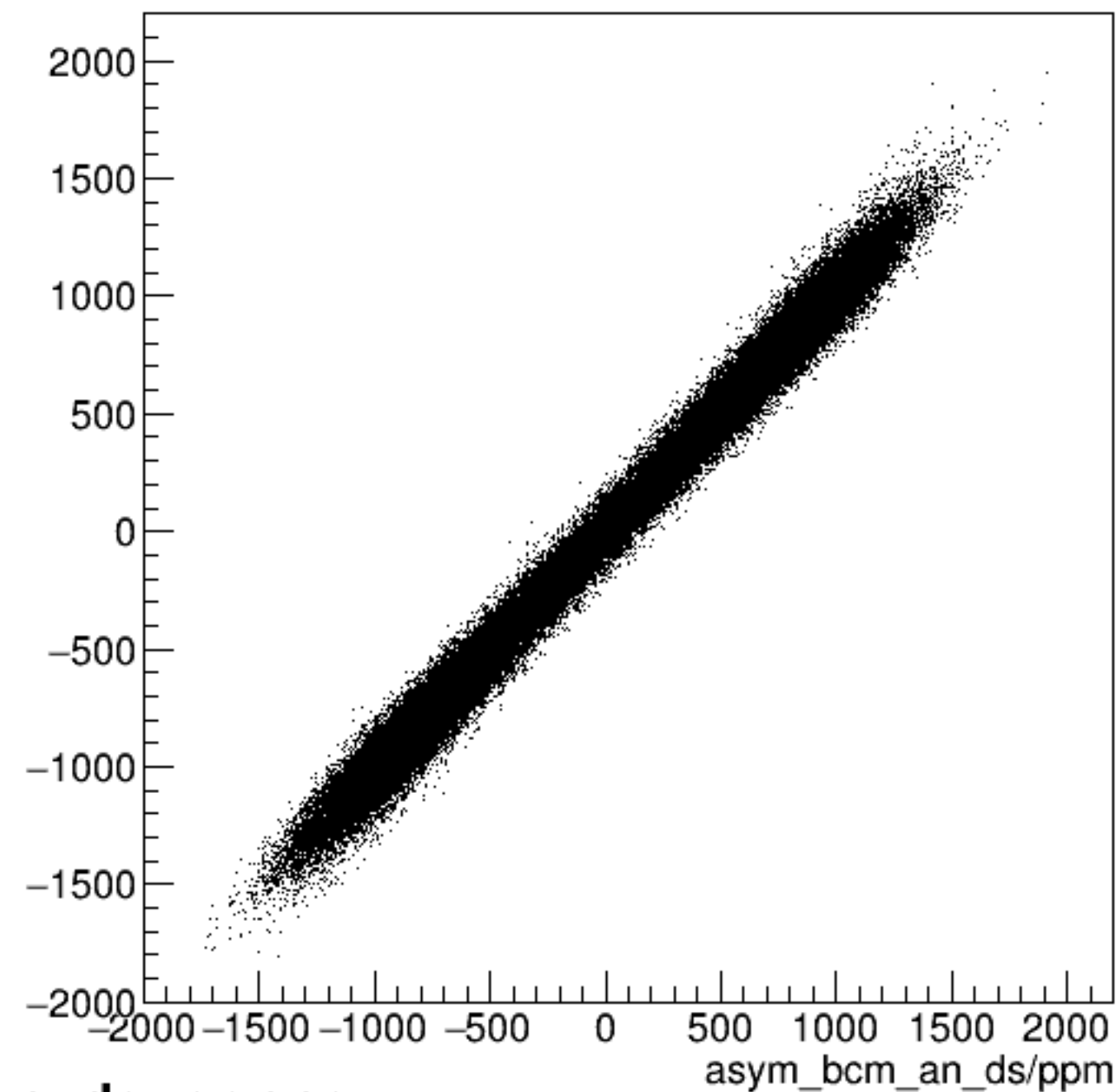
run6374_000_asym_bcm_dg_us_vs_asym_bcm_an_ds_pr.png
