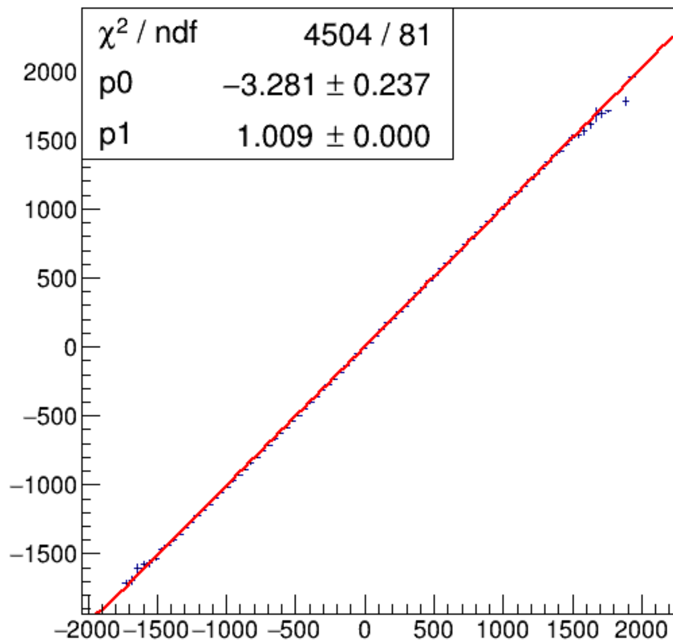
run6374_000_asym_bcm_dg_us_vs_asym_bcm_an_ds_pr.png
