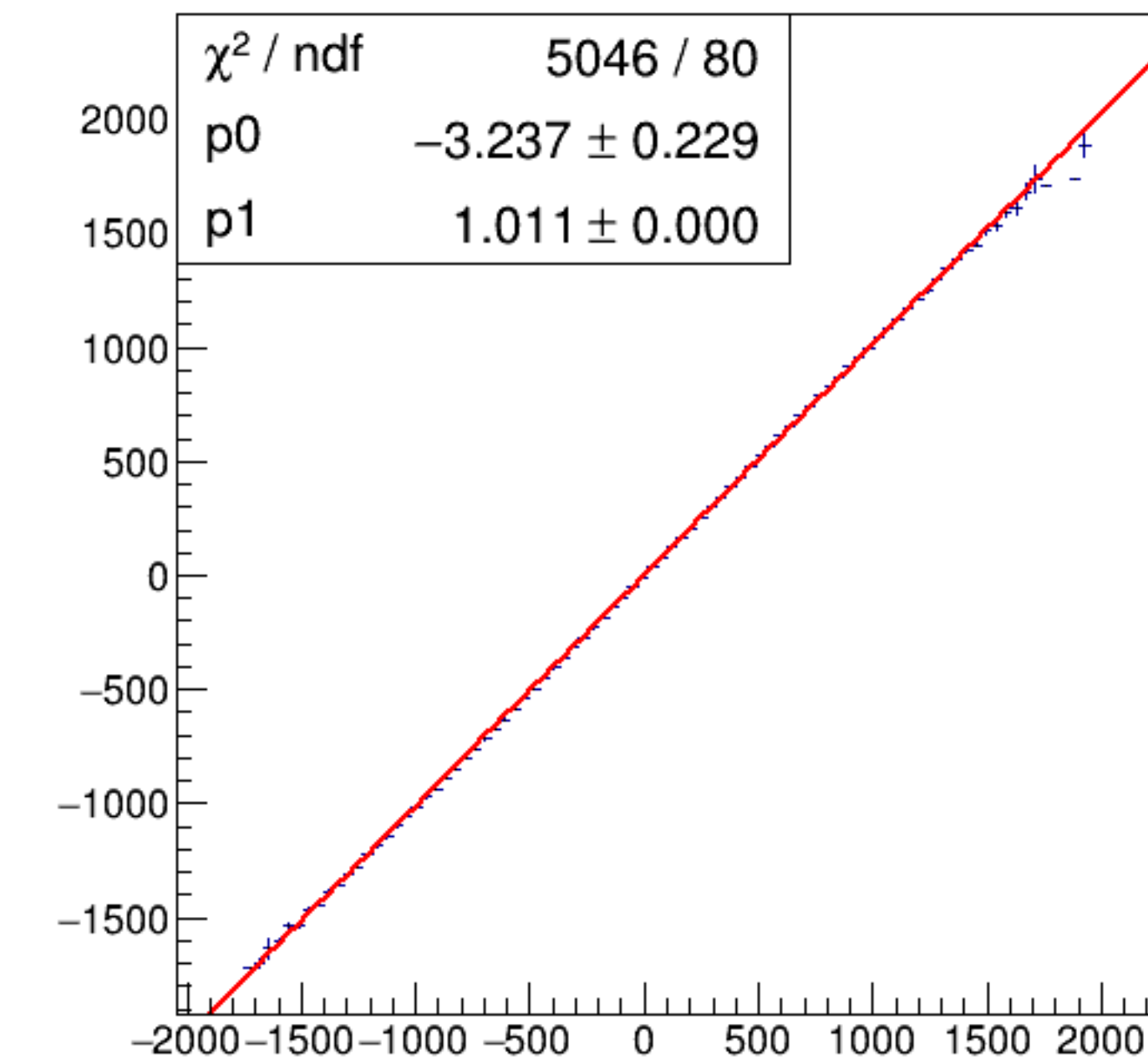
run6374_000_asym_bcm_dg_us_vs_asym_bcm_an_ds3_pr.png
