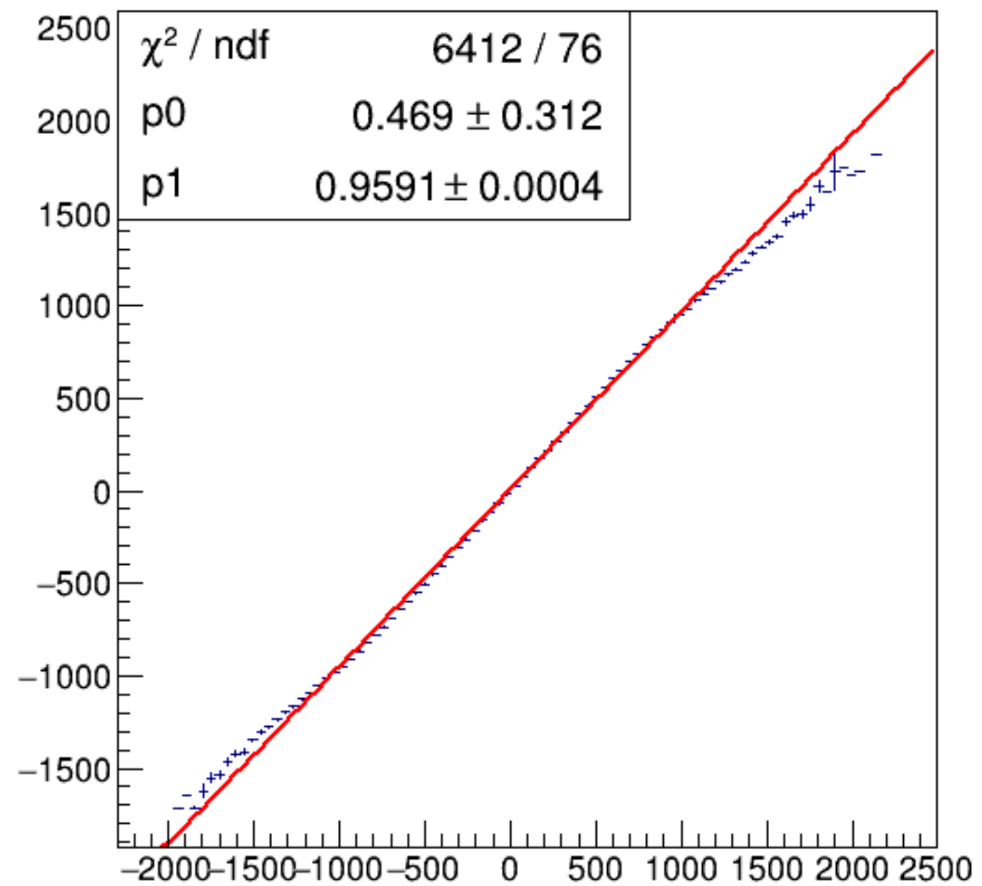
run6374_000_asym_bcm_dg_us_vs_asym_bcm_dg_ds_pr.png
