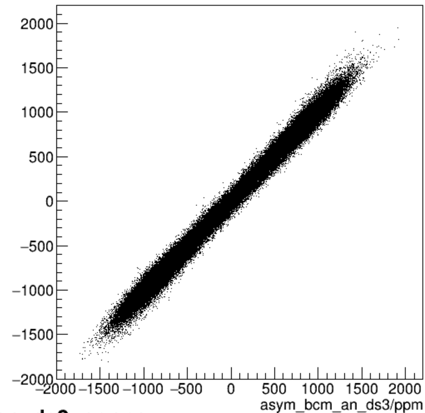
run6374_000_asym_bcm_dg_us_vs_asym_bcm_an_ds3_pr.png
