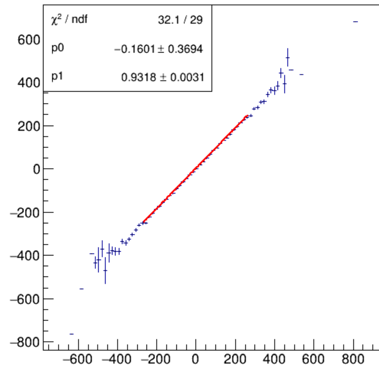
asym_bpm16WS/ppm:Aq/ppm {ErrorFlag==0}
