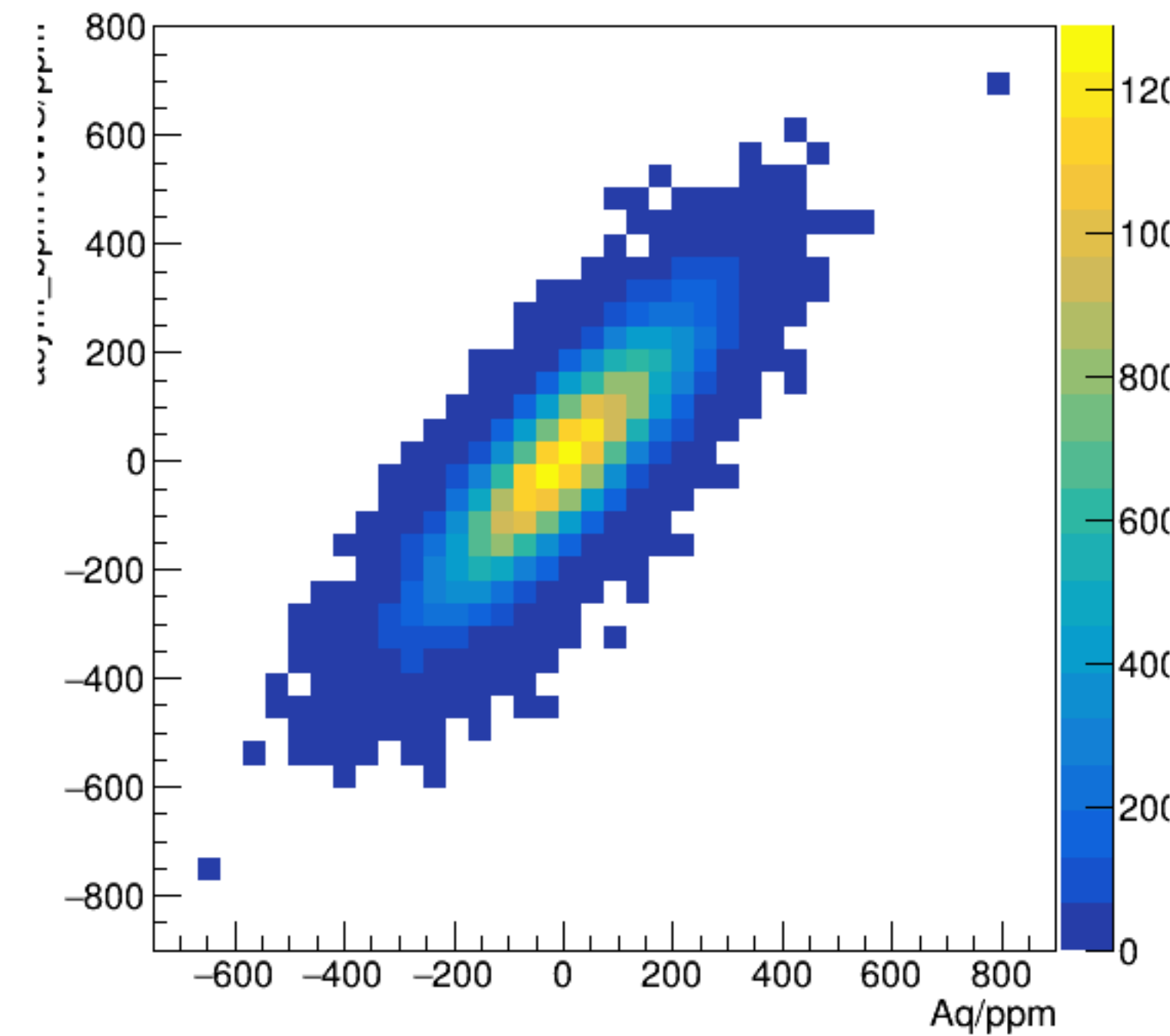
asym_bpm16WS/ppm:Aq/ppm {ErrorFlag==0}
