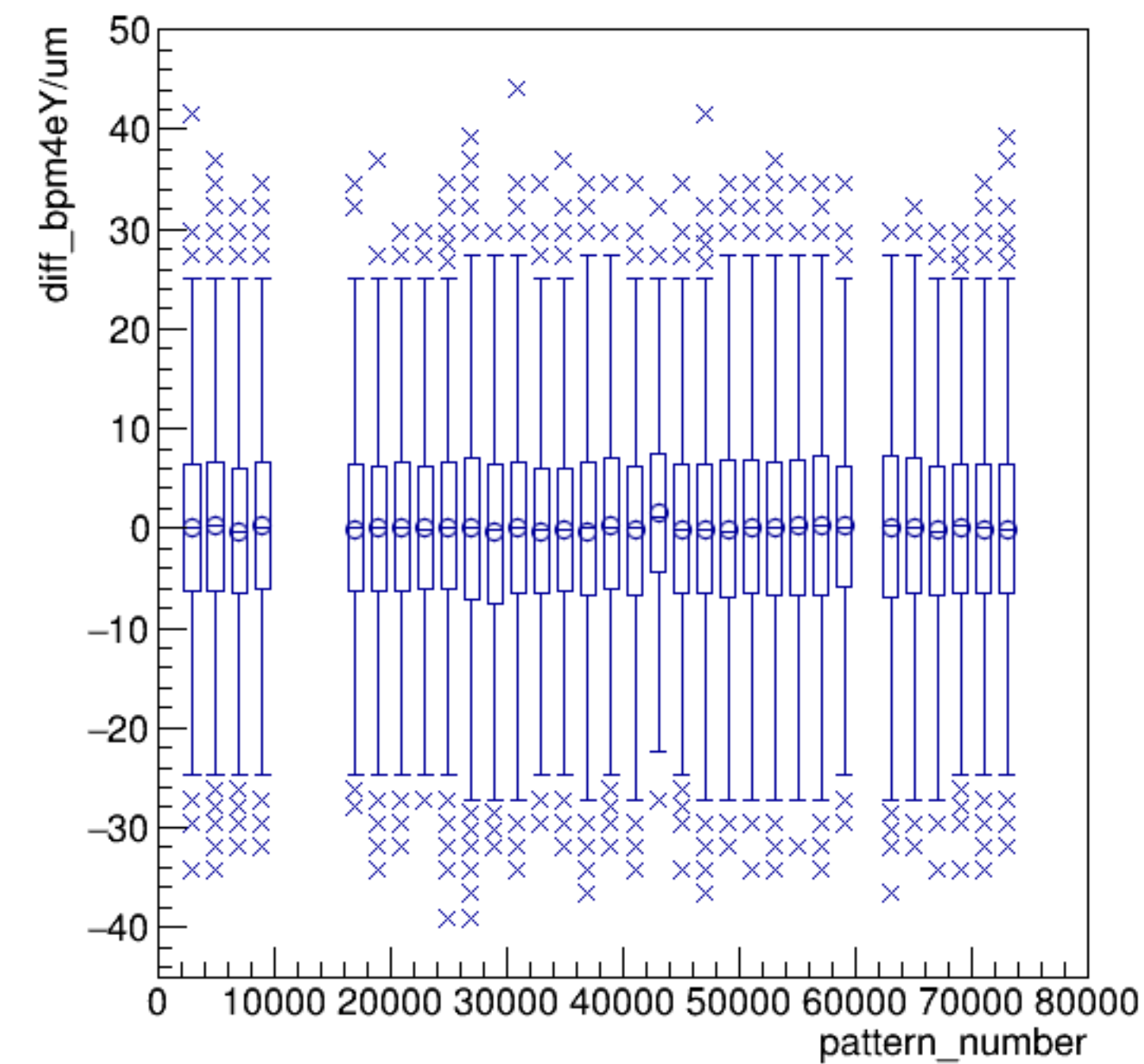
diff_bpm4eY/um:pattern_number {ErrorFlag==0}
