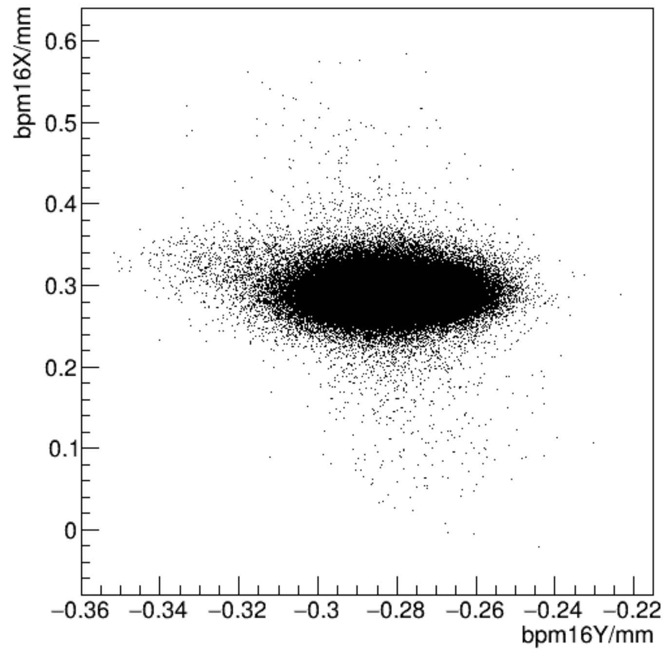
bpm16X/mm:bpm16Y/mm {ErrorFlag==0}
