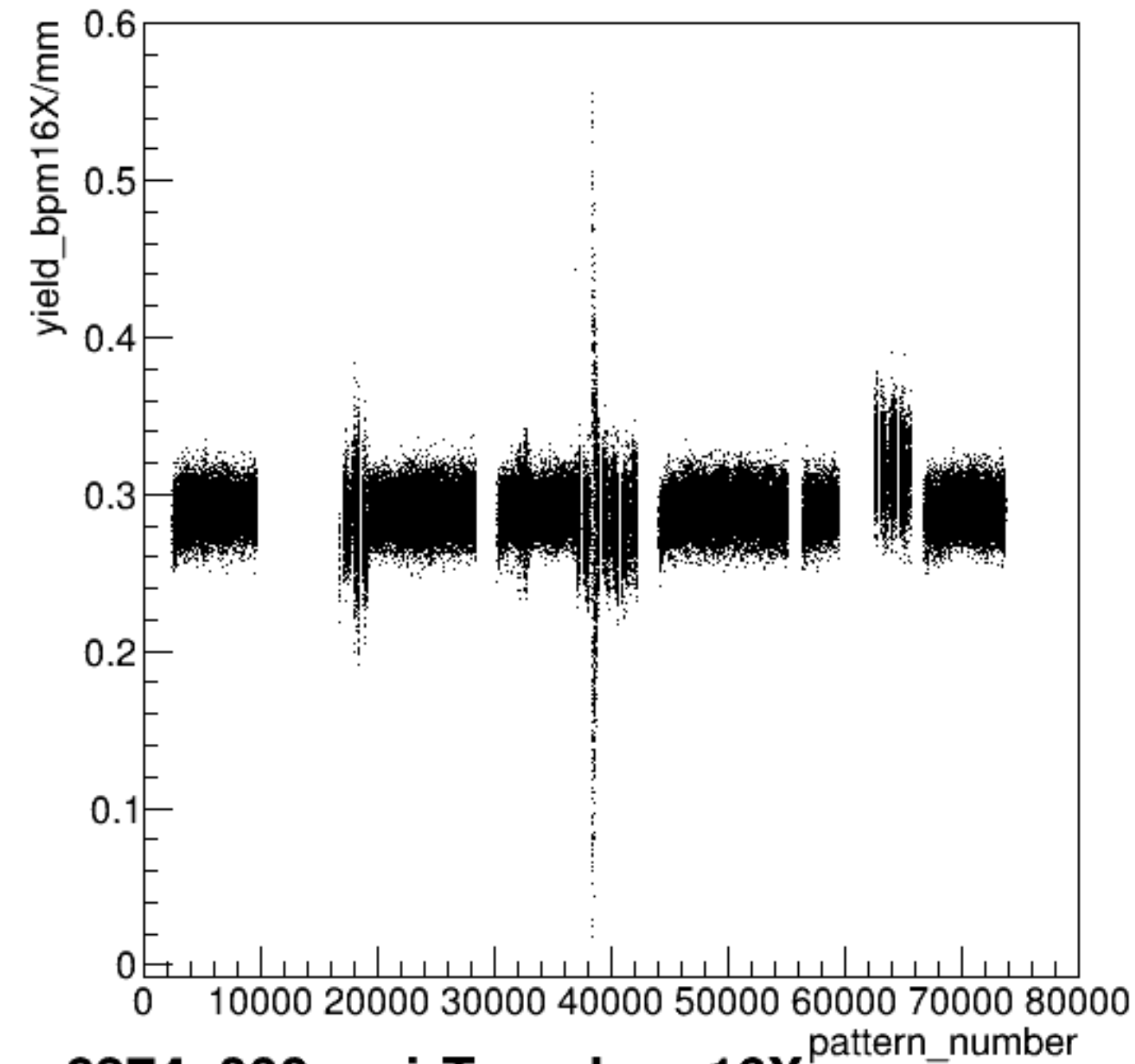
yield_bpm16X/mm:pattern_number {ErrorFlag==0}
