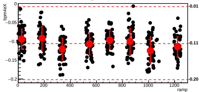
bmod_trim4,cyc=6080
