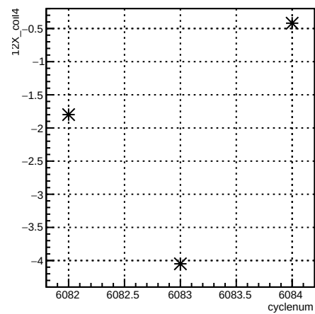
12X_coil4:cyclenum {run == 6375}
