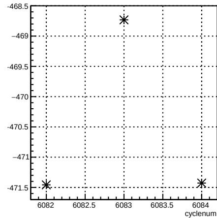
4eX_coil1:cyclenum {run == 6375}
