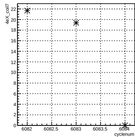
4eX_coil7:cyclenum {run == 6375}
