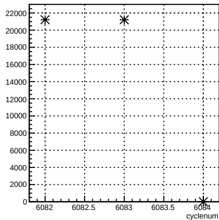
usr_coil7:cyclenum {run == 6375}
