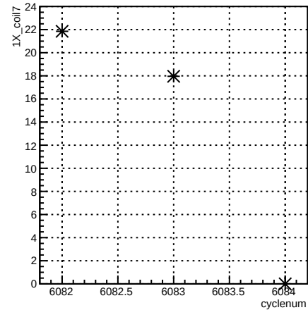
1X_coil7:cyclenum {run == 6375}
