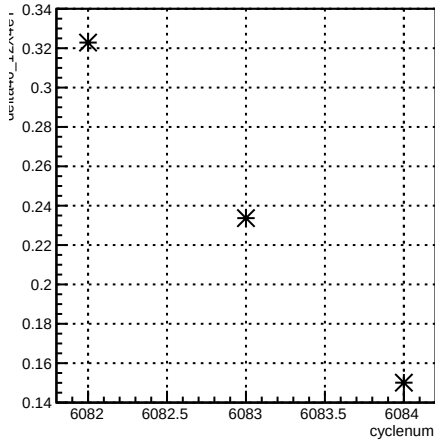
delta46_12X4eY:cyclenum {run == 6375}
