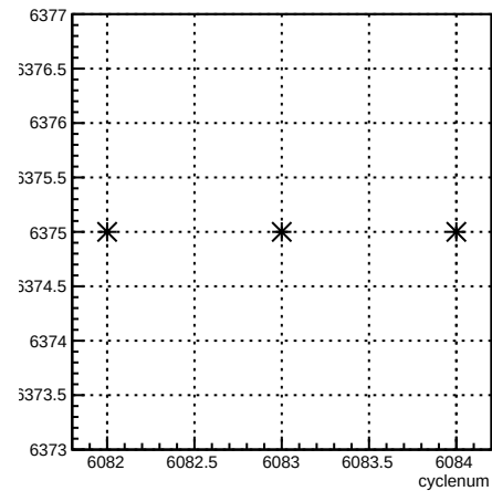
run:cyclenum {run == 6375}
