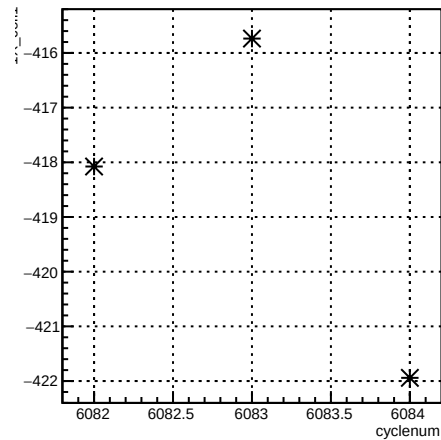
1X_coil1:cyclenum {run == 6375}
