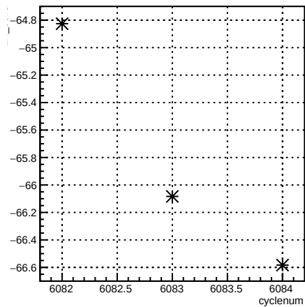
1X_coil3:cyclenum {run == 6375}
