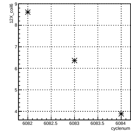
12X_coil6:cyclenum {run == 6375}
