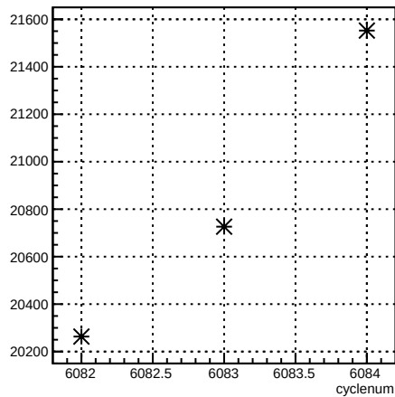
usl_coil6:cyclenum {run == 6375}
