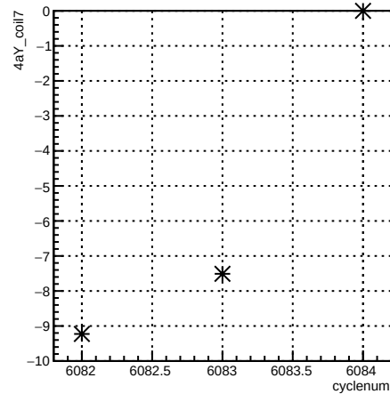
4aY_coil7:cyclenum {run == 6375}
