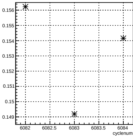
alpha13_4eX1X:cyclenum {run == 6375}
