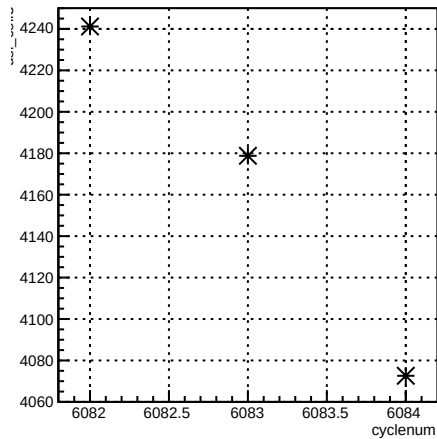
usl_coil7:cyclenum {run == 6375}
