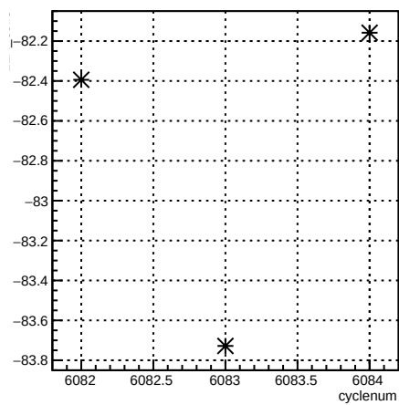
12X_coil3:cyclenum {run == 6375}
