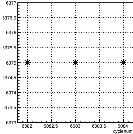
run:cyclenum {run == 6375}
