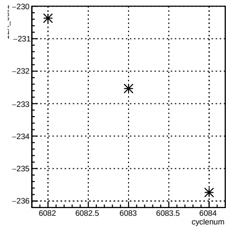
12X_coil1:cyclenum {run == 6375}
