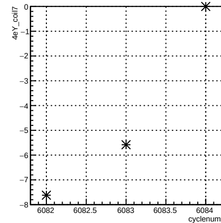
4eY_coil7:cyclenum {run == 6375}
