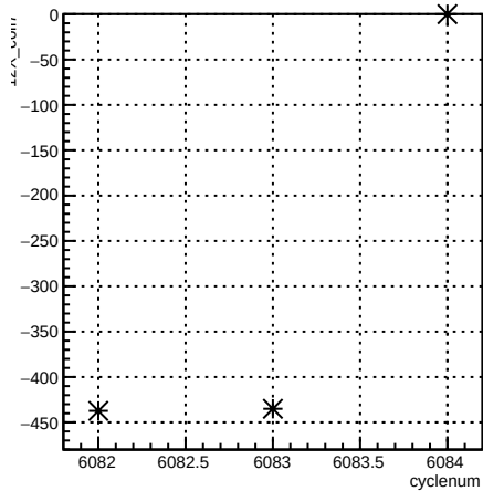
12X_coil7:cyclenum {run == 6375}
