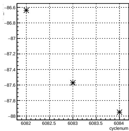
4eX_coil3:cyclenum {run == 6375}
