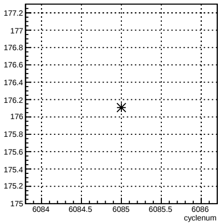
4eY_coil4:cyclenum {run == 6376}
