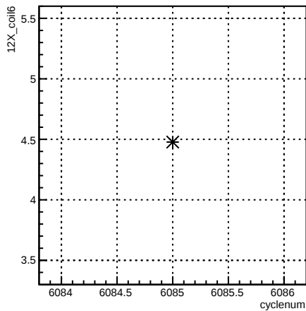
12X_coil6:cyclenum {run == 6376}
