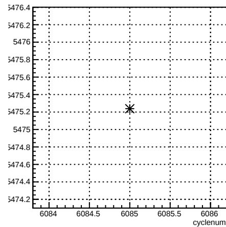
usr_coil4:cyclenum {run == 6376}
