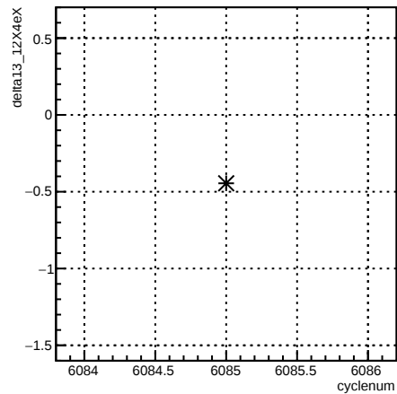
delta13_12X4eX:cyclenum {run == 6376}
