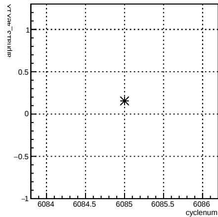
alpha13_4eX1X:cyclenum {run == 6376}
