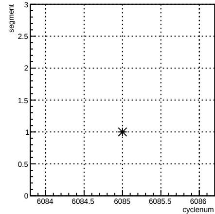
segment:cyclenum {run == 6376}
