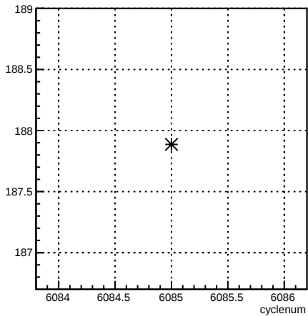
4eY_coil4:cyclenum {run == 6376}
