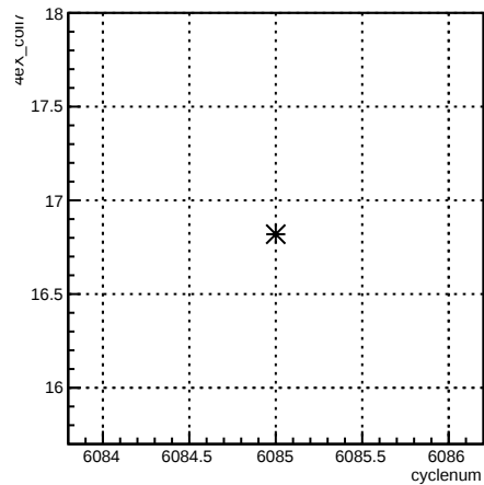
4eX_coil7:cyclenum {run == 6376}
