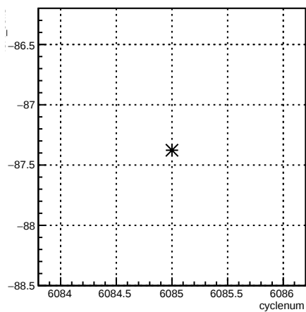
4eX_coil3:cyclenum {run == 6376}
