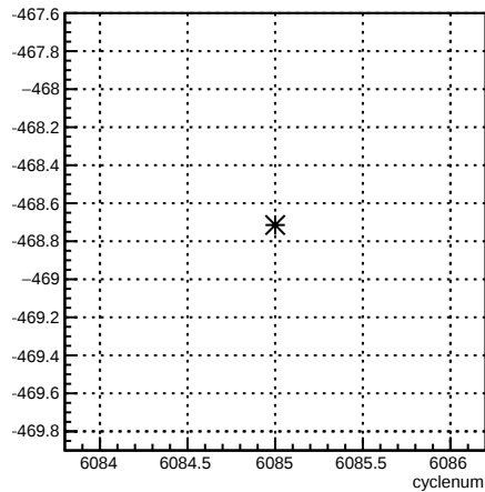
4eX_coil1:cyclenum {run == 6376}
