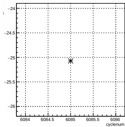
4eY_coil6:cyclenum {run == 6376}
