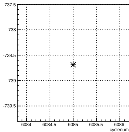
usr_coil6:cyclenum {run == 6376}
