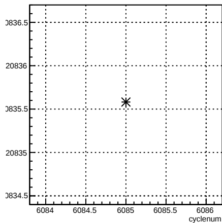
usr_coil7:cyclenum {run == 6376}
