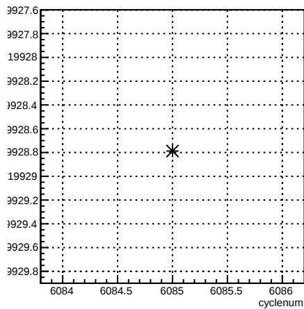
usr_coil1:cyclenum {run == 6376}
