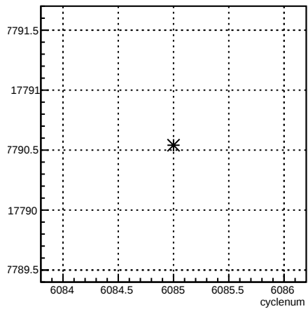
usl_coil7:cyclenum {run == 6376}
