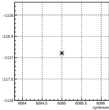
usl_coil6:cyclenum {run == 6376}
