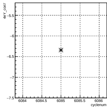
4eY_coil7:cyclenum {run == 6376}
