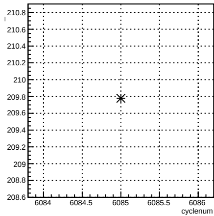
run:cyclenum {run == 6376}
