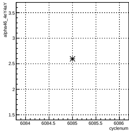
alpha46_4eY4aY:cyclenum {run == 6376}
