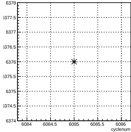
run:cyclenum {run == 6376}
