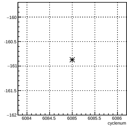
usr_4eY:cyclenum {run == 6376}
