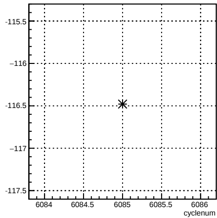
usl_4eY:cyclenum {run == 6376}
