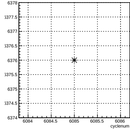
run:cyclenum {run == 6376}
