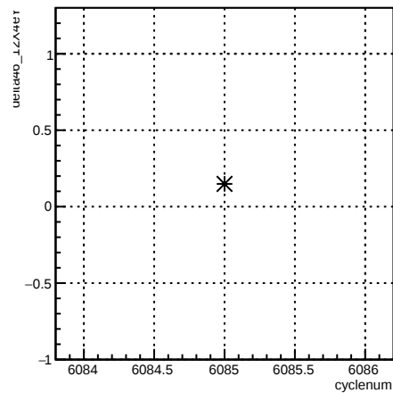
delta46_12X4eY:cyclenum {run == 6376}
