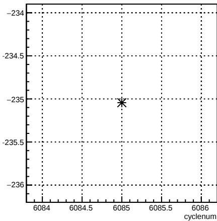
12X_coil6:cyclenum {run == 6376}
