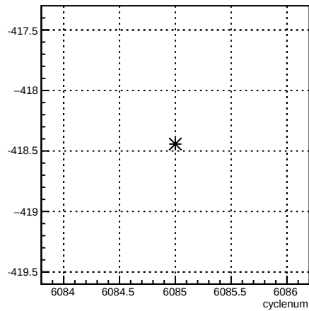
4eX_coil1:cyclenum {run == 6376}
