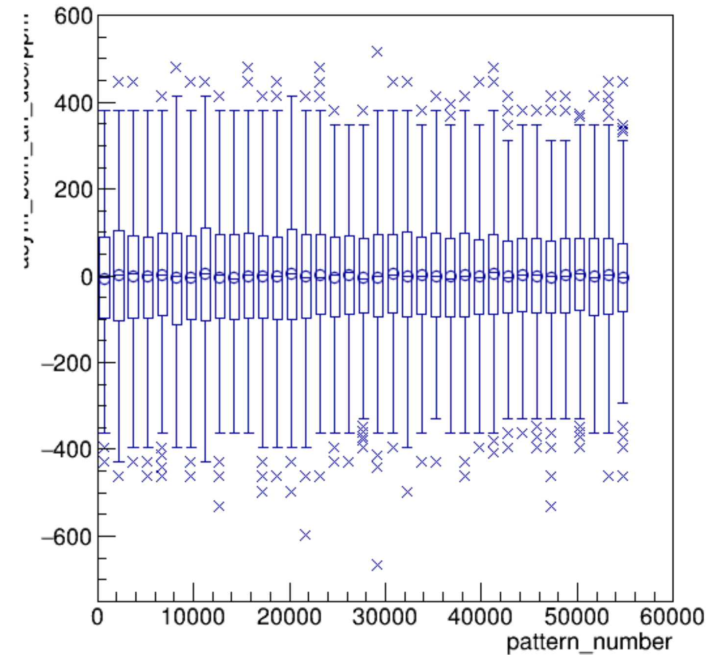
asym_bcm_an_ds3/ppm:pattern_number {ErrorFlag==0}
