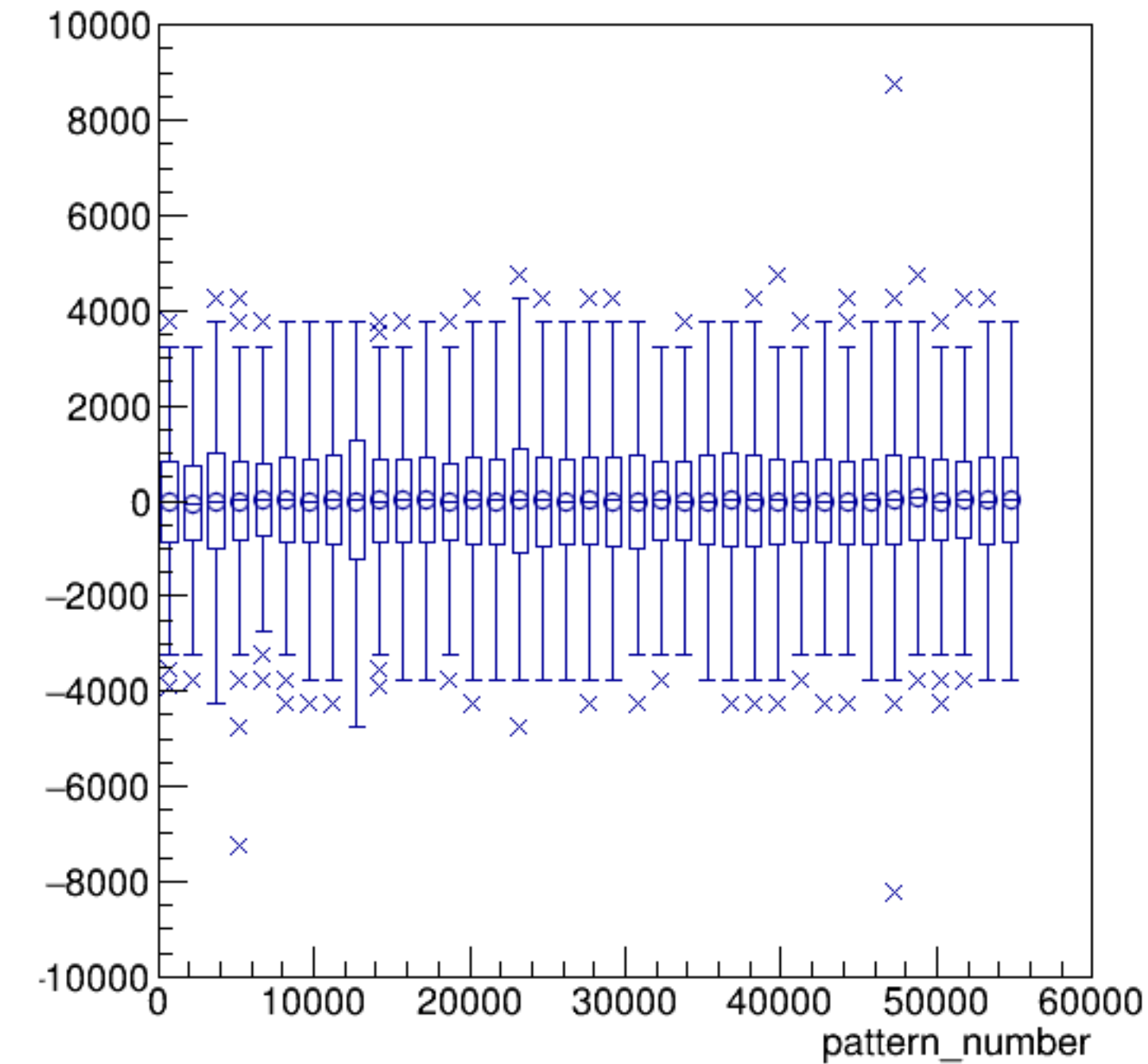
asym_sam6/ppm:pattern_number {ErrorFlag==0}
