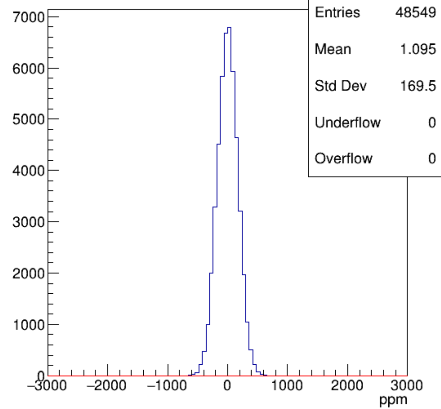
asym_sam7
