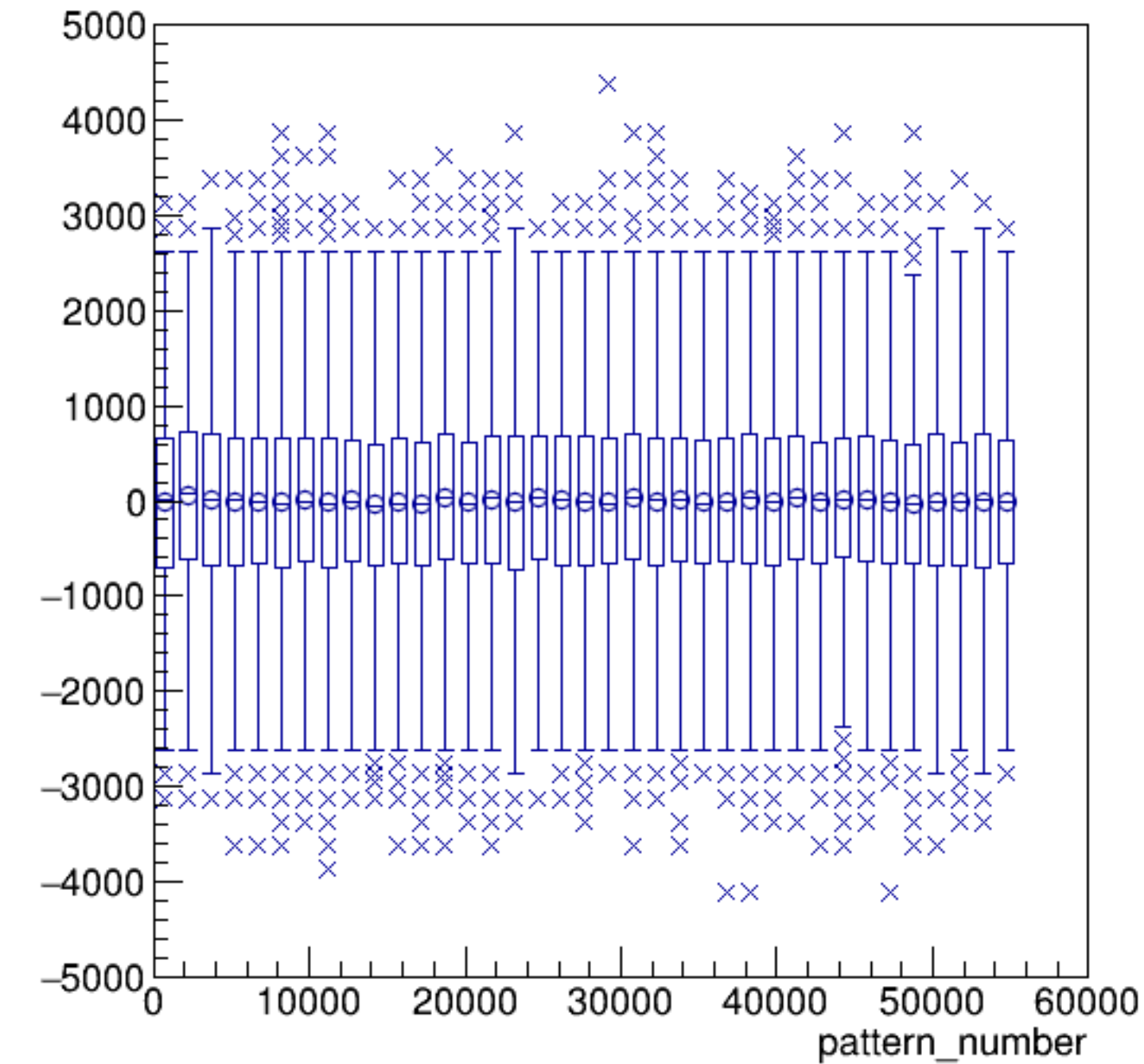
asym_sam1/ppm:pattern_number {ErrorFlag==0}
