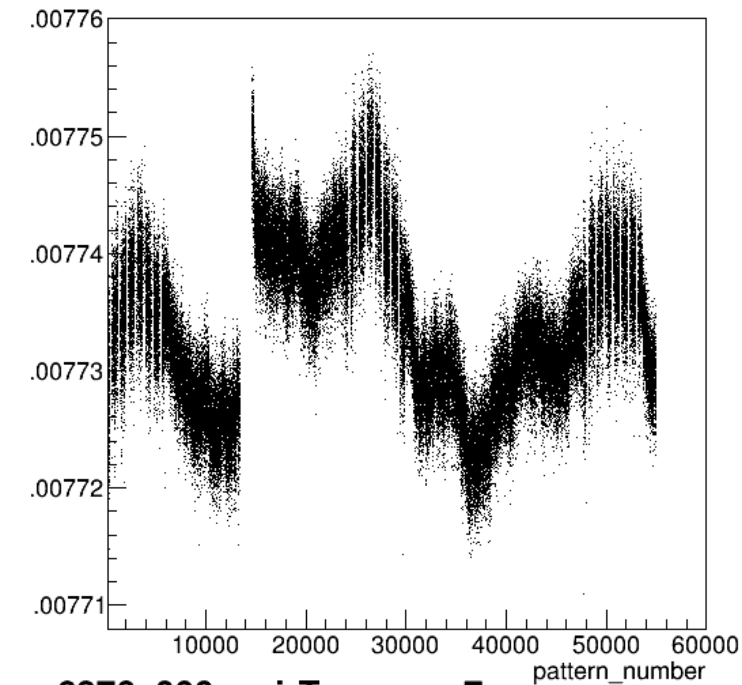
yield_sam7:pattern_number {ErrorFlag==0}
