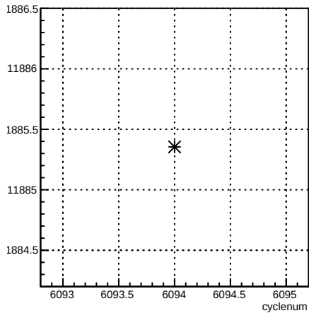
usl_coil7:cyclenum {run == 6380}
