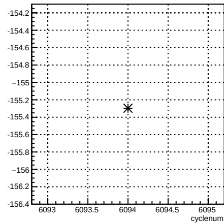
usr_4eY:cyclenum {run == 6380}
