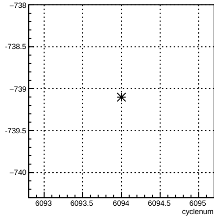
usr_coil6:cyclenum {run == 6380}
