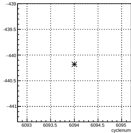
1X_coil1:cyclenum {run == 6380}
