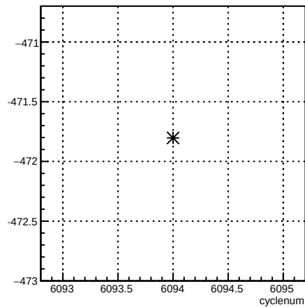
4eX_coil1:cyclenum {run == 6380}
