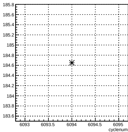
4eY_coil4:cyclenum {run == 6380}
