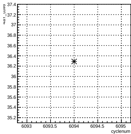
4aY_coil6:cyclenum {run == 6380}
