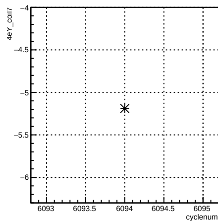
4eY_coil7:cyclenum {run == 6380}
