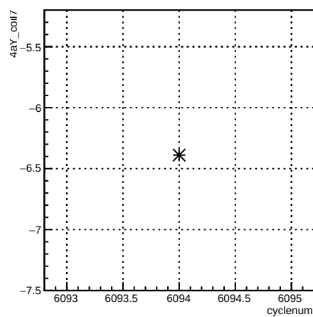
4aY_coil7:cyclenum {run == 6380}
