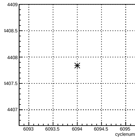
usr_coil4:cyclenum {run == 6380}
