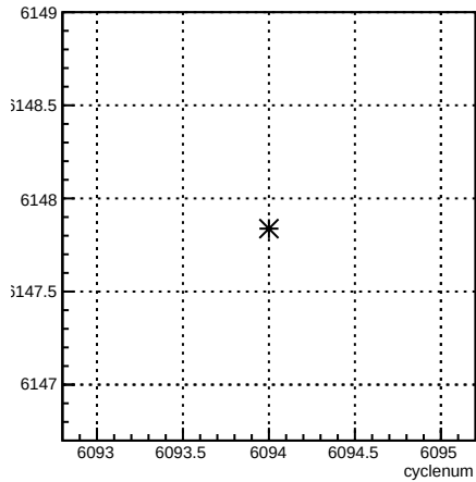
usl_coil3:cyclenum {run == 6380}
