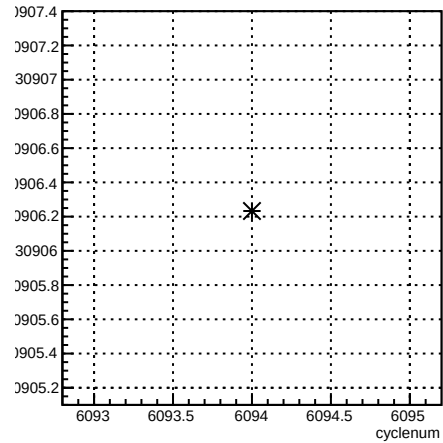
usl_coil1:cyclenum {run == 6380}
