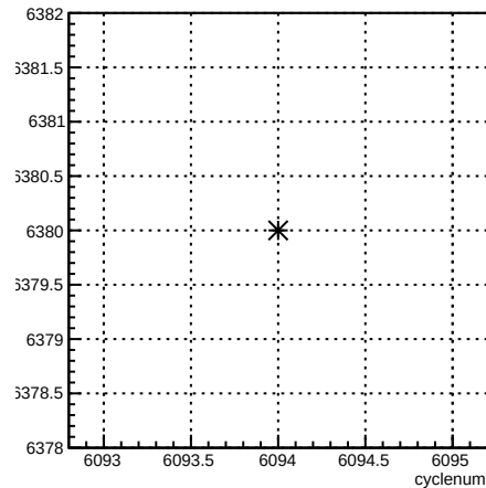
run:cyclenum {run == 6380}
