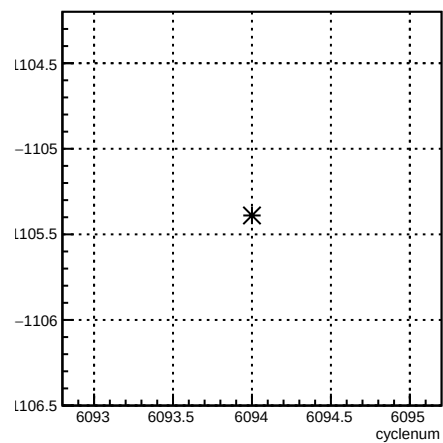
usl_coil6:cyclenum {run == 6380}
