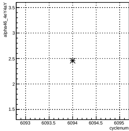
run:cyclenum {run == 6380}
