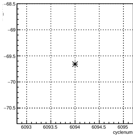
1X_coil3:cyclenum {run == 6380}
