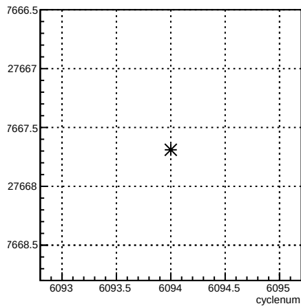
usr_coil1:cyclenum {run == 6380}
