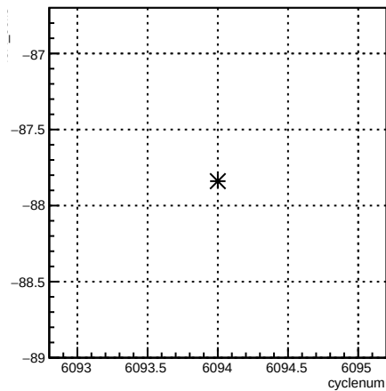
4eX_coil3:cyclenum {run == 6380}
