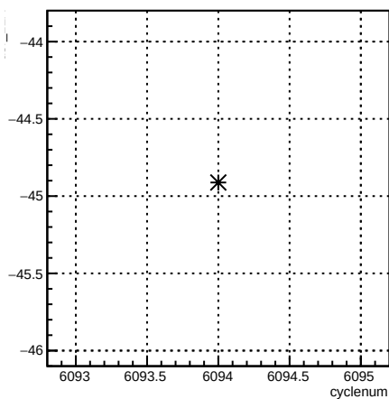
usr_12X:cyclenum {run == 6380}
