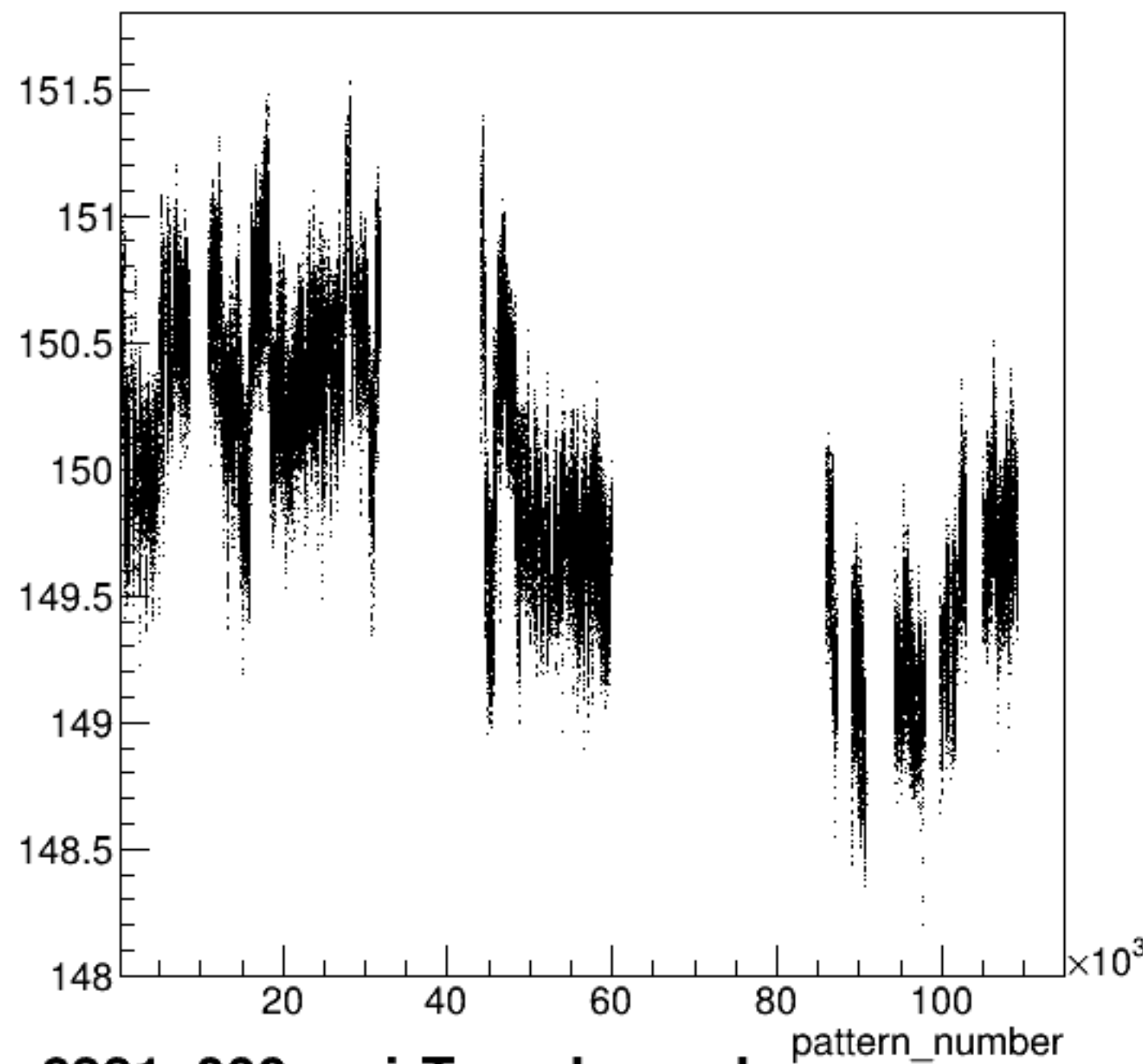
yield_bcm_dg_us:pattern_number {ErrorFlag==0}
