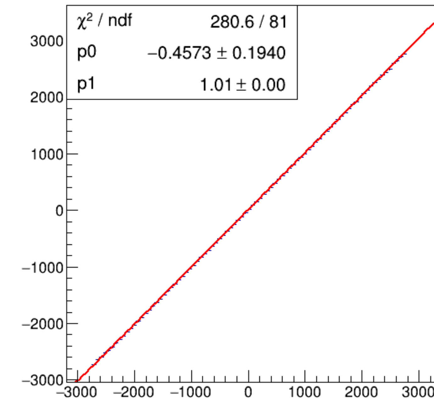
run6381_000_asym_bcm_dg_us_vs_asym_bcm_an_ds3_pr.png
