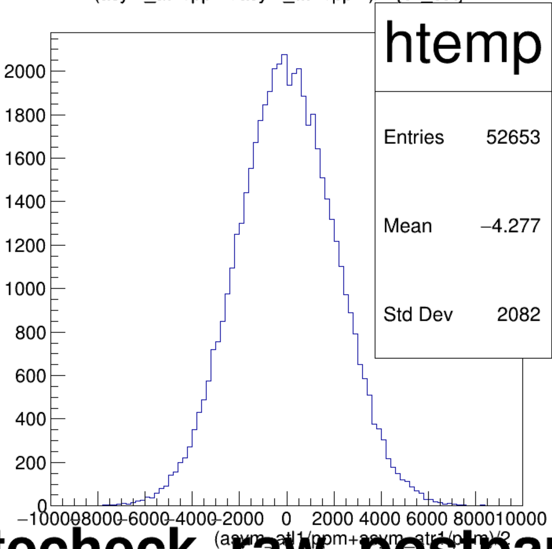
(asym_atl1/ppm+asym_atr1/ppm)/2 {ok_cut}
