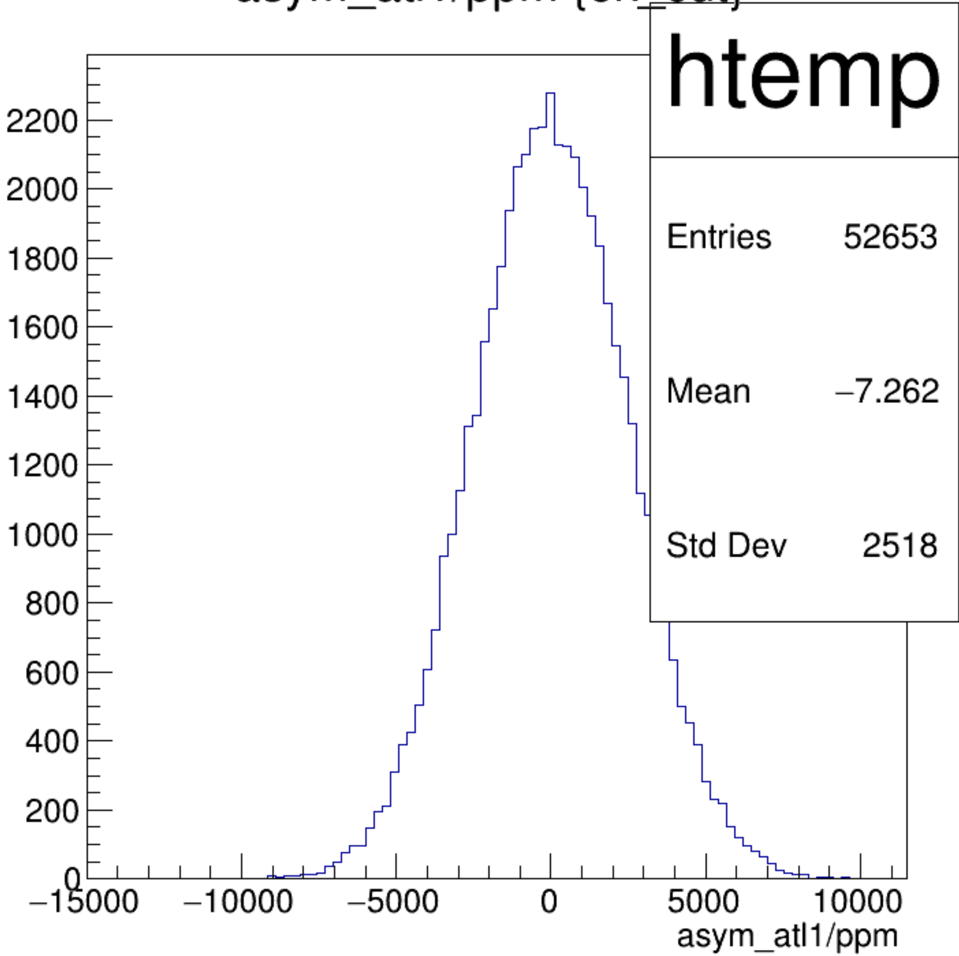
asym_atl1/ppm {ok_cut}
