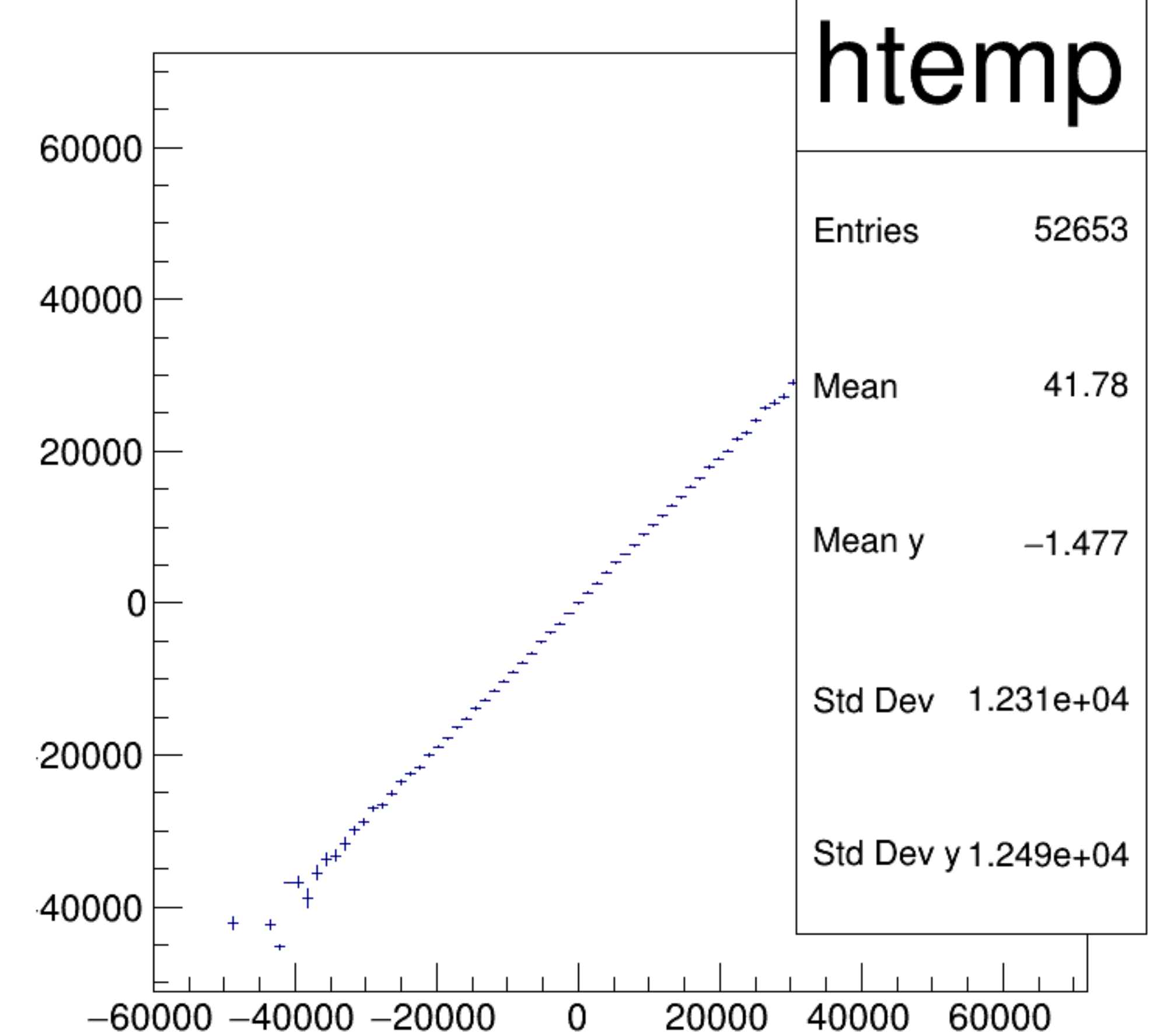
asym_atl2/ppm:asym_atr2/ppm {ok_cut}
