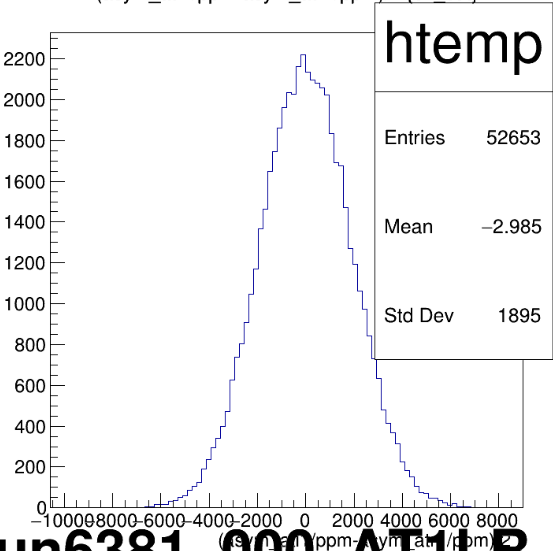
(asym_atl1/ppm-asym_atr1/ppm)/2 {ok_cut}
