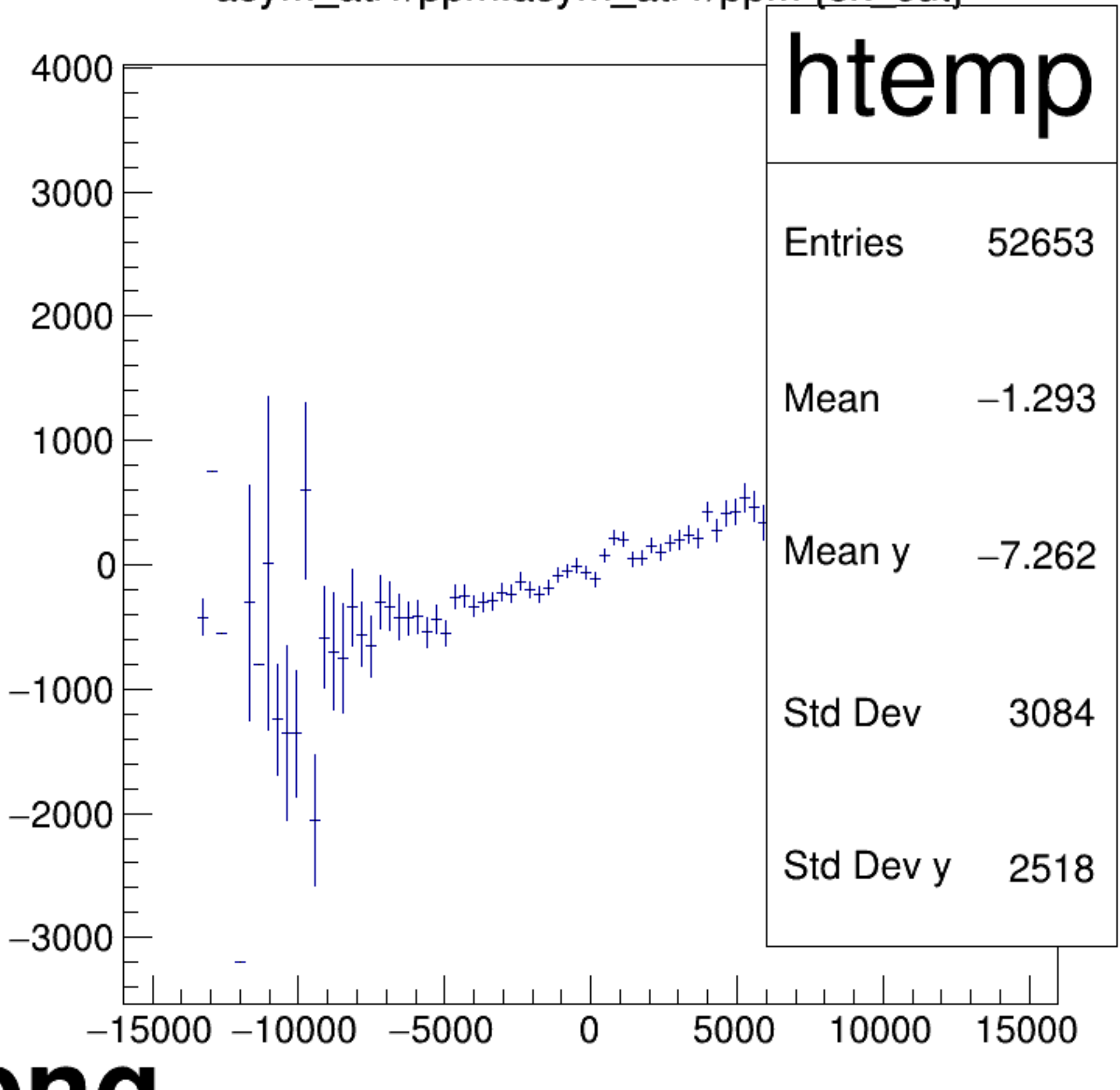
asym_atl1/ppm:asym_atr1/ppm {ok_cut}
