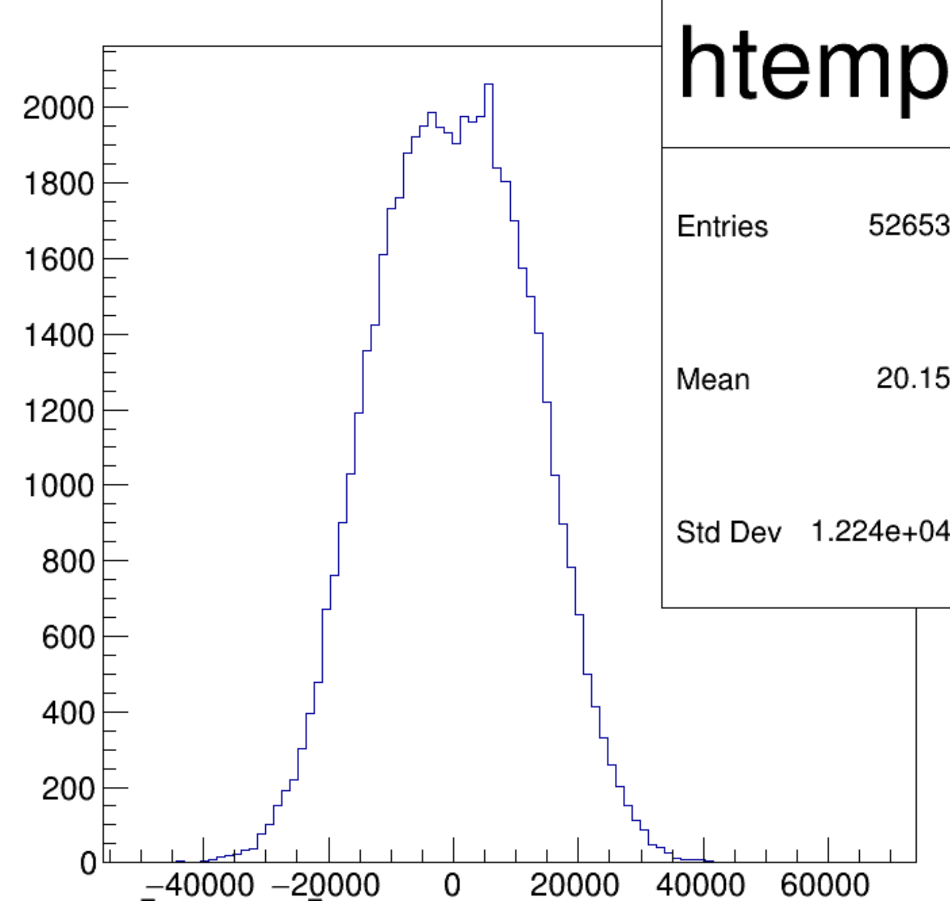
(asym_atl2/ppm+asym_atr2/ppm)/2 {ok_cut}
