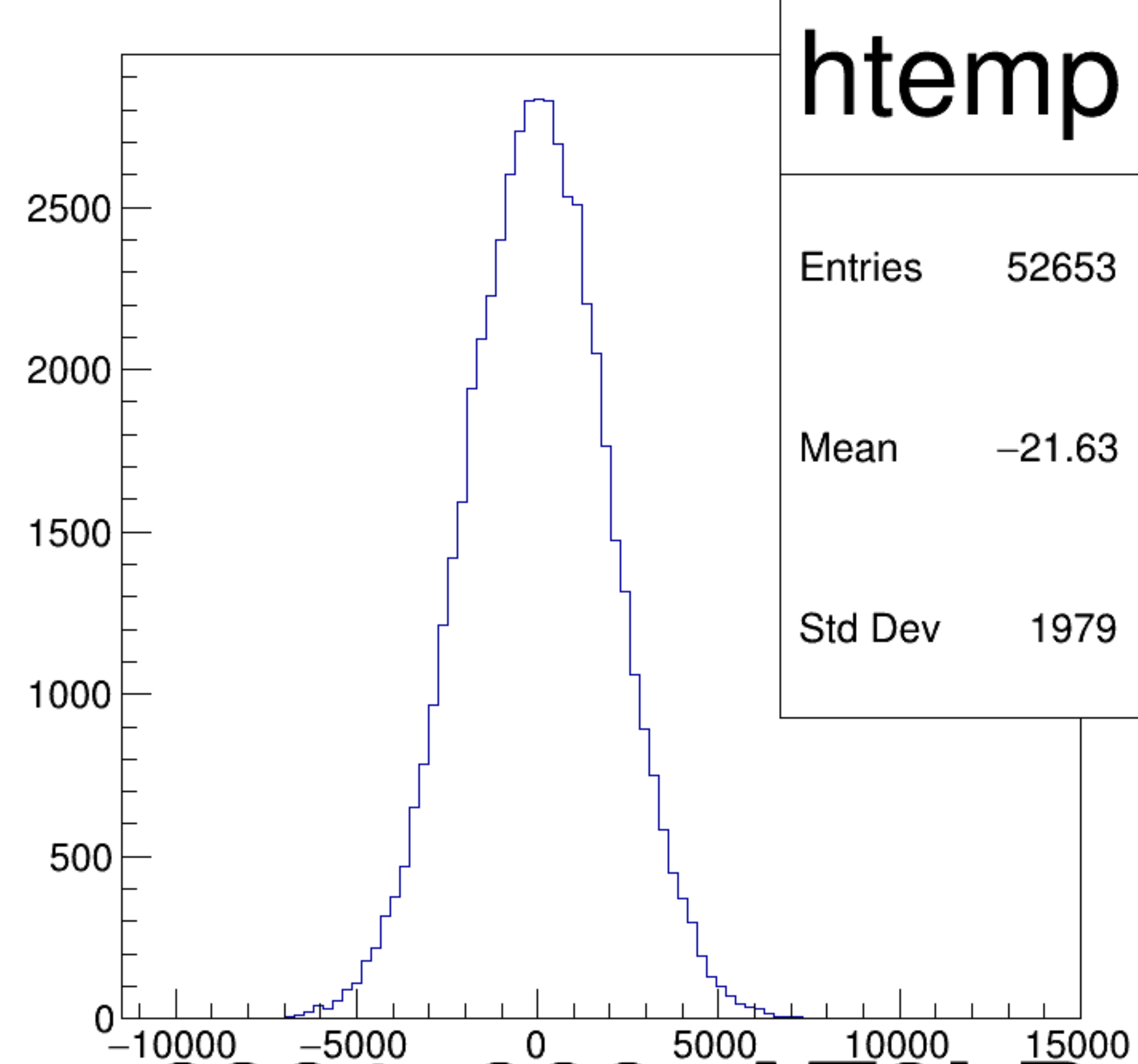
(asym_atl2/ppm-asym_atr2/ppm)/2 {ok_cut}
