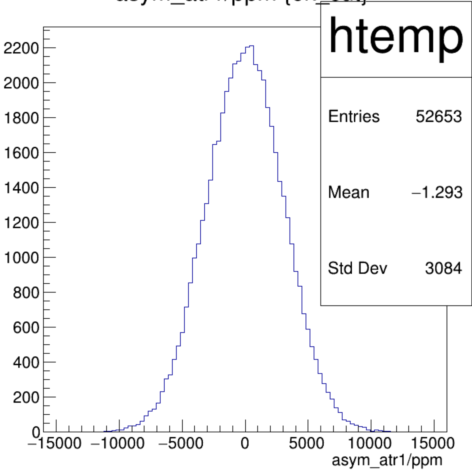
asym_atr1/ppm {ok_cut}
