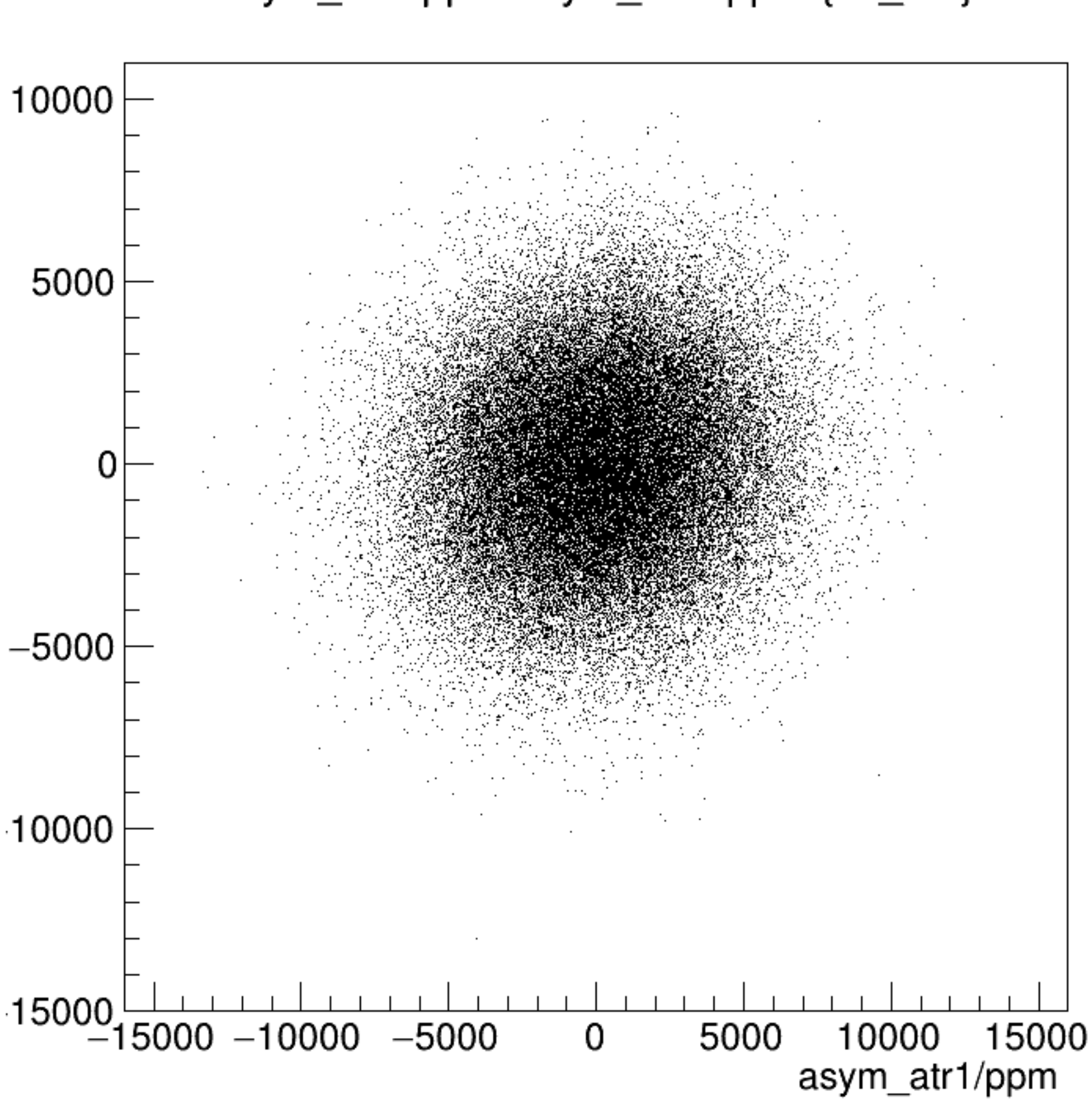
asym_atl1/ppm:asym_atr1/ppm {ok_cut}
