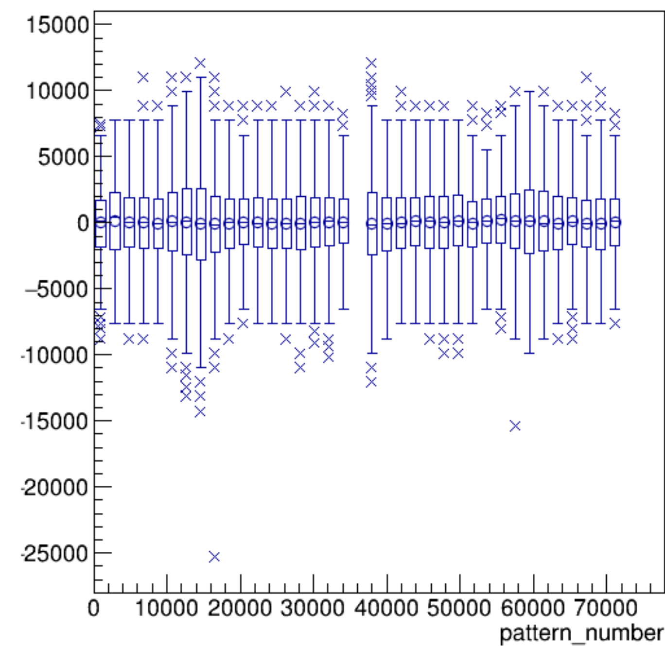
asym_sam2/ppm:pattern_number {ErrorFlag==0}
