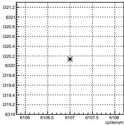
usl_coil7:cyclenum {run == 6383}
