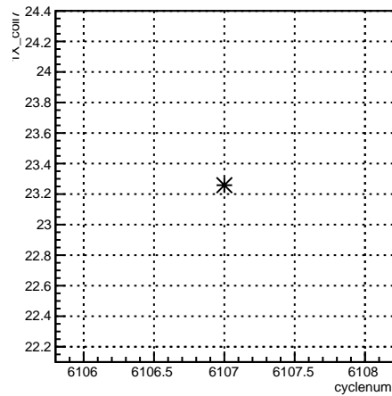
1X_coil7:cyclenum {run == 6383}
