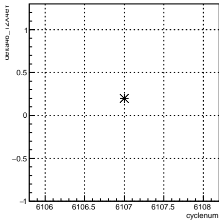
delta46_12X4eY:cyclenum {run == 6383}
