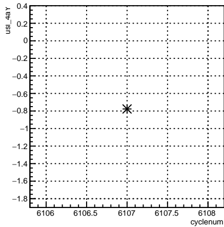
usl_4aY:cyclenum {run == 6383}
