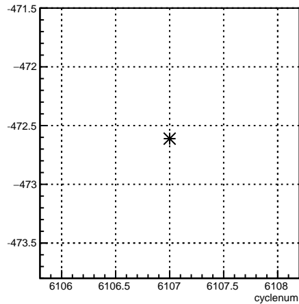
4eX_coil1:cyclenum {run == 6383}
