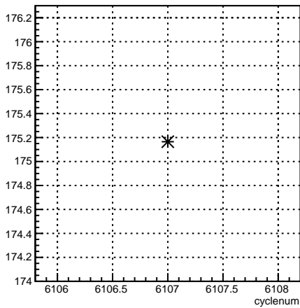
4eY_coil4:cyclenum {run == 6383}
