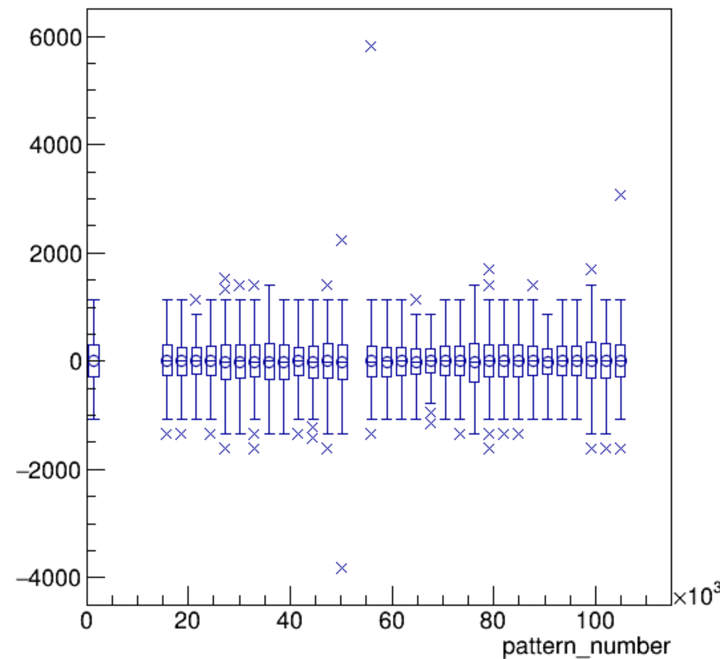
asym_sam8/ppm:pattern_number {ErrorFlag==0}
