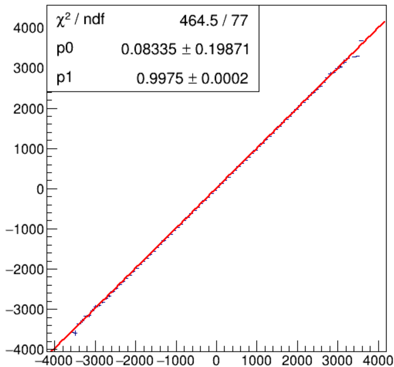
run6384_000_asym_bcm_dg_us_vs_asym_bcm_dg_ds_pr.png
