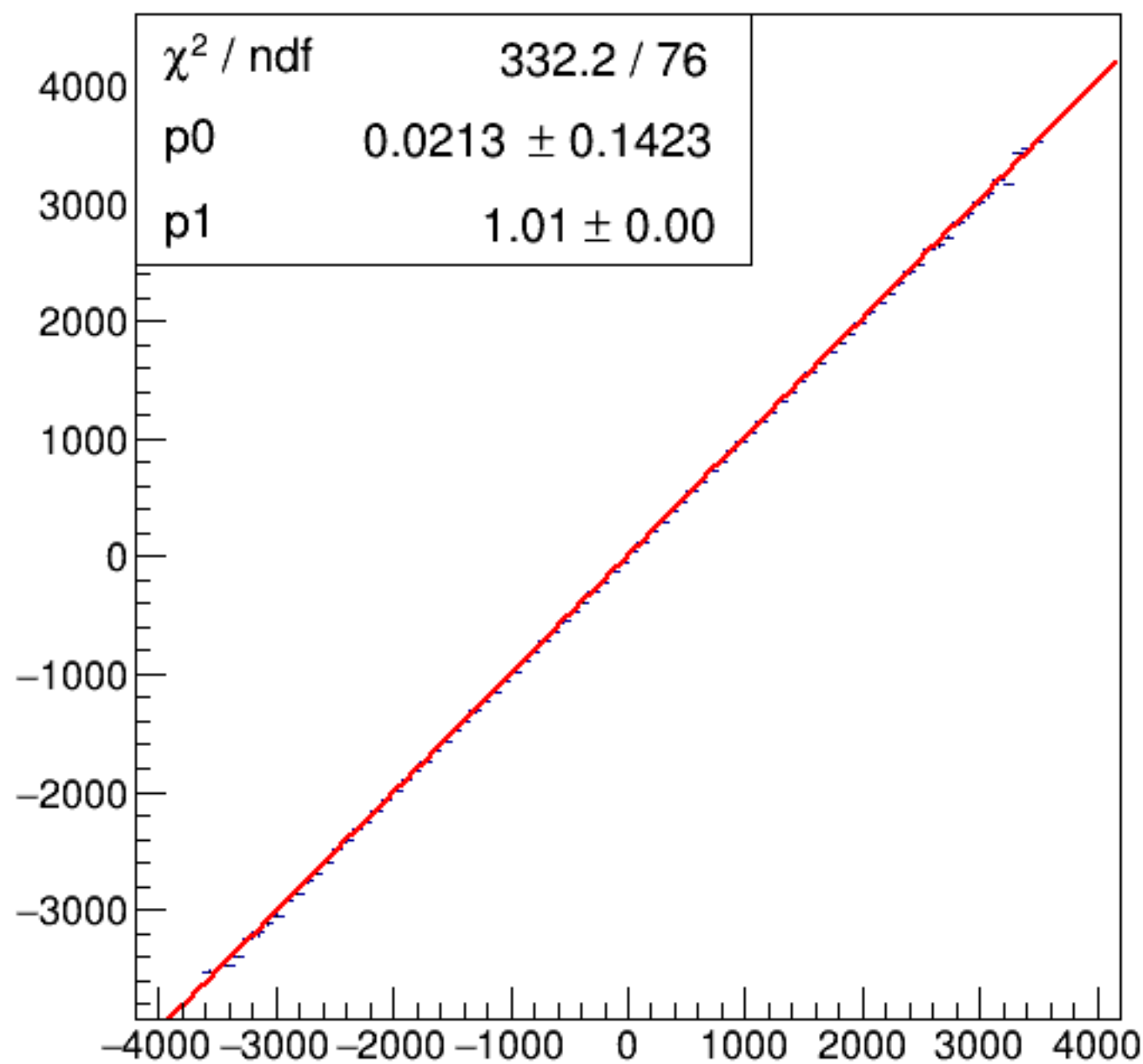
run6384_000_asym_bcm_dg_ds_vs_asym_bcm_an_us_pr.png
