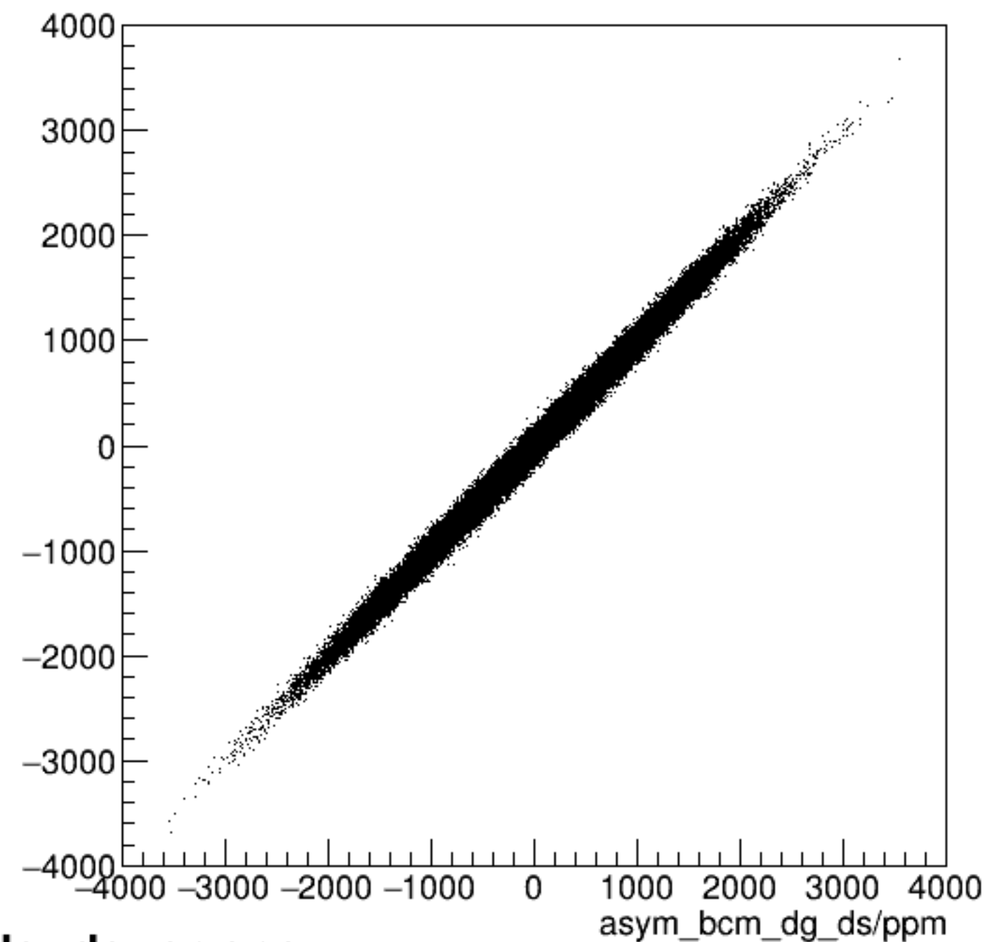
run6384_000_asym_bcm_dg_us_vs_asym_bcm_dg_ds_pr.png
