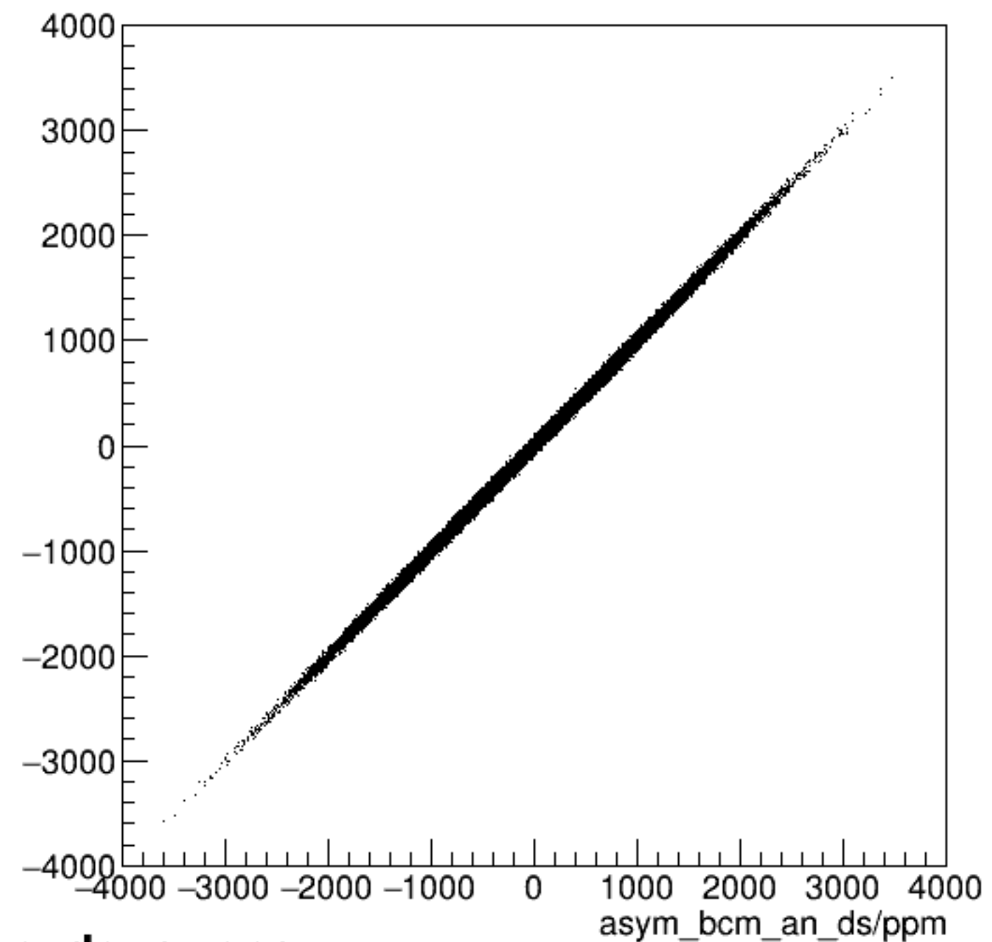
run6384_000_asym_bcm_an_us_vs_asym_bcm_an_ds_pr.png
