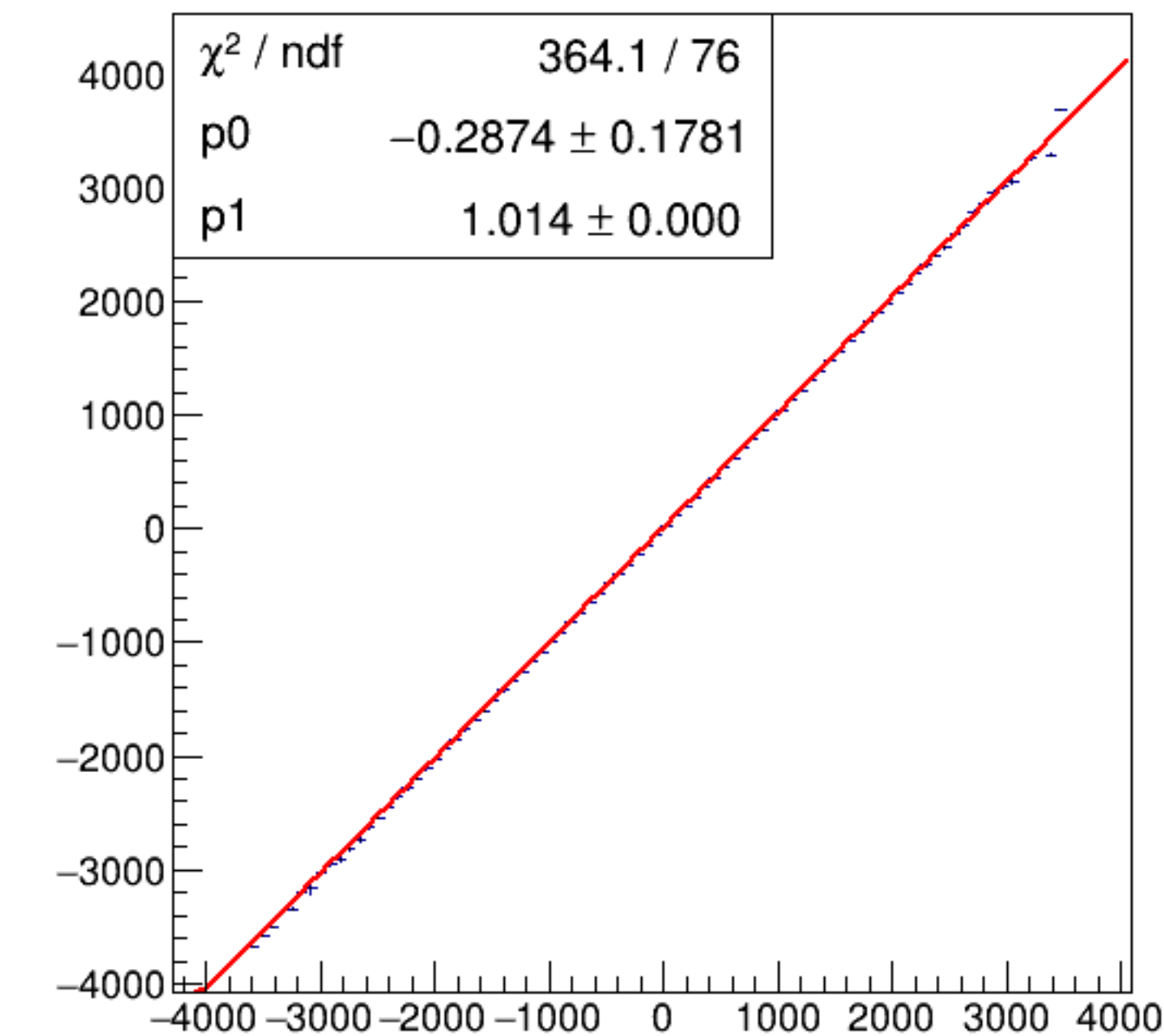
run6384_000_asym_bcm_dg_us_vs_asym_bcm_an_ds_pr.png
