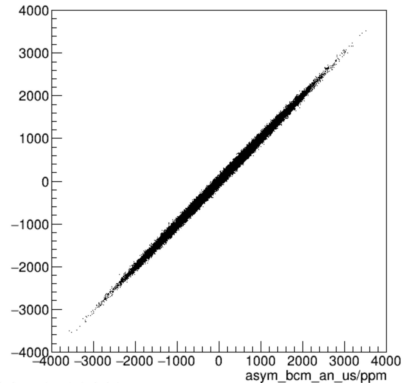
run6384_000_asym_bcm_dg_ds_vs_asym_bcm_an_us_pr.png
