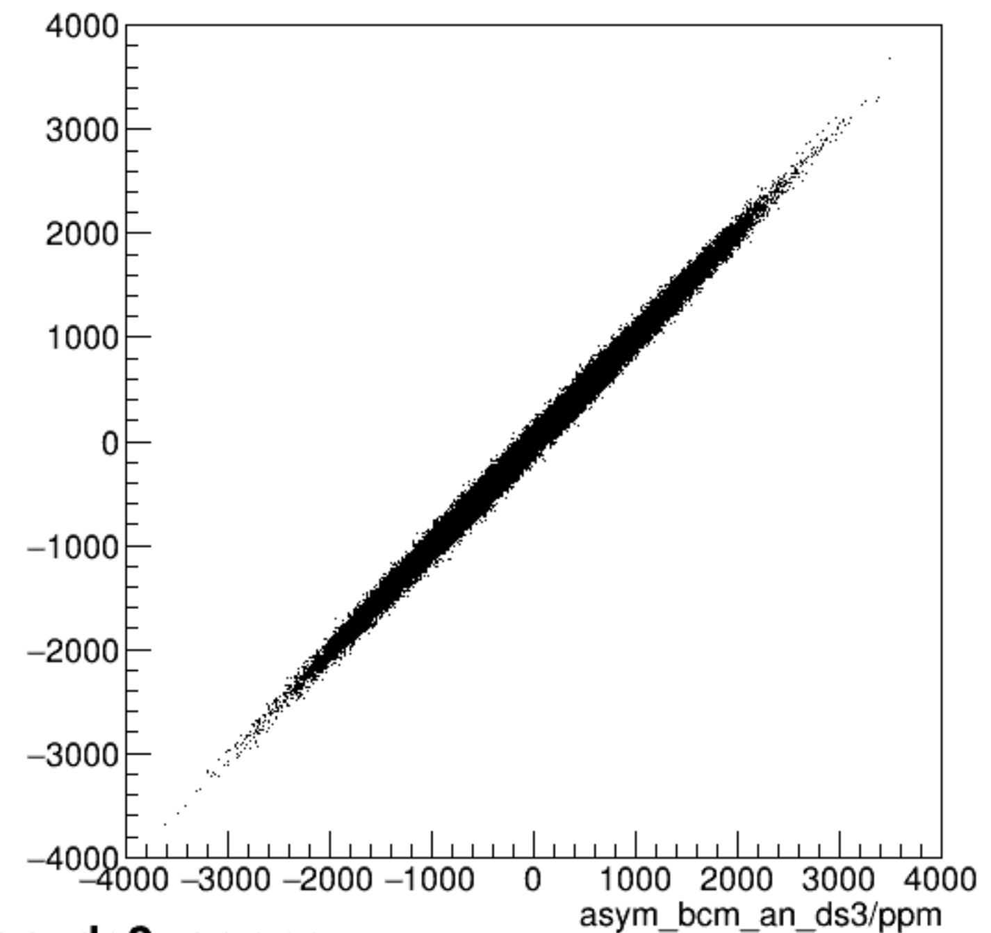
run6384_000_asym_bcm_dg_us_vs_asym_bcm_an_ds3_pr.png
