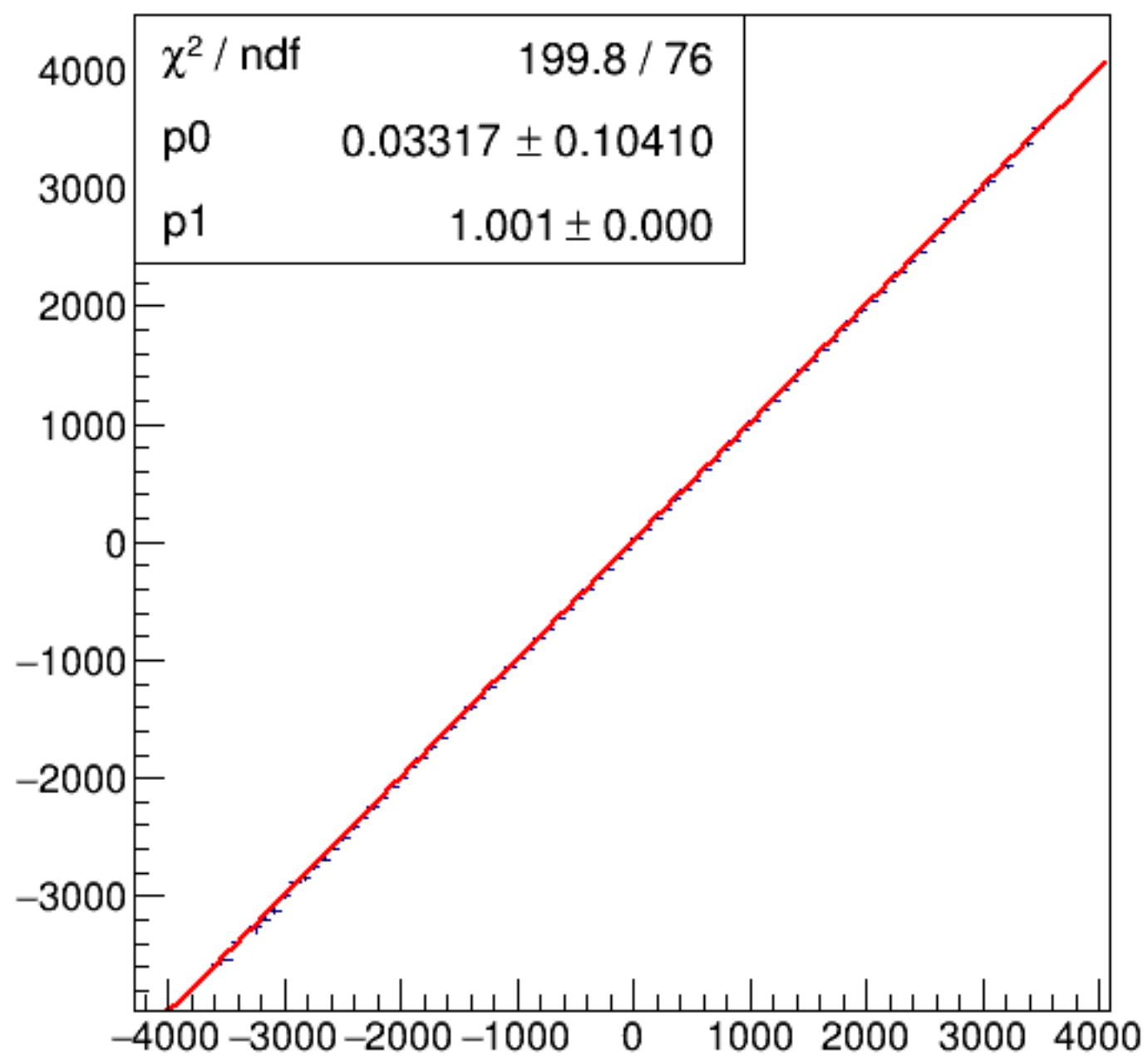
run6384_000_asym_bcm_an_us_vs_asym_bcm_an_ds_pr.png
