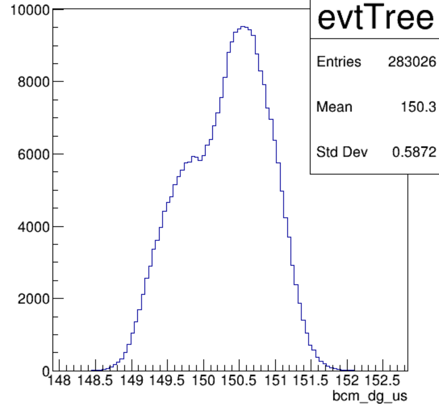
bcm_dg_us {ErrorFlag==0}
