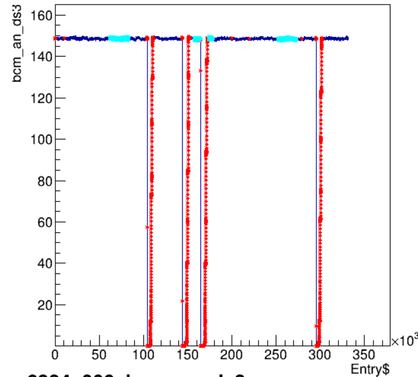
bcm_an_ds3:Entry$
