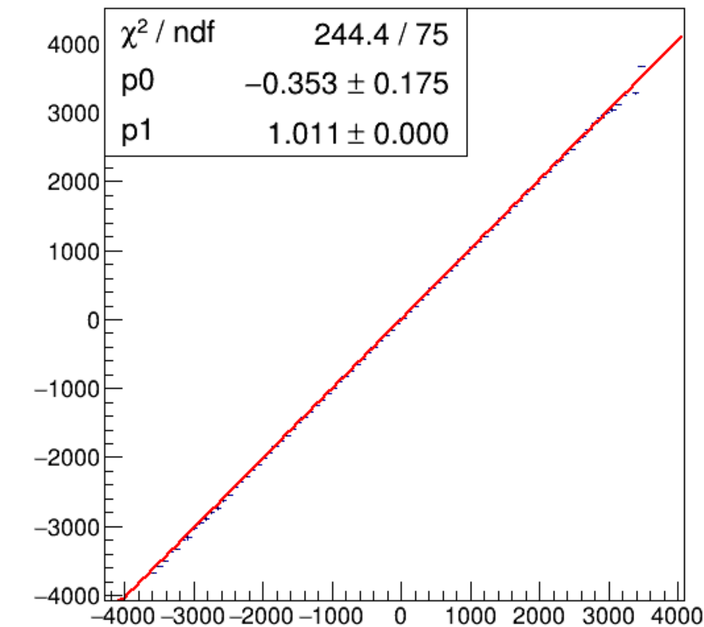
run6384_000_asym_bcm_dg_us_vs_asym_bcm_an_ds3_pr.png
