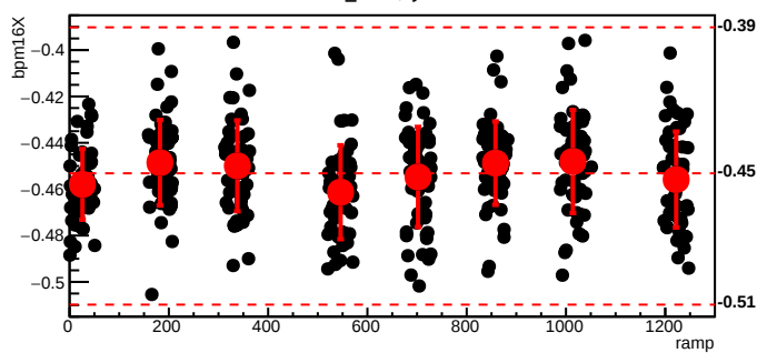
bmod_trim4,cyc=6114
