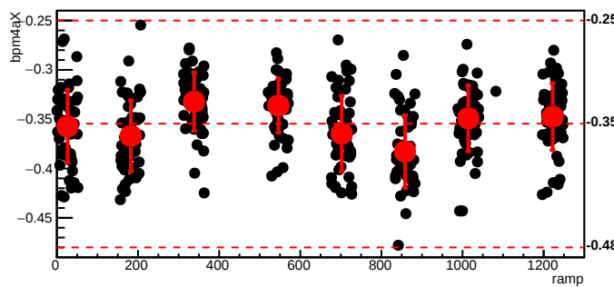
bmod_trim6,cyc=6114
