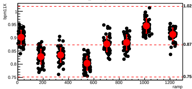
bmod_trim3,cyc=6114
