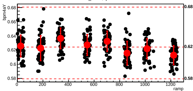
bmod_trim3,cyc=6113
