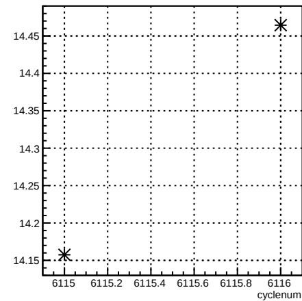
usr_4eY:cyclenum {run == 6385}
