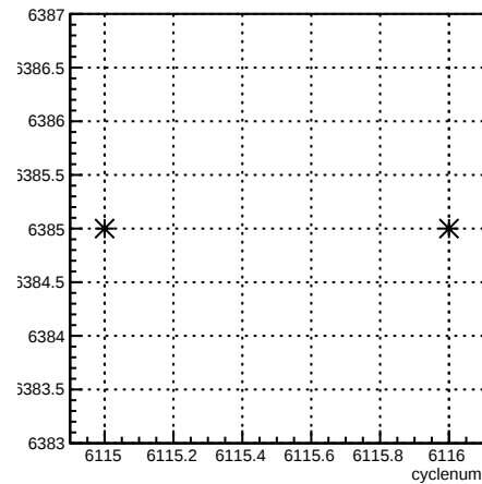
run:cyclenum {run == 6385}
