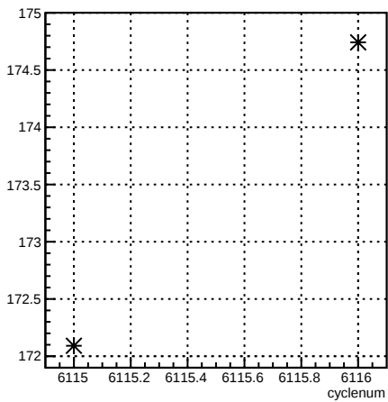
4aY_coil4:cyclenum {run == 6385}
