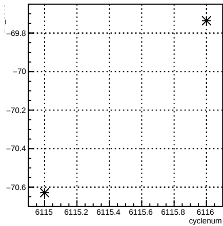
4eX_coil3:cyclenum {run == 6385}
