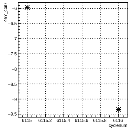
4eY_coil7:cyclenum {run == 6385}
