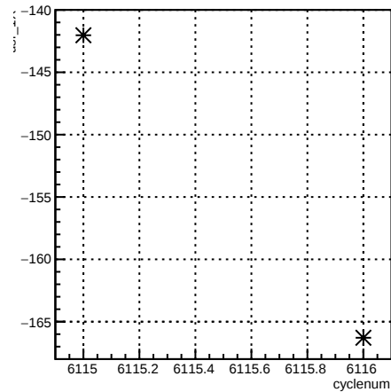
usr_1X:cyclenum {run == 6385}
