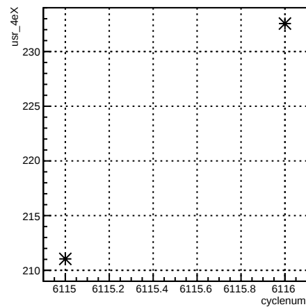
usr_4eX:cyclenum {run == 6385}
