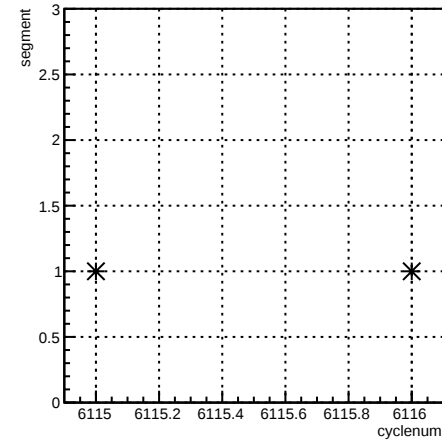
segment:cyclenum {run == 6385}
