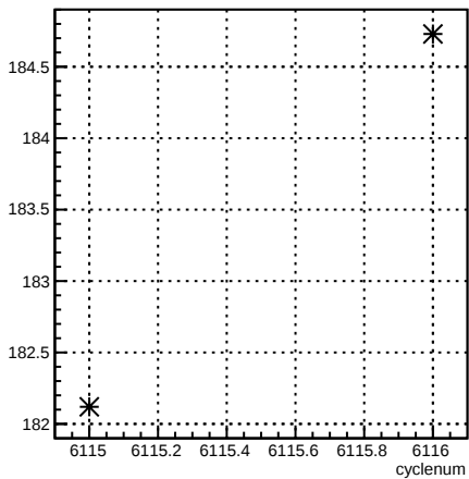
4eY_coil4:cyclenum {run == 6385}
