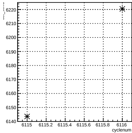
usl_coil7:cyclenum {run == 6385}
