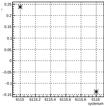
usl_12X:cyclenum {run == 6385}
