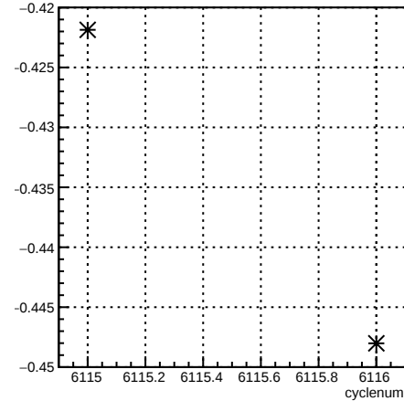
delta13_12X4eX:cyclenum {run == 6385}
