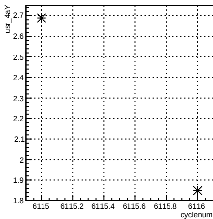
usr_4aY:cyclenum {run == 6385}
