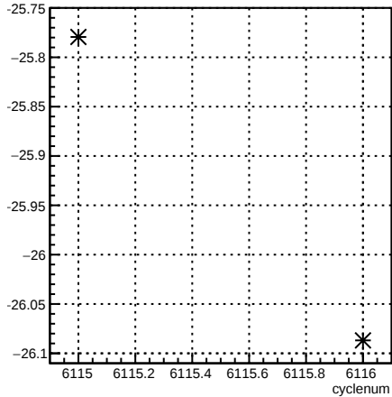
4eY_coil6:cyclenum {run == 6385}
