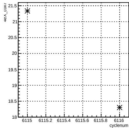
4eX_coil7:cyclenum {run == 6385}
