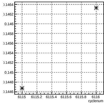
alpha13_4eX1X:cyclenum {run == 6385}
