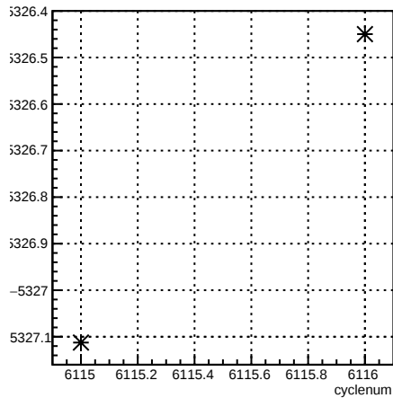
usr_coil3:cyclenum {run == 6385}
